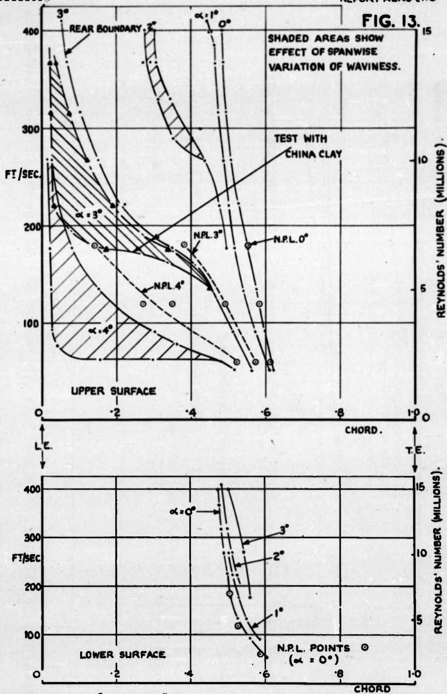
TRANSITION "FRONT" ON BOULTON PAUL WING IN THE R.A.E. No. 2-11½ FT. WIND TUNNEL.
