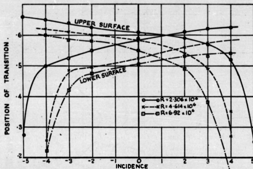
FIG. 4: VARIATION OF TRANSITION POINT WITH INCIDENCE.
