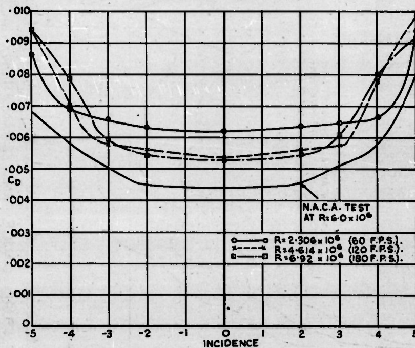
FIG. 5: VARIATION OF DRAG COEFFICIENT WITH INCIDENCE.
