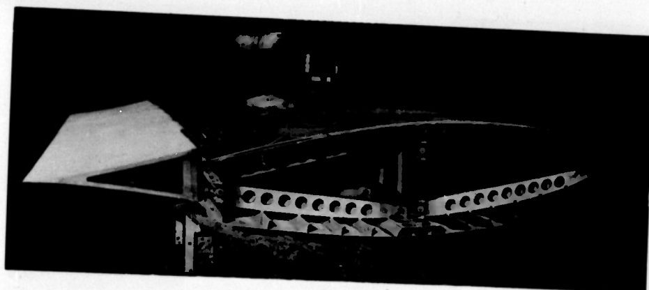
FIG. 11. TEST SECTION OF WING, SHOWING POLISHED SKIN AND INTERNAL STRUCTURE
