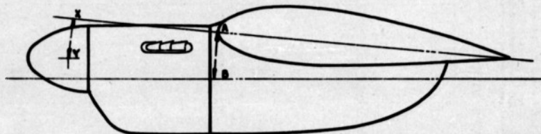
NACELLE C3 : THRUST LINE AT -5^\circ TO WING CHORD : C3 (-5)
