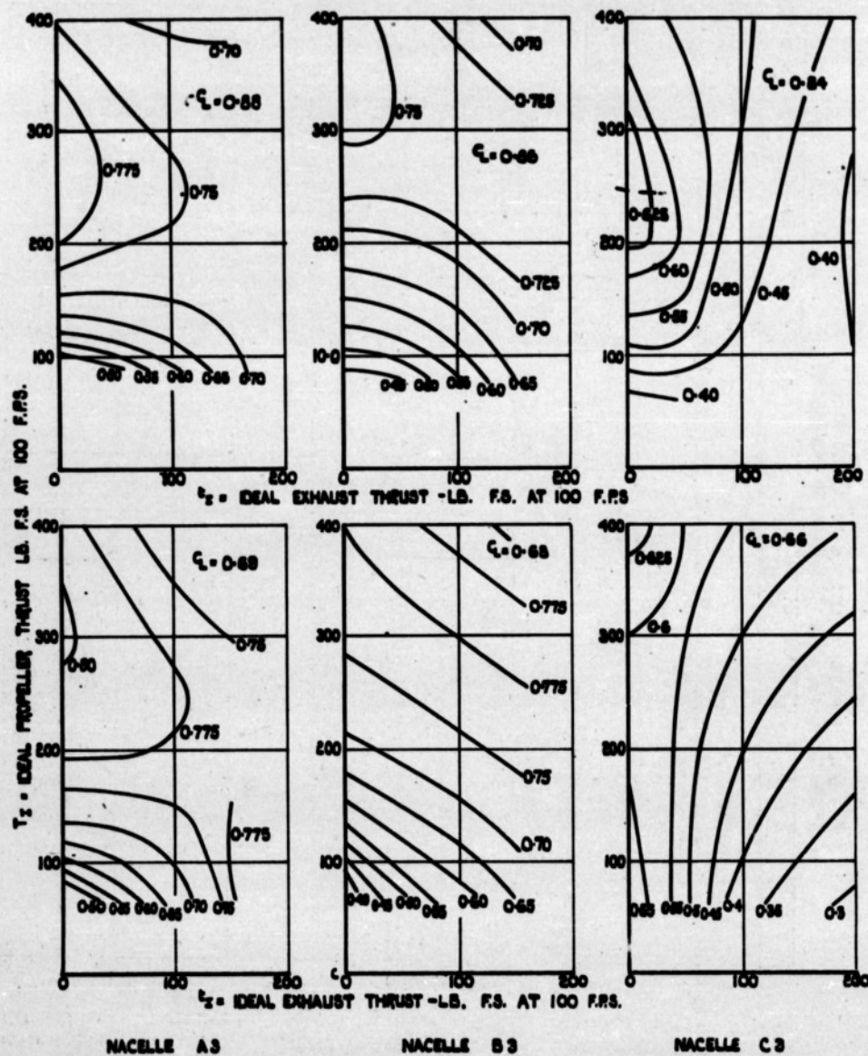
NACELLE WITH THRUST LINE AT -5^\circ TO CHORD LINE - HIGH EXHAUST POSITION CONTOURS OF NET OVERALL EFFICIENCY FOR INFINITE ASPECT RATIO.
