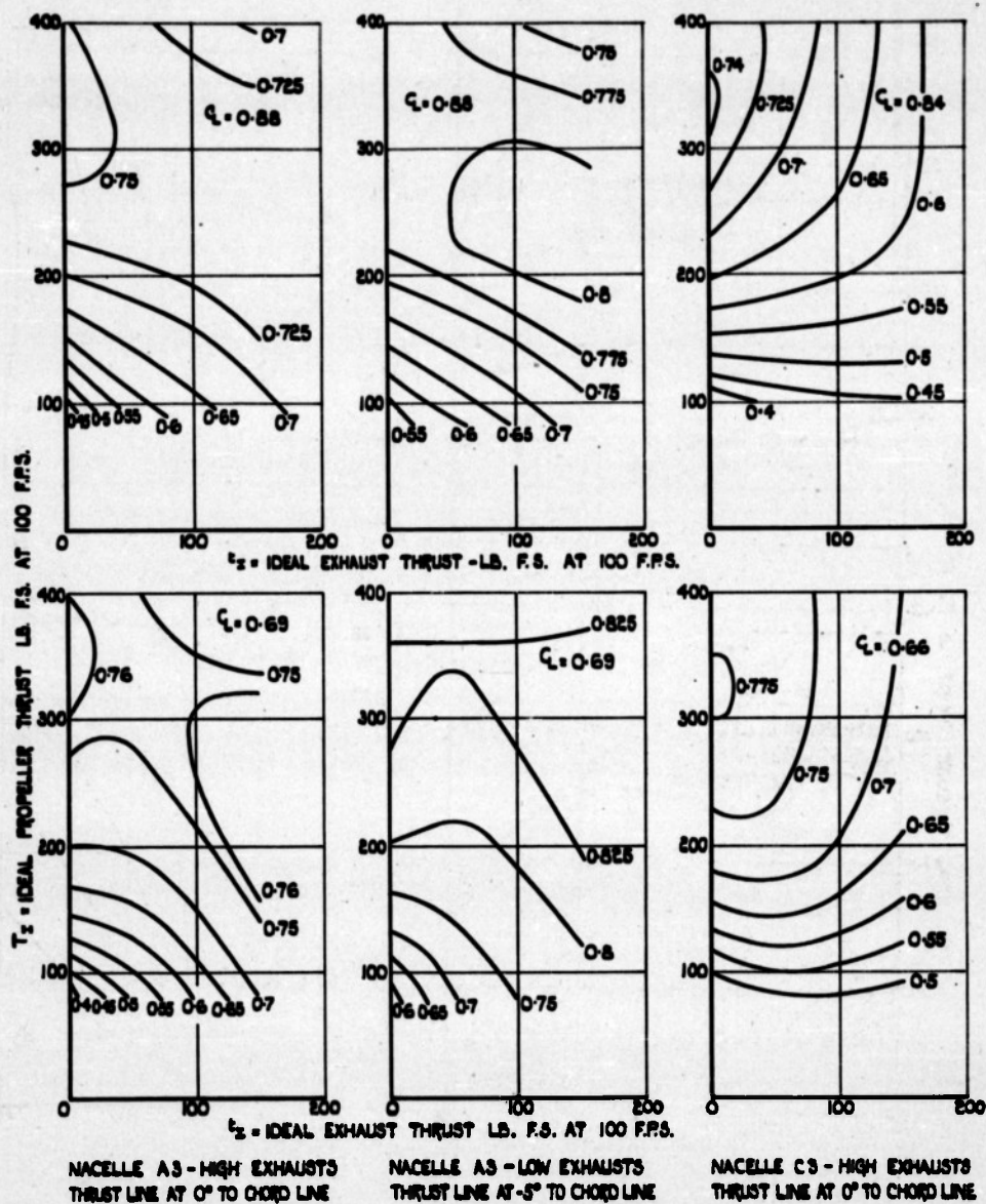
CONTOURS OF NET OVERALL EFFICIENCY FOR INFINITE ASPECT RATIO.
