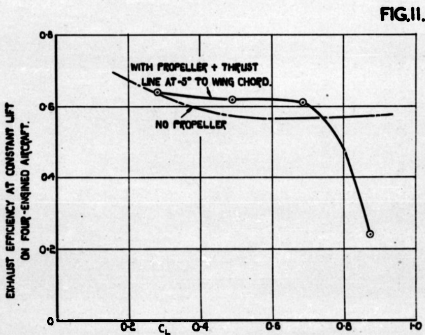
EXHAUST EFFICIENCY - NACELLE C3 - HIGH EXHAUSTS - 800 B.H.P.
