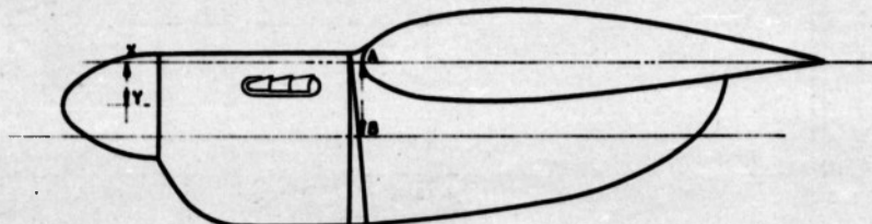
NACELLE C3 : THRUST LINE AT 0^\circ TO WING CHORD : C3 (0)
