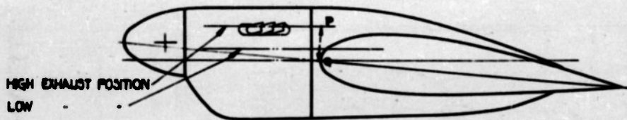
NACELLE A3 : THRUST LINE AT -5^\circ TO WING CHORD : A3 (-5)
