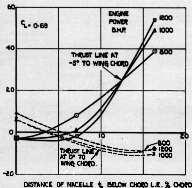
NACELLE + PROPELLER INTERFERENCE DRAG.
