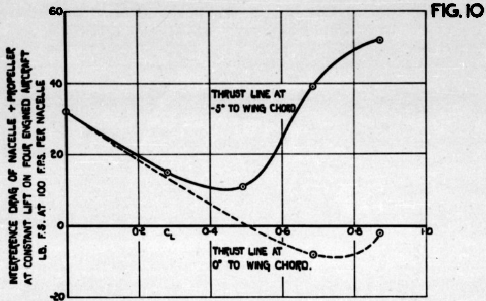
NACELLE + PROPELLER INTERFERENCE DRAG-NACELLE C3 ENGINE POWER = 800 B.H.P.
