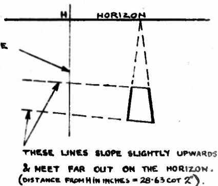
FIG. 4. VIEW FROM POSITION A. AIRCRAFT HEADING 2^\circ TO LEFT, NO BANK.
