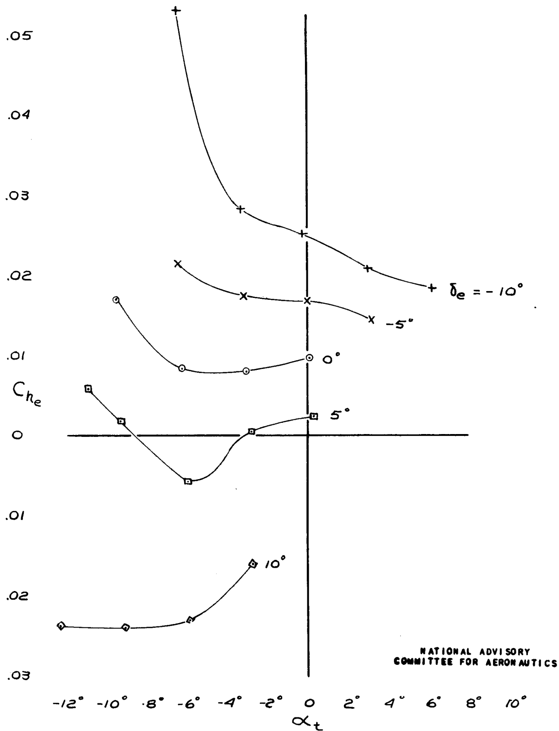
(4) METAL-COVERED ELEVATOR FIGURE 9.- CONCLUDED.
