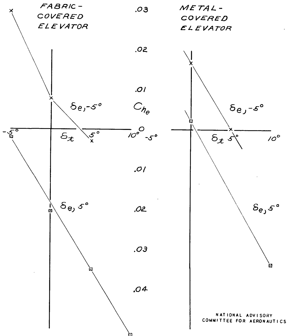
FIGURE 34.-VARIATION OF ELEVATOR HINGE-MOMENT COEFFICIENT WITH TAB ANGLE. M, 0.33; \alpha_t, 0^\circ
