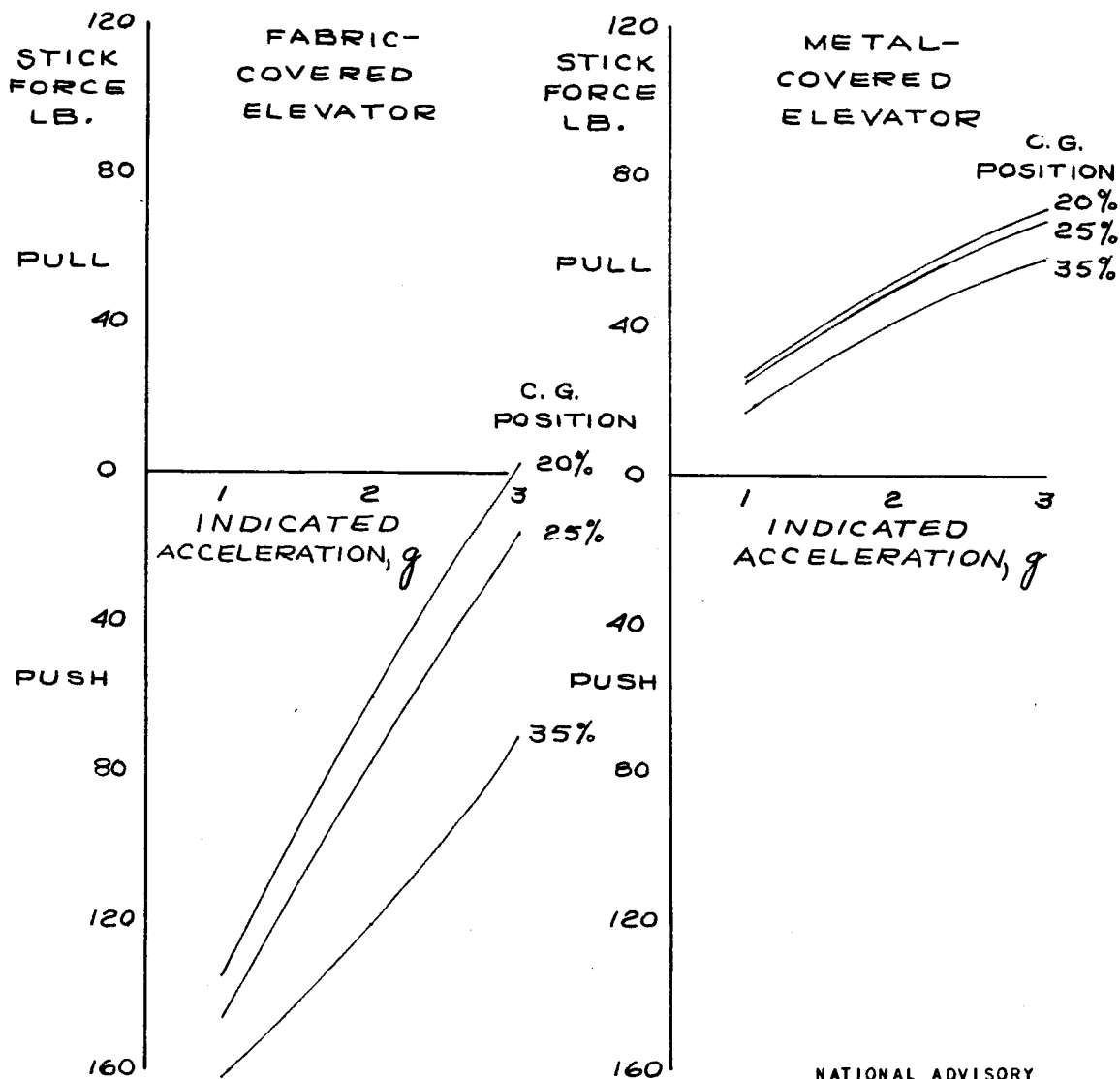
(Q) SEA LEVEL FIGURE 19.- VARIATION OF ELEVATOR STICK FORCE WITH INDICATED ACCELERATION AT M, 0.72; \delta_t, 0^\circ
