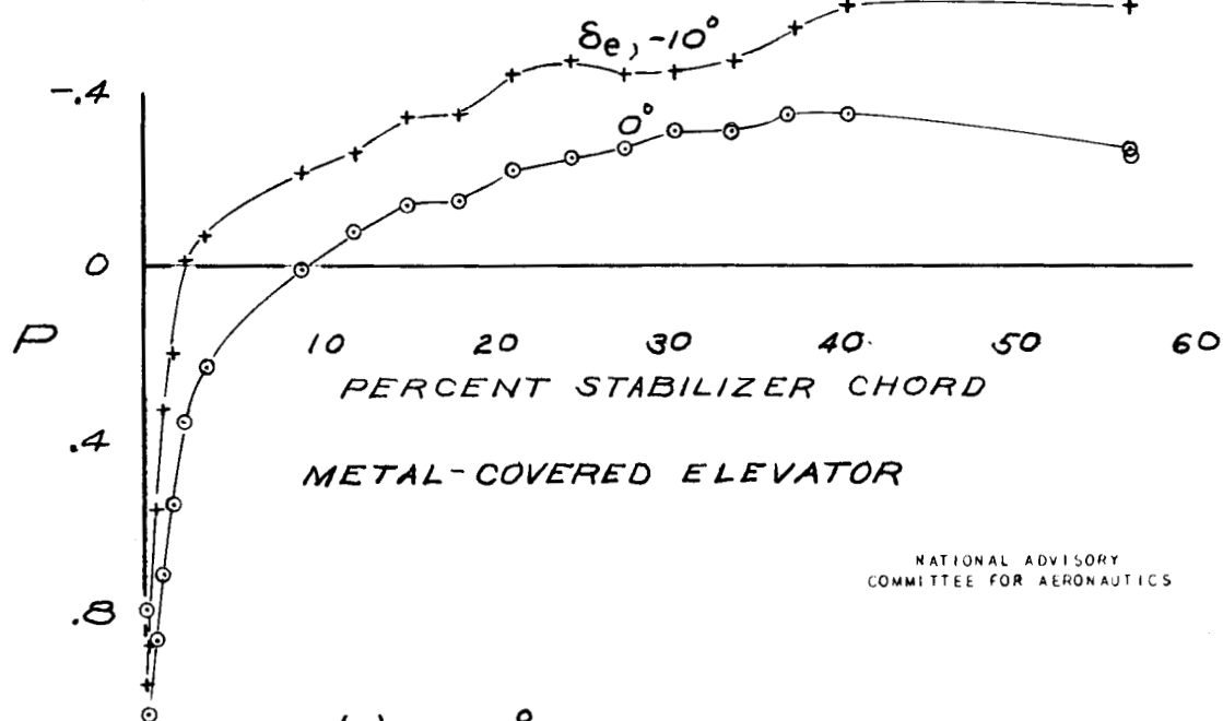
FIGURE 20.-VARIATION OF PRESSURE COEFFICIENT WITH CHORDWISE STATION ON THE LOWER SURFACE. M, 0.33 ; \delta_x, 0^\circ ; STATION 92.
