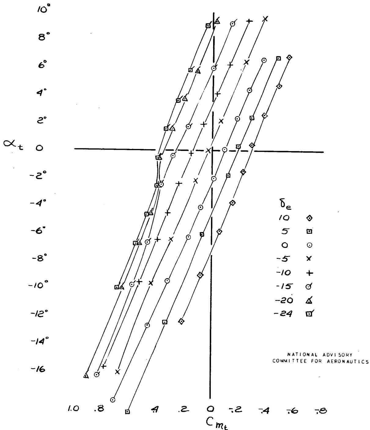
(b) METAL-COVERED ELEVATOR FIGURE 6.- CONCLUDED.
