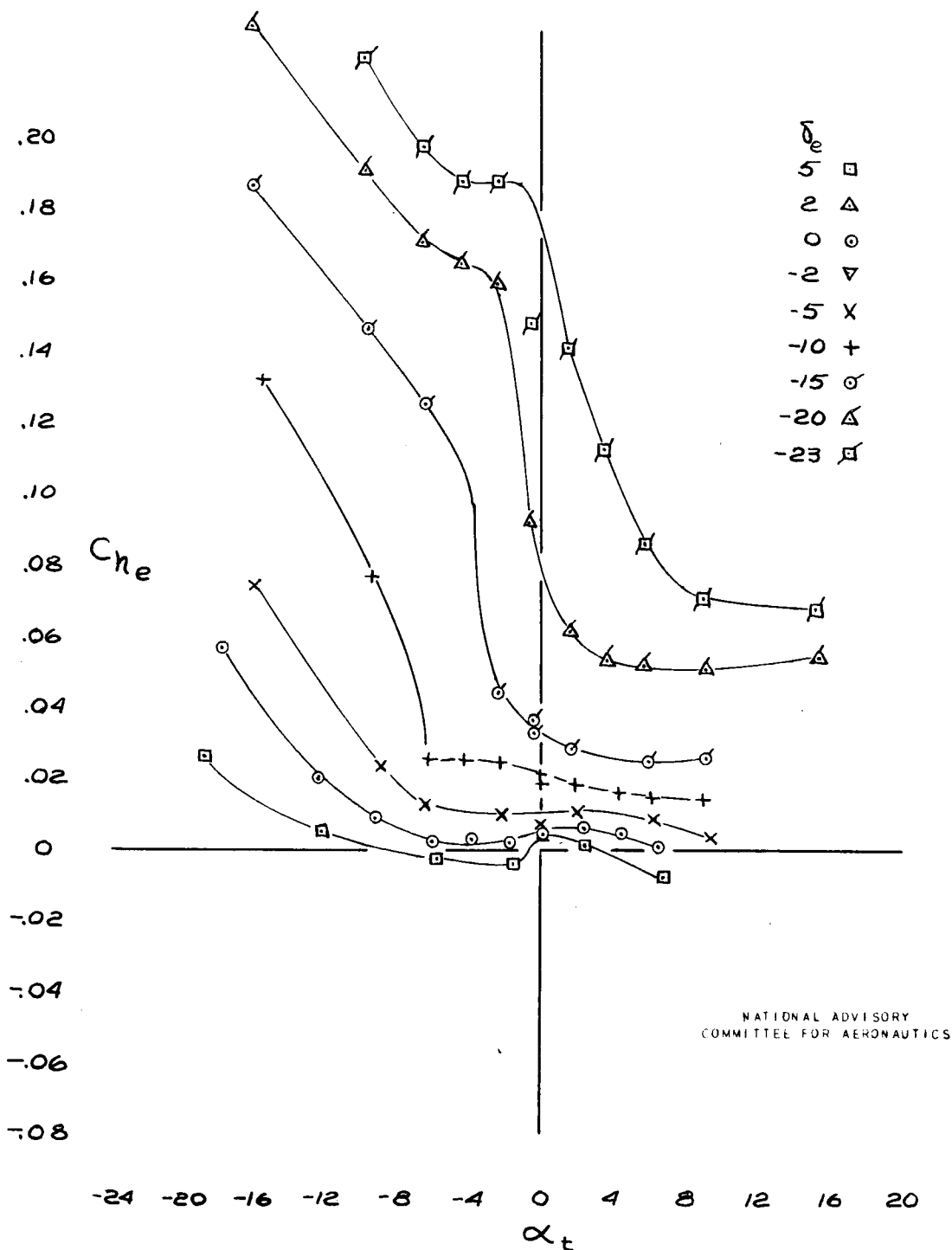
(6) METAL-COVERED ELEVATOR FIGURE 5. - CONCLUDED.
