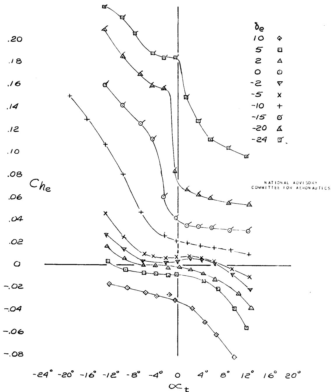
(Q.) FABRIC-COVERED ELEVATOR FIGURE 5. - VARIATION OF HINGE-MOMENT COEFFICIENT WITH TAIL ANGLE OF ATTACK. M, 0.133 ; \delta_t, 0^\circ .
