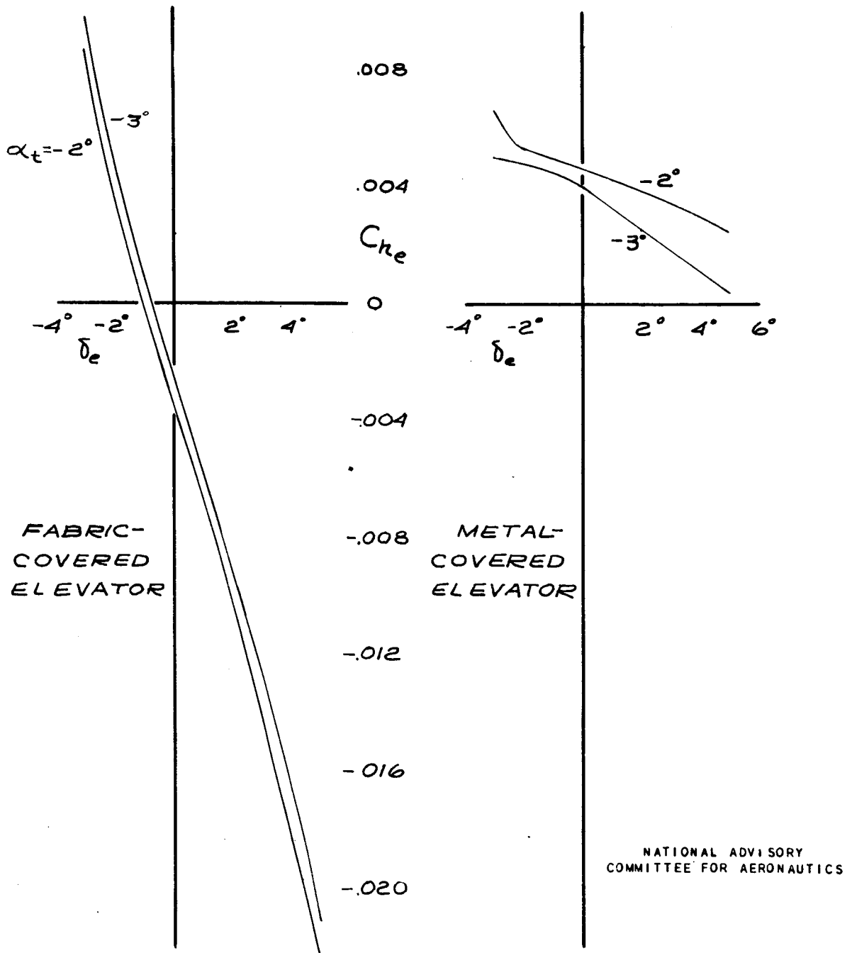
FIGURE 17.- VARIATION OF ELEVATOR HINGE-MOMENT COEFFICIENT WITH ELEVATOR ANGLE. M, 0.72 ; \delta_t, 0^\circ .
