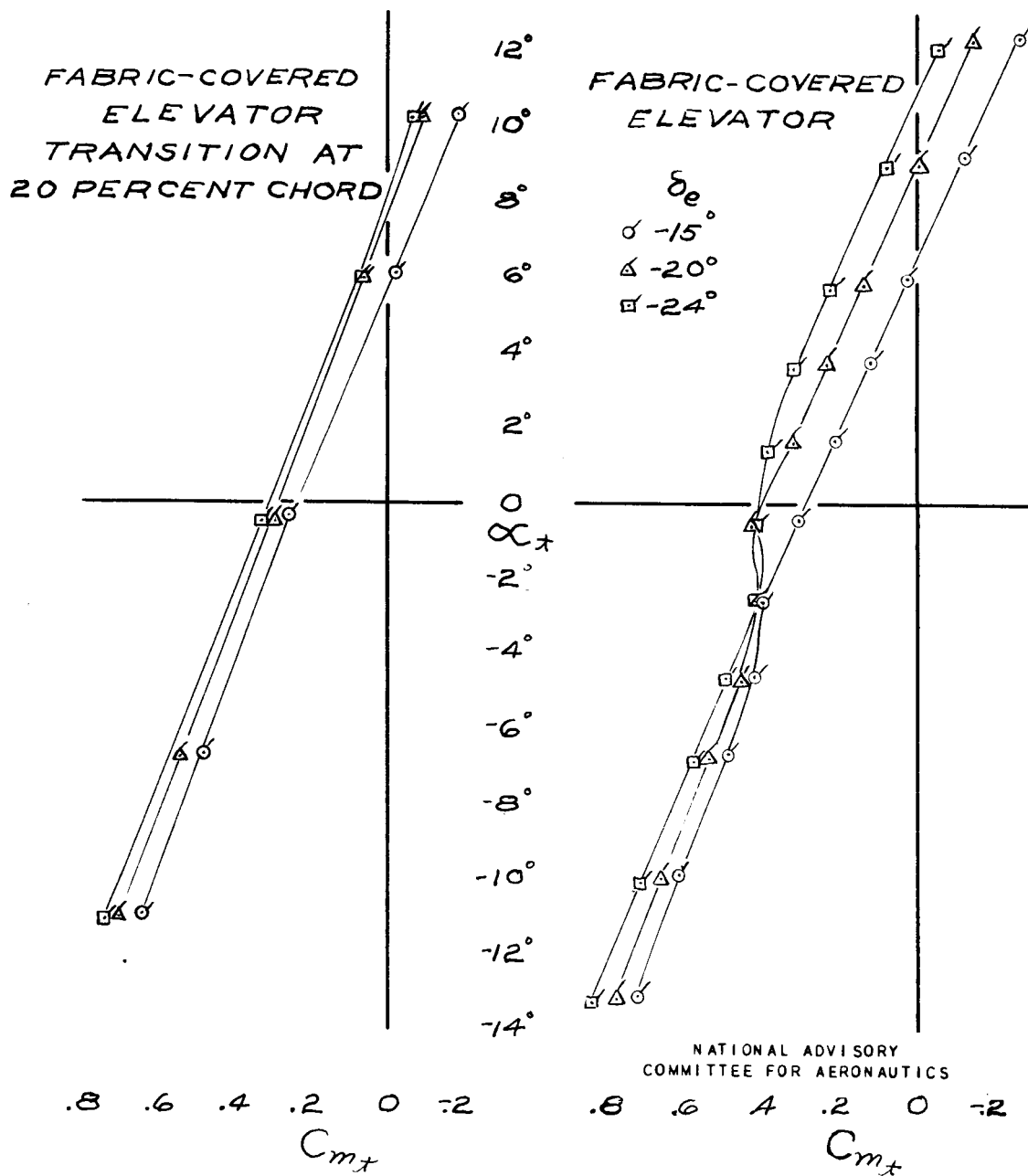
FIGURE 38.- VARIATION OF PITCHING-MOMENT COEFFICIENT DUE TO THE TAIL WITH TAIL ANGLE OF ATTACK, WITH AND WITHOUT TRANSITION FIXED; M, 0.133 ; \delta_t, 0^\circ .
