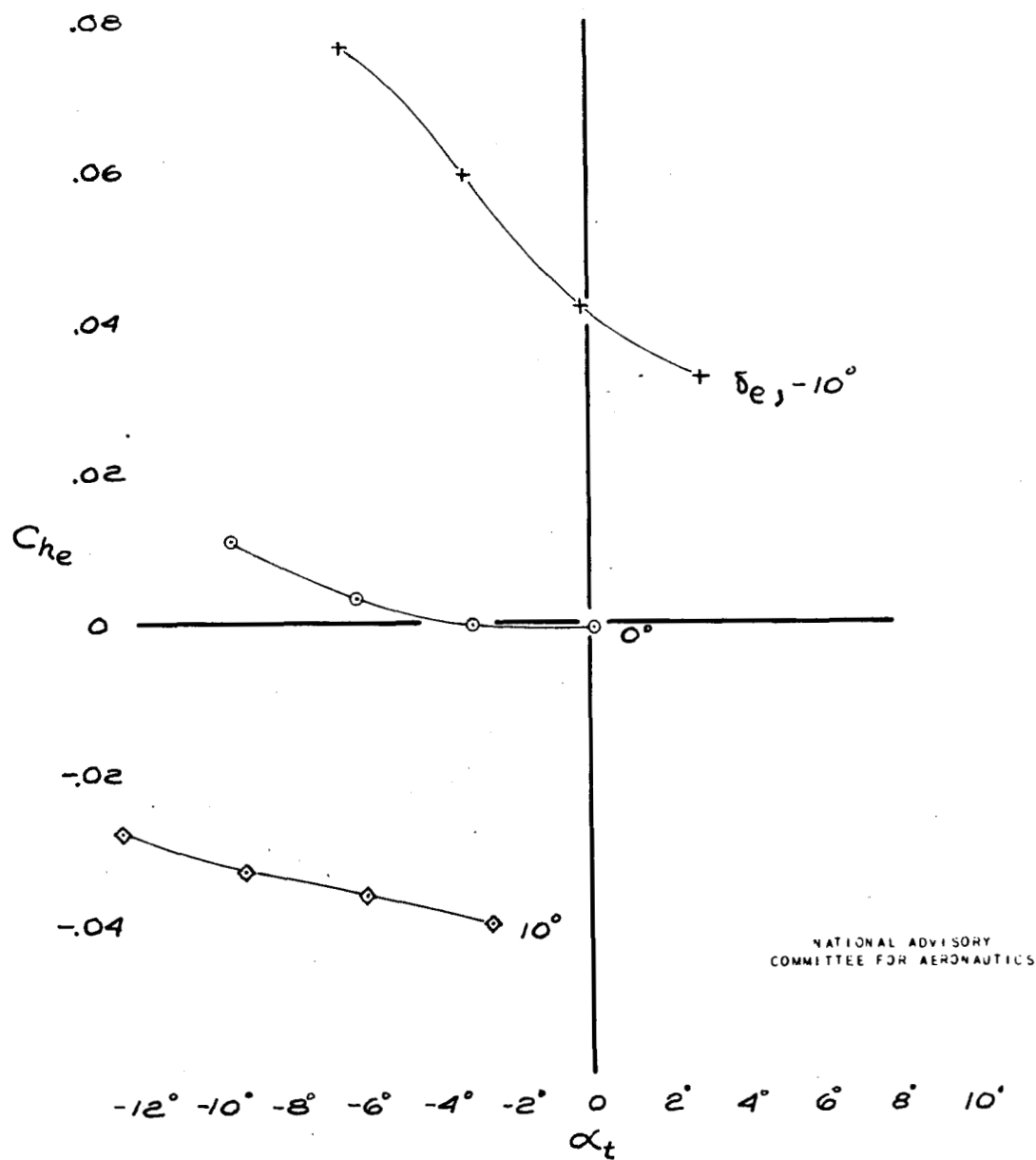
FIGURE 29.-VARIATION OF HINGE-MOMENT COEFFICIENT WITH TAIL ANGLE OF ATTACK, FABRIC-COVERED ELEVATOR WITH LEAK HOLES IN BALANCE SEAL. M, 0.33 ; \delta_t, 0^\circ .
