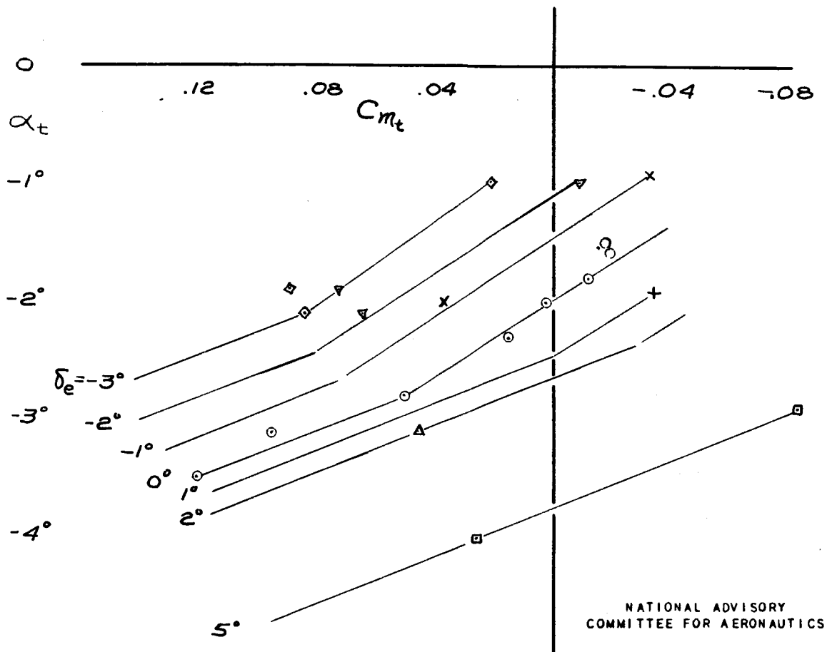
(2) FABRIC-COVERED ELEVATOR FIGURE 18 - VARIATION OF PITCHING-MOMENT COEFFICIENT DUE TO THE TAIL WITH TAIL ANGLE OF ATTACK. M, 0.72; \delta_t, 0^\circ .
