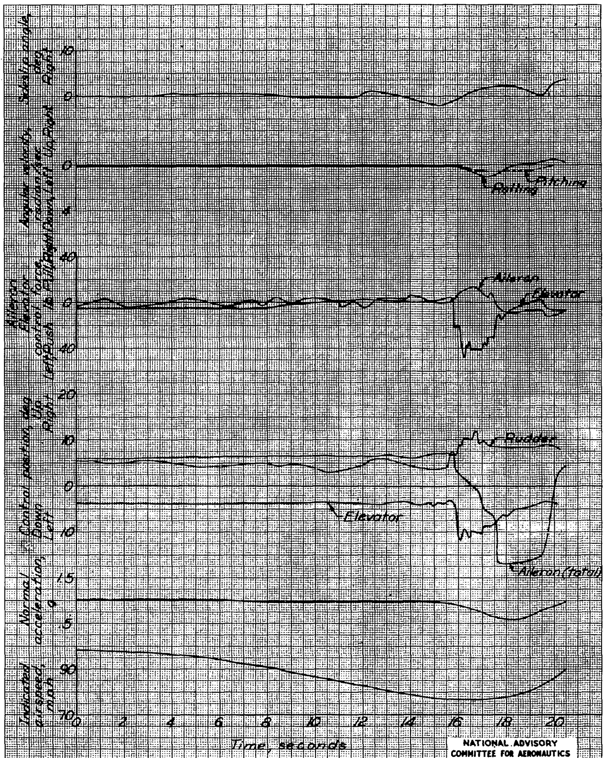
Figure 29. - Time history of a stall in the wave-off condition, center of gravity at 34.4 percent mean aerodynamic chord, DeHavilland Mosquito F-5 airplane.
