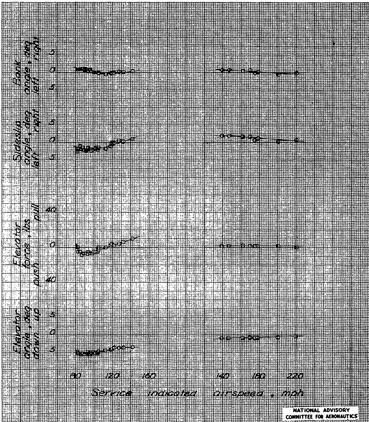
(c) Approach condition, center of gravity at 36.0 percent mean aerodynamic chord, elevator trimming tabs 7.2 degrees up.
