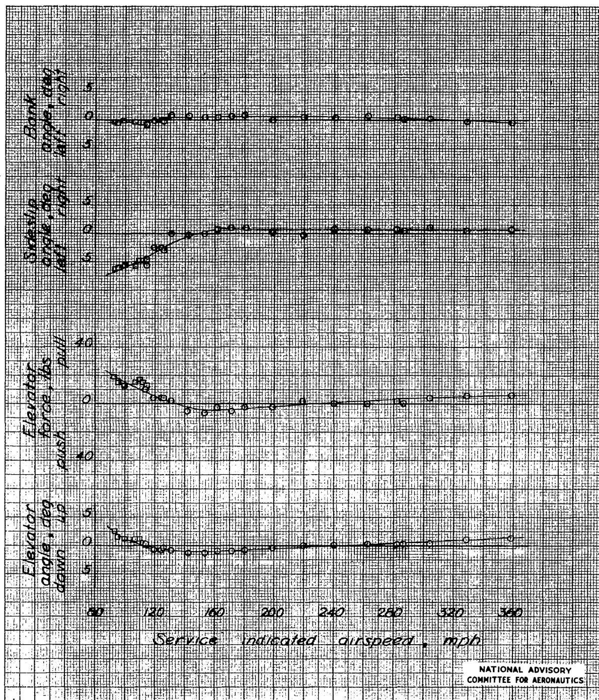
(c). Center of gravity at 38.2 percent mean aerodynamic chord, elevator trimming tabs 2.3 degrees up. Figure 6. - Concluded.
