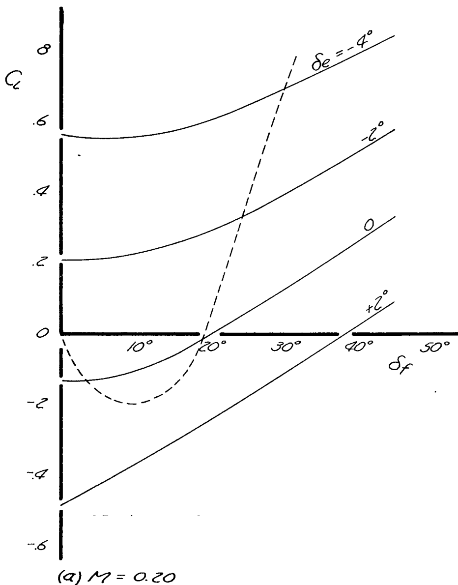
FIGURE 35.— VARIATION OF BALANCE LIFT COEFFICIENT WITH DEFLECTION OF THE 0.6-BY 12-INCH FLAPS
