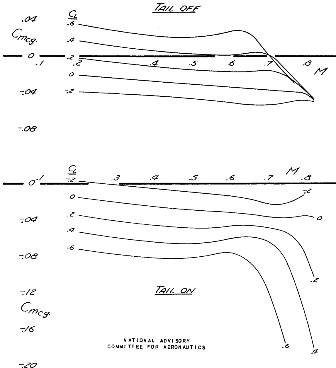
FIGURE 8. - VARIATION OF PITCHING-MOMENT COEFFICIENT WITH MACH NUMBER FOR THE STANDARD MODEL WITH ELEVATORS NEUTRAL AND FOR THE MODEL WITH THE TAIL REMOVED.
