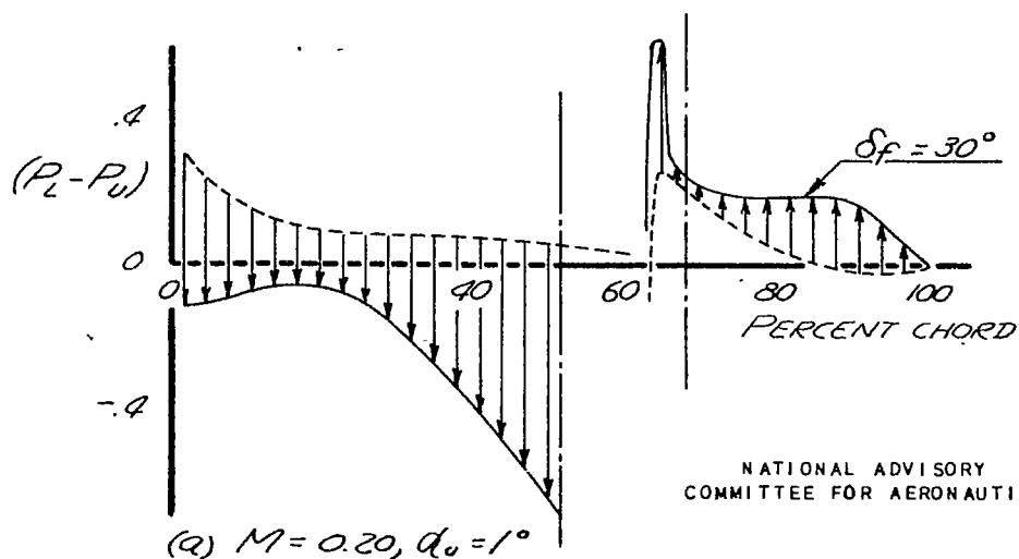
FIGURE 41.- LOAD DISTRIBUTION AT STATION 10.0 OF THE HORIZONTAL TAIL FOR SEVERAL DEFLECTIONS OF THE 1.2- BY 12-INCH FLAPS. \delta_e = 0
