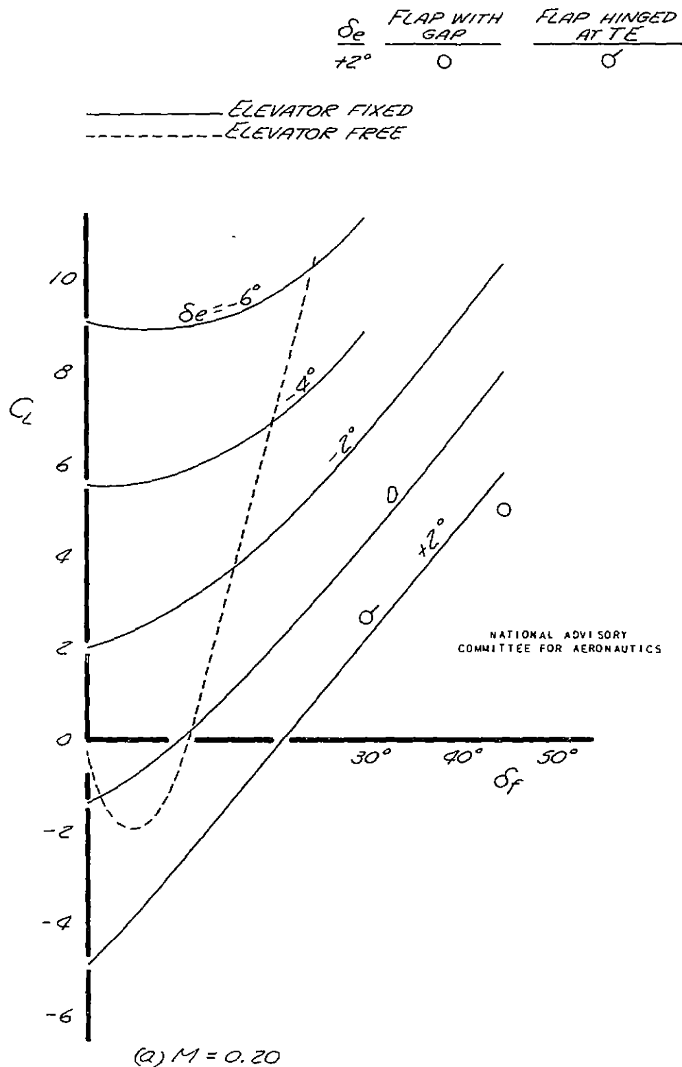
FIGURE 34 - VARIATION OF BALANCE LIFT COEFFICIENT WITH DEFLECTION OF THE 12-BY 12-INCH FLAPS
