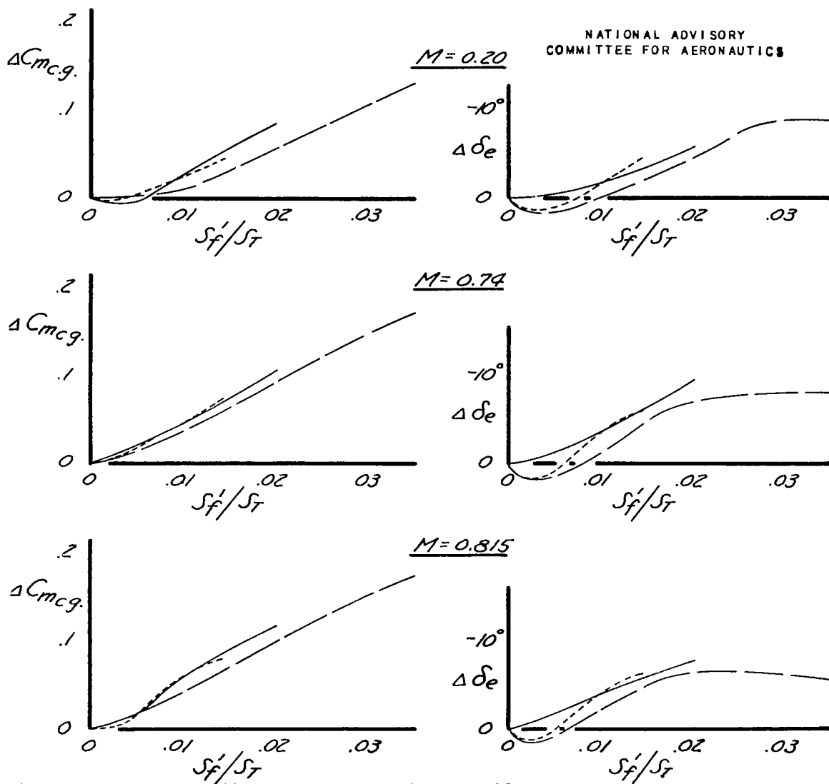
FIGURE 33.— INCREMENT OF PITCHING-MOMENT COEFFICIENT AT C_L = 0 AND \delta_e = 0 , AND OF ELEVATOR FLOATING ANGLE AT C_L = 0 , AS A FUNCTION OF THE PROJECTED AREA OF THE FLAPS NORMAL TO THE STABILIZER SURFACE.
