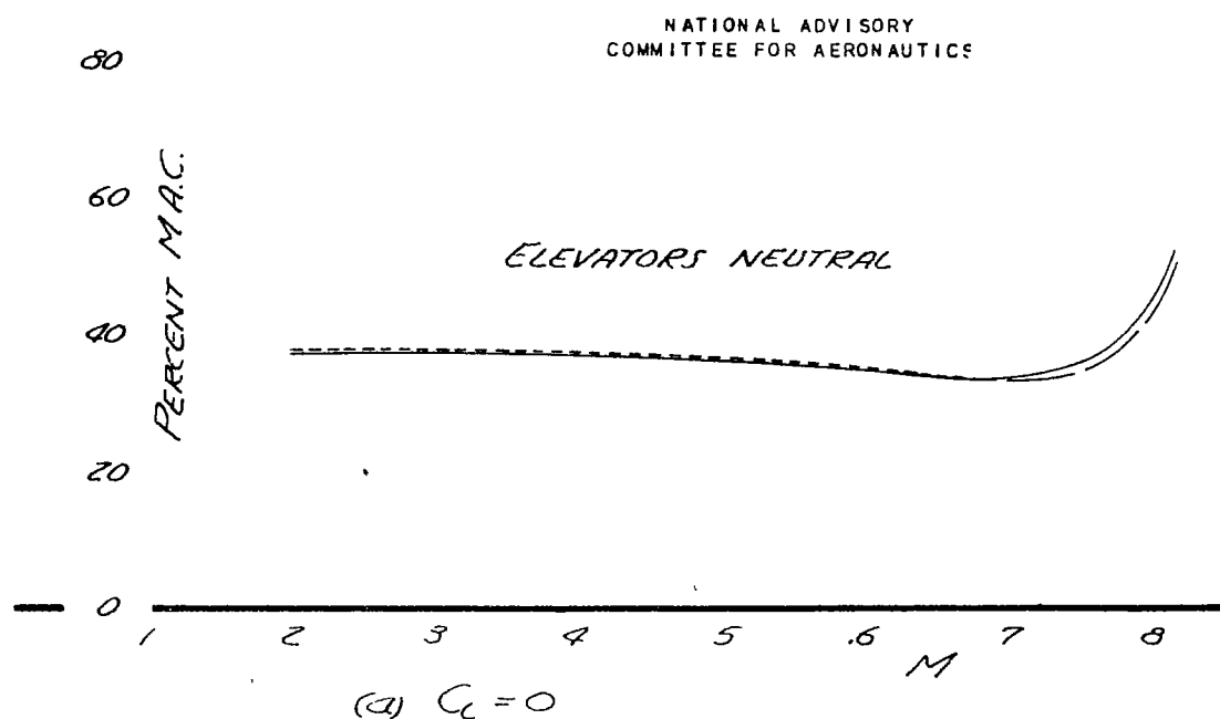
FIGURE 94.- STICK-FREE AND STICK-FIXED NEUTRAL POINT FOR SEVERAL DEFLECTIONS OF THE 1.2- BY 12-INCH FLAPS
