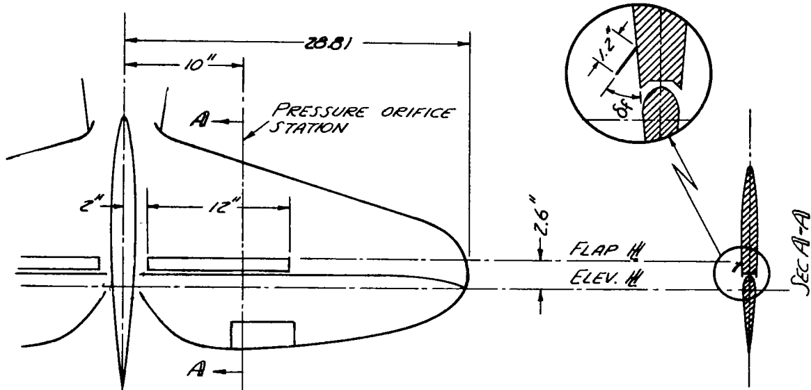
(a) 1.2-BY 12-INCH FLAP
