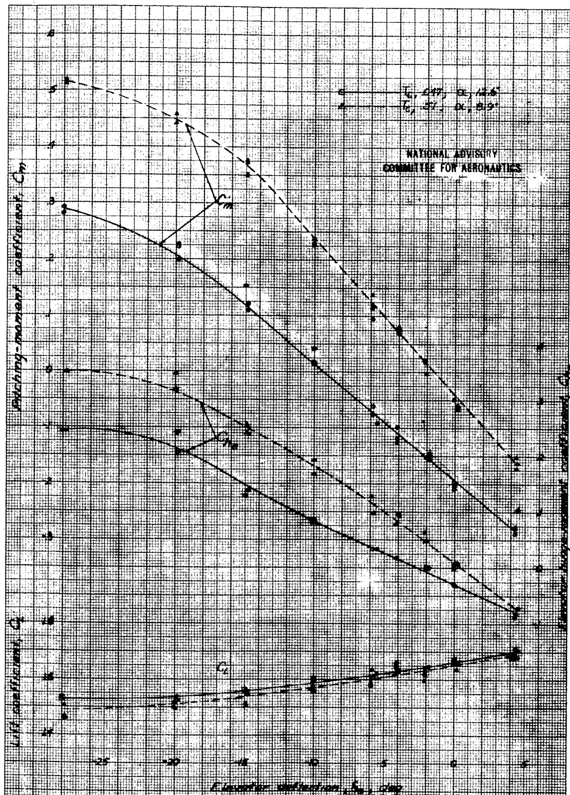
Figure 36. Effect of elevator deflection on the aerodynamic characteristics of the XP-55 model in the landing attitude ( V , 200; q , 40; \gamma , 16°; \rho , 0.0018; \mu , 0.0017; elevator tab locked).
