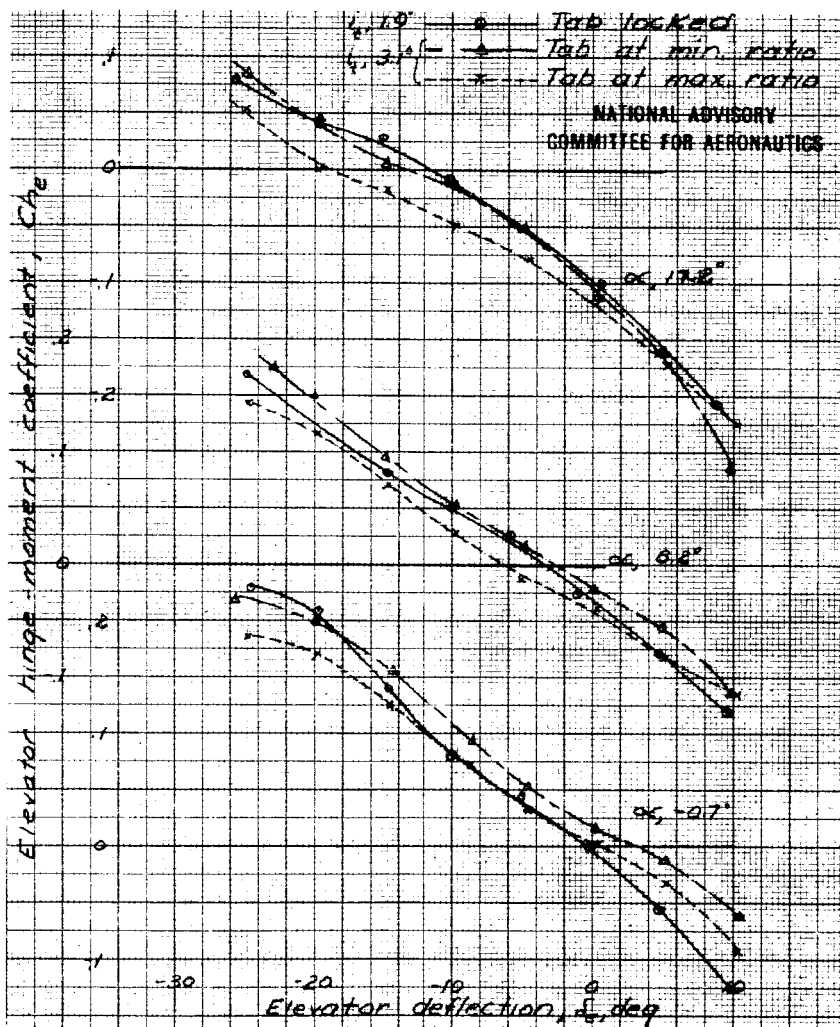
Figure 27.- Effect of tab setting on rate of change of C_{H_e} with \delta_e . Propellers removed, \delta_f, 0^\circ .
