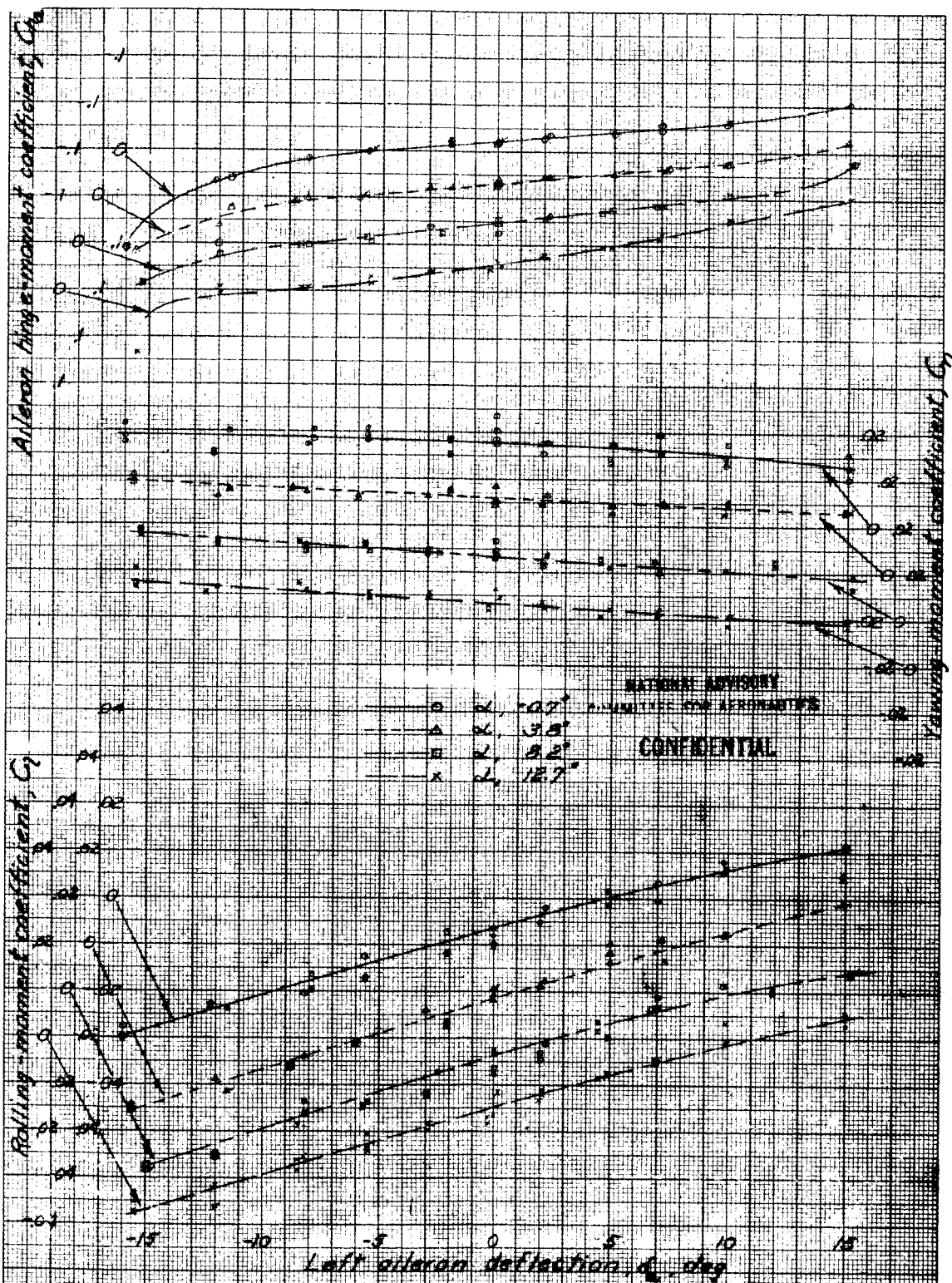
Figure 67. - Effect of aileron deflection on the aerodynamic characteristics of the XP-69 model. Propellers removed, right aileron locked, left aileron tab locked. \eta , 10.1; \delta_r , 0^\circ ; \delta_l , 15^\circ .
