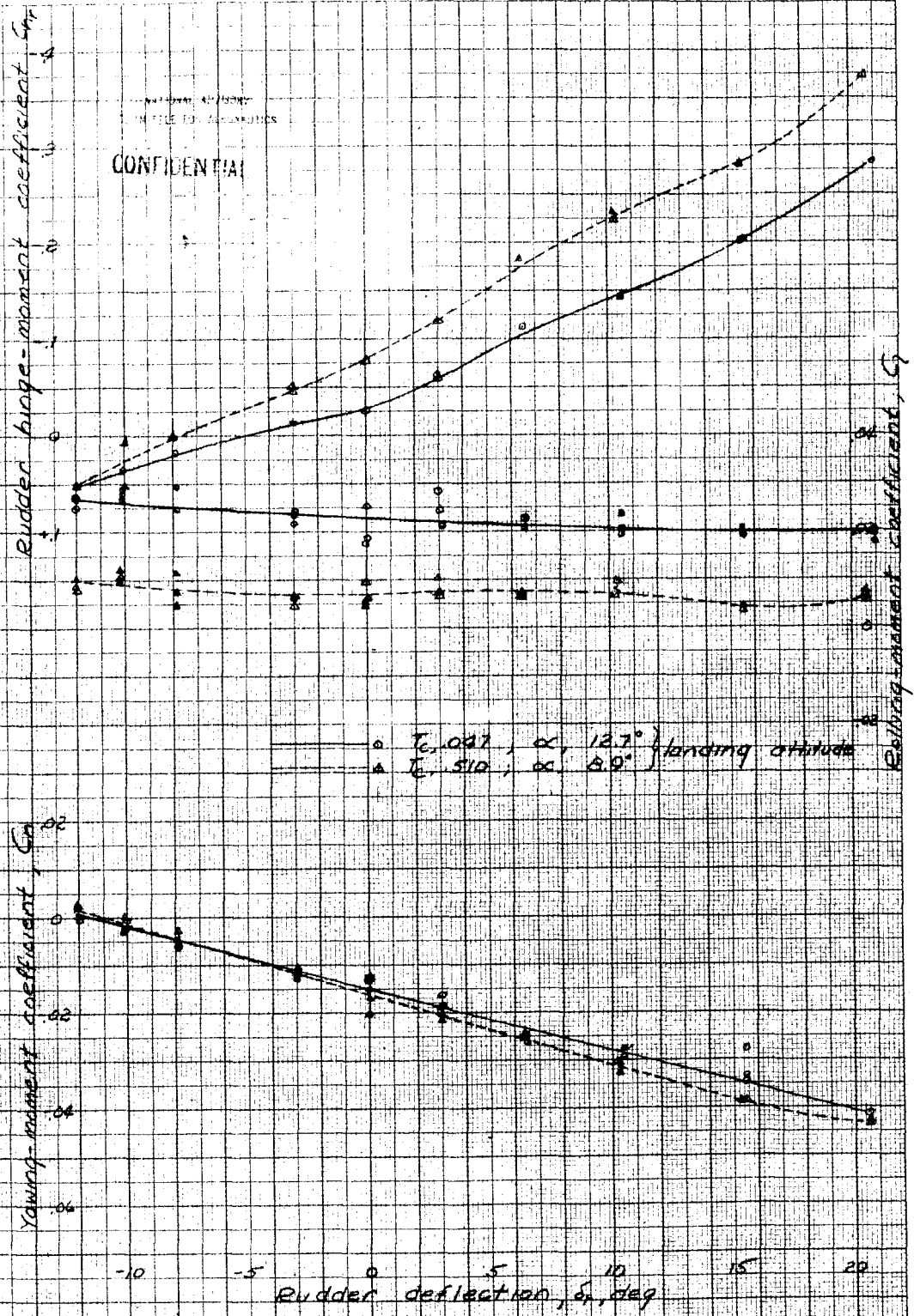
(a) C_n , C_l , C_{hr} Figure 55.-Effect of rudder deflection on the aerodynamic characteristics of the XP-69 model in yaw. V_0 , 15.1^\circ ; \delta_r , 40^\circ ; \delta_r , 16^\circ ; \delta_r , 0^\circ ; \delta_r , 20^\circ ; \delta_r , 27^\circ ; rudder tab at ratio 1.
