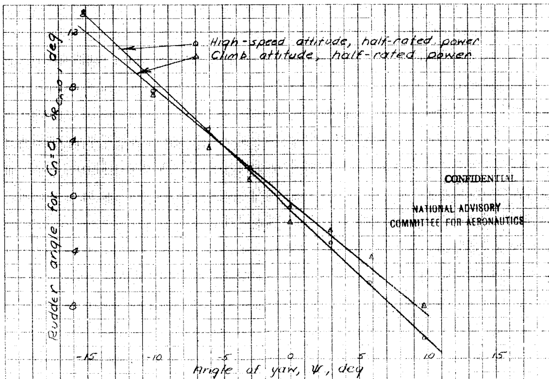
Figure 63.- Variation of rudder angle at C_n=0 with angle of yaw. \beta_1, 20^\circ ; \beta_2, 27.7^\circ ; \delta, 0 ; rudder tab at ratio 1.
