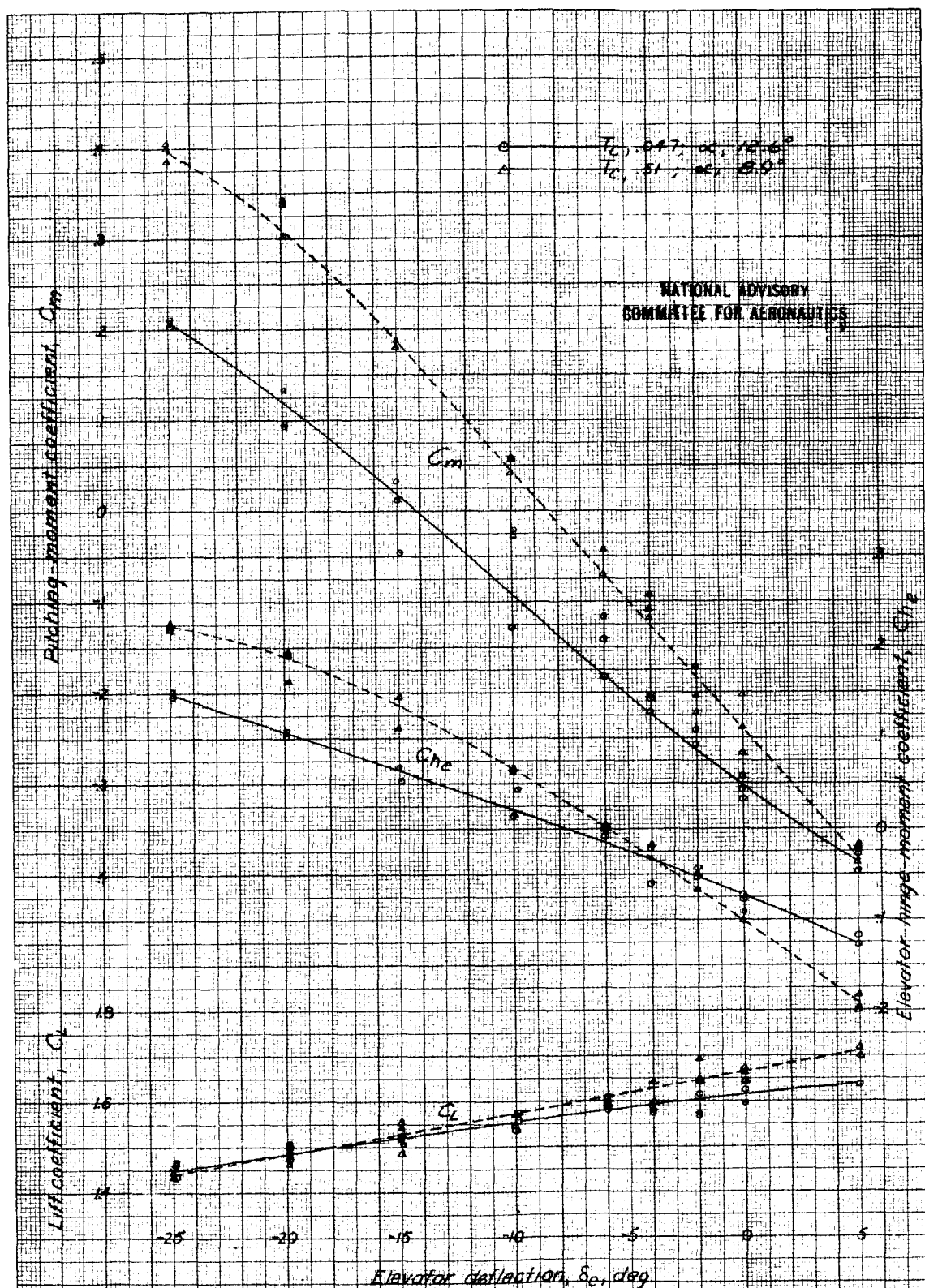
Figure 37- Effect of elevator deflection on the aerodynamic characteristics of the XP-69 model in the landing attitude. V_e, 151 ; \delta, 40 ; V_L, 1.6 ; \beta, 28^\circ ; R_e, 2.77 ; elevator tab locked.
