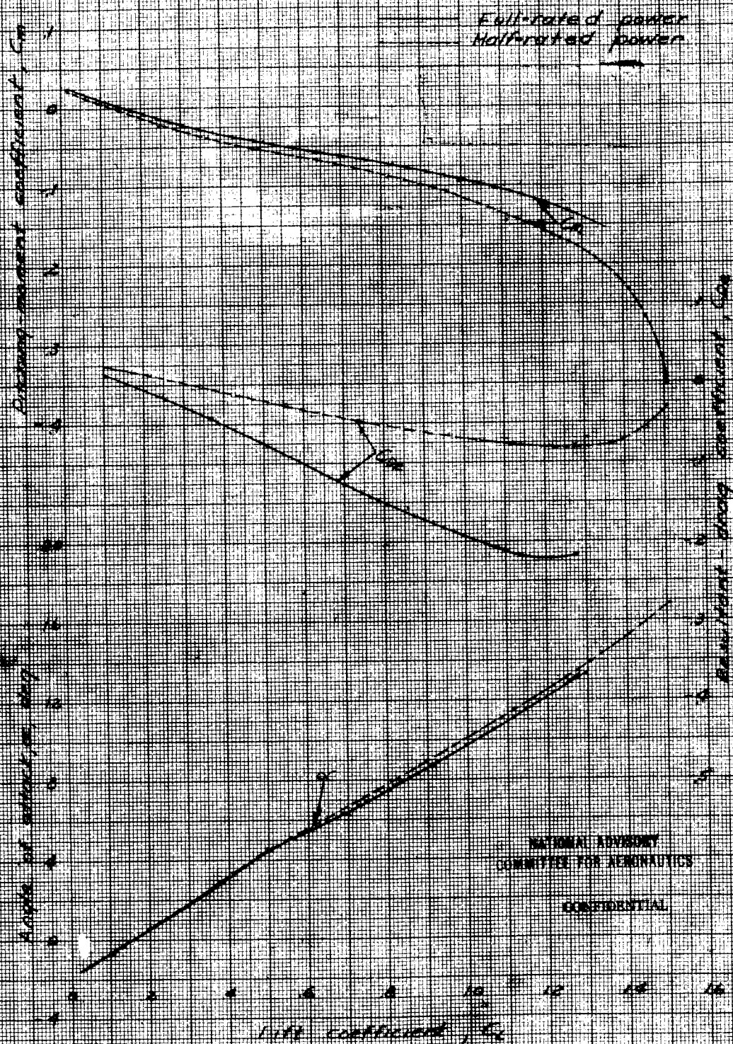
Figure 17. - Effect of propeller operation on the aerodynamic characteristics of the XP-59 model. \alpha , 0°; \alpha , 16°; \alpha , 0°; \alpha , 28°; \alpha , 27°.
