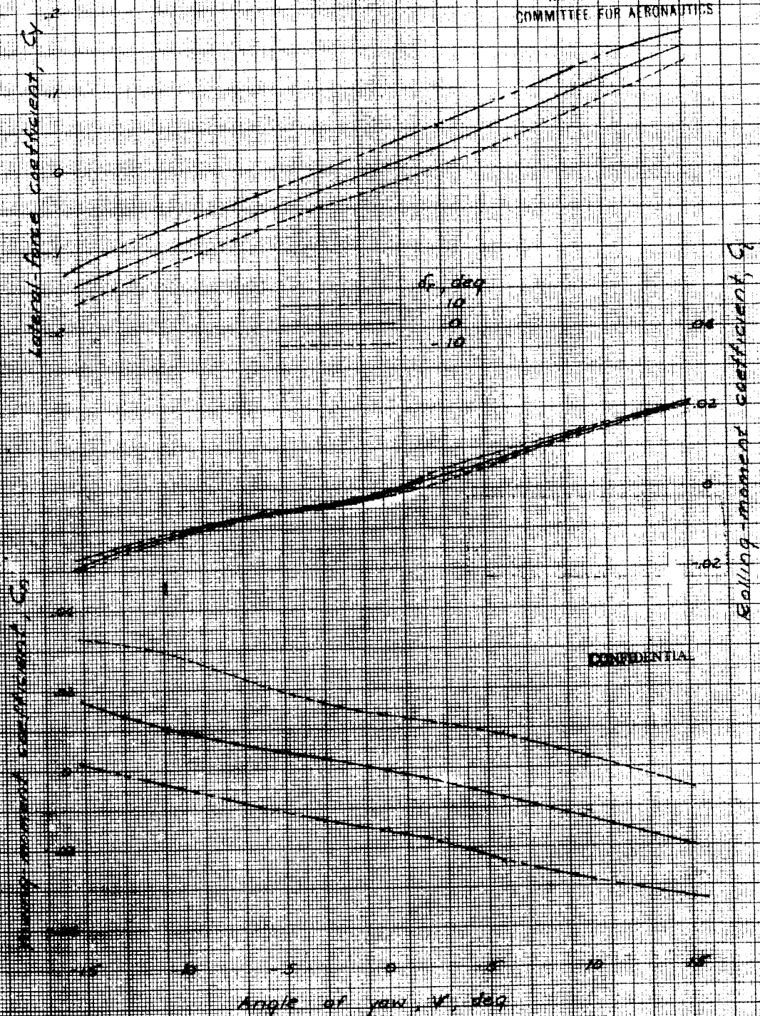
Figure 14- Variation of C_n , C_p , and C_y with angle of yaw. Model in climbing attitude, full-rated power. \delta_c , 10°, 0°, -10°; \delta_r , 27°, 0°, -27°; \delta_s , 0°, 5°, 10°; rudder tab at 10°.
