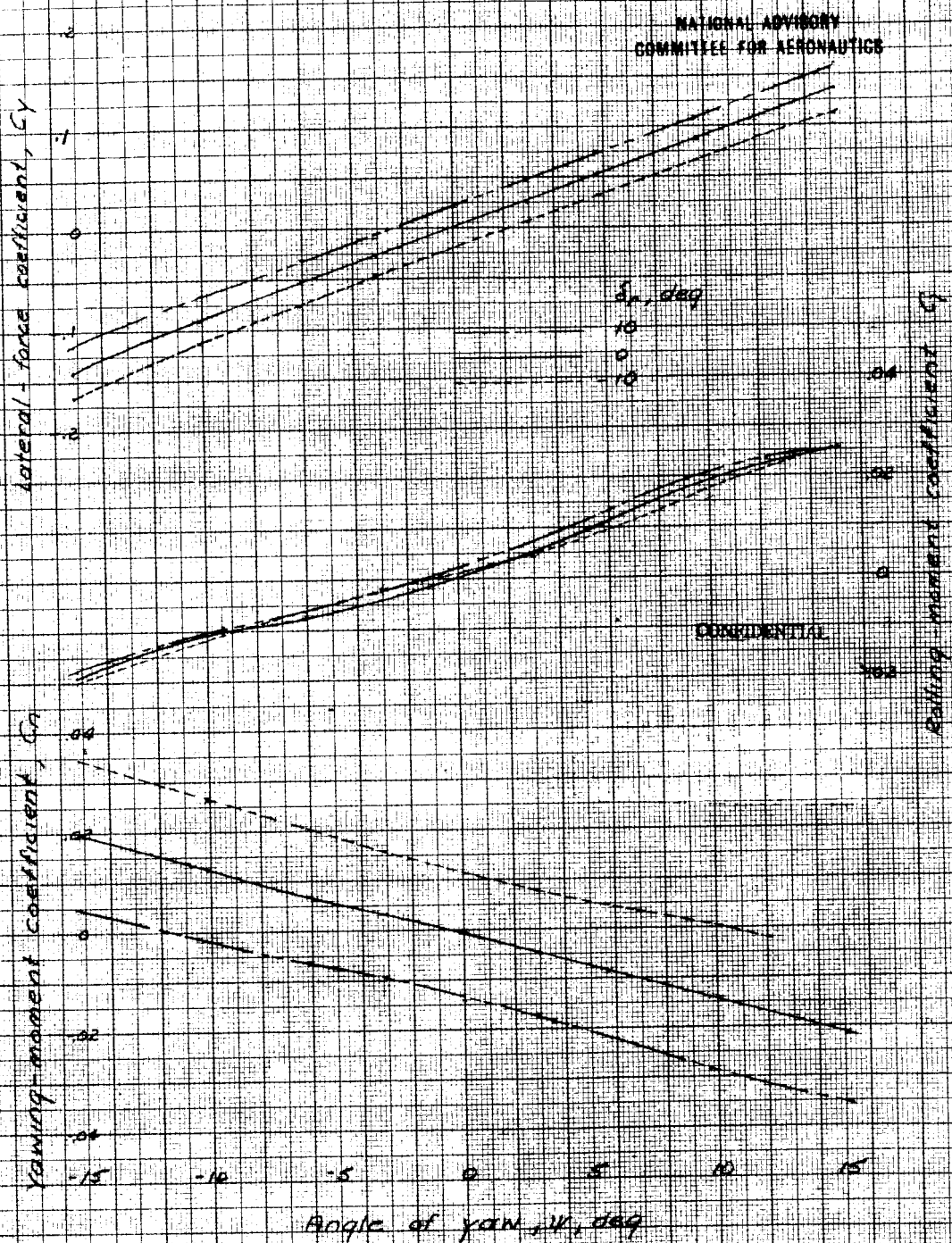
Figure 42. - Variation of C_n , C_r , and C_y with angle of yaw. Model in high-speed attitude, full-rated power, T_0, 0.25 ; \beta_r, 23^\circ ; \beta_0, 22.7^\circ ; \delta, 0^\circ ; \alpha, +0.2^\circ ; rudder tab at ratio 1.
