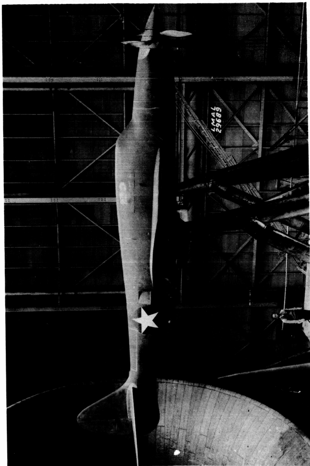
Figure 2.- The 3/4-scale model of the XP-69 airplane mounted in the NACA full-scale tunnel.
