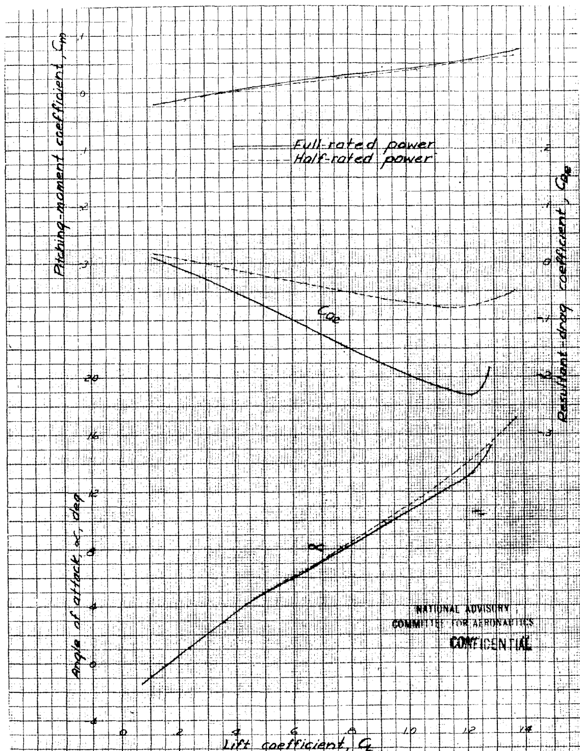
Figure 12.- Effect of propeller operation on the aerodynamic characteristics of the XP-69 model with horizontal and vertical tail surfaces removed \beta_1, 0^\circ ; \beta_2, 20^\circ ; \beta_3, 27^\circ .
