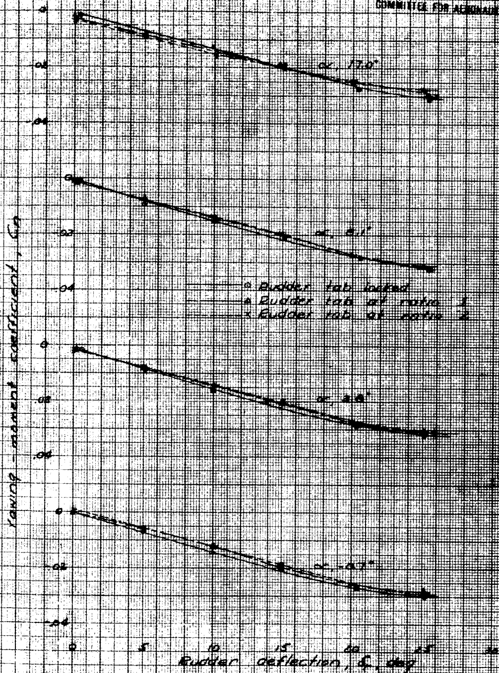
Figure 51 - Effect of tab setting on rate of change of C_n with \delta . Propellers removed, \delta, 0^\circ ; \gamma, 0^\circ .
