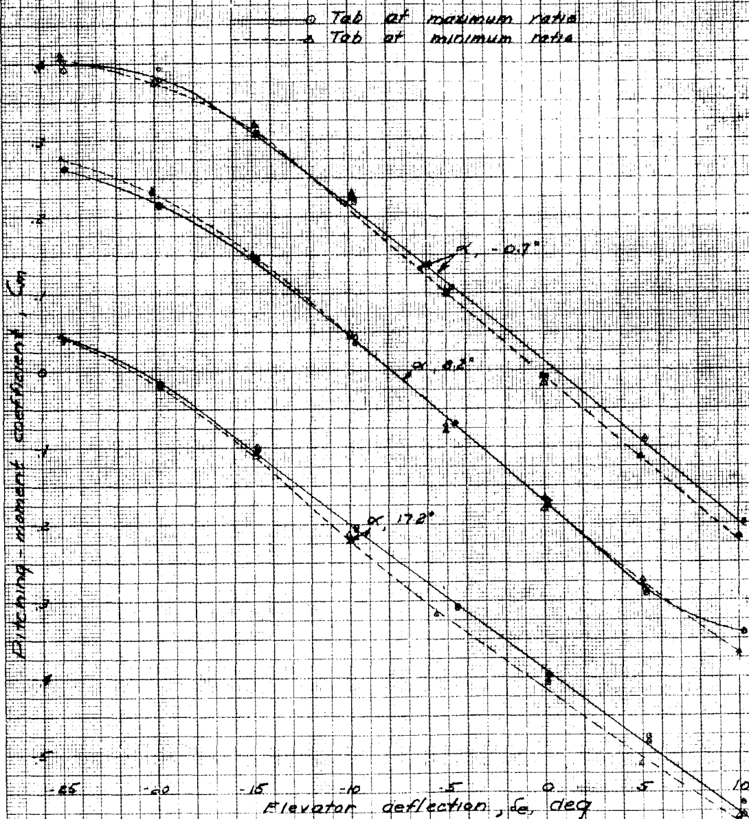
Figure 20.- Effect of tab setting on rate of change of C_m with \delta_e of 6°, 1/2, 31°. Propellers removed.
