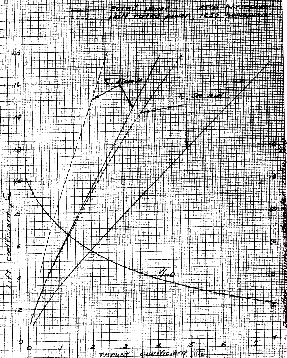
Figure 6 - Variation of T_c with C_l and V/na for constant power operation at sea level and at 35,000 feet altitude. \beta_F, 28^\circ ; \beta_R, 27.7^\circ
