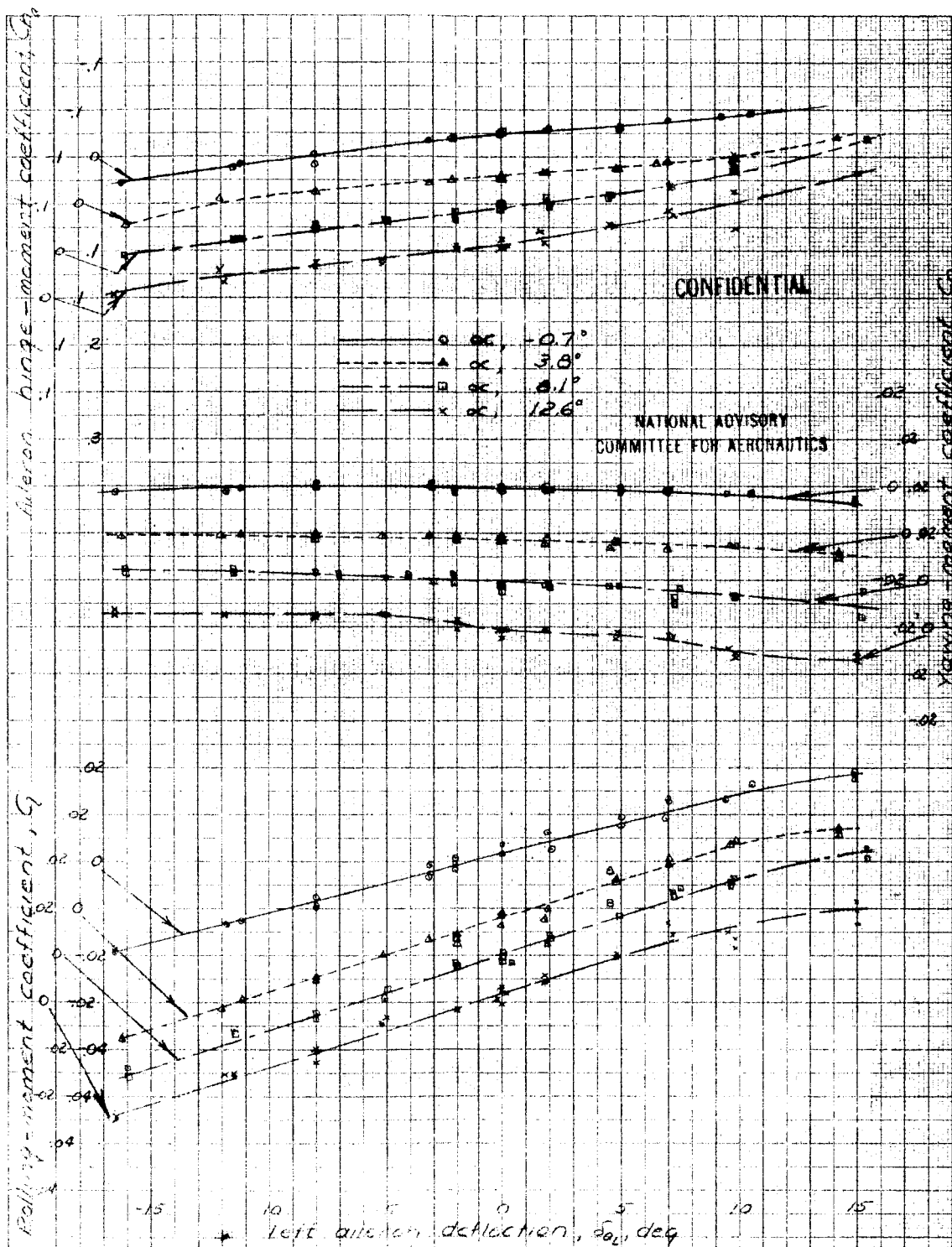
Figure 65. Effect of aileron deflection on the aerodynamic characteristics of the XP-69 model. Propellers removed, right aileron locked, left aileron tab locked, V_\infty , 87.0^\circ ; 4, 16^\circ
