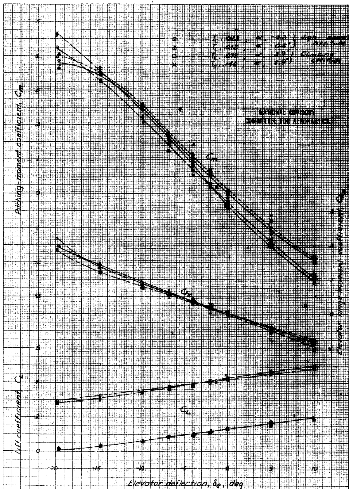
Figure 34.- Effect of elevator deflection on the aerodynamic characteristics of the XP-69 model in the high-speed and climbing attitudes. V_e 5.75; \delta_e 0°; V_e 16°; \alpha 20°; \alpha 27°; elevator tab locked.
