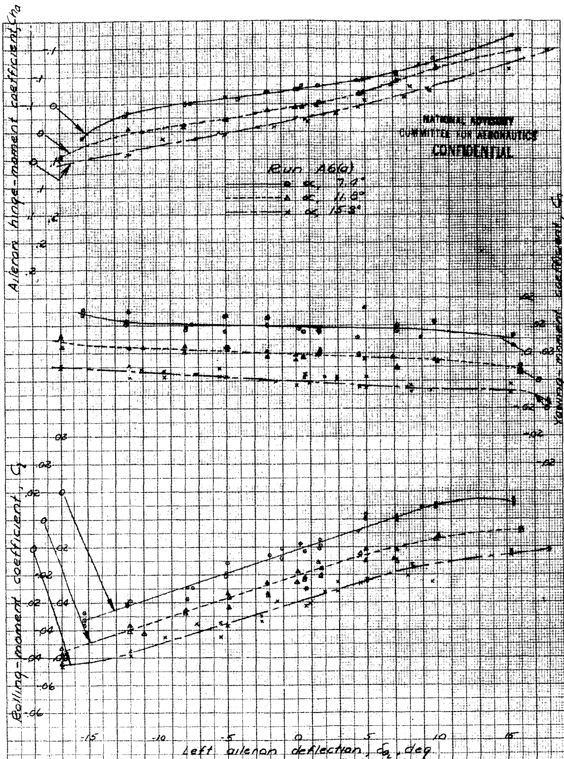
Figure 72.- Effect of aileron deflection on the aerodynamic characteristics of the XP-69 model. Propellers removed; wing tanks on; right aileron locked; left aileron tab locked. M_\infty = 10.7 ; \delta_r = 40^\circ ; \eta = 1.6^\circ
