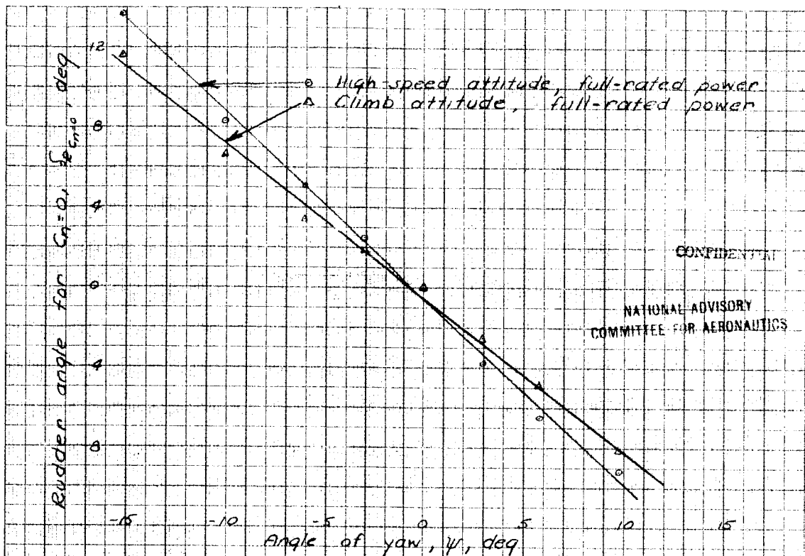
Figure 62.- Variation of rudder angle at C_n=0 with angle of yaw. \beta_1, 20^\circ ; \beta_2, 27.7^\circ ; \delta, 0 ; rudder tab at ratio 2.
