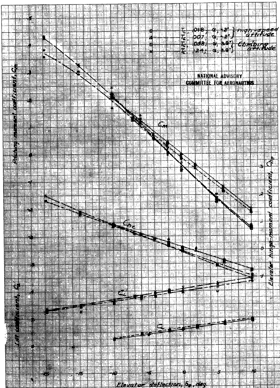
Figure 35.- Effect of elevator deflection on the aerodynamic characteristics of the XP-60 model in the high-speed and climbing attitudes \alpha, 1.5^\circ; \delta_e, 0^\circ; \alpha, 1.0^\circ; \alpha, 2.0^\circ; \alpha, 2.2^\circ ; elevator tab locked.
