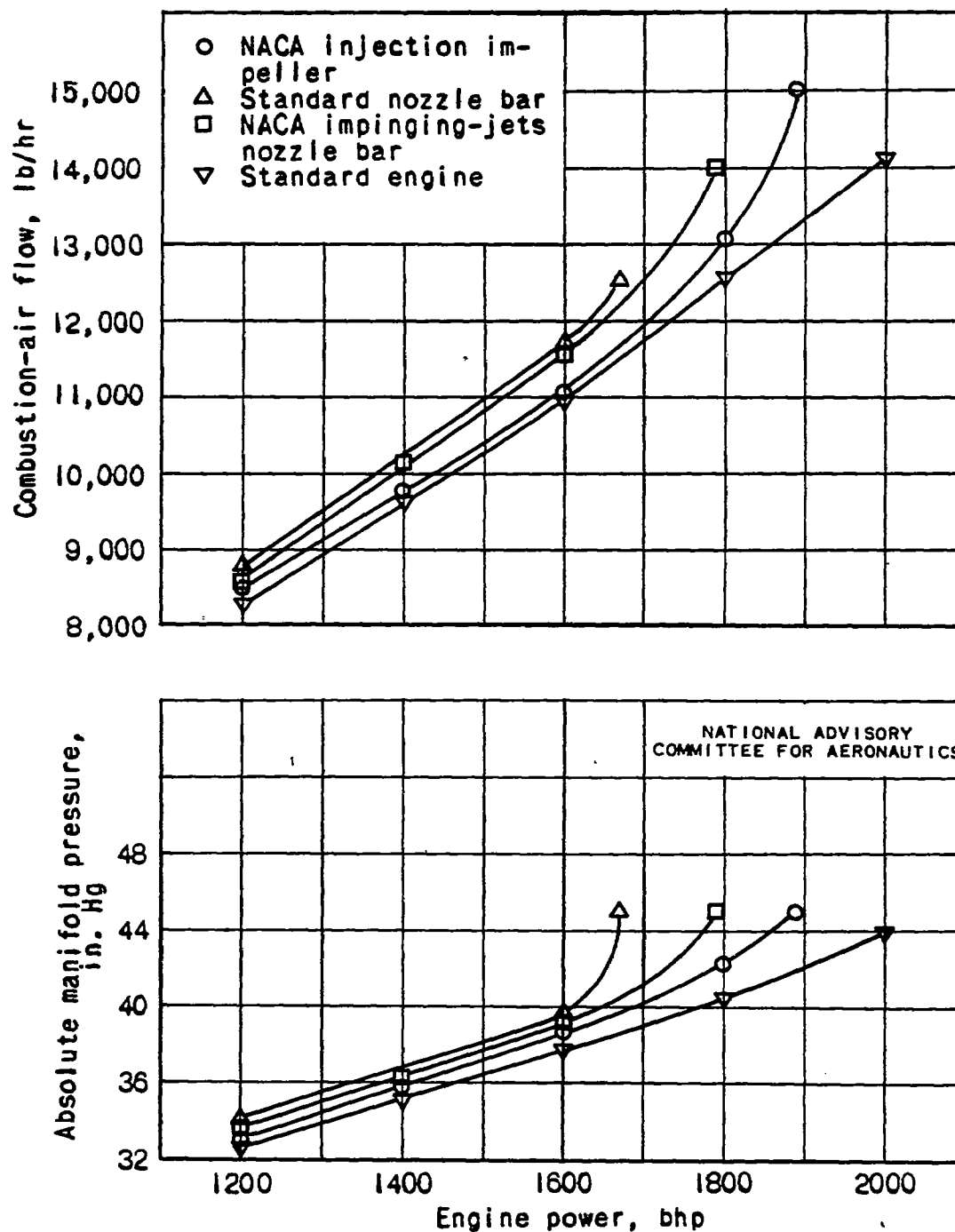
Figure 11. - Engine air flow and manifold pressure required at standard powers for standard nozzle-bar injection of gasoline and for safety-fuel injection by NACA injection impeller, NACA impinging-jets nozzle bar, and standard nozzle bar.
