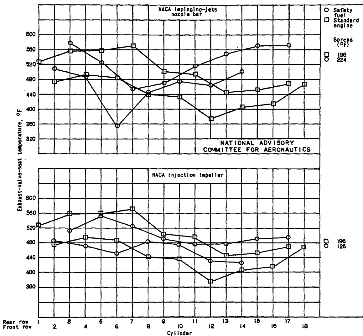
Figure 8. - Continued. Exhaust-valve-seat temperature distribution obtained at standard powers for standard nozzle-bar injection of gasoline and for safety-fuel injection by NACA injection impeller, NACA impinging-jets nozzle bar, and standard nozzle bar. Combustion-air temperature, 100° F.
