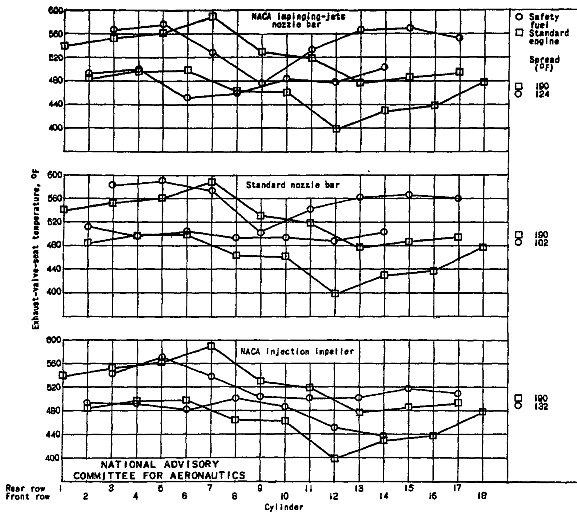
Figure 8. - Exhaust-valve-seat temperature distribution obtained at standard powers for standard nozzle-bar injection of gasoline and for safety-fuel injection by NACA injection impeller, NACA impinging-jets nozzle bar, and standard nozzle bar. Combustion-air temperature, 1000° F.
