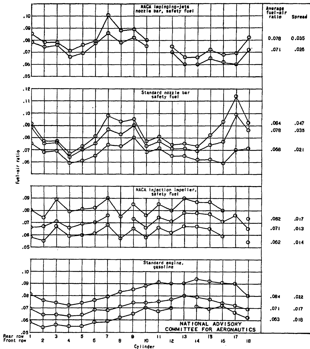
Figure 9. - Mixture distribution obtained at several average fuel-air ratios for standard nozzle-bar injection of gasoline and for safety-fuel injection by NACA injection impeller, NACA impinging-jets nozzle bar, and standard nozzle bar. Brake horsepower, 1200; combustion-air temperature, 100° F.
