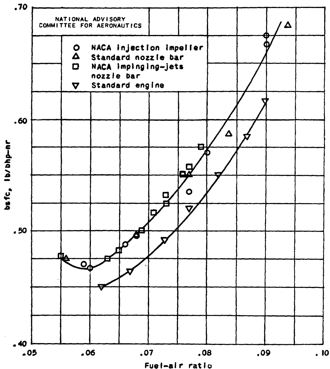
Figure 12. - Brake specific fuel consumption at 1200 brake horsepower for standard nozzle-bar injection of gasoline and for safety-fuel injection by NACA injection impeller, NACA impinging-jets nozzle bar, and standard nozzle bar.
