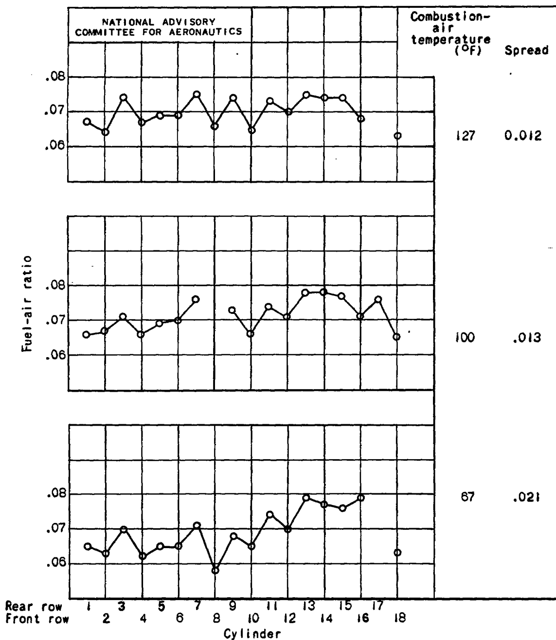
Figure 10. - Continued. Mixture distribution obtained at several combustion-air temperatures for standard nozzle-bar injection of gasoline and for safety-fuel injection by NACA injection impeller, NACA impinging-jets nozzle bar, and standard nozzle bar. Brake horsepower, 1200; approximate average fuel-air ratio, 0.069.
