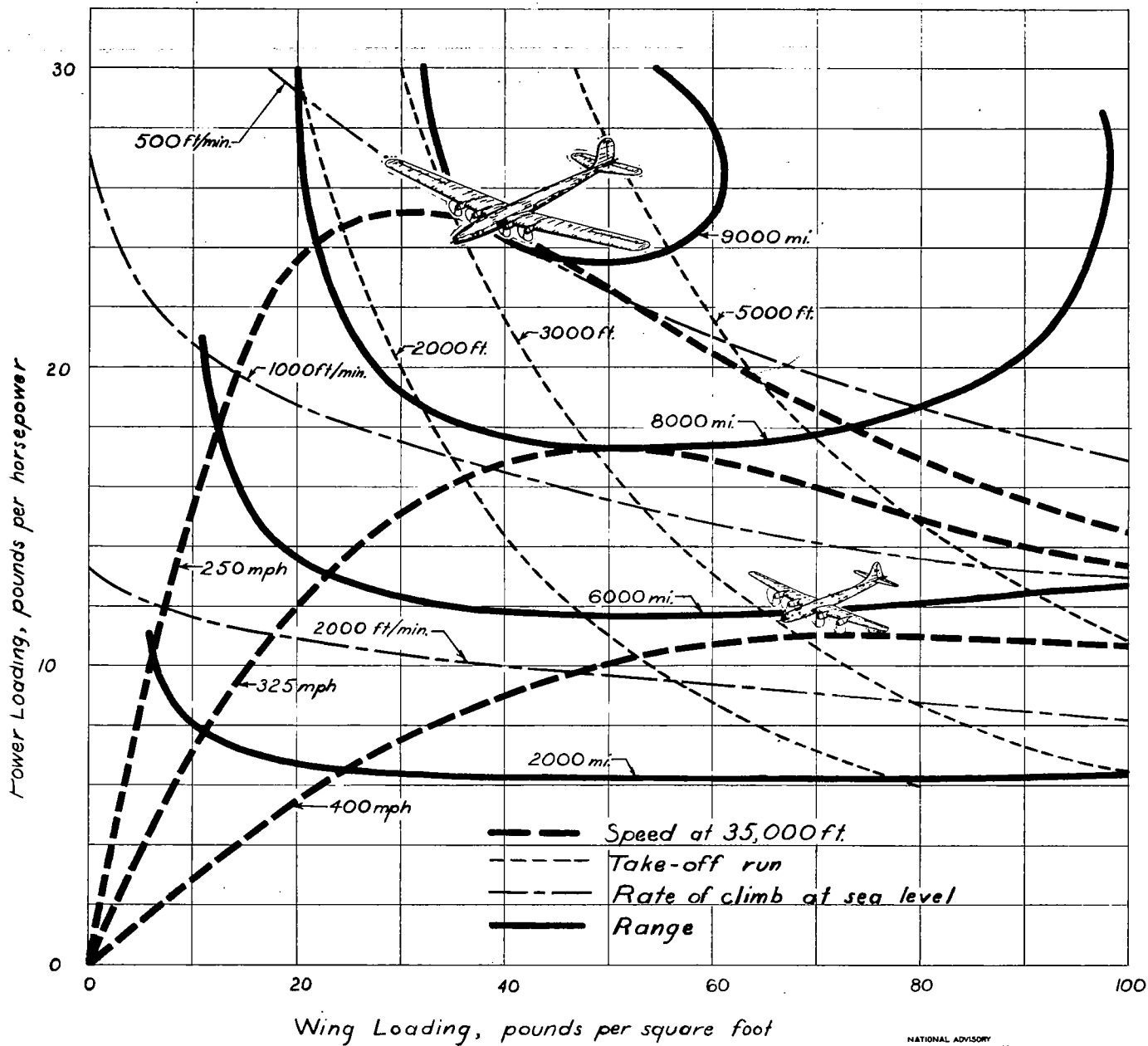
FIG-1 EFFECT OF POWER LOADING AND WING LOADING ON RANGE, SPEED, RATE OF CLIMB AND TAKE OFF
