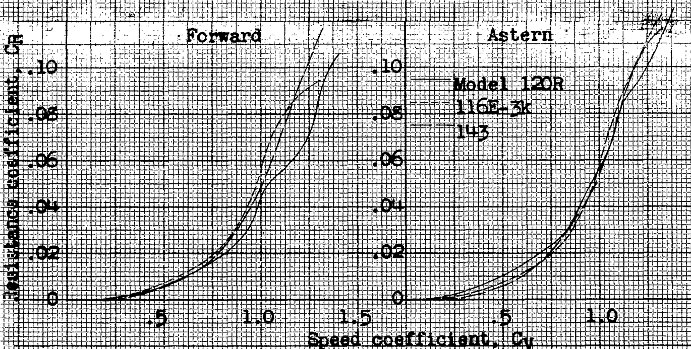
Figure 10.- Comparison of resistance coefficient at low speeds for three models. C_A = 0.8 . Free-to-trim.
