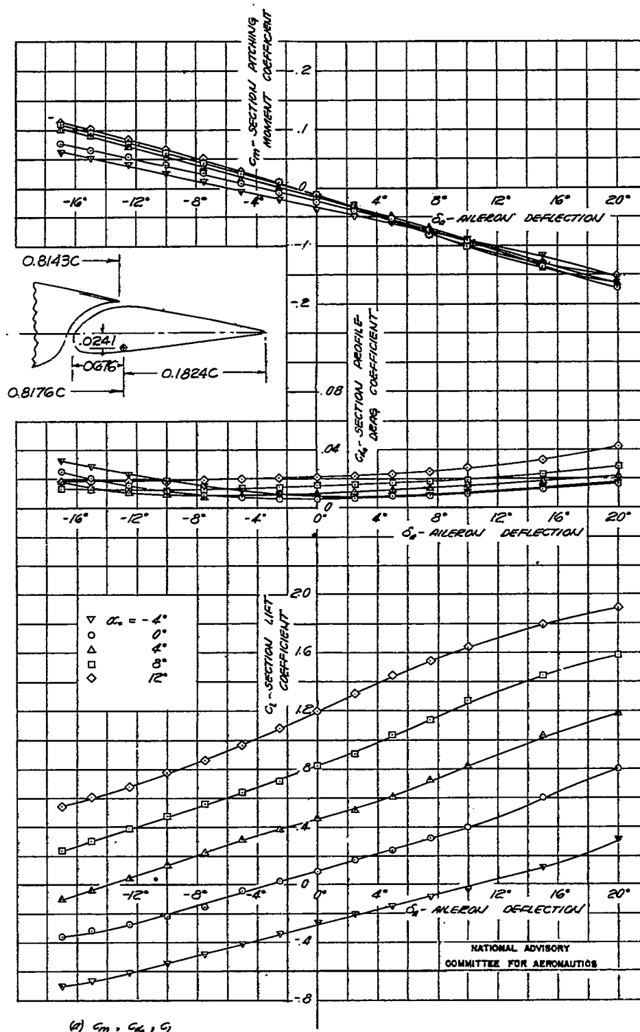
FIGURE 13.- SECTION AERODYNAMIC CHARACTERISTICS OF THE NACA 66(215)-216 ( R=0.6 ) AIRFOIL EQUIPPED WITH THE 0.25 CHORD STRAIGHT SIDED AILERON WITH A 37.05 PERCENT AERODYNAMIC BALANCE; HINGE LOCATION S.
