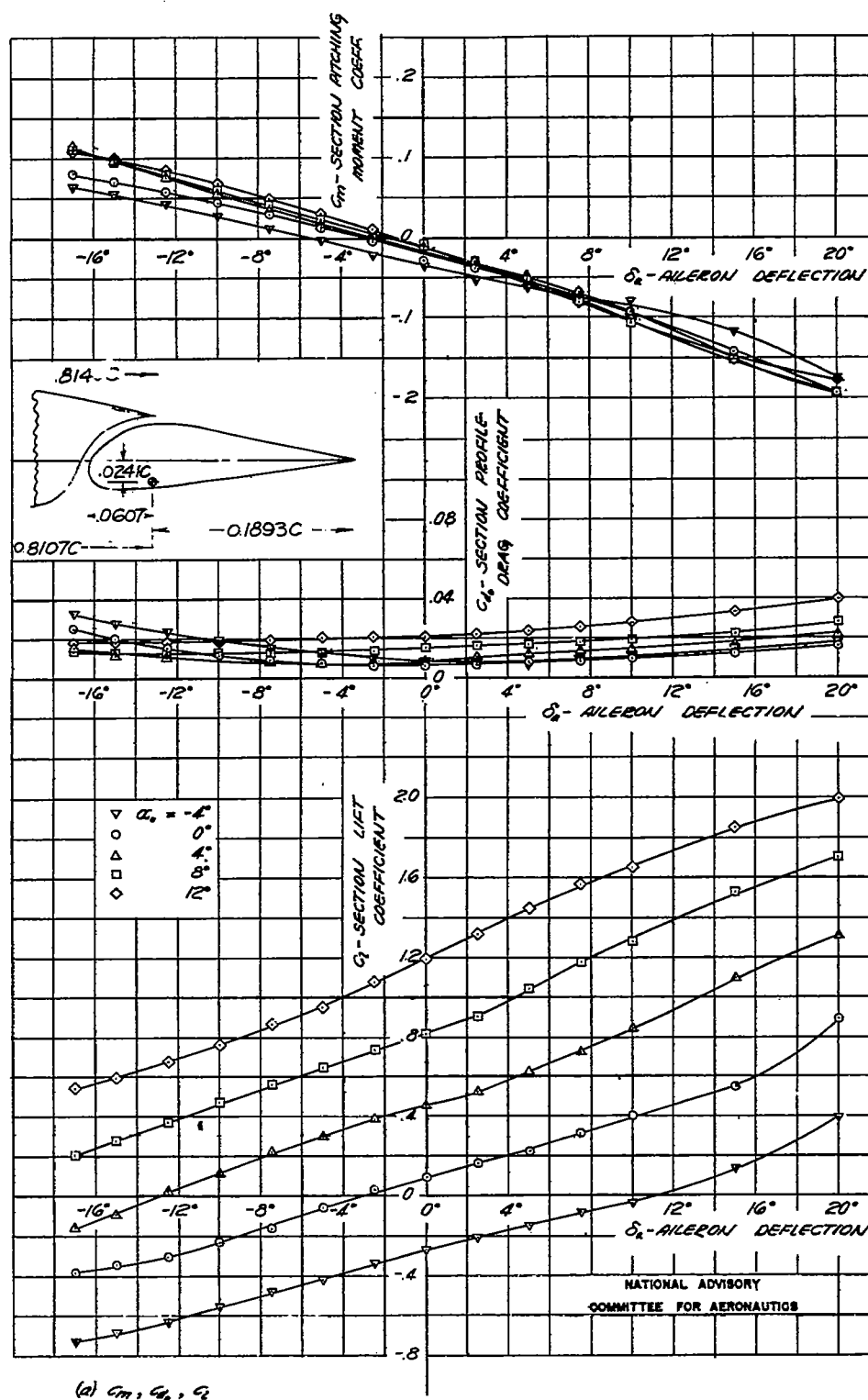
FIGURE 14.-SECTION AERODYNAMIC CHARACTERISTICS OF THE NACA 66(215)-216 ( \alpha=0.6 ) AIRFOIL EQUIPPED WITH THE 0.25 CHORD STRAIGHT SIDED AILERON WITH A 32.05 PERCENT AERODYNAMIC BALANCE; HINGE LOCATION T.
