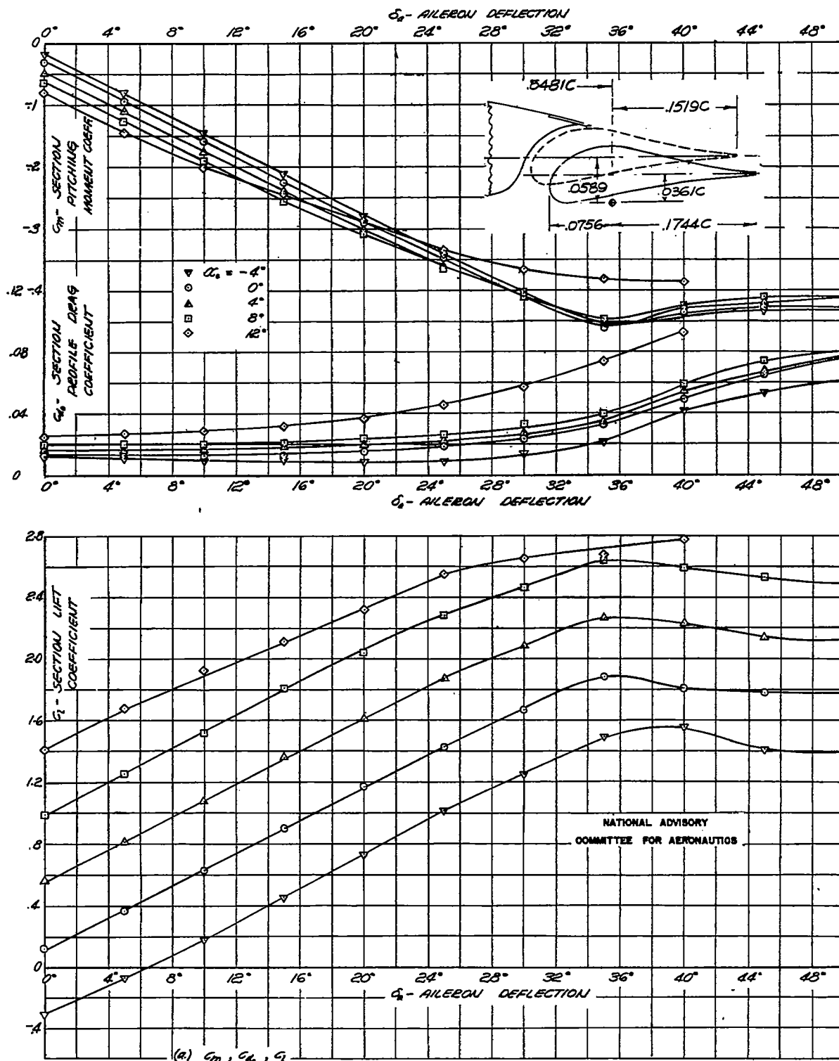
FIGURE 9 - SECTION AERODYNAMIC CHARACTERISTICS OF THE NACA 66(215)-216 ( q=6 ) AIRFOIL EQUIPPED WITH THE 0.25-CHORD NORMAL PROFILE AILERON WITH 44.33 PERCENT AERODYNAMIC BALANCE; HINGE LOCATION C.
