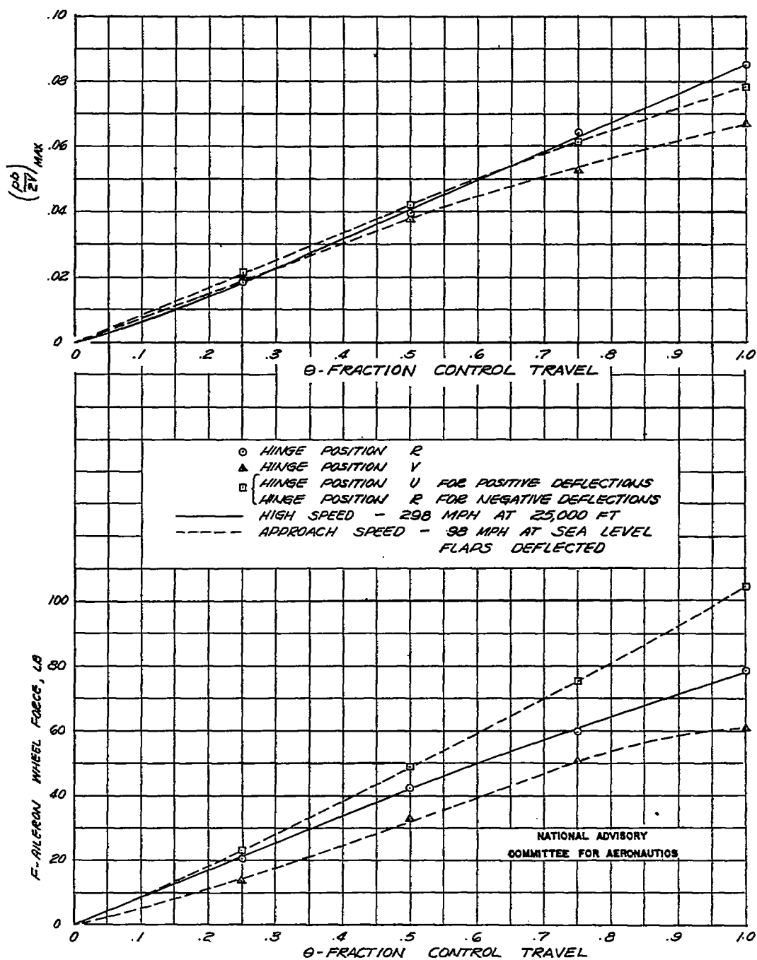
FIGURE 22.- VARIATION OF (\frac{pb}{2V})_{\max} AND WHEEL FORCE WITH CONTROL TRAVEL IN ROLLS WITH THE RUDDER LOCKED FOR THE EXEMPLARY AIRPLANES EQUIPPED WITH THE 0.25 CHORD STRAIGHT SIDED AILERON.
