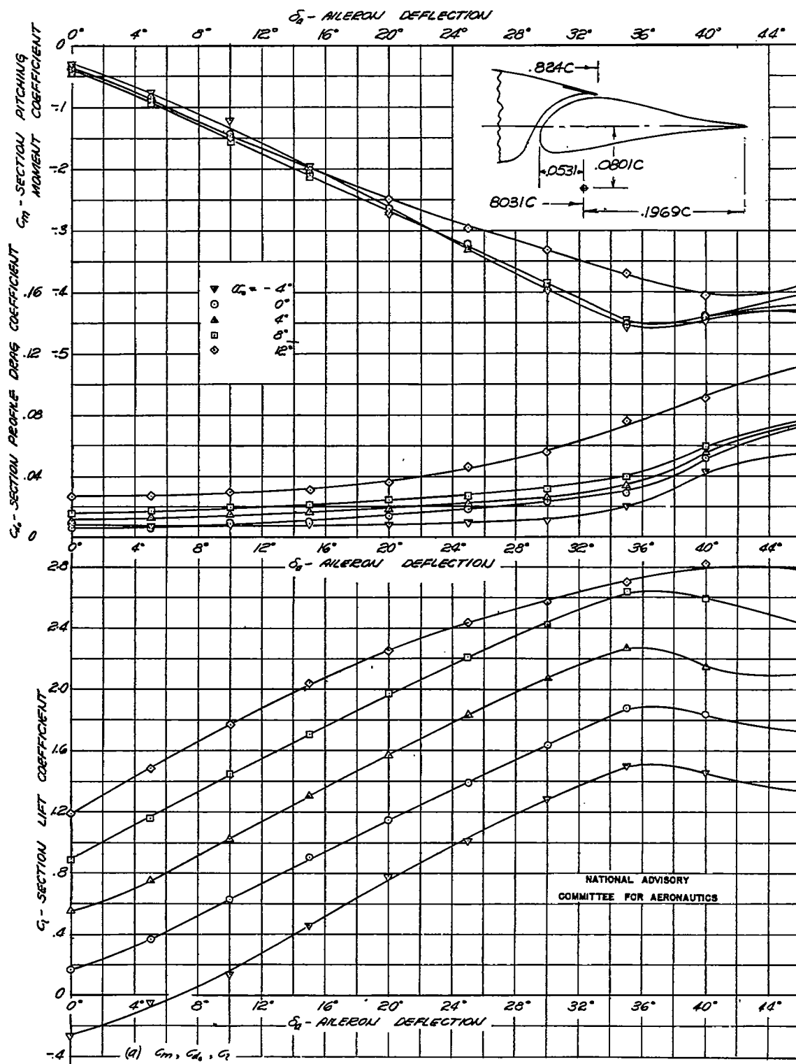
FIGURE 8 - SECTION AERODYNAMIC CHARACTERISTICS OF THE NACA 66(215)-216 ( \alpha=0^\circ ) AIRFOIL EQUIPPED WITH THE 0.25-CHORD NORMAL PROFILEAILERON WITH A 26.98 PERCENT AERODYNAMIC BALANCE; HINGE LOCATION B.
