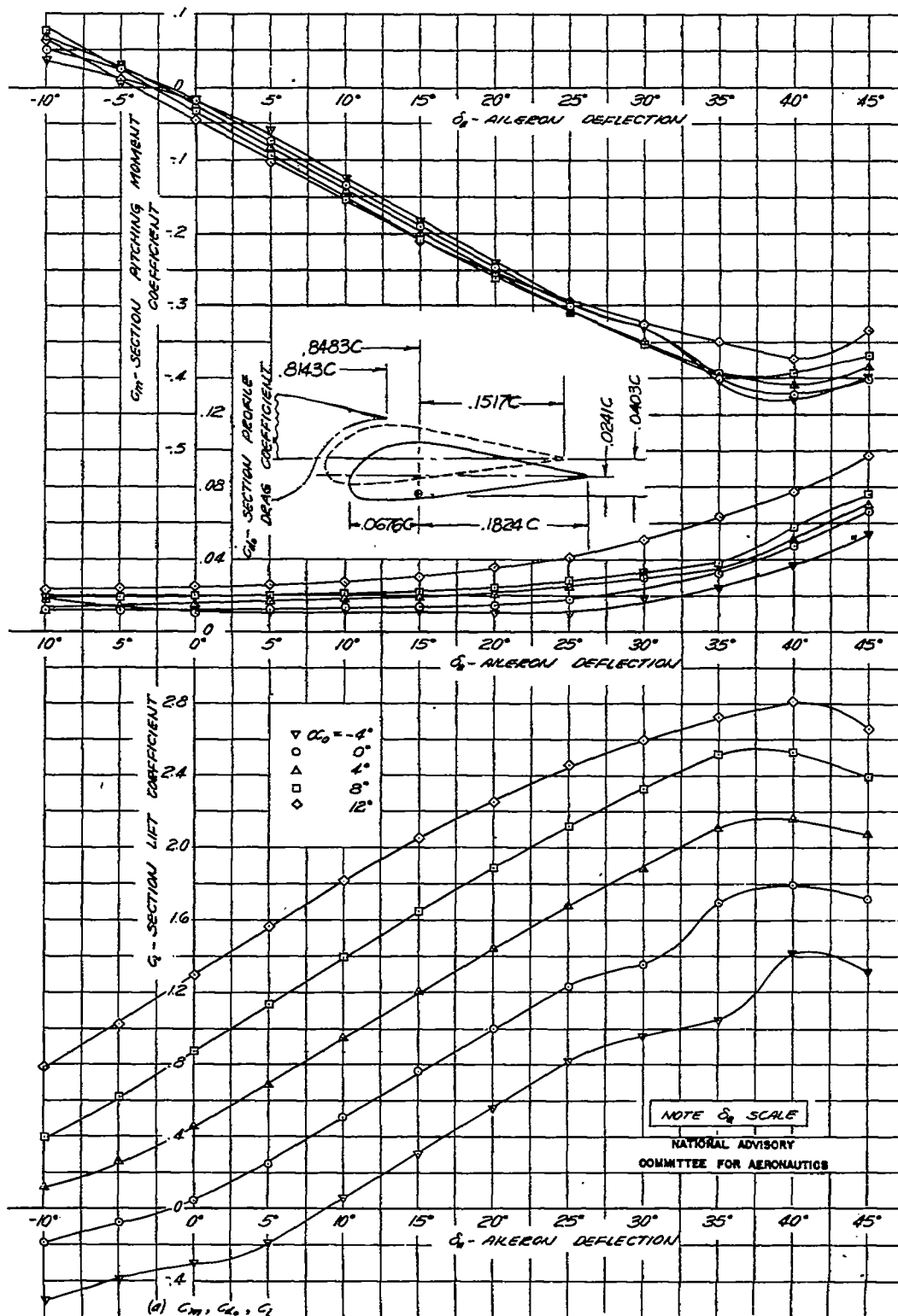
FIGURE 17.-SECTION AERODYNAMIC CHARACTERISTICS OF THE NACA 66(215)-216 ( \alpha=0.6 ) AIRFOIL EQUIPPED WITH THE 0.25-CHORD STRAIGHT SIDED AILERON WITH A 37.05 PERCENT AERODYNAMIC BALANCE; HINGE LOCATION W .
