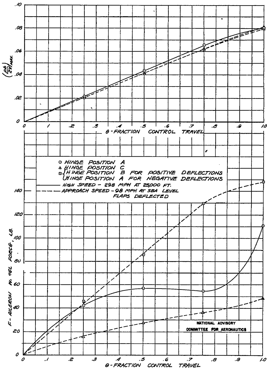
FIGURE 21 - VARIATION OF (pb/2V)_{MAX} AND WHEEL FORCE WITH CONTROL TRAVEL IN ROLLS WITH THE RUDDER LOCKED FOR THE EXEMPLARY AIRPLANES EQUIPPED WITH THE 0.25 CHORD NORMAL PROFILE AILERON.
