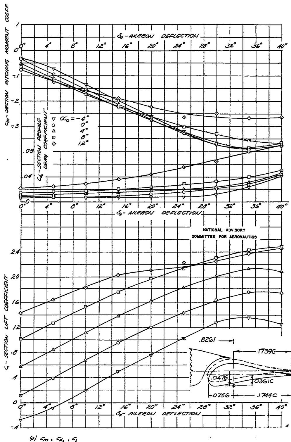
FIGURE 11 - SECTION AERODYNAMIC CHARACTERISTICS OF THE NACA 66(215)-216 ( q=6 ) AIRFOIL EQUIPPED WITH THE 0.25-CHORD NORMAL PROFILE AILERON WITH A 43.35 PERCENT AERODYNAMIC BALANCE; HINGE LOCATION E.
