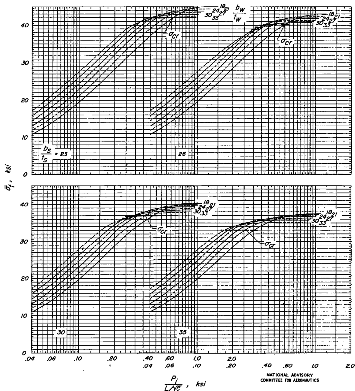
Figure 7.- Design chart for 24S-T Y-panels of the proportions tested. t_w/t_s = 0.40 .
