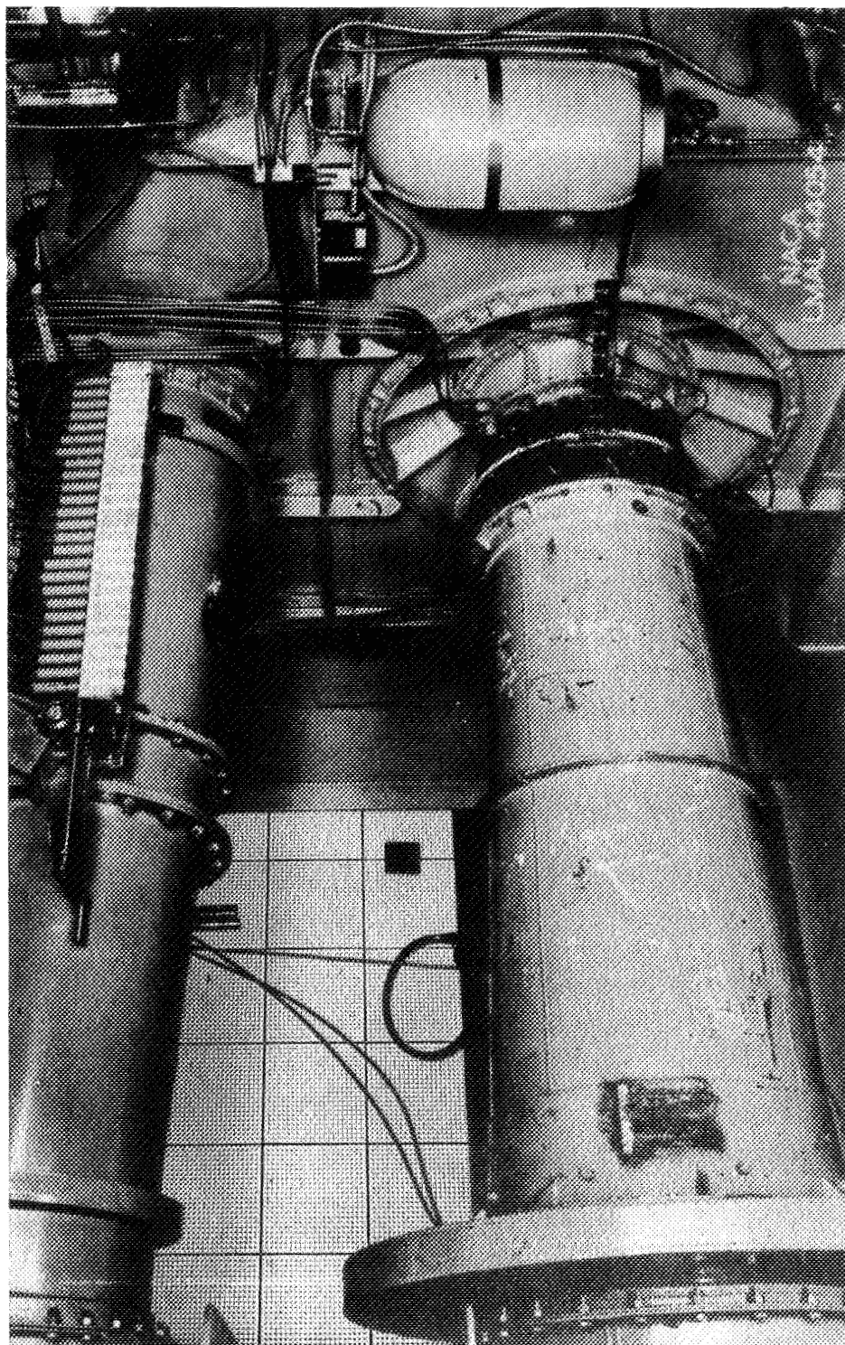
Figure 12.- Supersonic-compressor test setup. The throttling-valve lever and protractor are visible on the upper return section. The velocity-of-sound meter for determining the composition of the test fluid is shown at the upper right.
