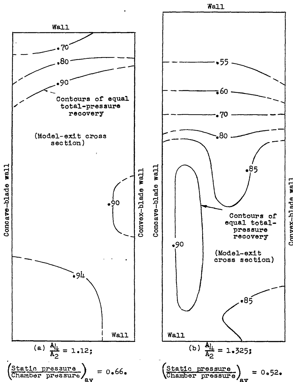
Figure 7.- Typical contour curves of total-pressure recovery \left( \frac{\text{Local total pressure}}{\text{Chamber pressure}} \right) showing the extent of the separated regions of low total pressure over the model exit cross-sectional areas. Two models of different expansion ratio are shown.
