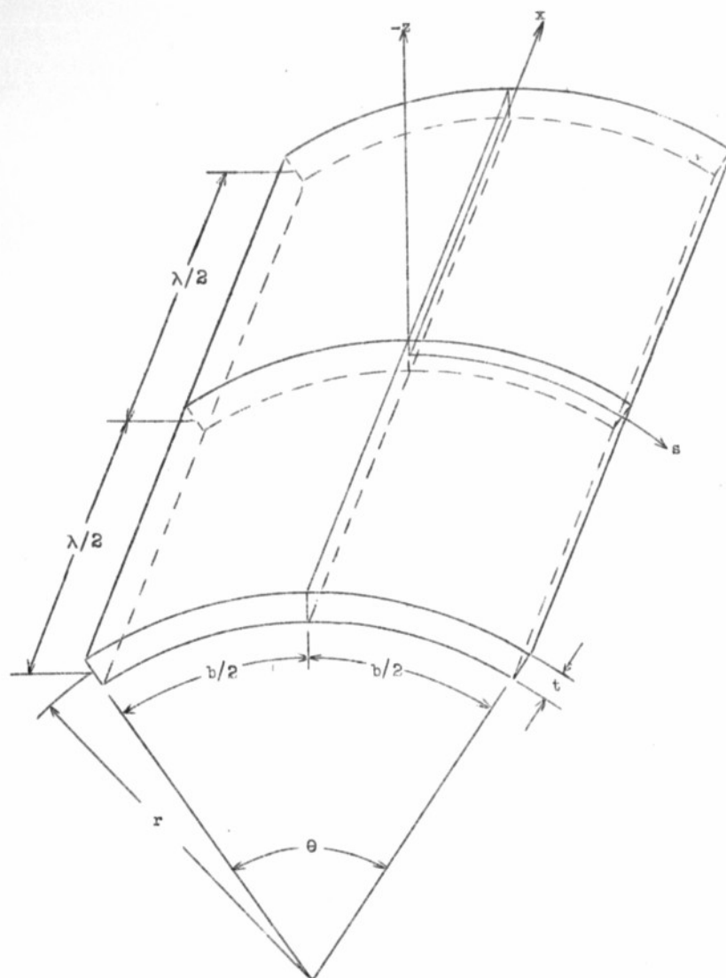
Figure 1.- Coordinate system for curved sheet.
