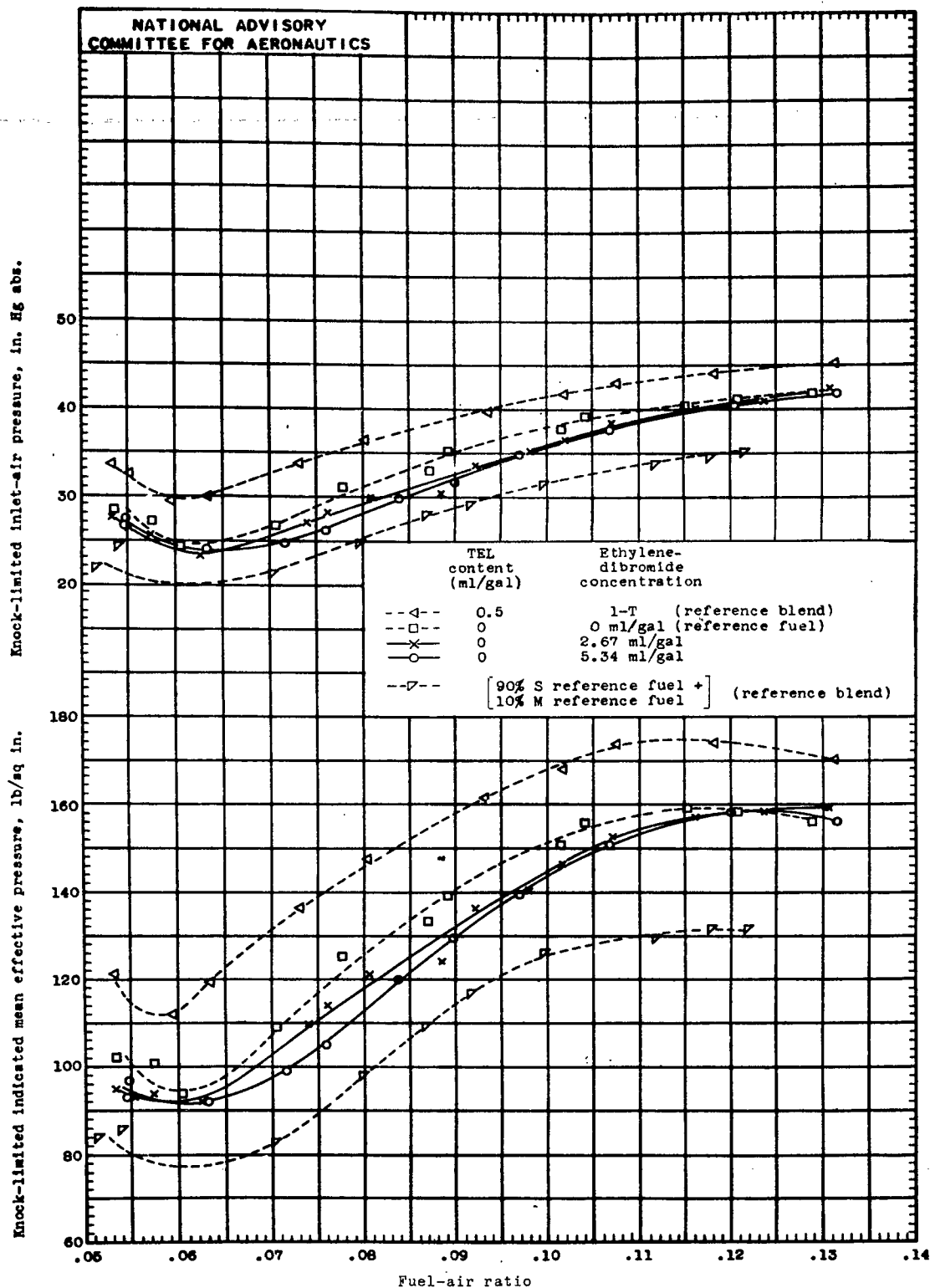
Figure 2. - Effect of ethylene dibromide in unleaded S reference fuel on knock-limited performance of a CFR engine. Engine speed, 1800 rpm; compression ratio, 7.0; spark advance, 45° B.T.C.; coolant temperature, 375° F; inlet-air temperature, 225° F.
