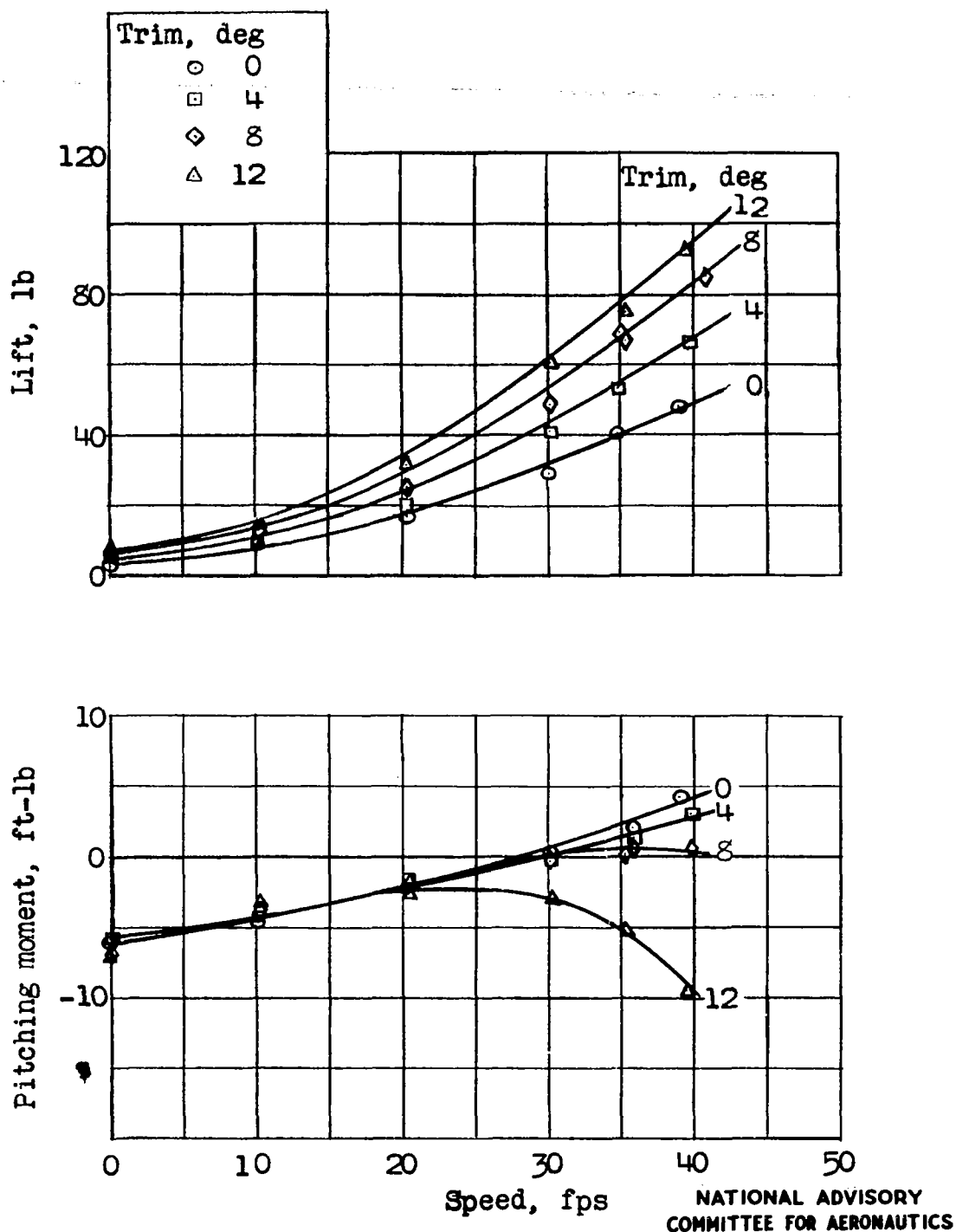
Figure 5 .- Model 203A. Variation in aerodynamic lift and pitching moment with speed. Full power, 4,550 rpm; center of gravity, 24 percent M.A.C.; flap deflection, 20^{\circ} ; elevator deflection, -10^{\circ} .
