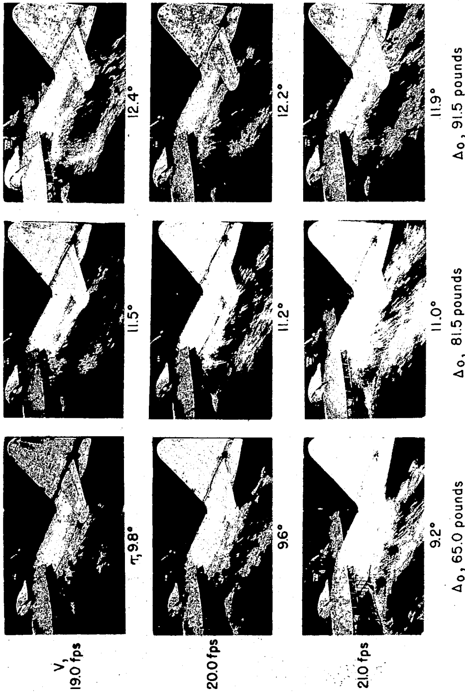
Figure 10.- Model 203A. Concluded.
