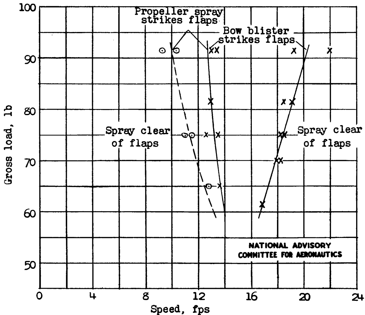
Figure 12.- Model 203A . Speed range over which spray strikes the flaps. Full power, 4,500 rpm; center of gravity, 28 percent M.A.C.; flap deflection, 20^{\circ} ; elevation deflection, -10^{\circ} .
