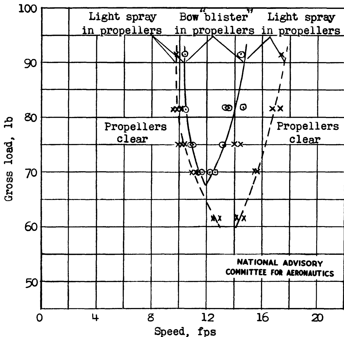
Figure 6 .- Model 203A. Speed range over which spray enters the propellers. Full power, 4,550 rpm; center of gravity, 28 percent M.A.C; flap deflection, 20^{\circ} ; elevator deflection, -10^{\circ} .
