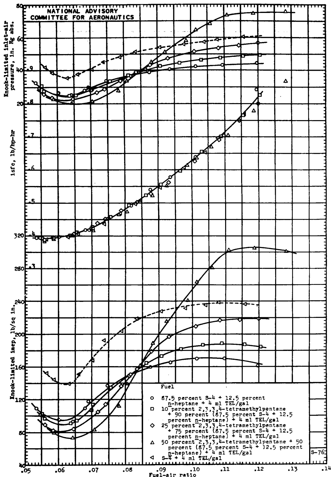
Figure 3. - The knock-limited performance of leaded blends of 2,3,3,4-tetramethylpentane and a base fuel consisting of 87.5 percent S-4 plus 12.5 percent n-heptane in an F-4 engine.
