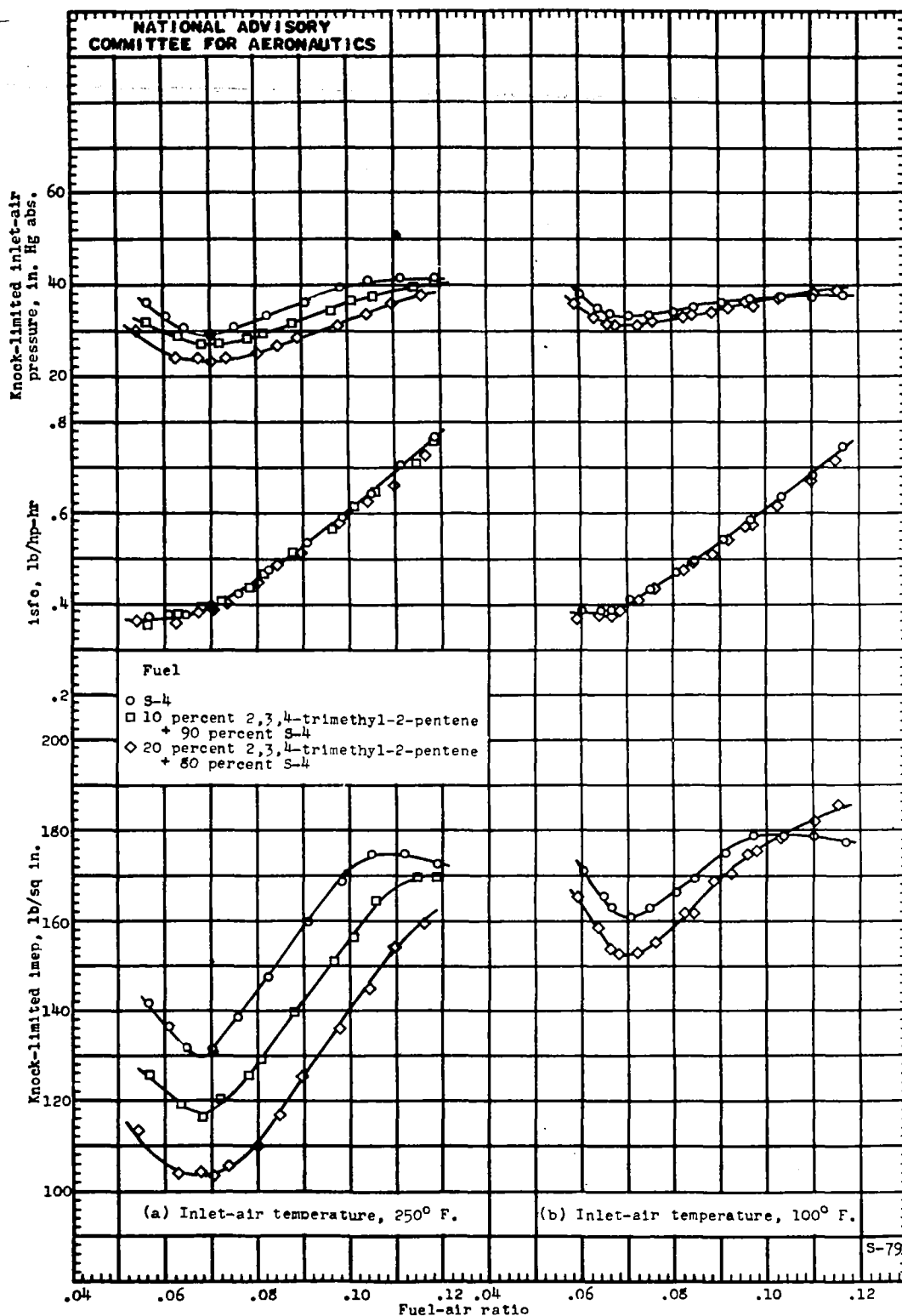
Figure 19. - The knock-limited performance of unleaded blends of 2,3,4-trimethyl-2-pentene and S-4 reference fuel in a 17.6 engine. Compression ratio, 7.0; engine speed, 1800 rpm; spark advance, 30° B.T.C.; outlet-coolant temperature, 212° F.
