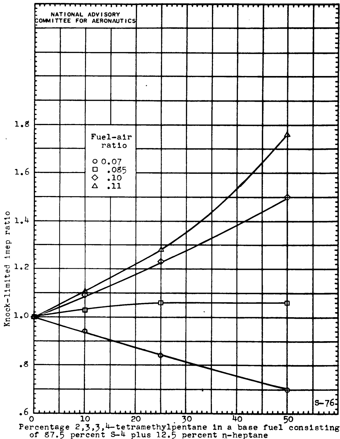
Figure 7. - The blending sensitivity of 2,3,3,4-tetramethylpentane in a base fuel consisting of 87.5 percent S-4 plus 12.5 percent n -heptane. F-4 engine; final blends leaded to 4 ml TEL per gallon.
