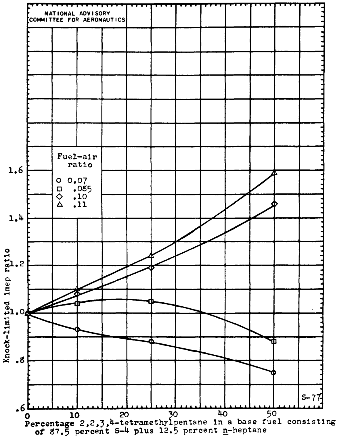
Figure 6. - The blending sensitivity of 2,2,3,4-tetramethylpentane in a base fuel consisting of 87.5 percent S-4 plus 12.5 percent n -heptane. F-4 engine; final blends leaded to 4 ml TEL per gallon.
