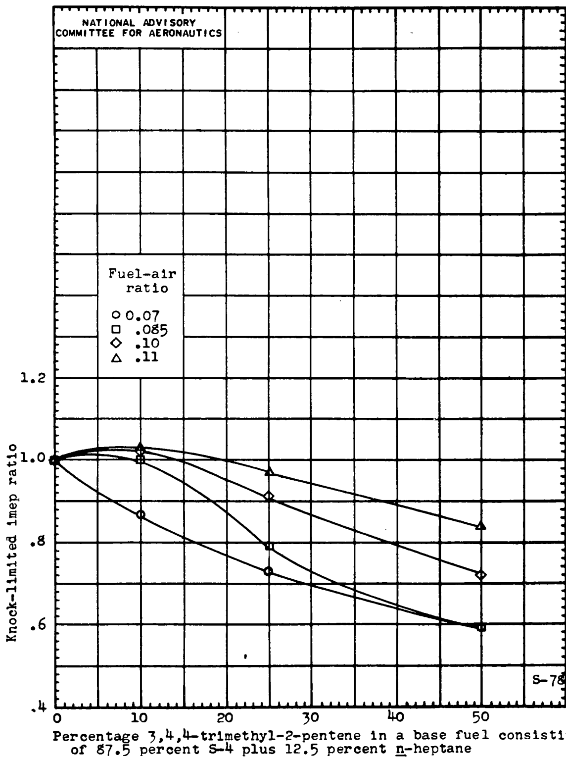
Figure 8. - The blending sensitivity of 3,4,4-trimethyl-2-pentene in a base fuel consisting of 87.5 percent S-4 plus 12.5 percent n -heptane. F-4 engine; final blends leaded to 4 ml TEL per gallon.
