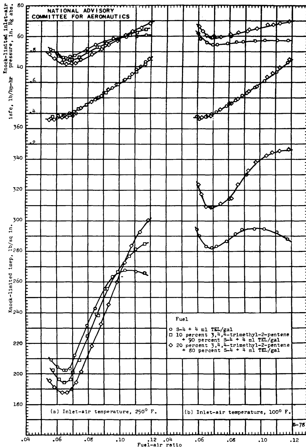
Figure 17. - The knock-limited performance of leaded blends of 3,4,4-trimethyl-2-pentene and S-4 reference fuel in a 17.6 engine. Compression ratio, 7.0; engine speed, 1800 rpm; spark advance, 30° B.T.C.; outlet-coolant temperature, 212° F.
