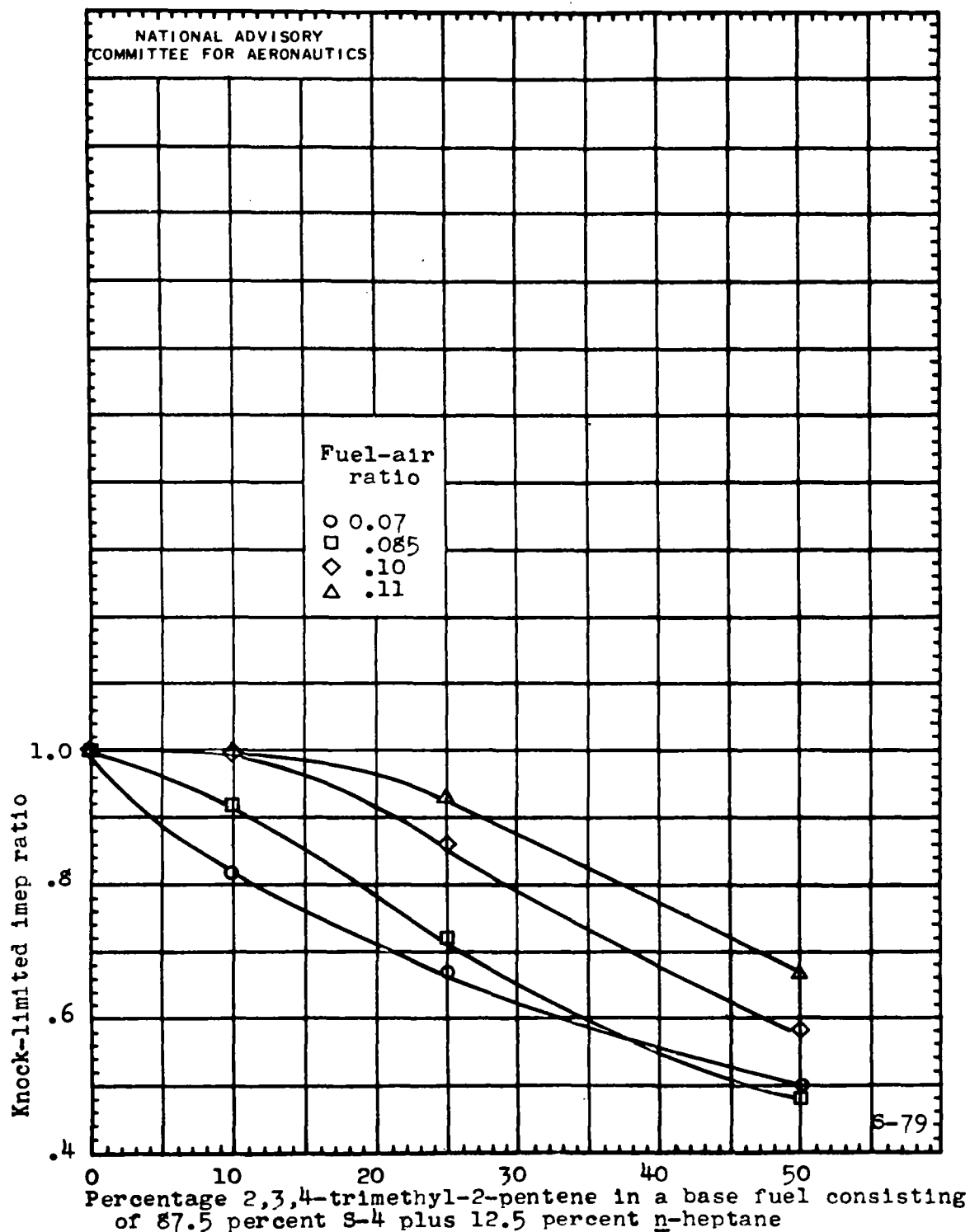
Figure 9. - The blending sensitivity of 2,3,4-trimethyl-2-pentene in a base fuel consisting of 87.5 percent S-4 plus 12.5 percent n -heptane. F-4 engine; final blends leaded to 4 ml TEL per gallon.
