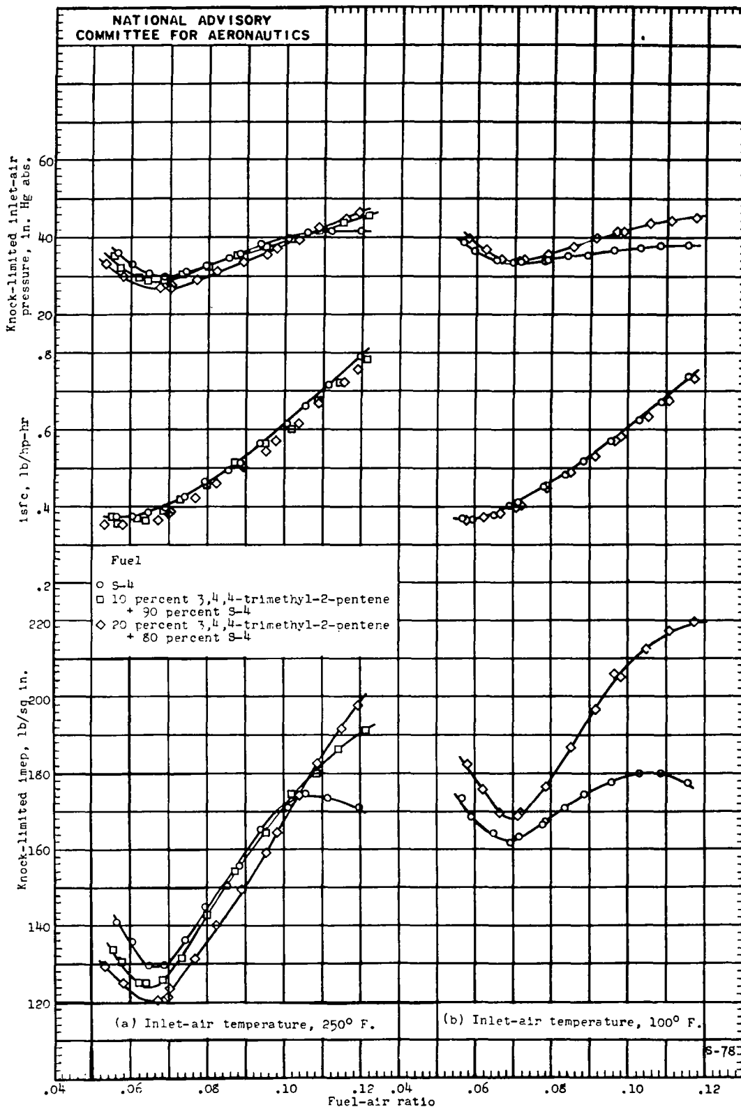
Figure 16. - The knock-limited performance of unleaded blends of 3,4,4-trimethyl-2-pentene and S-4 reference fuel in a 17.6 engine. Compression ratio, 7.0; engine speed, 1800 rpm; spark advance, 30° B.T.C.; outlet-coolant temperature, 212° F.
