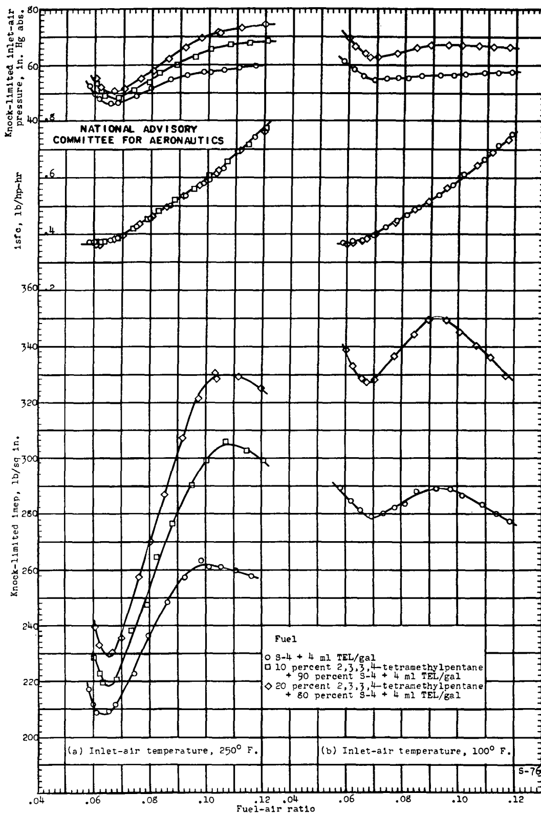
Figure 14. - The knock-limited performance of leaded blends of 2,3,3,4-tetramethylpentane and S-4 reference fuel in a 17.6 engine. Compression ratio, 7.0; engine speed, 1800 rpm; spark advance, 30° B.T.C.; outlet-coolant temperature, 212° F.
