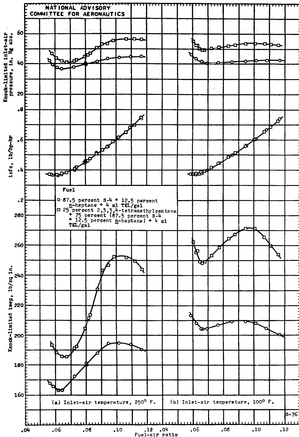
Figure 15. - The knock-limited performance of leaded blends of 2,3,3,4-tetramethylpentane and a base fuel consisting of 87.5 percent S-4 plus 12.5 percent n -heptane in a 17.6 engine. Compression ratio, 7.0; engine speed, 1800 rpm; spark advance, 30° B.T.C.; outlet-coolant temperature, 212° F.
