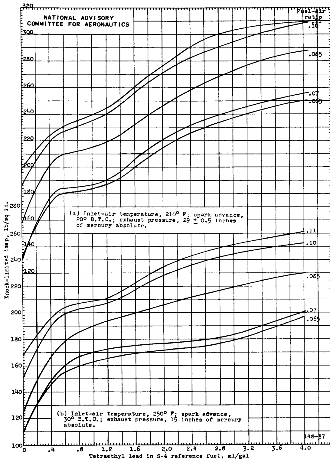
Figure 29. - Relation between knock-limited indicated mean effective pressure and lead concentration in S-4 reference fuel for different fuel-air ratios. Full-scale cylinder; compression ratio, 7.3; engine speed, 2000 rpm.
