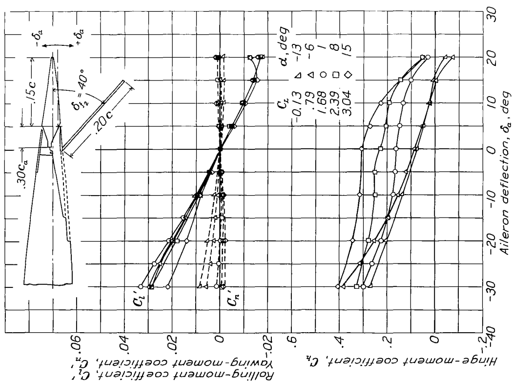
Figure 11.- \delta_{f_1} = 40^\circ ; \delta_{f_2} = 40^\circ .
