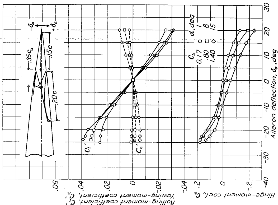
Figure 16.- \delta_{f_1} = 0^\circ ; \delta_{f_2} = 0^\circ . Balance 0.35c a
