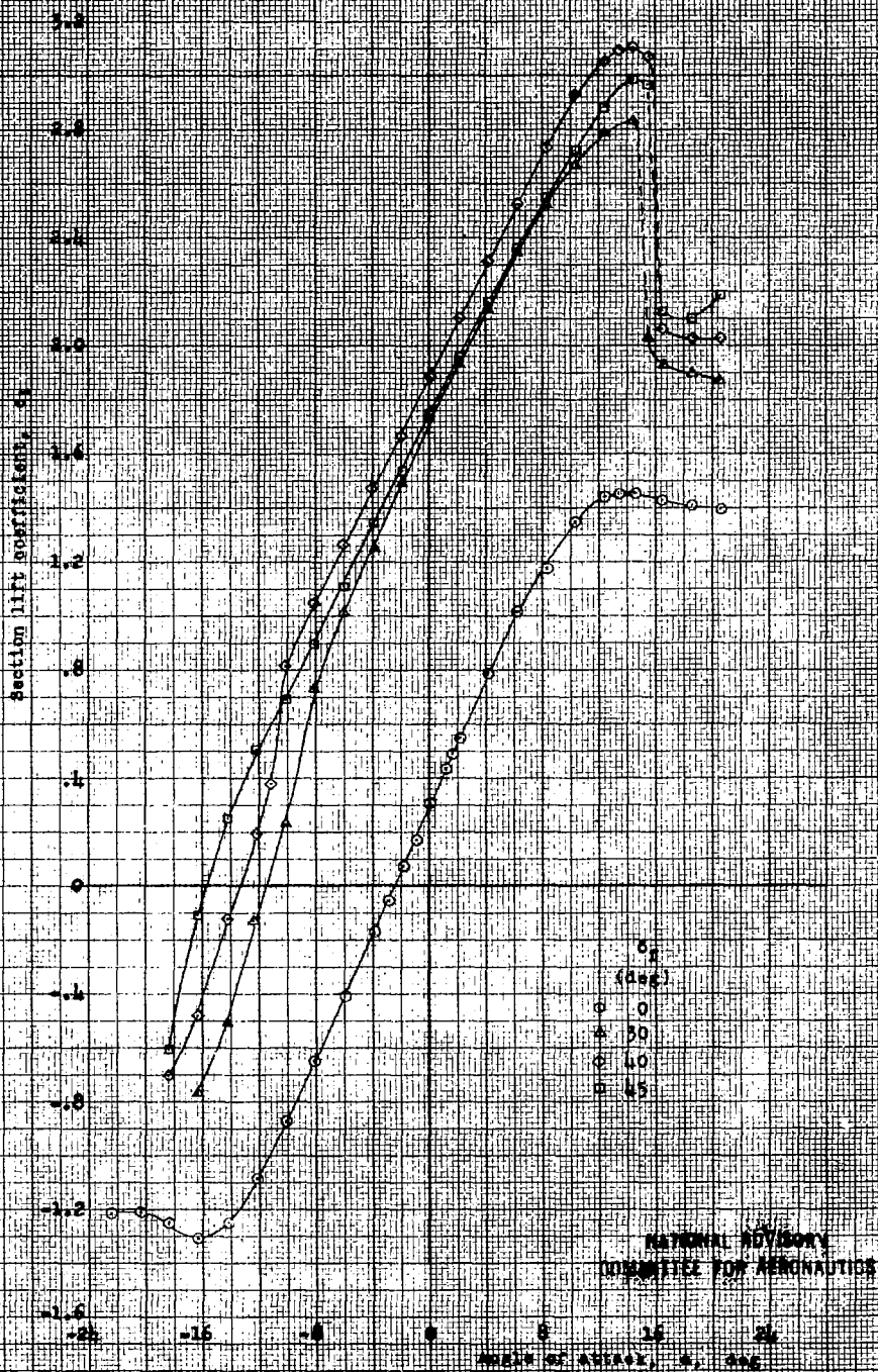
Figure 2.- Lift characteristics of inboard wing section model of KB-30 airplane with slotted flap. Flap 1, slot entry 1; R, 9 \times 10^6 .
