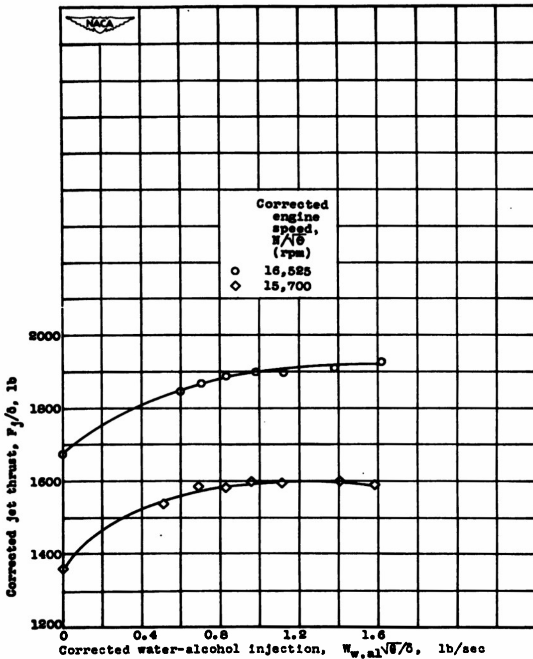
Figure 11. - Effect of water-alcohol injection rate on corrected jet thrust for two engine speeds at standard sea level and ram-pressure ratio of 0.995. Alcohol, 20 percent by weight.
