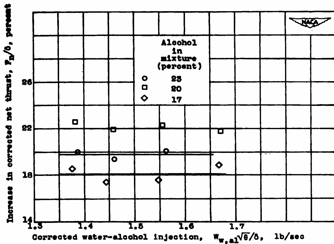
Figure 5. - Increase in corrected net thrust for three water-alcohol mixtures at NACA standard altitude of 10,000 feet and ram-pressure ratio of 1.095. Corrected engine speed, N/\sqrt{\theta} , 16,000 rpm.
