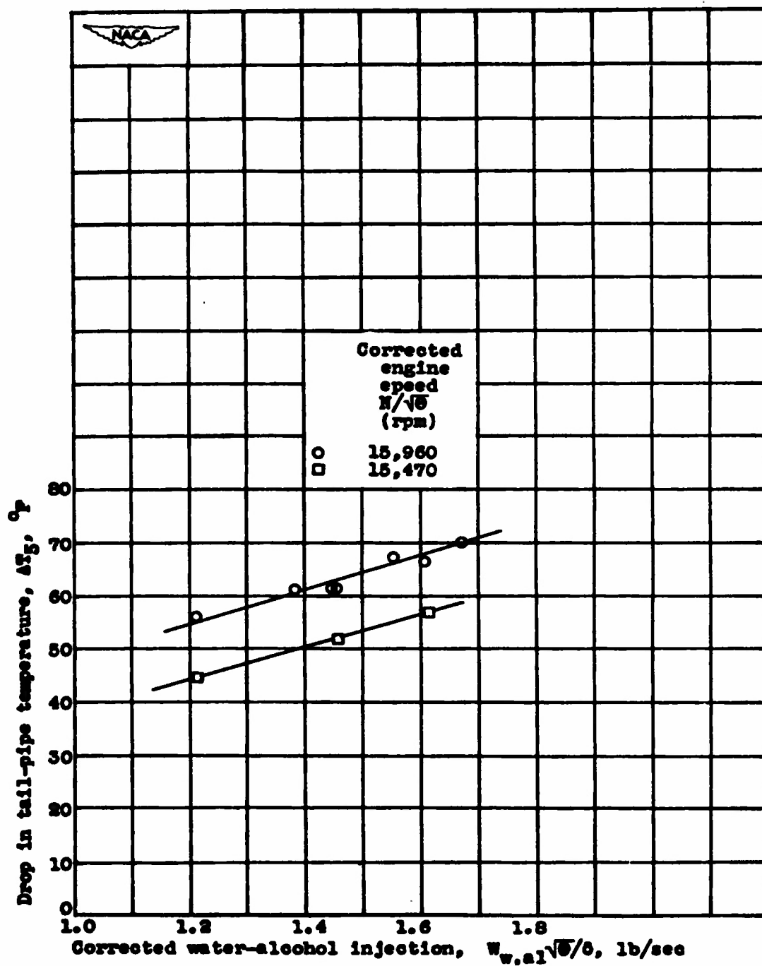
Figure 9. - Decrease in tail-pipe temperature from normal for various water-alcohol injection rates and two corrected engine speeds at NACA standard altitude of 10,000 feet and ram-pressure ratio of 1.095. Alcohol, 20 percent by weight.
