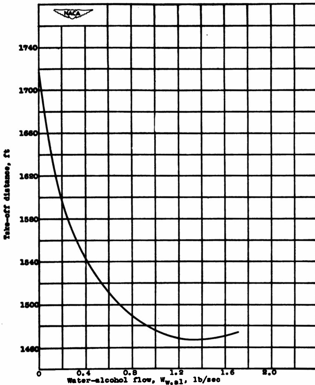
Figure 12.- Thrust-augmented sea-level take-off distances for idealized twin-engine airplane as affected by various water-alcohol (20-percent alcohol by weight) injection rates. Maximum lift-drag ratio, 12; wing loading, 28.5 pounds per square foot; take-off weight, 12,000 pounds.
