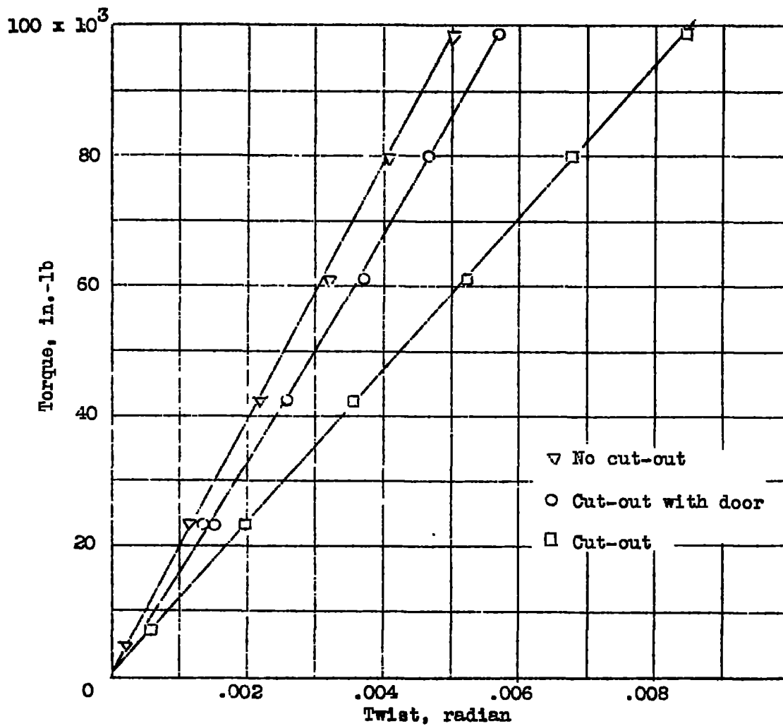
Figure 3.- Torque-twist, curves for box.
