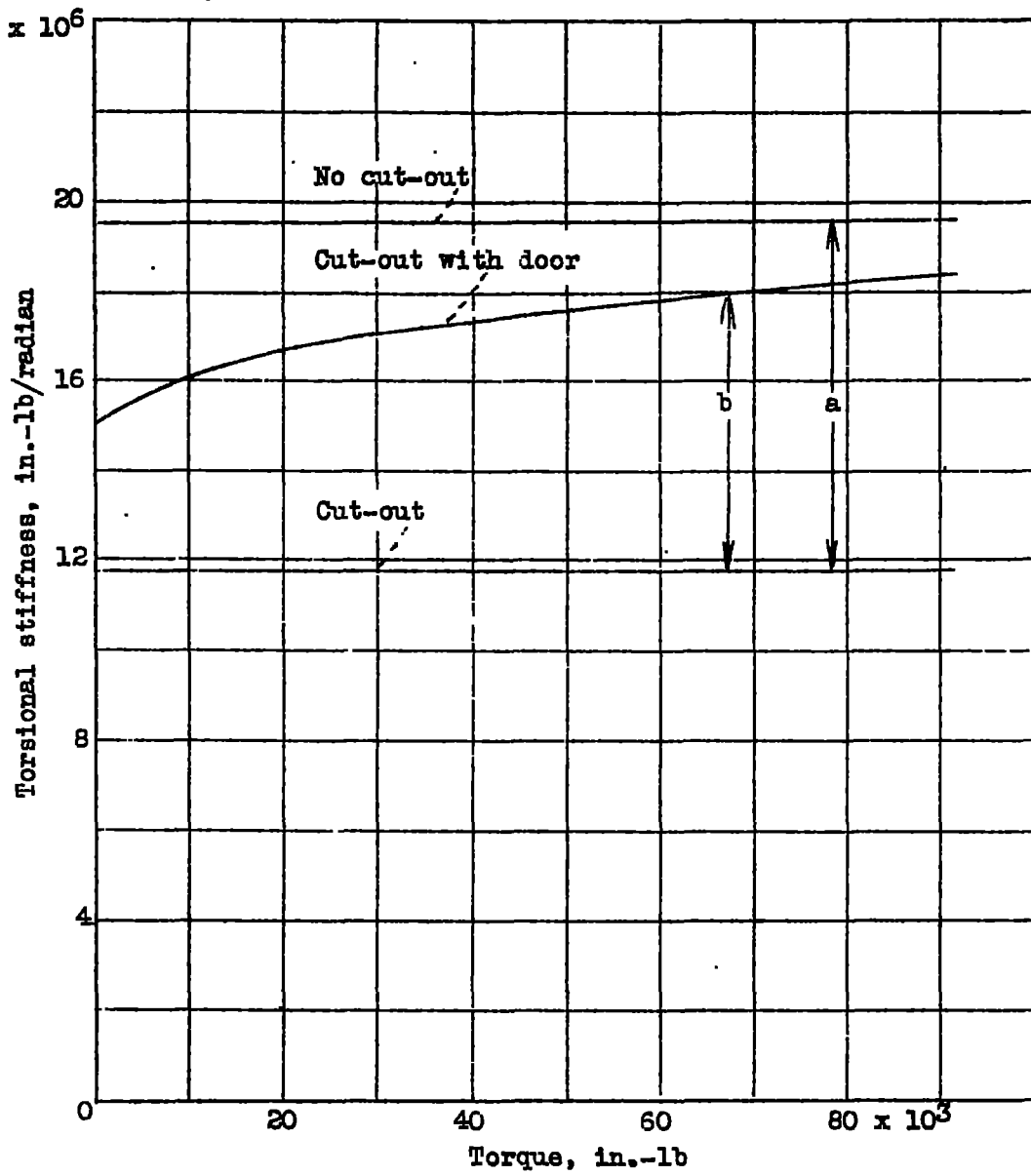
Figure 4.- Torsional stiffness of box.
