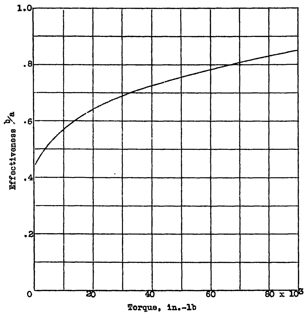
Figure 5.- Effectiveness of door.
