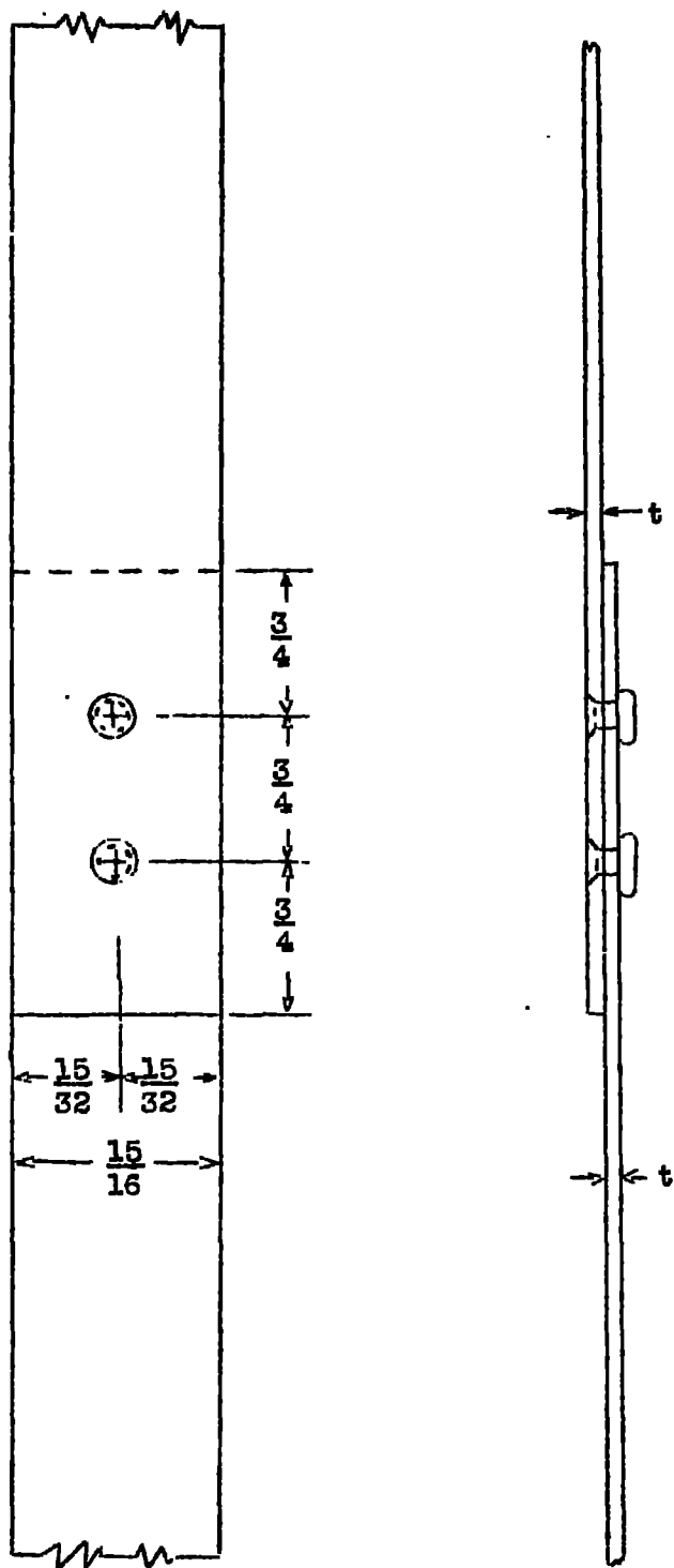
Figure 1.- Test specimen.
