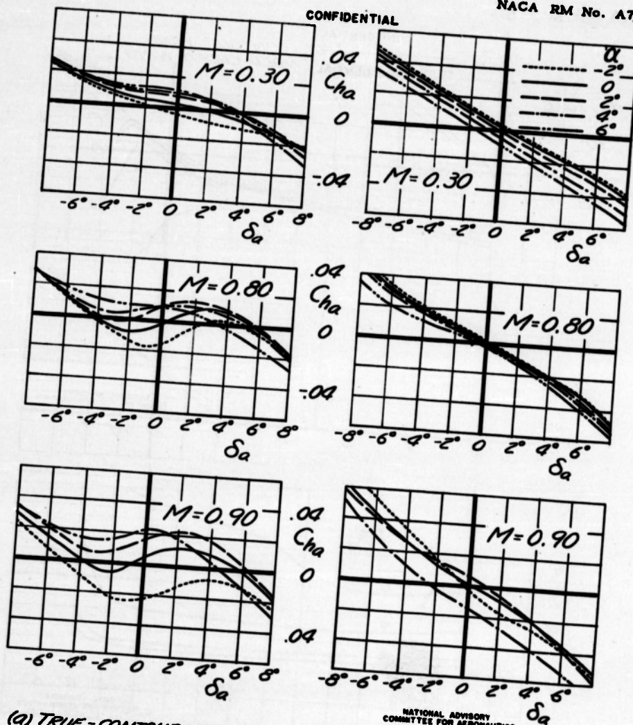
FIGURE 9.- EFFECT OF WING TRAILING-EDGE CONTOUR ON THE AILERON HINGE MOMENT
