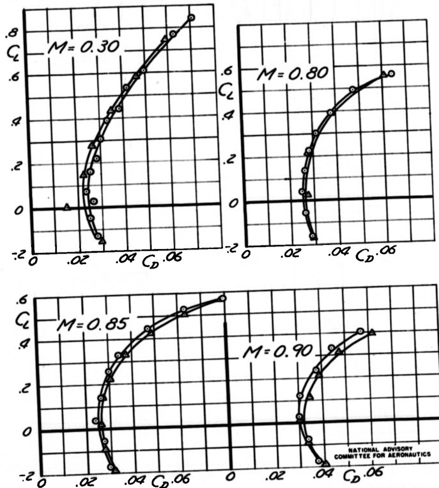
FIGURE 22.-EFFECT OF WING LEADING-EDGE EXTENSION ON THE TAIL-ON DRAG
