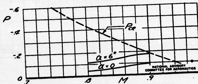
(b) MAXIMUM STATIC PRESSURE DECREASE ON THE TUNNEL WALL ABOVE THE WING ROOT OF THE MODEL
