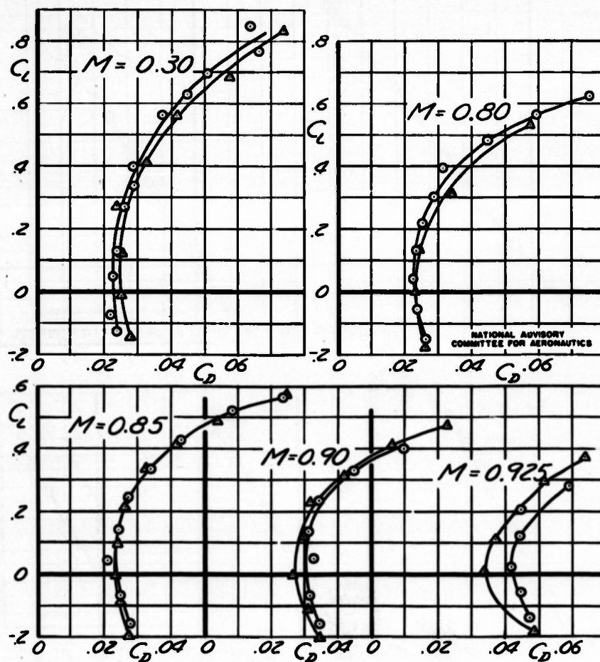
FIGURE 17.-EFFECT OF FUSELAGE CONTOUR ON THE TAIL-OFF DRAG
