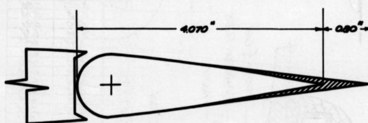
(b) SECTION OF THE WING THROUGH THE AILERON NORMAL TO THE QUARTER-CHORD LINE SHOWING THE TRAILING-EDGE EXTENSION.
