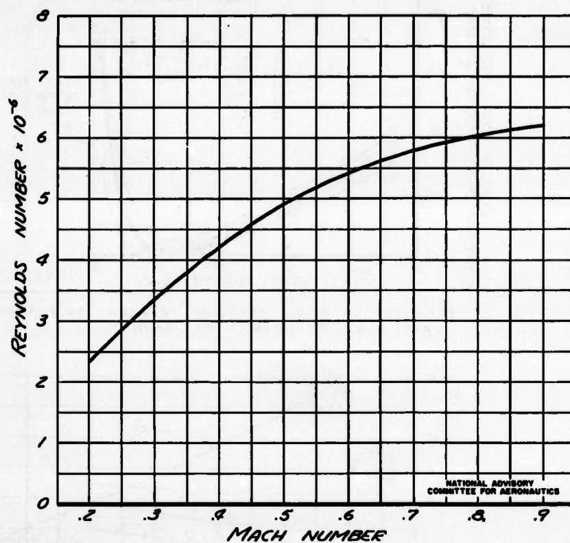
FIGURE 7.- VARIATION OF REYNOLDS NUMBER WITH MACH NUMBER FOR THE MODEL IN THE AMES 16-FOOT HIGH-SPEED WIND TUNNEL
