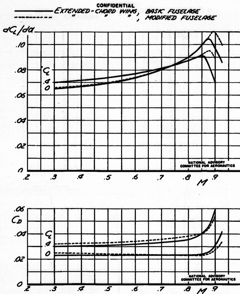
FIGURE 18. - EFFECT OF FUSELAGE CONTOUR ON THE VARIATION OF LIFT-CURVE SLOPE AND DRAG COEFFICIENT WITH MACH NUMBER
