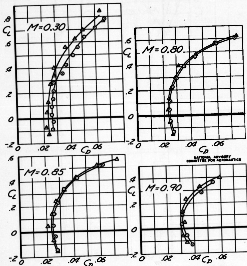
FIGURE 12.-EFFECT OF WING TRAILING-EDGE CONTOUR ON THE TAIL-OFF DRAG CONFIDENTIAL
