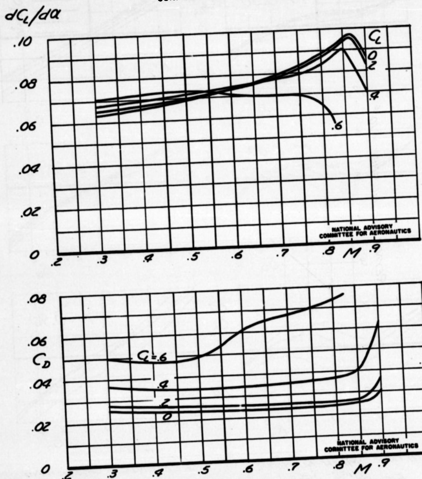
FIGURE 8.- LIFT AND DRAG CHARACTERISTICS FOR THE MODEL WITH THE TRUE-CONTOUR WING, TAIL OFF CONFIDENTIAL
