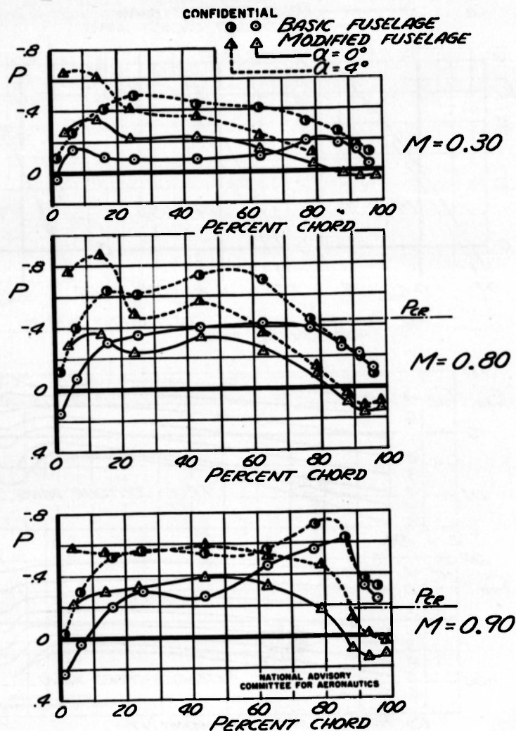
FIGURE 15.—EFFECT OF FUSELAGE CONTOUR ON THE PRESSURE DISTRIBUTION ALONG THE WING-FUSELAGE INTERSECTION.
