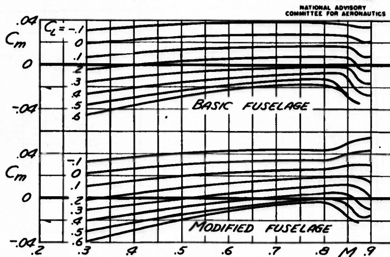
FIGURE 20.- EFFECT OF FUSELAGE CONTOUR ON THE TAIL-ON PITCHING MOMENT
