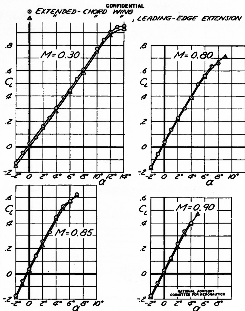
FIGURE 21.- EFFECT OF WING LEADING-EDGE EXTENSION ON THE TAIL-ON LIFT
