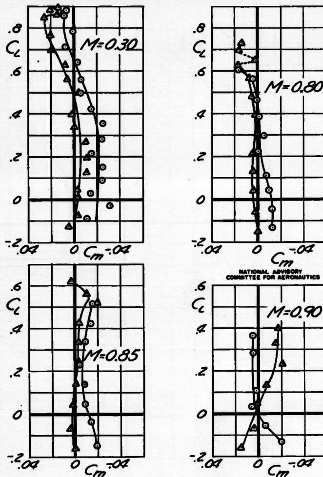
FIGURE 13.- EFFECT OF WING TRAILING-EDGE CONTOUR ON THE TAIL-OFF PITCHING MOMENT CONFIDENTIAL
