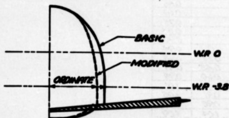
FIGURE 4.- COMPARISON OF BASIC AND MODIFIED FUSELAGE CONTOURS
