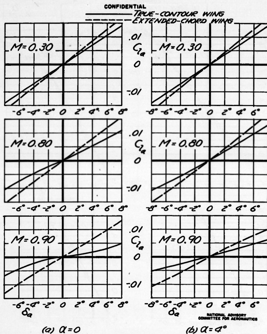
FIGURE 10.-EFFECT OF WING TRAILING-EDGE CONTOUR ON AILERON EFFECTIVENESS
