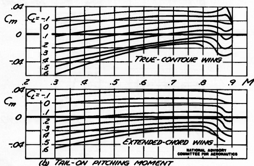
FIGURE 14.—EFFECT OF WING TRAILING-EDGE CONTOUR ON THE TAIL-ON PITCHING MOMENT
