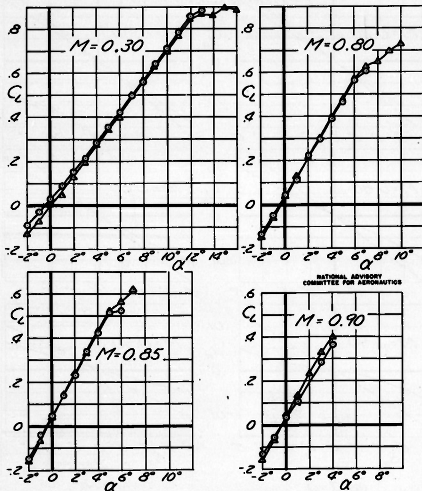
FIGURE 11.-EFFECT OF WING TRAILING-EDGE CONTOUR ON THE TAIL-OFF LIFT
