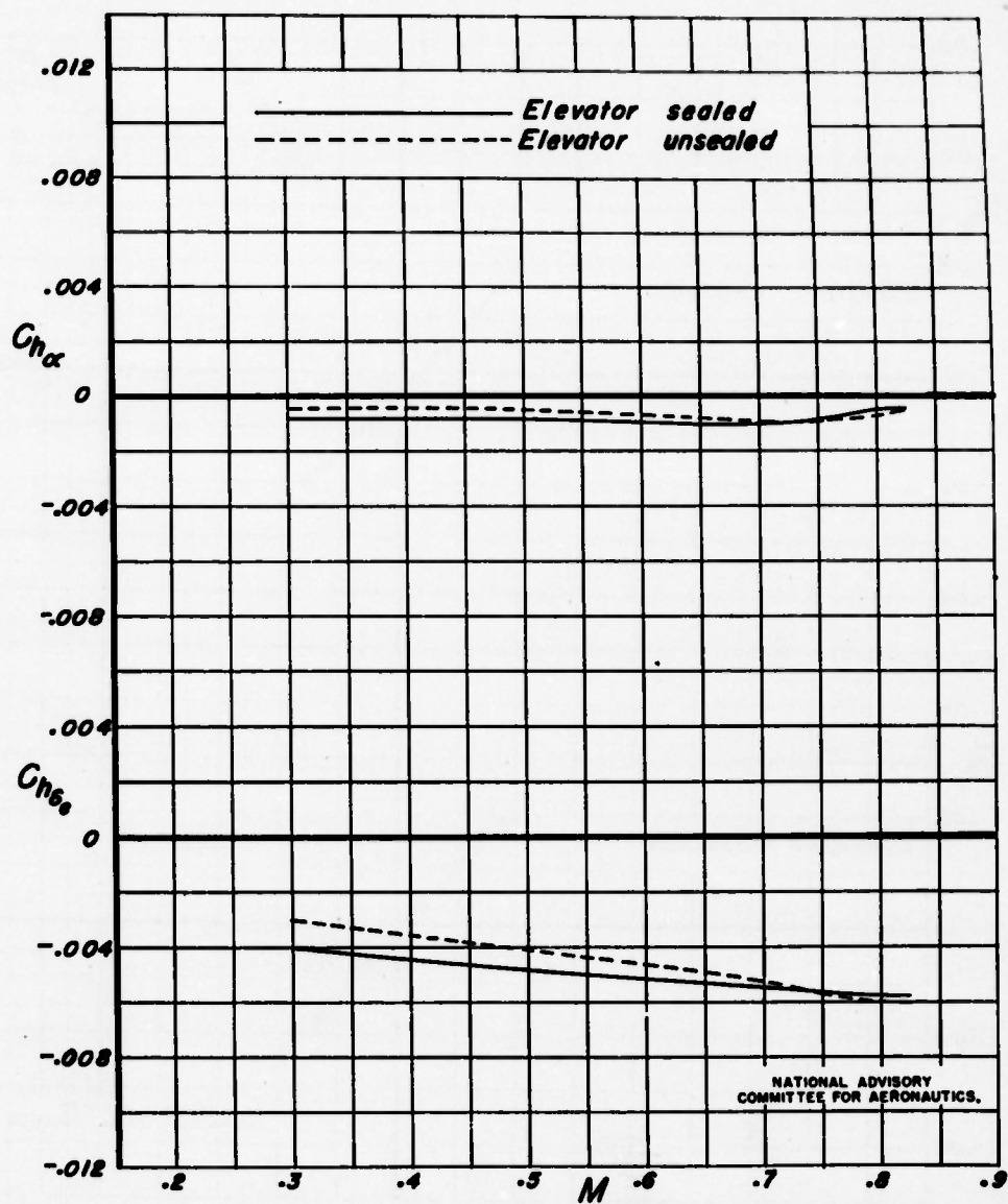
Figure 19.— Variation of elevator hinge-moment parameters with Mach number for the sealed and unsealed overhang-balance elevator having a reduced semispan.
