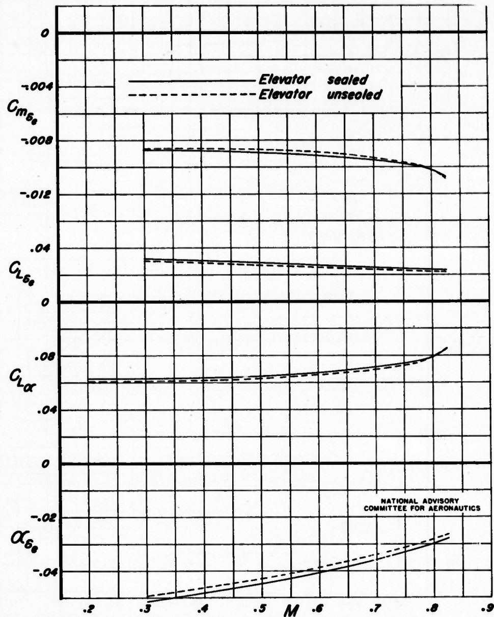
Figure 17.—Variation of pitching-moment, lift, and elevator effectiveness parameters with Mach number for the sealed and unsealed overhang-balance elevator having a reduced semispan.
