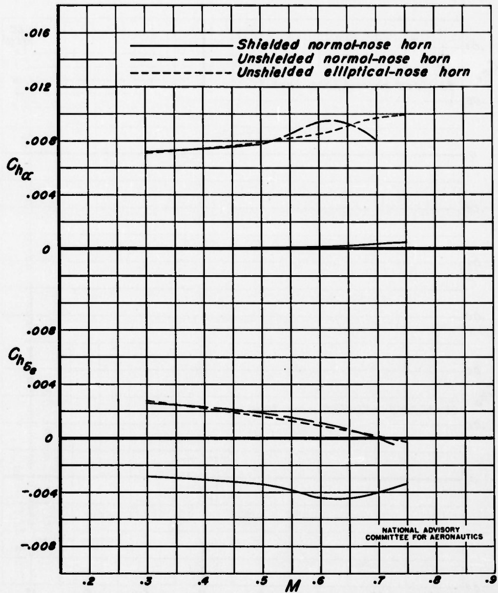
Figure 28.—Variation of elevator hinge-moment parameters with Mach number for the shielded and unshielded horn-balance elevators.
