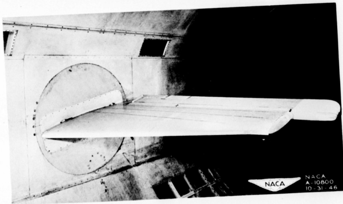
(b) Overhang with unshielded tip.
