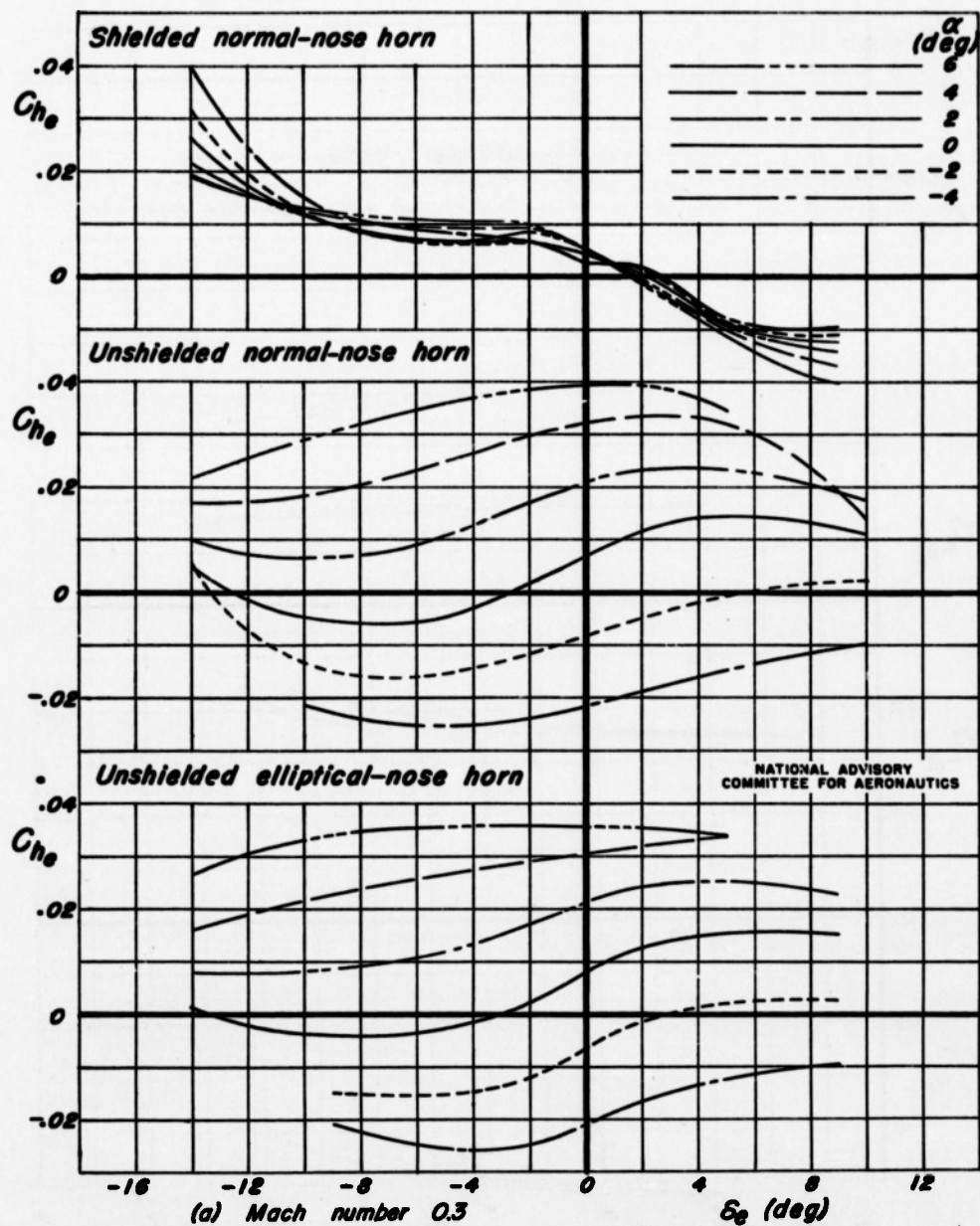
Figure 27.—Variation of hinge-moment coefficient with elevator angle for the shielded and unshielded horn-balance elevators.
