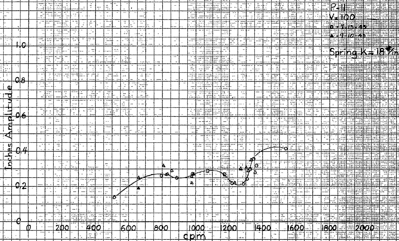
Figure 28: - Forced vibration response.
