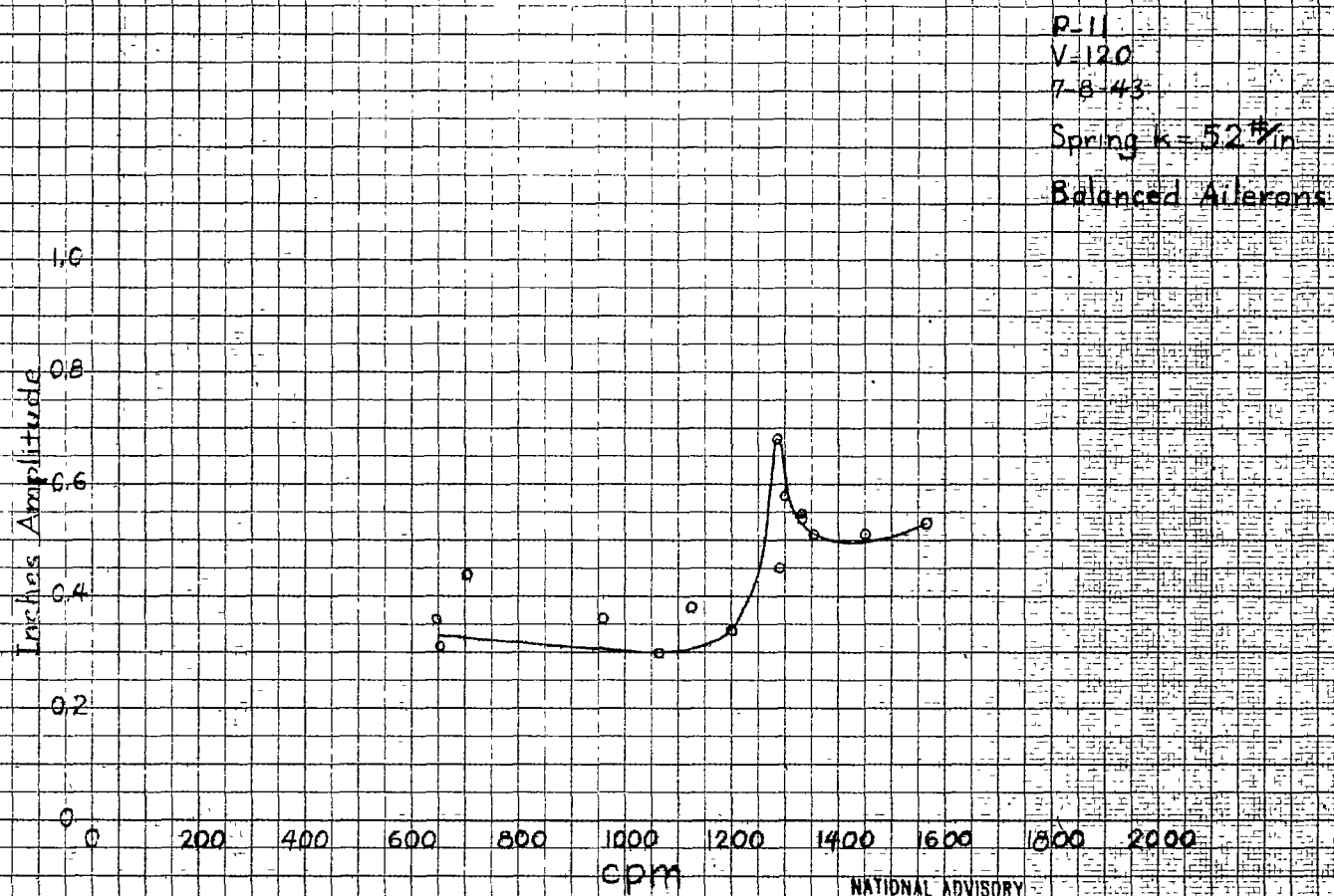
Figure 24. - Forced vibration response.
