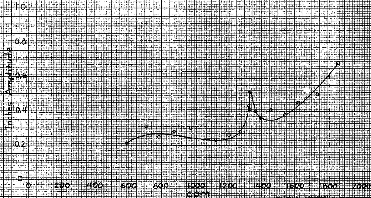
Figure 23, - Forced vibration response.
