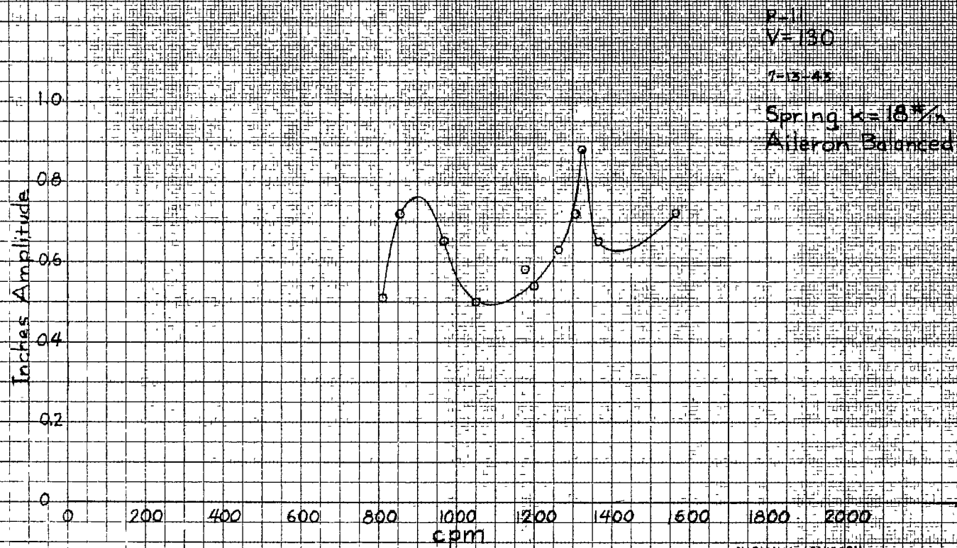
Figure 33. - Forced vibration response.
