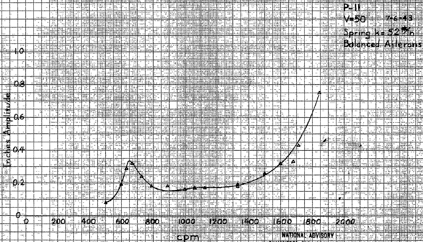
Figure 19. - Forced vibration response.
