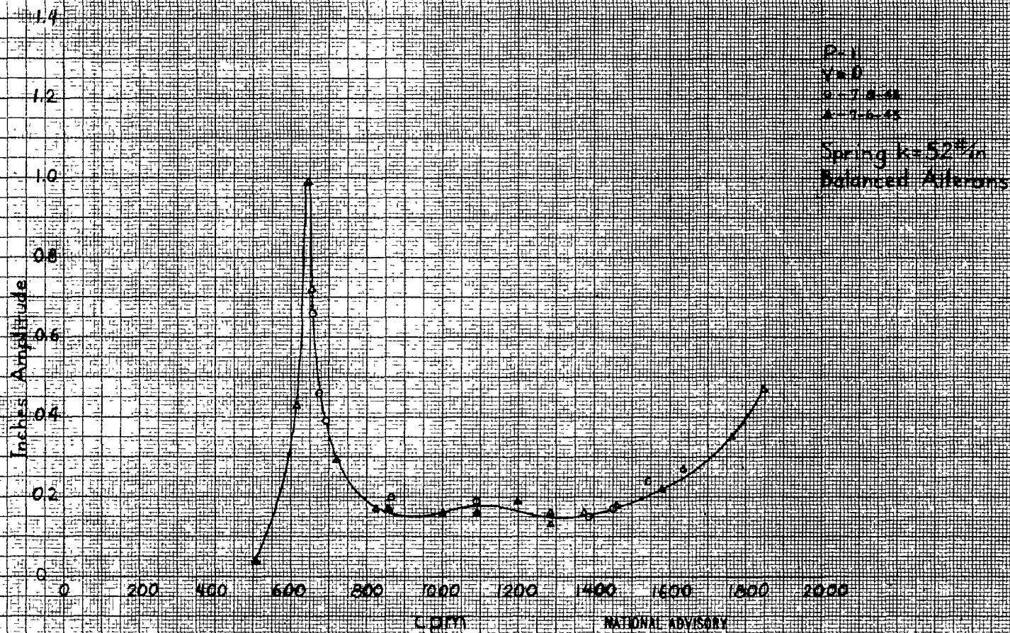
Figure 18. - Forced vibration response.
