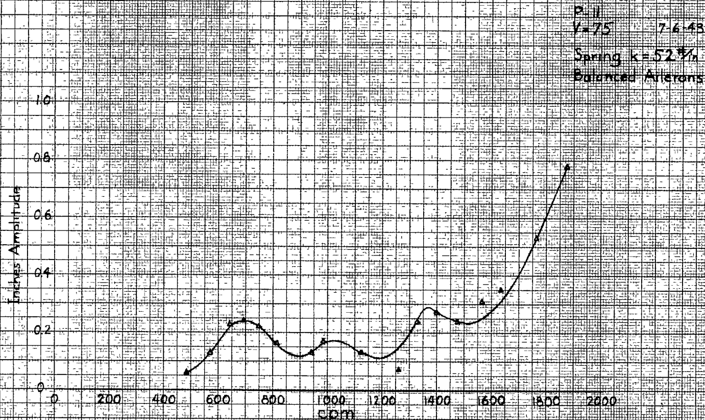
Figure 20 - Forced vibration response.
