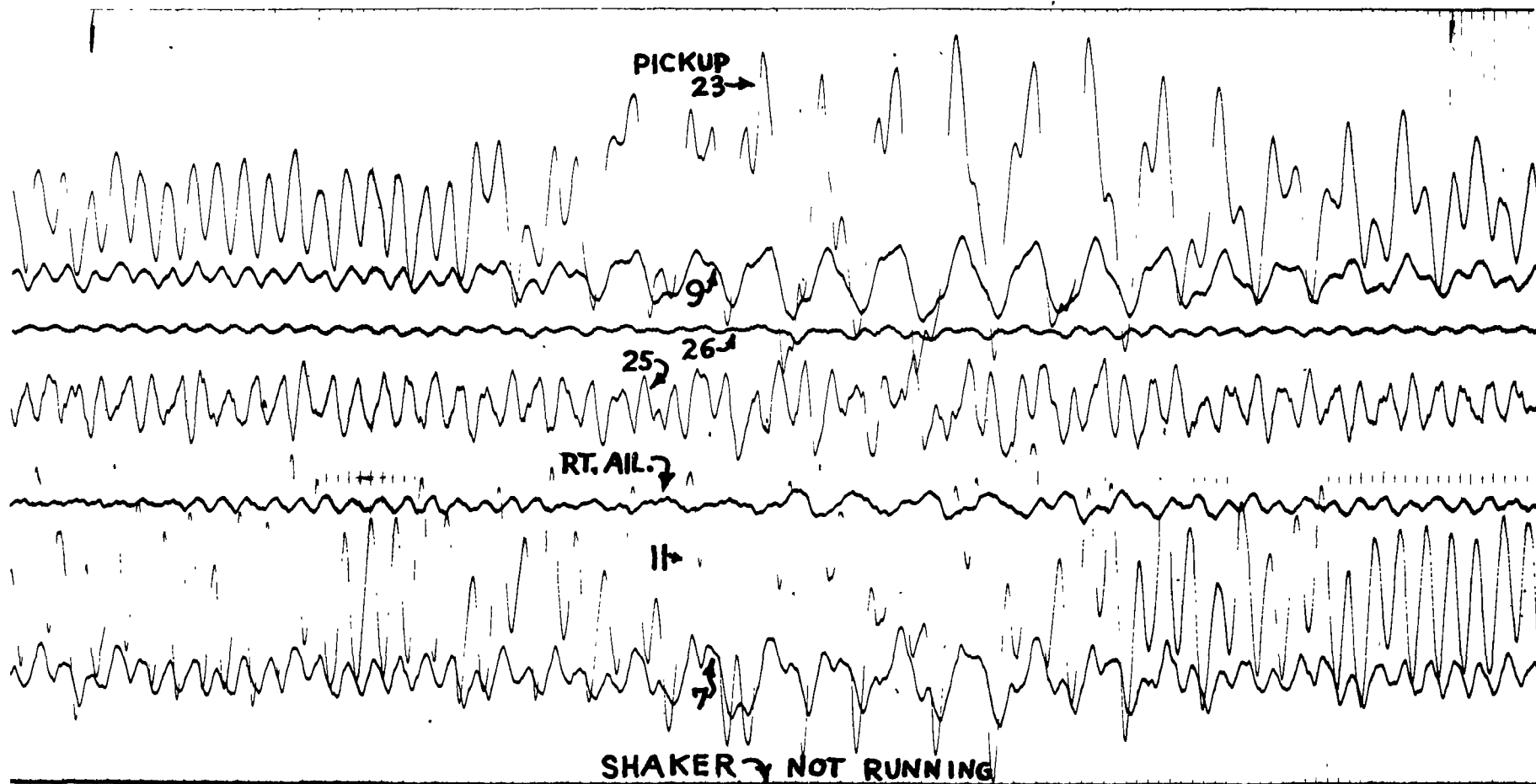
Fig. 15 ACCELERATED RUN, 130 TO 150 M.P.H BURST AT ABOUT 1000 C.P.M.
