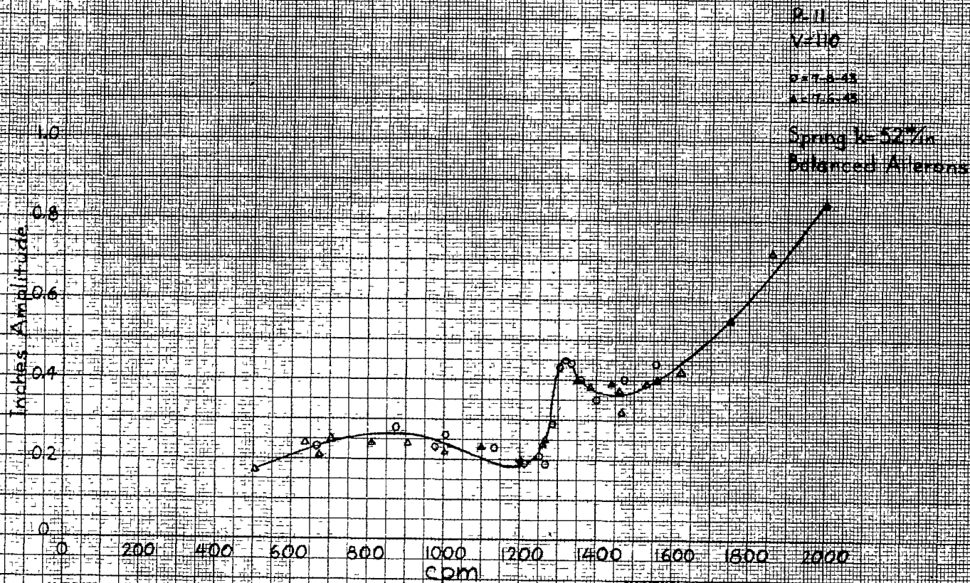
Figure 22. - Forced vibration response.
