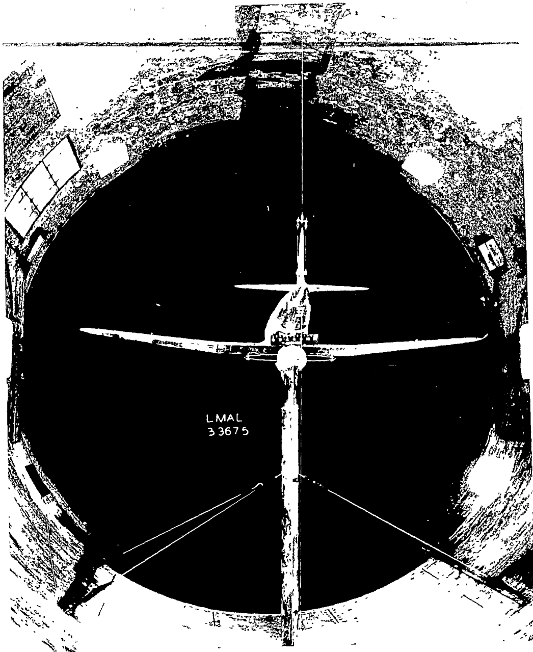
Figure 1.- Test setup.
