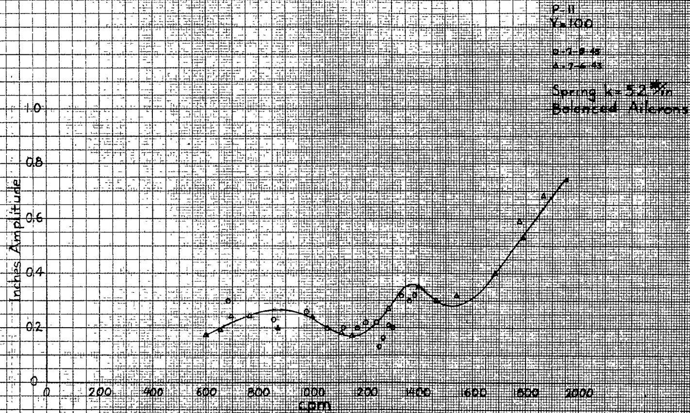
Figure 21. - Proposed vibration response.
