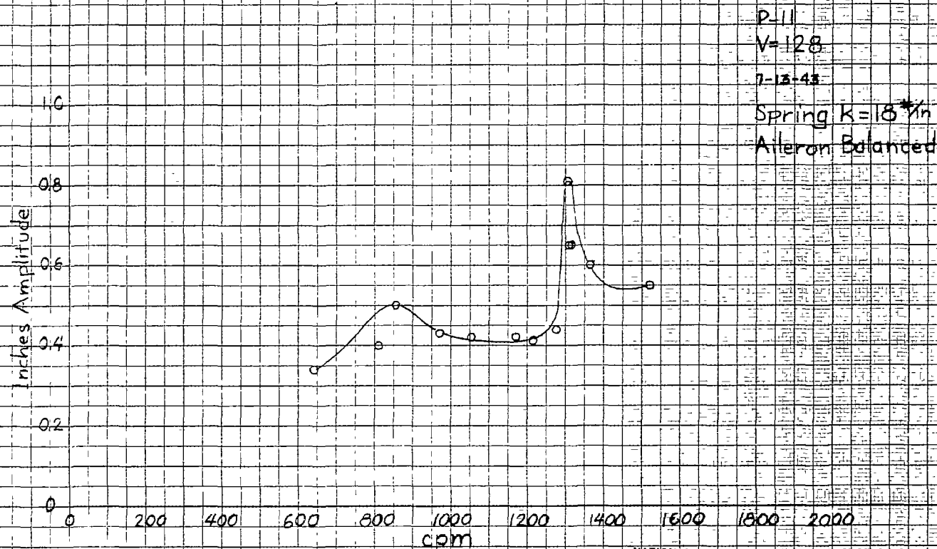
Figure 32. - Forced vibration response.
