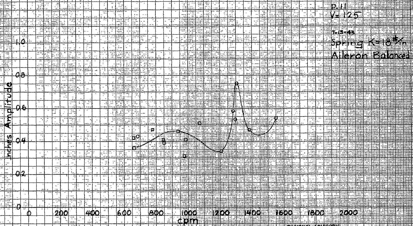
Figure 31. - Forced vibration response.
