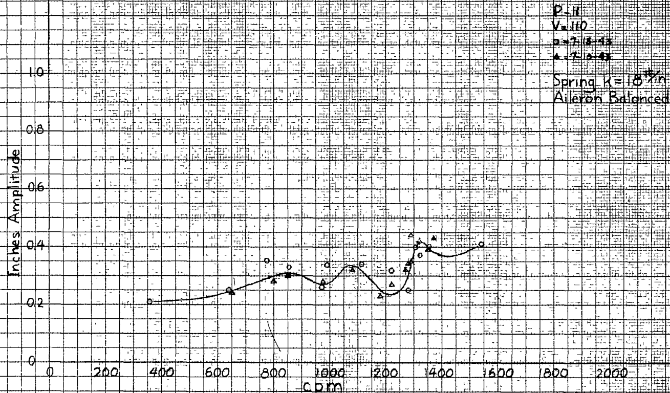
Figure 29. - Forced vibration response.
