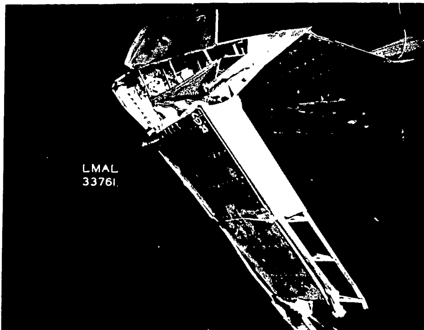
Figure 38.- The wing after flutter.
