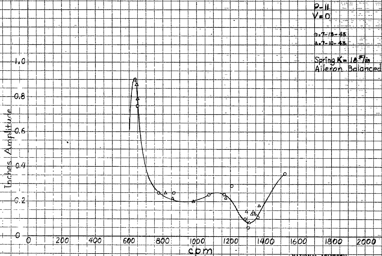
Figure 25. + Forced vibration response.
