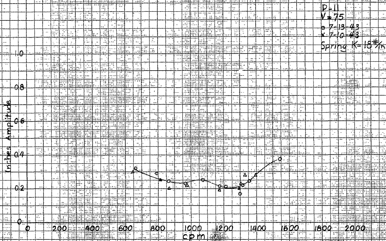
Figure 27. - Forced vibration response.
