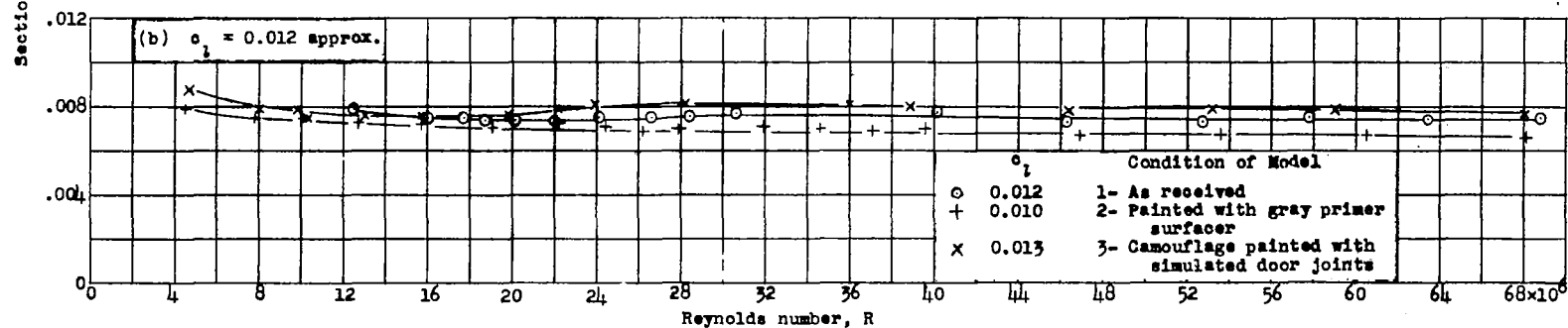
Figure 2 .- Drag scale effect of a 100-inch-chord NACA 23016 practical construction wing section submitted by Chance Vought Aircraft. Tests, TDT 430, 432, and 443.
