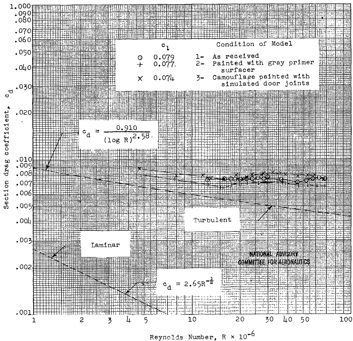
Figure 3.- Comparison of the drag coefficient of the NACA 23016 airfoil section with the skin friction of smooth flat plates.
