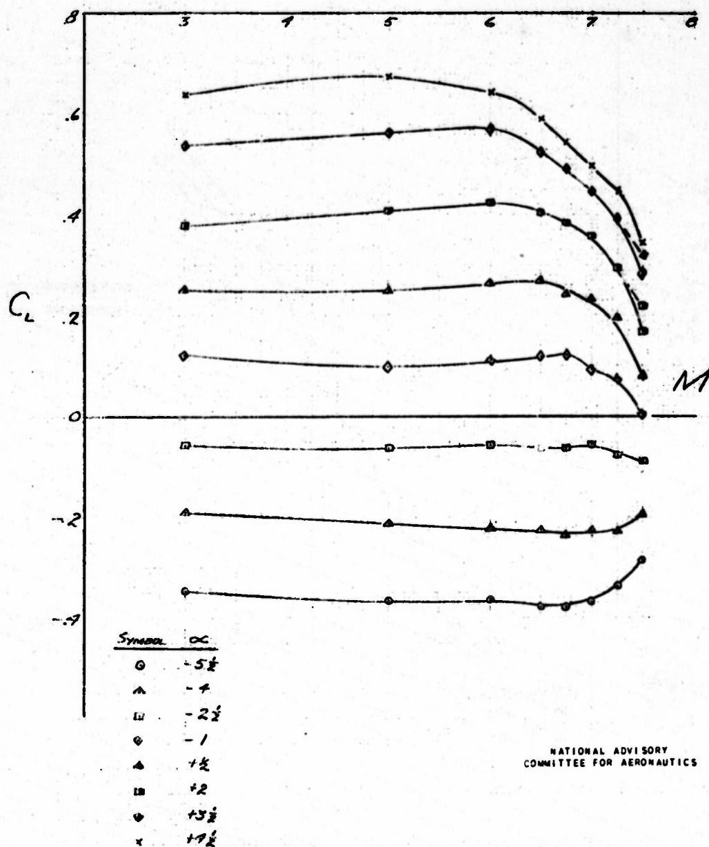
(c) Variation of C_L with Mach number at constant angles of attack. Figure 32. - Continued. Wing, booms, standard fuselage, and raised tail.
