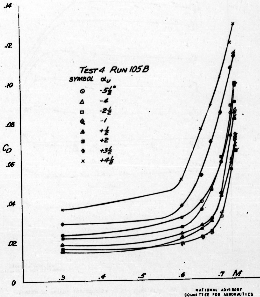
Figure 26. - Continued. Wing with revised twist, booms, long symmetrical fuselage, constant-radius fillet, and tail. Elevator at 0^\circ .
