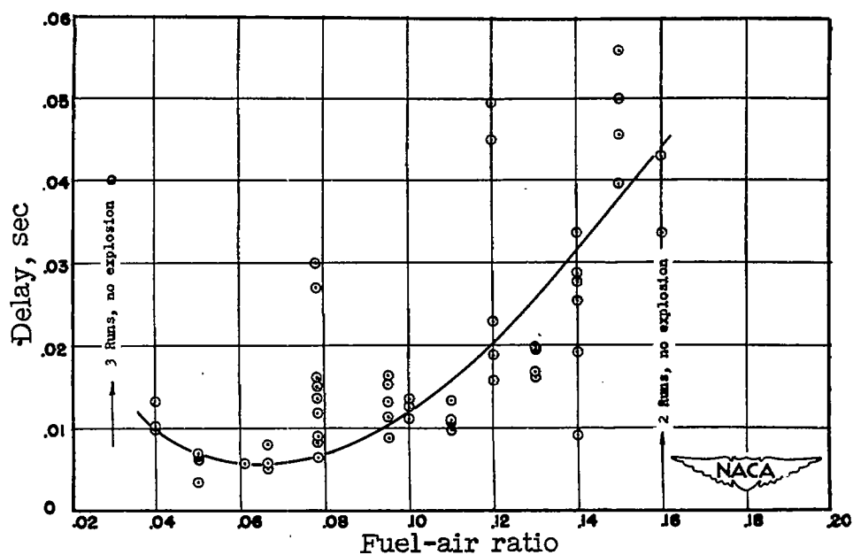
Figure 36.- Effect of fuel-air ratio on ignition delay of 100-octane gasoline. Plotted points represent actual experimental values.
