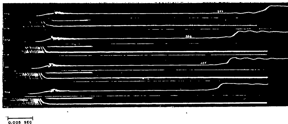
Figure 46.- Explosion records made with the M.I.T. rapid compression machine to determine the effect of saturated air on reproducibility. Fuel, isooctane; dew point of air, 68^{\circ} F, fuel-air ratio, 0.16; compression ratio, 11.7.
