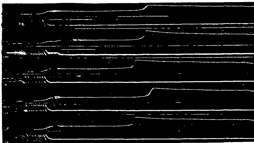
Figure 13.- Explosion records obtained with the M.I.T. rapid compression machine for 100-octane gasoline at various fuel-air ratios.
