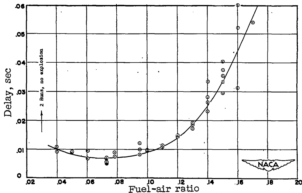
Figure 35.- Effect of fuel-air ratio on ignition delay of isooctane. Plotted points represent actual experimental values.
