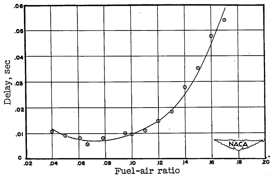
Figure 4.- Effect of fuel-air ratio on ignition delay of isooctane. Plotted points represent average values.
