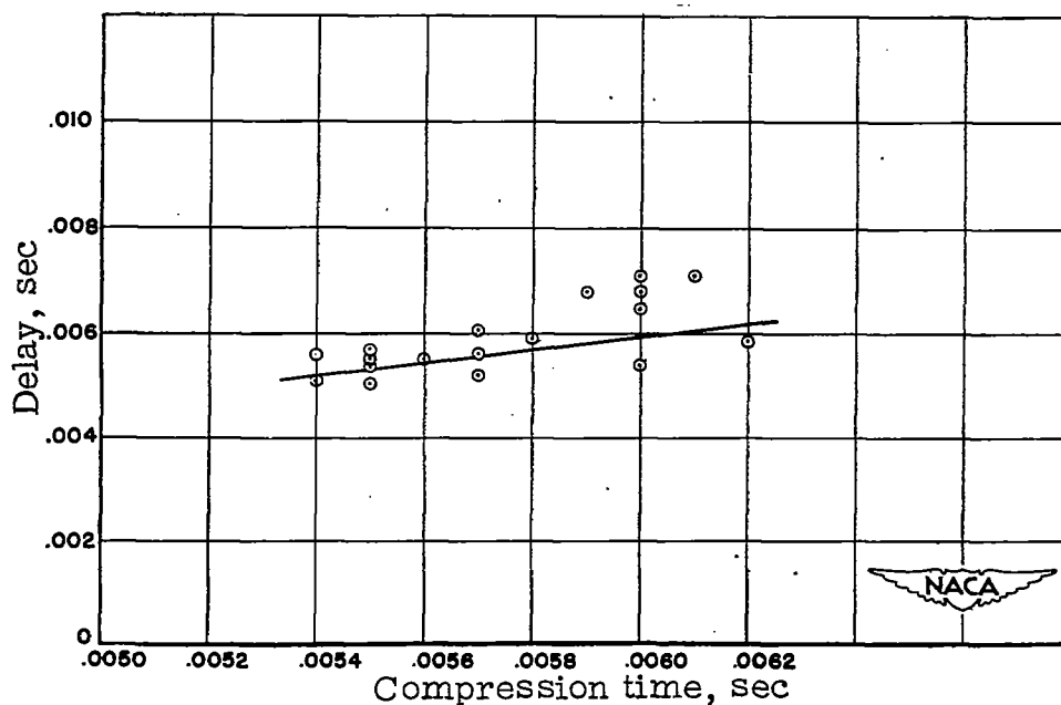
Figure 34.- Effect of compression time on ignition delay of isooctane. . Fuel-air ratio, 0.067; compression ratio, 11.7.
