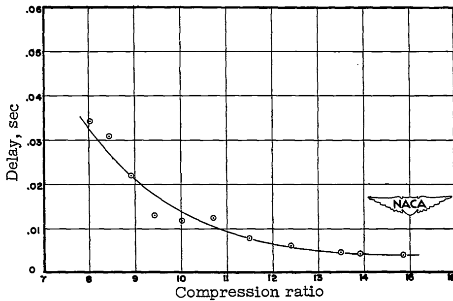
Figure 9.- Effect of compression ratio on ignition delay of isooctane. Plotted points represent average values.
