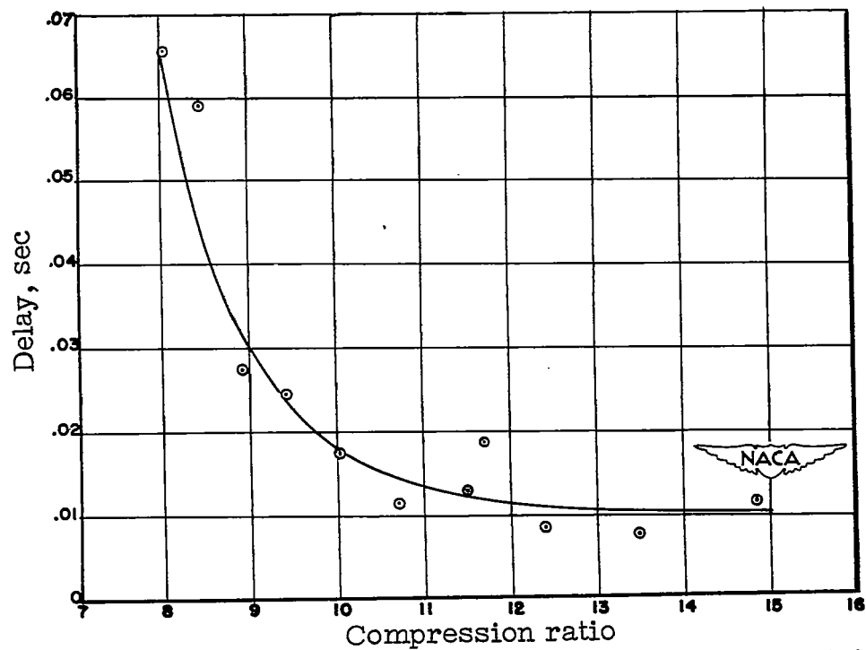
Figure 25.- Effect of compression ratio on ignition delay of triptane. Plotted points represent average values.
