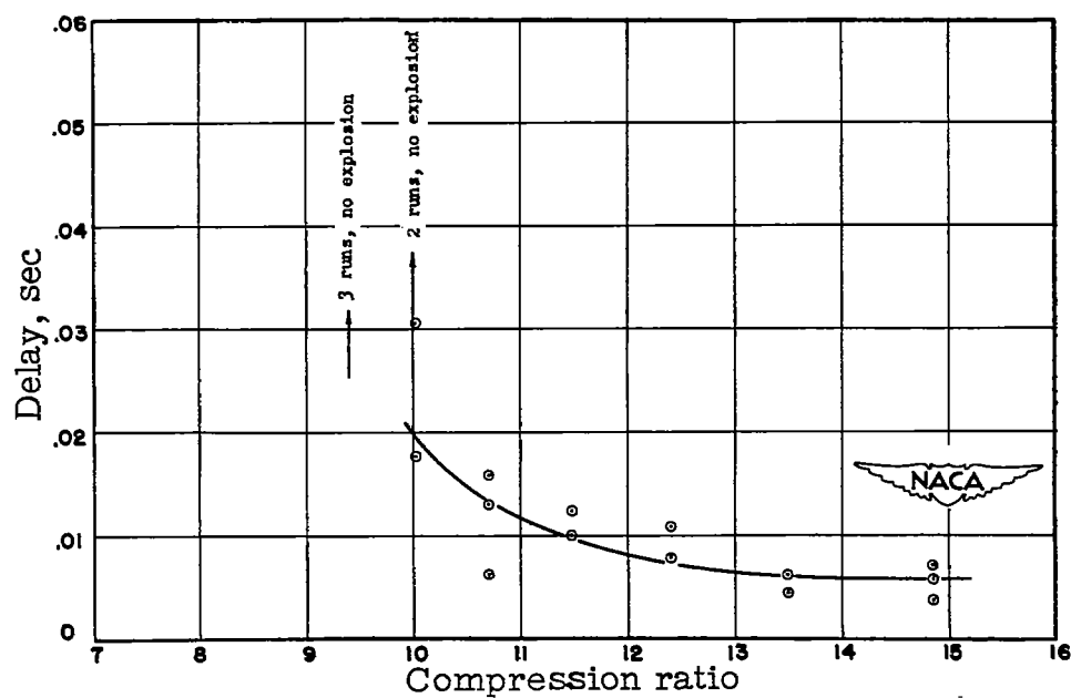
Figure 42.- Effect of compression ratio on ignition delay of benzene. Plotted points represent actual experimental values.
