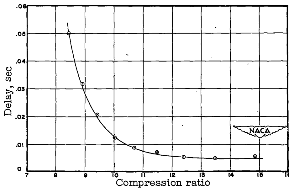
Figure 19.- Effect of compression ratio on ignition delay of 100-octane gasoline. Plotted points represent average values.
