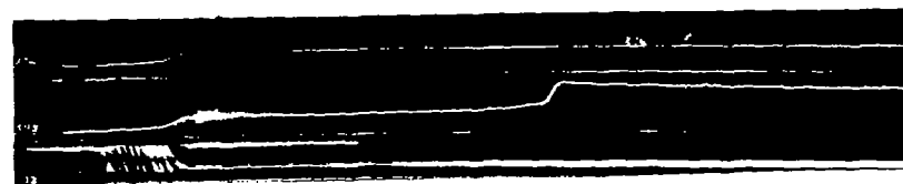
Figure 21.- Explosion records obtained with the M.I.T. rapid compression machine for triptane at various fuel-air ratios.
