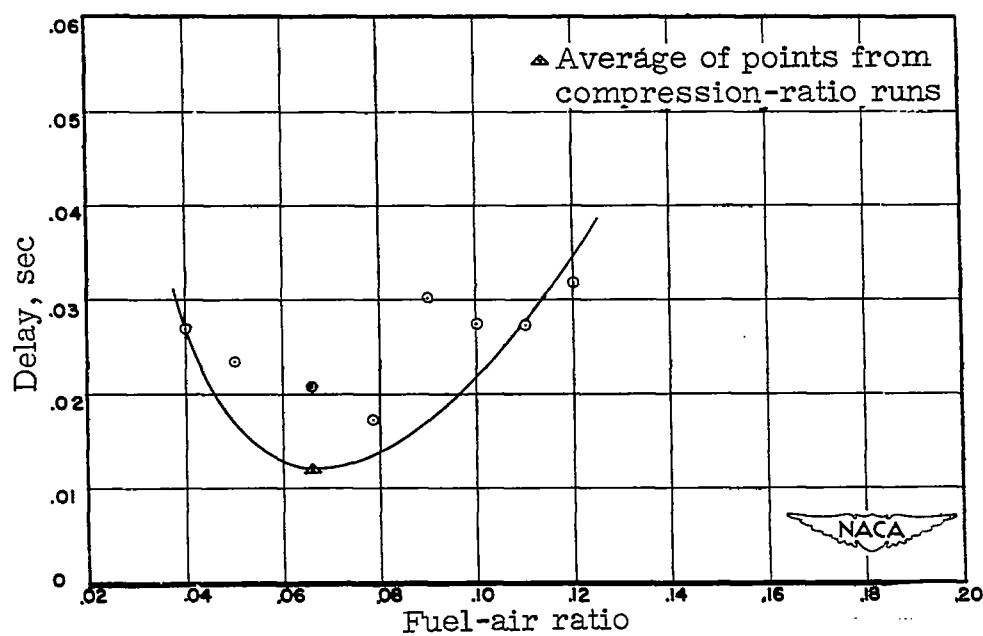
Figure 22.- Effect of fuel-air ratio on ignition delay of triptane. Plotted points represent average values.
