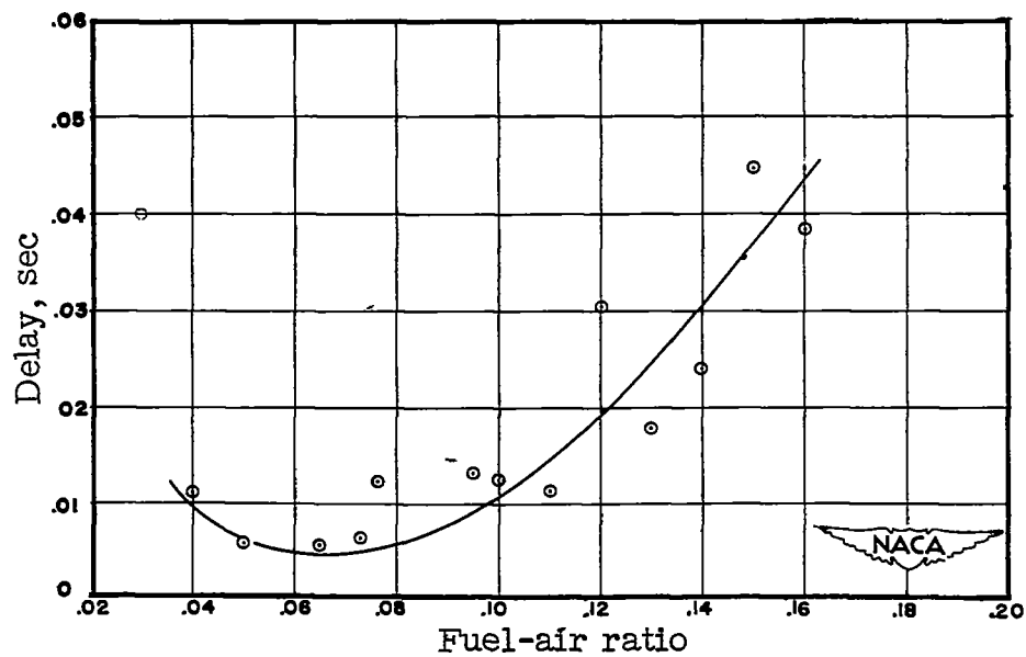
Figure 15.- Effect of fuel-air ratio on ignition delay of 100-octane gasoline. Plotted points represent average values.
