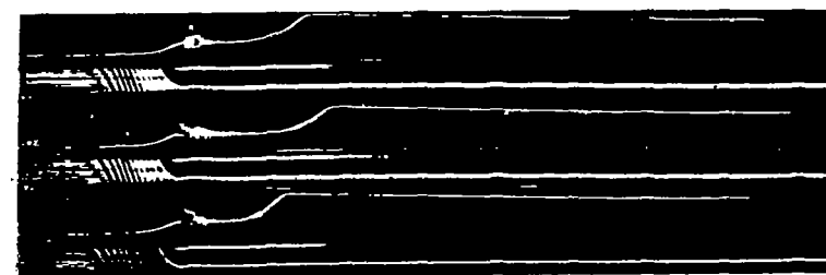
Figure 26.- Explosion records obtained with the M.I.T. rapid compression machine for benzene at various fuel-air ratios.
