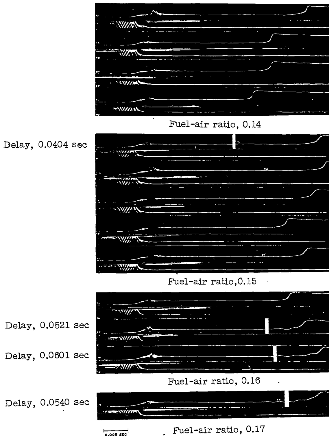
Figure 3.- Explosion records obtained with M.I.T. rapid compression machine for isooctane at various fuel-air ratios.
