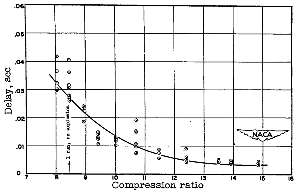
Figure 39.- Effect of compression ratio on ignition delay of isooctane. Plotted points represent actual experimental values.
