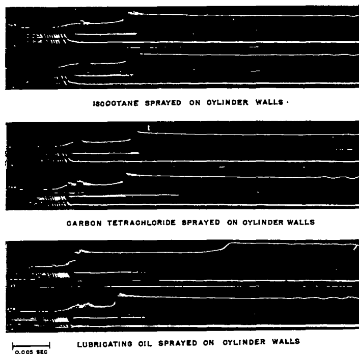
Figure 48.- Explosion records made with M.I.T. rapid compression machine to determine the effect on reproducibility of spraying the combustion cylinder walls with various fluids. Fuel, isooctane; fuel-air ratio, 0.067; compression ratio, 11.7.
