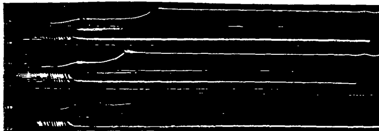
Figure 23.- Explosion records obtained with the M.I.T. rapid compression machine for triptane at various compression ratios.
