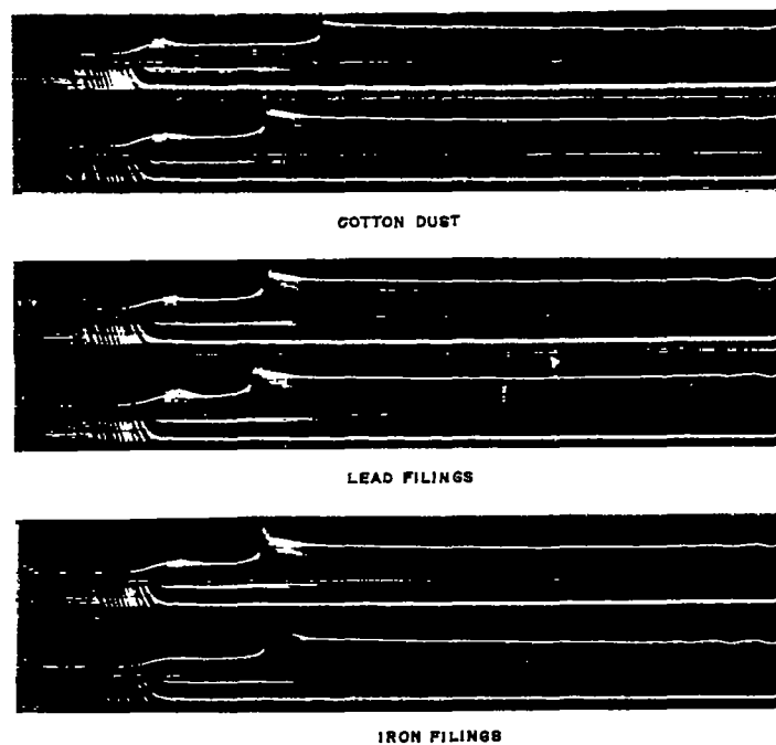
Figure 47.- Explosion records made with M.I.T. rapid compression machine to determine the effect of dust particles on reproducibility. Fuel, isooctane; fuel-air ratio, 0.067; compression ratio, 11.7.
