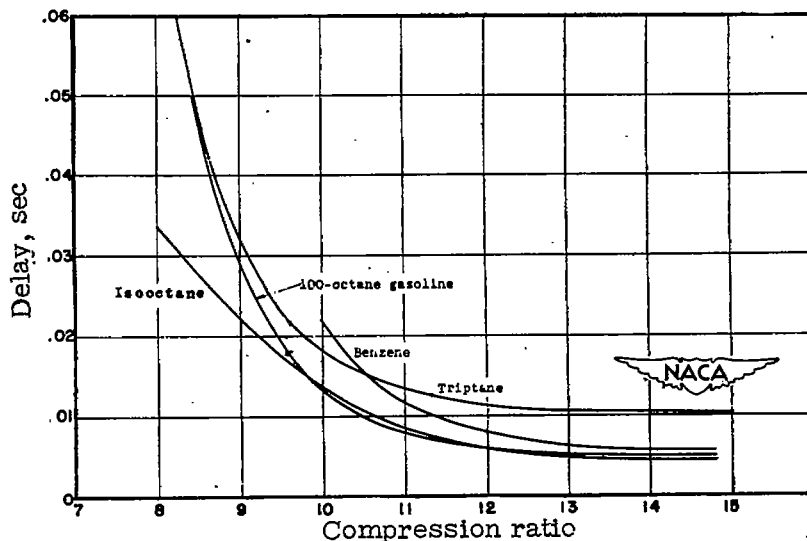
Figure 33.- Comparison of isooctane, 100-octane gasoline, triptane, and benzene with respect to variation in ignition delay with compression ratio. Test conditions: fuel-air ratio, chemically correct; initial pressure, 14.7 pounds per square inch absolute; initial temperature, 149° F; compression time, 0.006 second.
