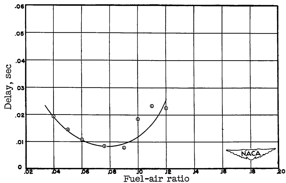
Figure 28.- Effect of fuel-air ratio on ignition delay of benzene. Plotted points represent average values.
