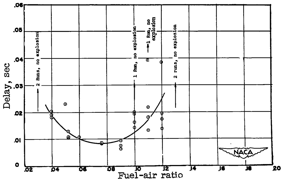
Figure 38.- Effect of fuel-air ratio on ignition delay of benzene. Plotted points represent actual experimental values.
