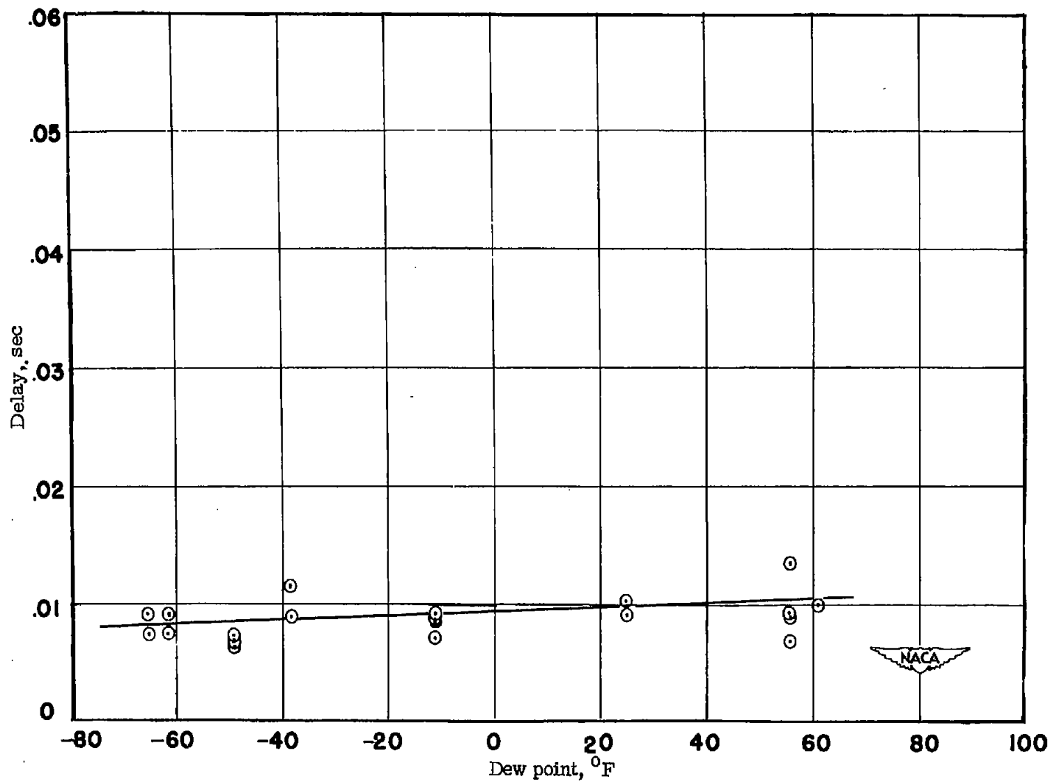
Figure 45.- Effect of air dew point on ignition delay of isooctane-air mixtures.
