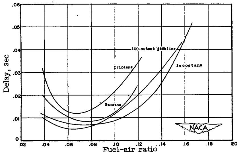
Figure 32.- Comparison of isooctane, 100-octane gasoline, triptane, and benzene with respect to variation in ignition delay with fuel-air ratio. Test conditions: compression ratio, 11.7; initial pressure, 14.7 pounds per square inch absolute; initial temperature, 149° F; compression time, approximately 0.006 second.
