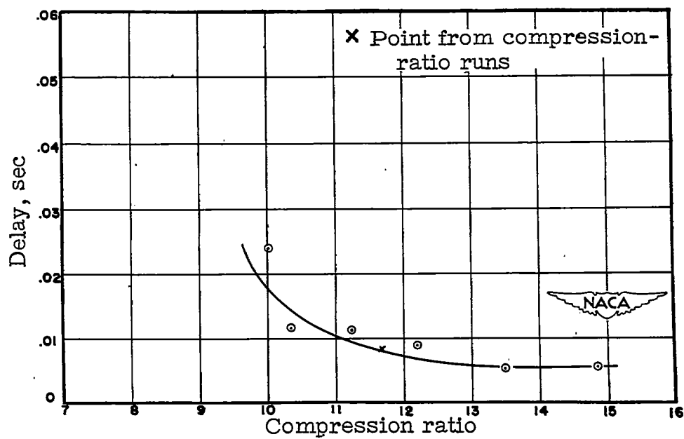
Figure 31.- The effect of compression ratio on ignition delay of benzene Plotted points are average values.
