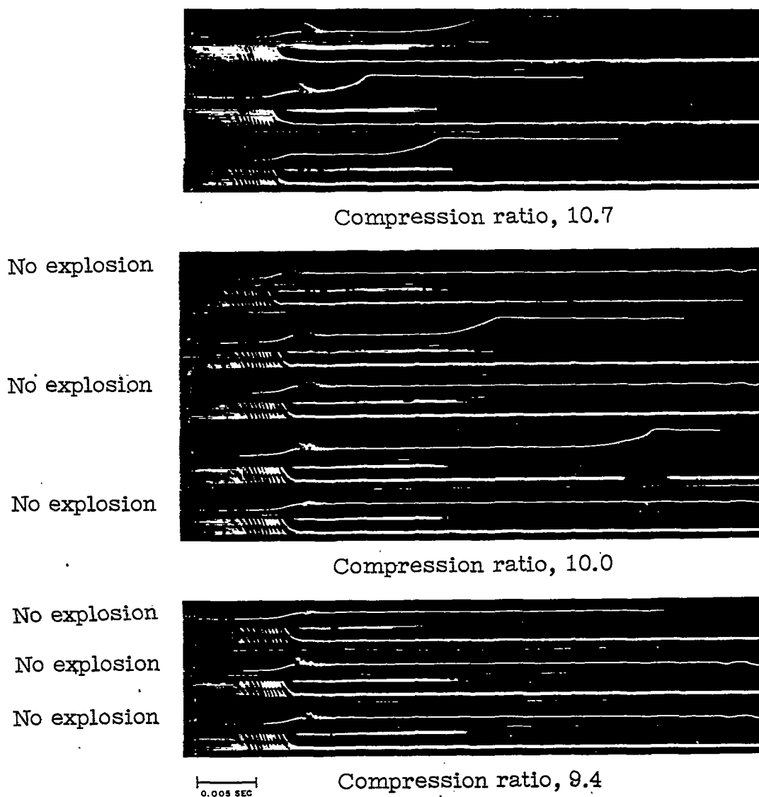
Figure 30.- Explosion records obtained with M.I.T. rapid compression machine for benzene at various compression ratios.
