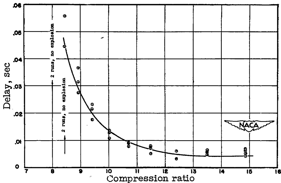
Figure 40.- Effect of compression ratio on ignition delay of 100-octane gasoline. Plotted points represent actual experimental values.
