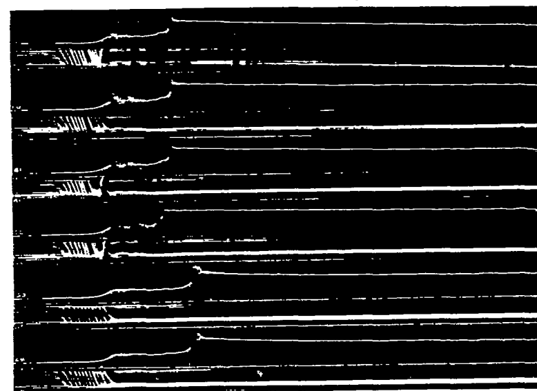
Figure 1.- Explosion records obtained with M.I.T. rapid compression machine for isooctane at various fuel-air ratios.
