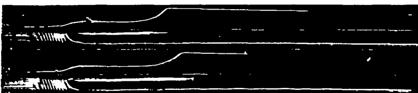
Figure 29.- Explosion records obtained with M.I.T. rapid compression machine for benzene at various compression ratios.
