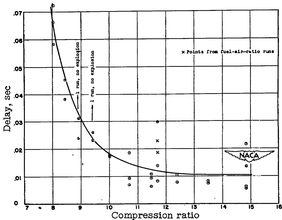
Figure 41.- Effect of compression ratio on ignition delay of triptane. Plotted points represent actual experimental values.
