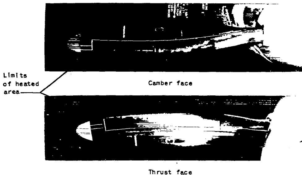
(a) Propeller speed, 675 rpm; ambient-air temperature, 2^{\circ} F; heat-on time, 24 seconds; cycle time, 96 seconds.
