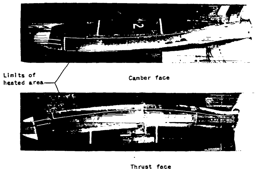
(b) Ambient-air temperature, 2^{\circ}\text{F} ; heat-on time, 24 seconds; cycle time, 96 seconds.
