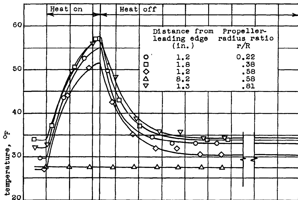
(a) Propeller speed, 675 rpm.
