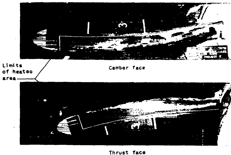
(b) Propeller speed, 675 rpm; heat-on time, 24 seconds; cycle time, 96 seconds.
