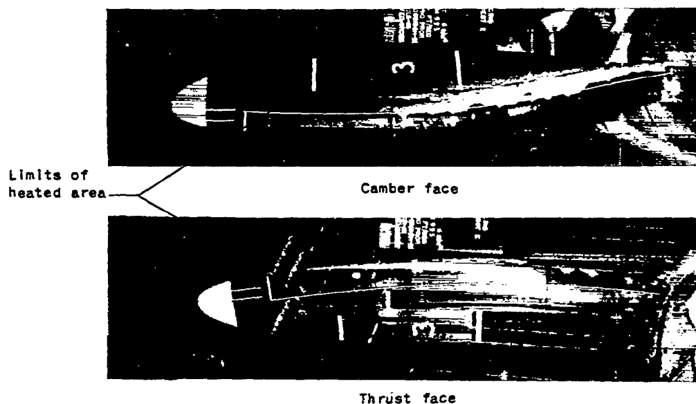
(b) Ambient-air temperature, 11^{\circ}\text{F} ; heat-on time, 24 seconds; cycle time, 96 seconds.
