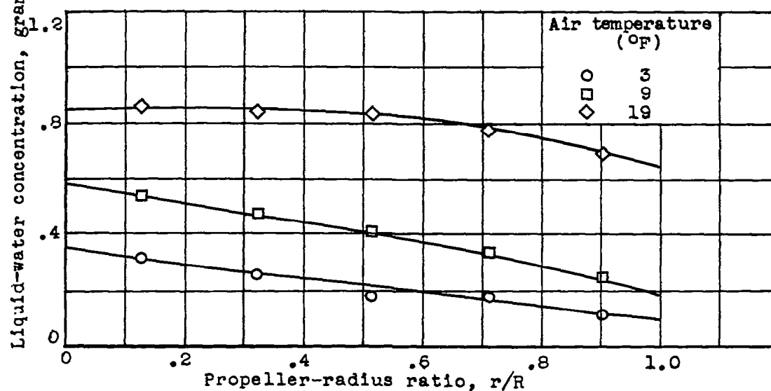
(b) Radial distribution of liquid-water concentration.
