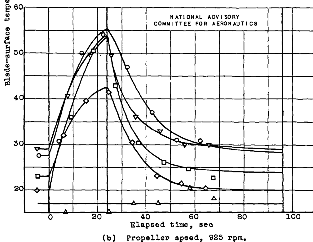
Figure 28. - Variation of blade-surface temperature with time on thrust face during cyclic de-icing. Heating pattern 9; ambient-air temperature, 2^{\circ}\text{F} ; heat-on time, 24 seconds; cycle time, 96 seconds.
