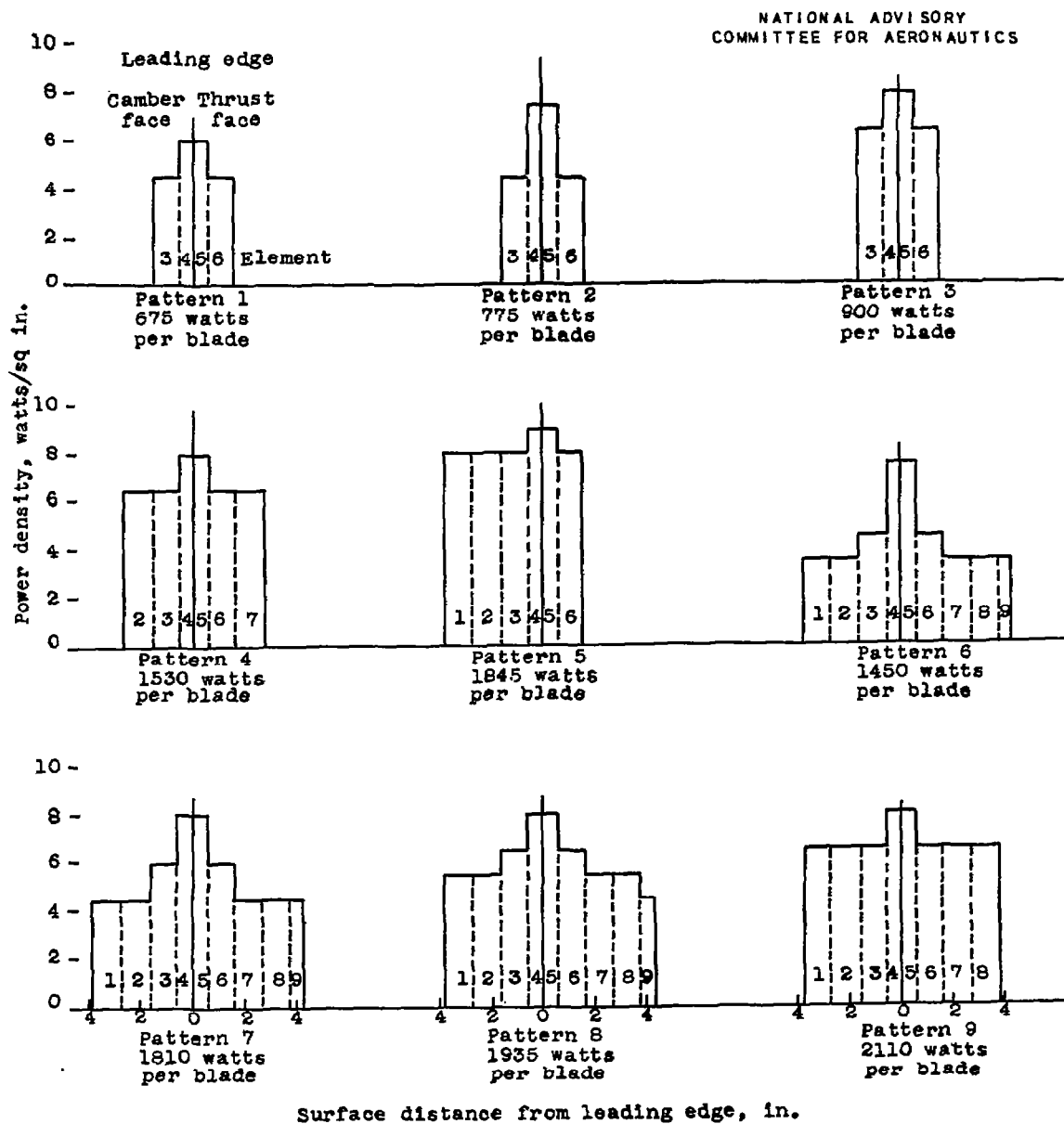
Figure 9. - Chordal-heating power distribution.
