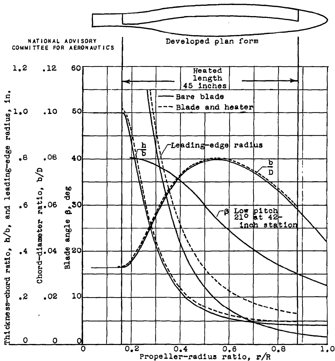
Figure 2. - Blade-form characteristics for propeller blade with external rubber-clad blade heater.
