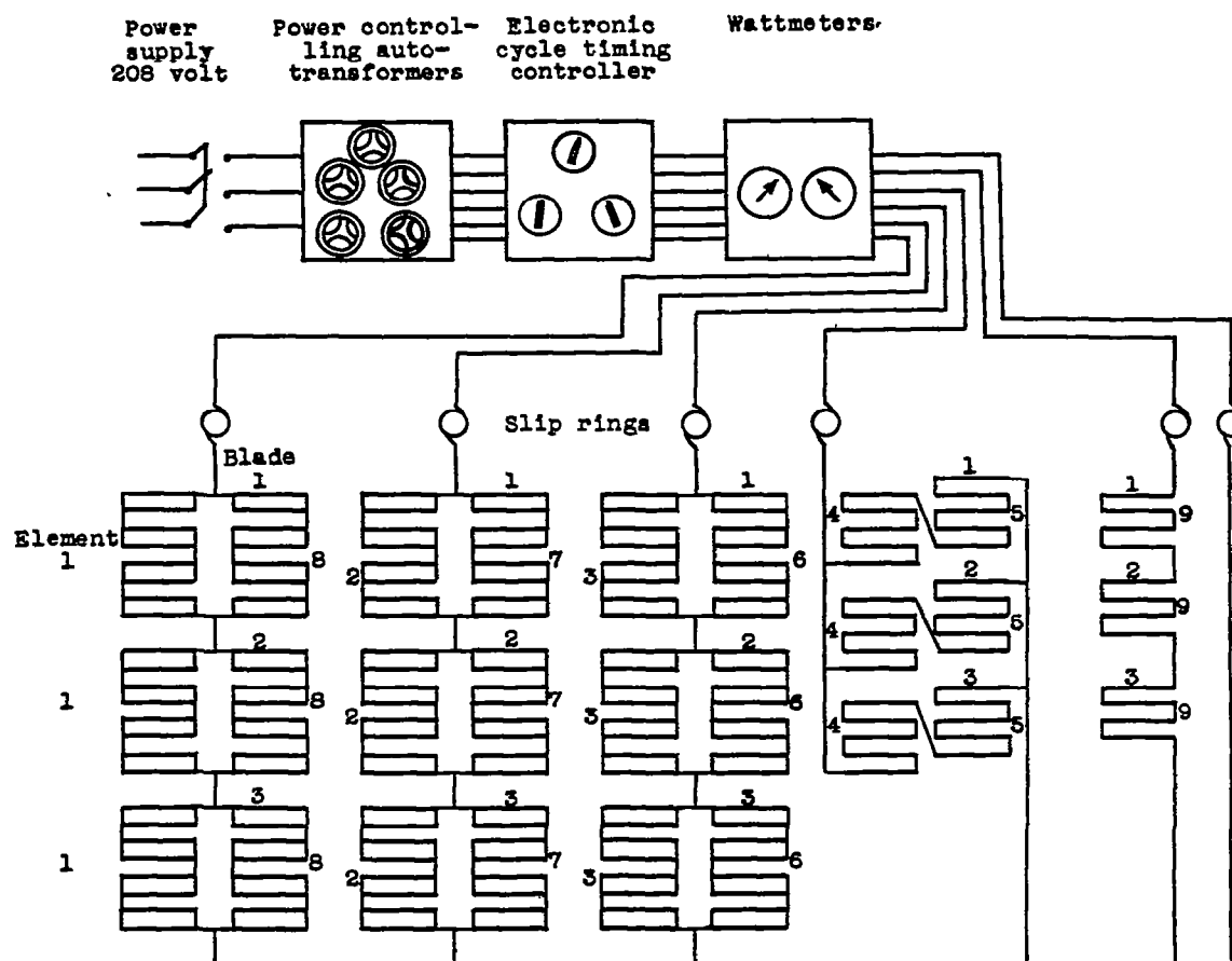
Figure 5. - Typical blade-heating circuit.
