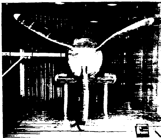
(b) Setup in tunnel.
