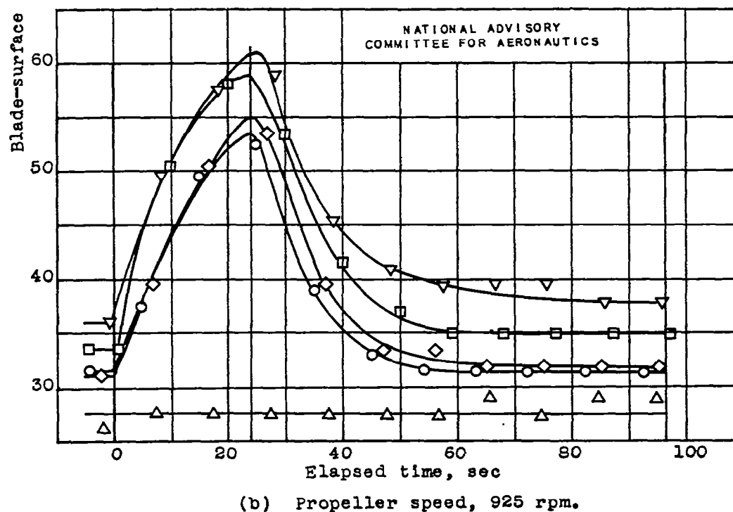
Figure 30. - Variation of blade-surface temperature with time on thrust face during cyclic de-icing. Heating pattern 9; ambient-air temperature, 11^{\circ}\text{F} ; heat-on time, 24 seconds; cycle time, 96 seconds.
