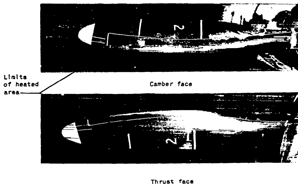
(d) Ambient-air temperature, 11^{\circ} F; heat-on time, 23 seconds; cycle time, 184 seconds.
