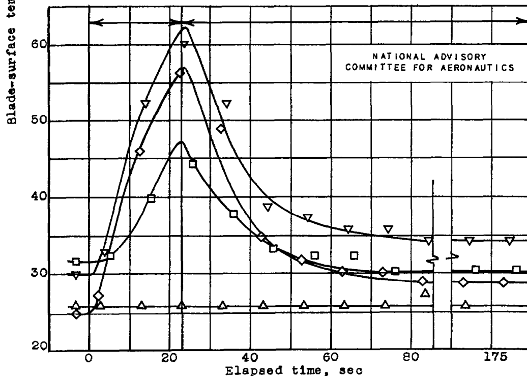
(b) Heating pattern 5; propeller speed, 925 rpm; heat-on time, 23 seconds; cycle time, 184 seconds.
