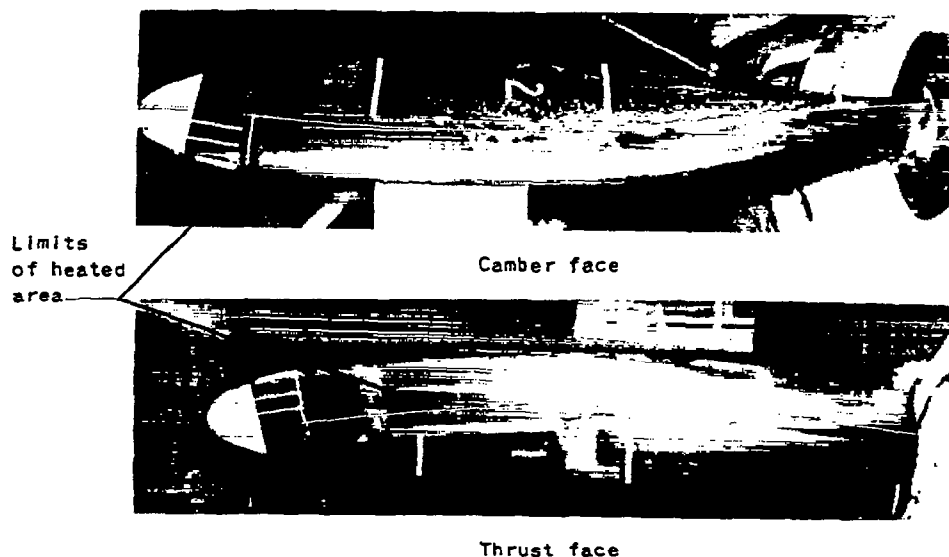
(e) Propeller speed, 675 rpm; ambient-air temperature, 11^{\circ} F; heat-on time, 24 seconds; cycle time, 96 seconds.
