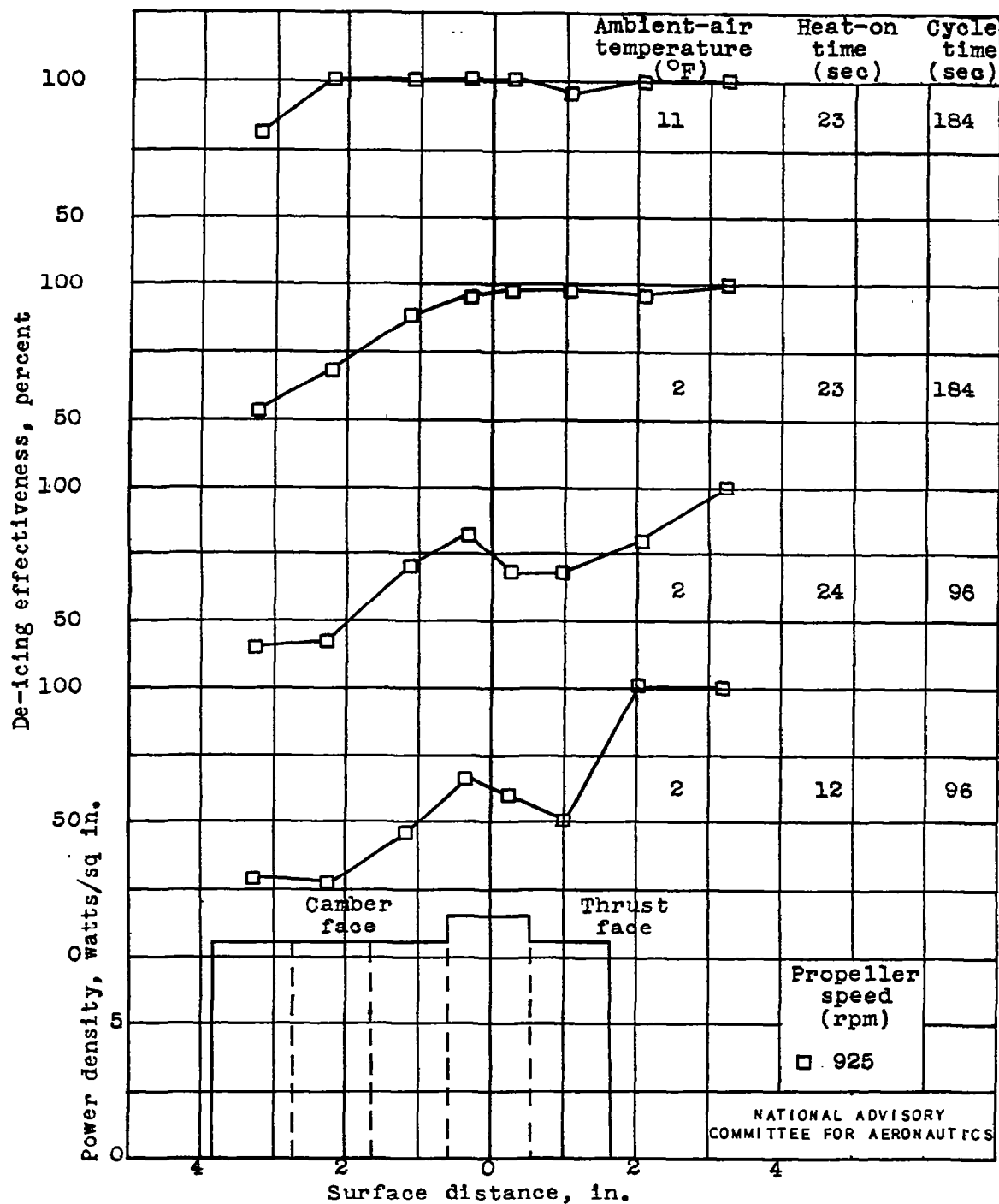
(e) Heating pattern 5.
