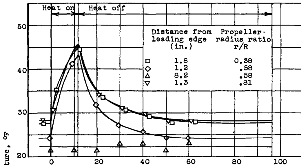
(a) Heating pattern 8; propeller speed, 675 rpm; heat-on time, 12 seconds; cycle time, 96 seconds.
