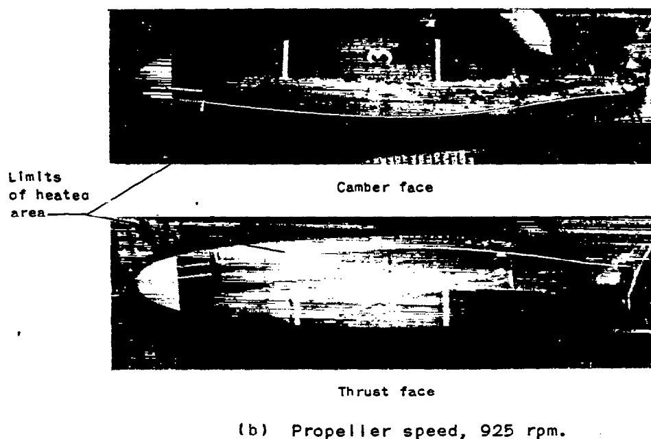
Figure 16. - Views of residual ice after cyclic de-icing with heating pattern 1. Ambient-air temperature, 21^{\circ}\text{F} ; heat-on time, 12 seconds; cycle time, 96 seconds.
