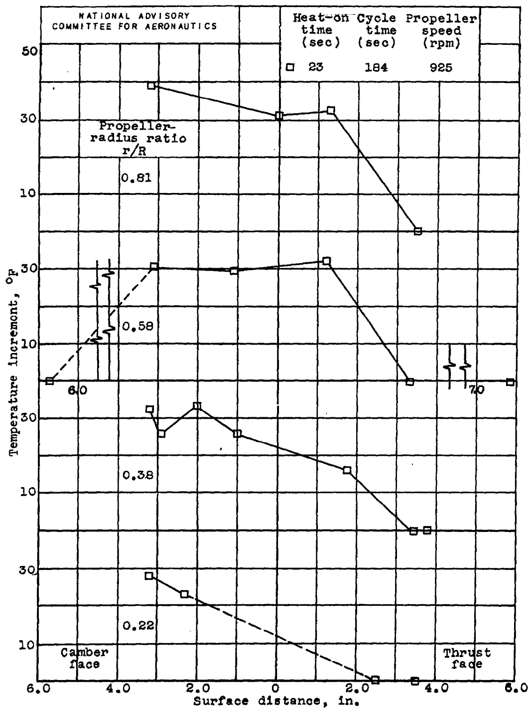
Figure 32. - Continued. Variation of blade-surface temperature increment with chordwise surface distance.
