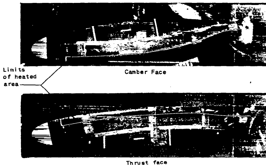
(d) Propeller speed, 925 rpm; ambient-air temperature, 21^{\circ} F; heat-on time, 12 seconds; cycle time, 96 seconds.
