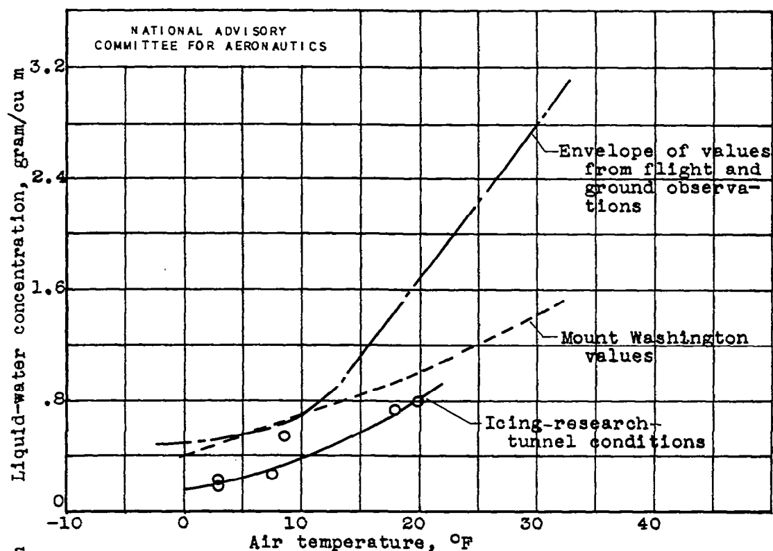
(a) Variation of liquid-water concentration with air temperature.
