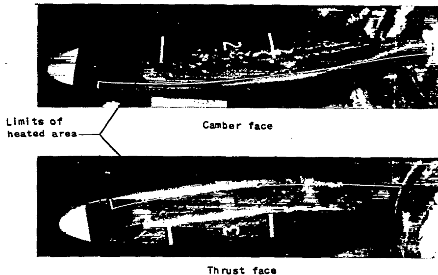
(a) Propeller speed, 675 rpm; ambient-air temperature, 21^{\circ} F; heat-on time, 12 seconds; cycle time, 48 seconds.
