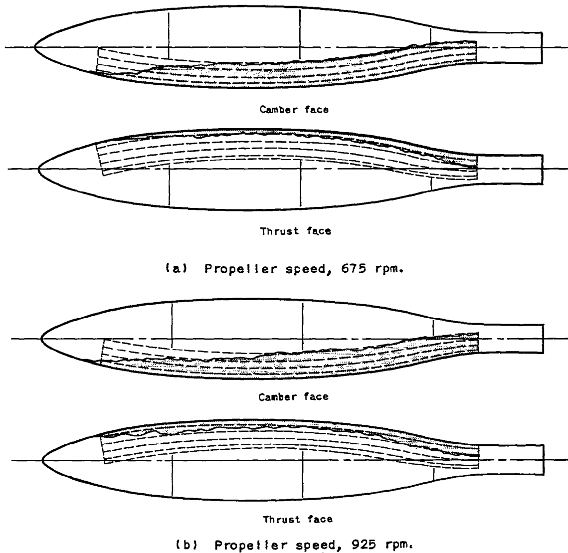
Figure 12. - Typical ice coverage obtained on unheated blade at ambient-air temperature of 11° F and liquid-water concentration of 0.4 gram per cubic meter.
