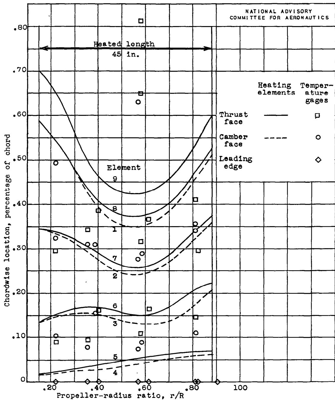
Figure 10. - Radial variation of chordwise-location heater elements and temperature gages.
