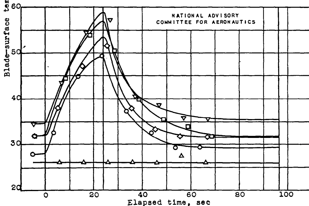
(b) Propeller speed, 925 rpm.
