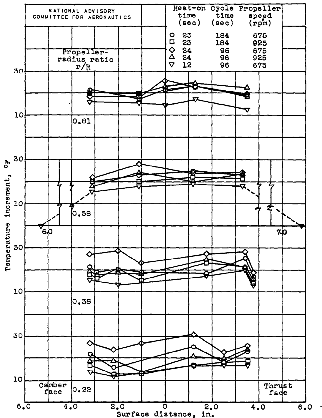
(c) Heating pattern 8; ambient-air temperature, 11° F.
