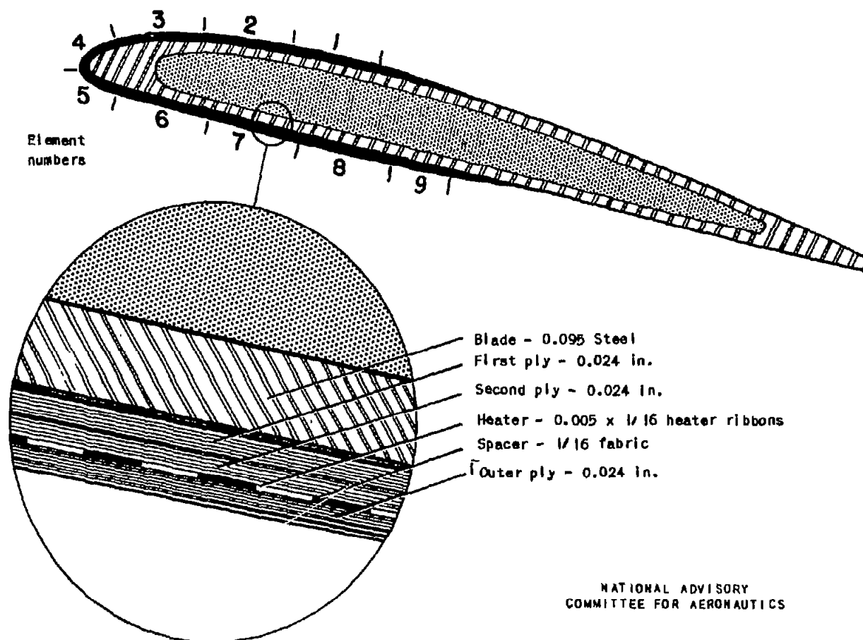
Figure 3. - Details of construction of electrical, external, rubber-clad propeller-blade heaters.
