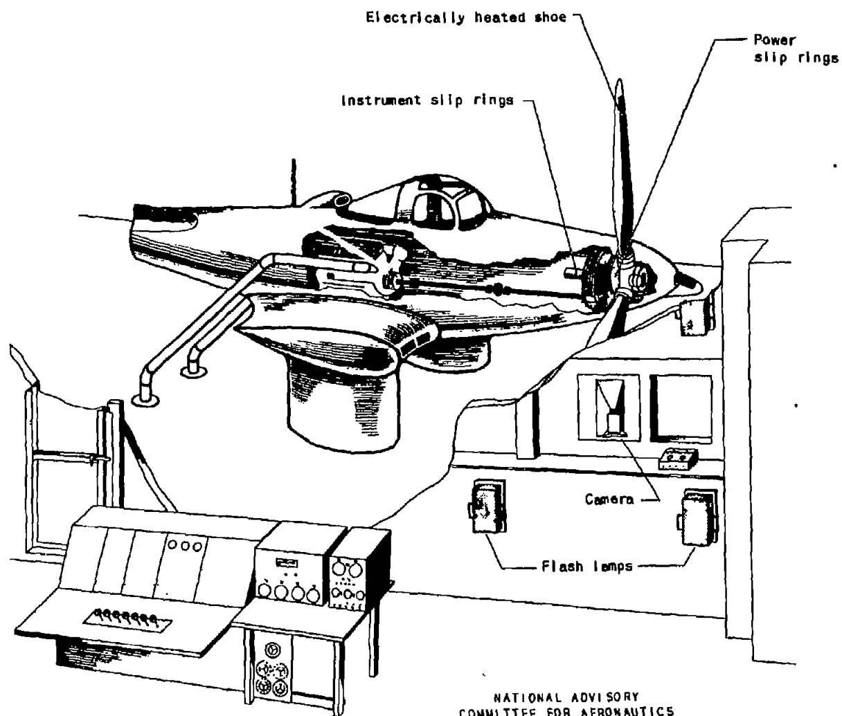
(c) Details of installation.
