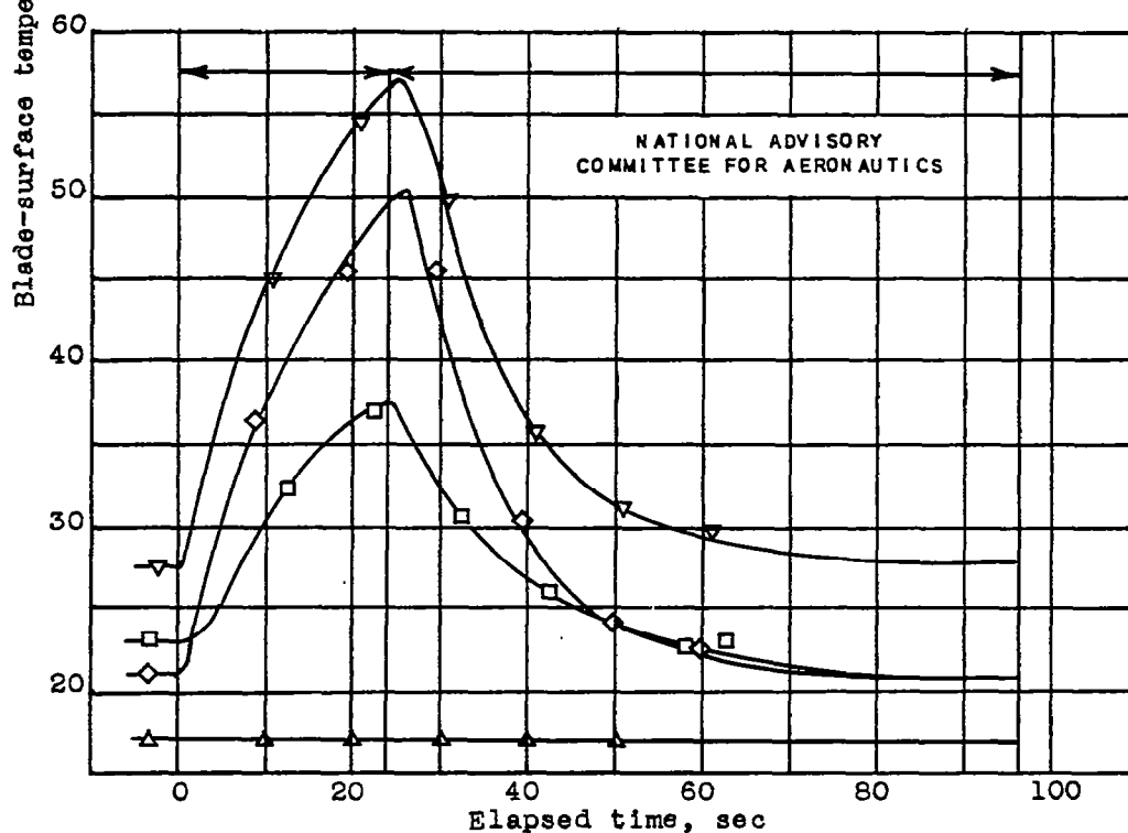
Figure 24. - Variation of blade-surface temperature with time on thrust face during cyclic de-icing. Heating pattern 5; propeller speed, 925 rpm; ambient-air temperature, 2° F; cycle time, 96 seconds.
