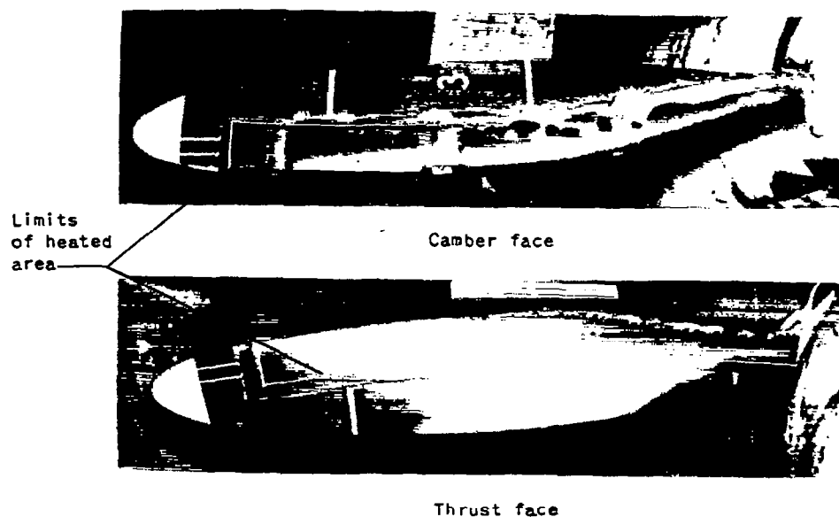
(f) Propeller speed, 925 rpm; ambient-air temperature, 11^{\circ} F; heat-on time, 24 seconds; cycle time, 96 seconds.
