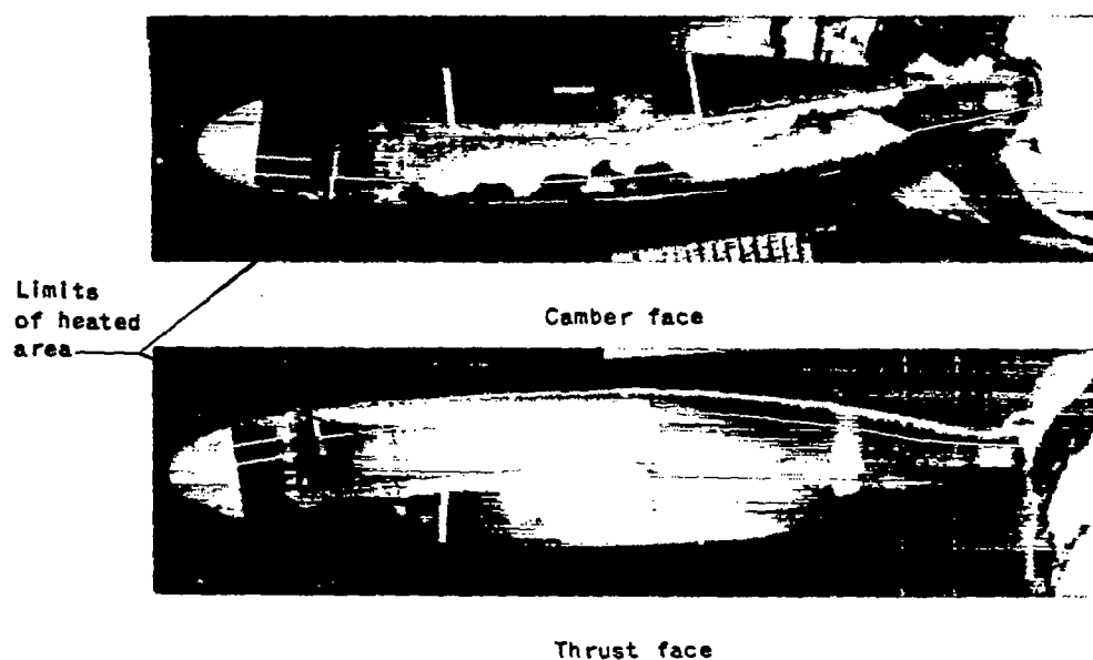
(b) Propeller speed, 925 rpm.
