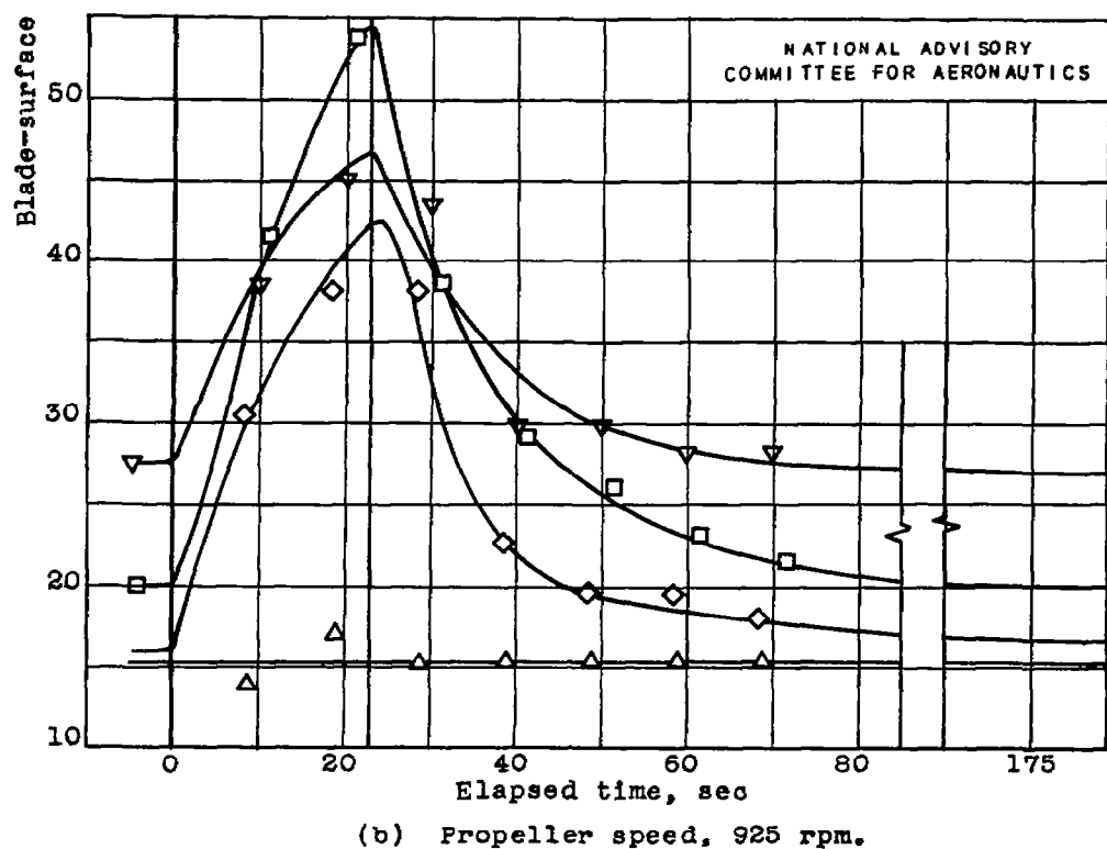
Figure 29. - Variation of blade-surface temperature with time on thrust face during cyclic de-icing. Heating pattern 9; ambient-air temperature, 2° F; heat-on time, 23 seconds; cycle time, 184 seconds.
