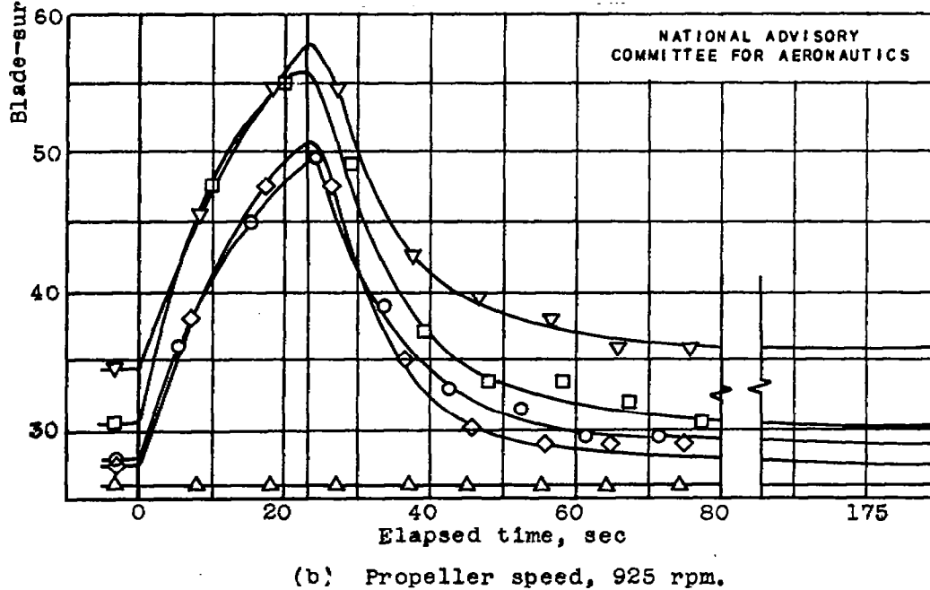
Figure 31. - Variation of blade-surface temperature with time on thrust face during cyclic de-icing. Heating pattern 9; ambient-air temperature, 11° F; heat-on time, 23 seconds; cycle time, 184 seconds.
