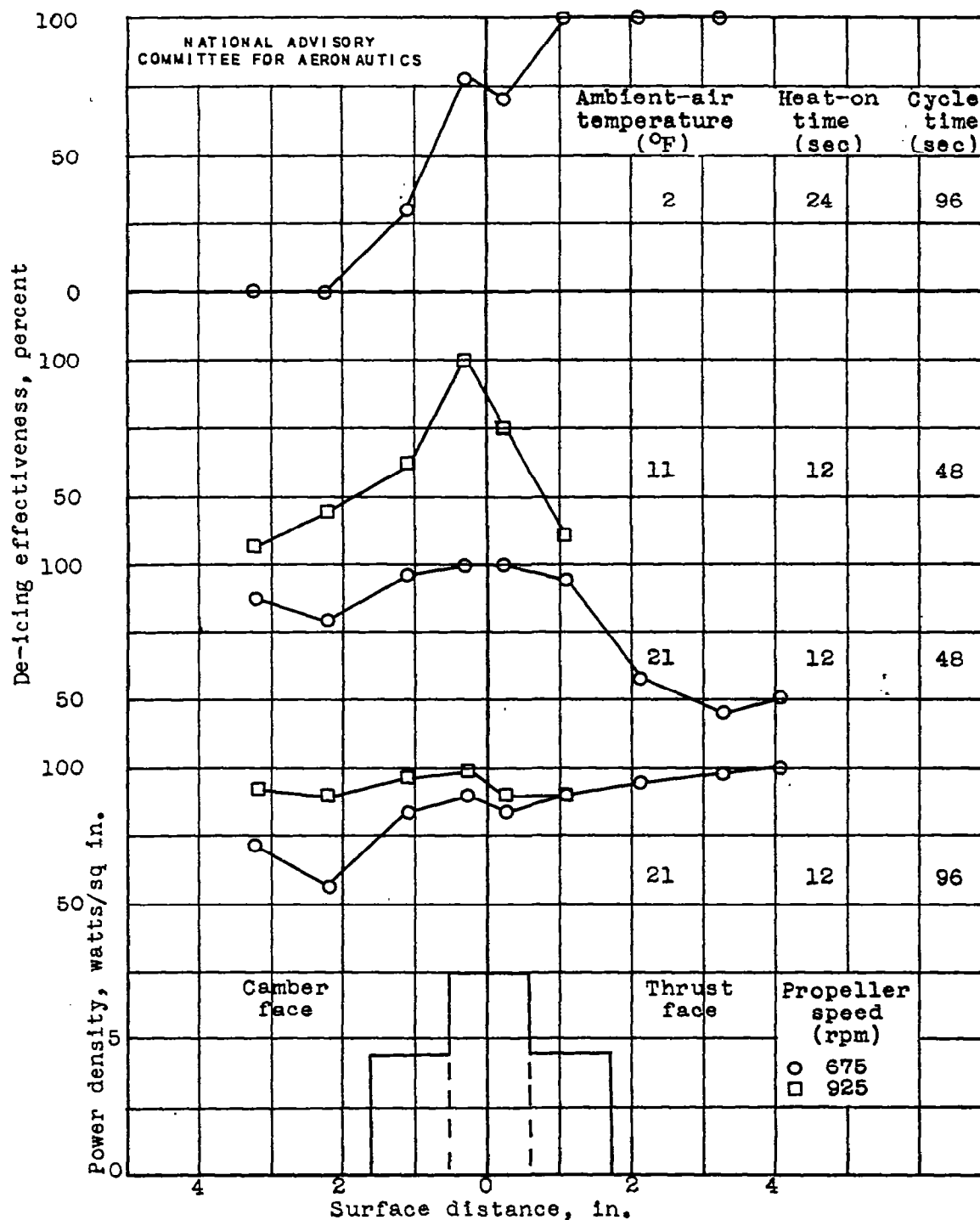
(c) Heating pattern 2.
