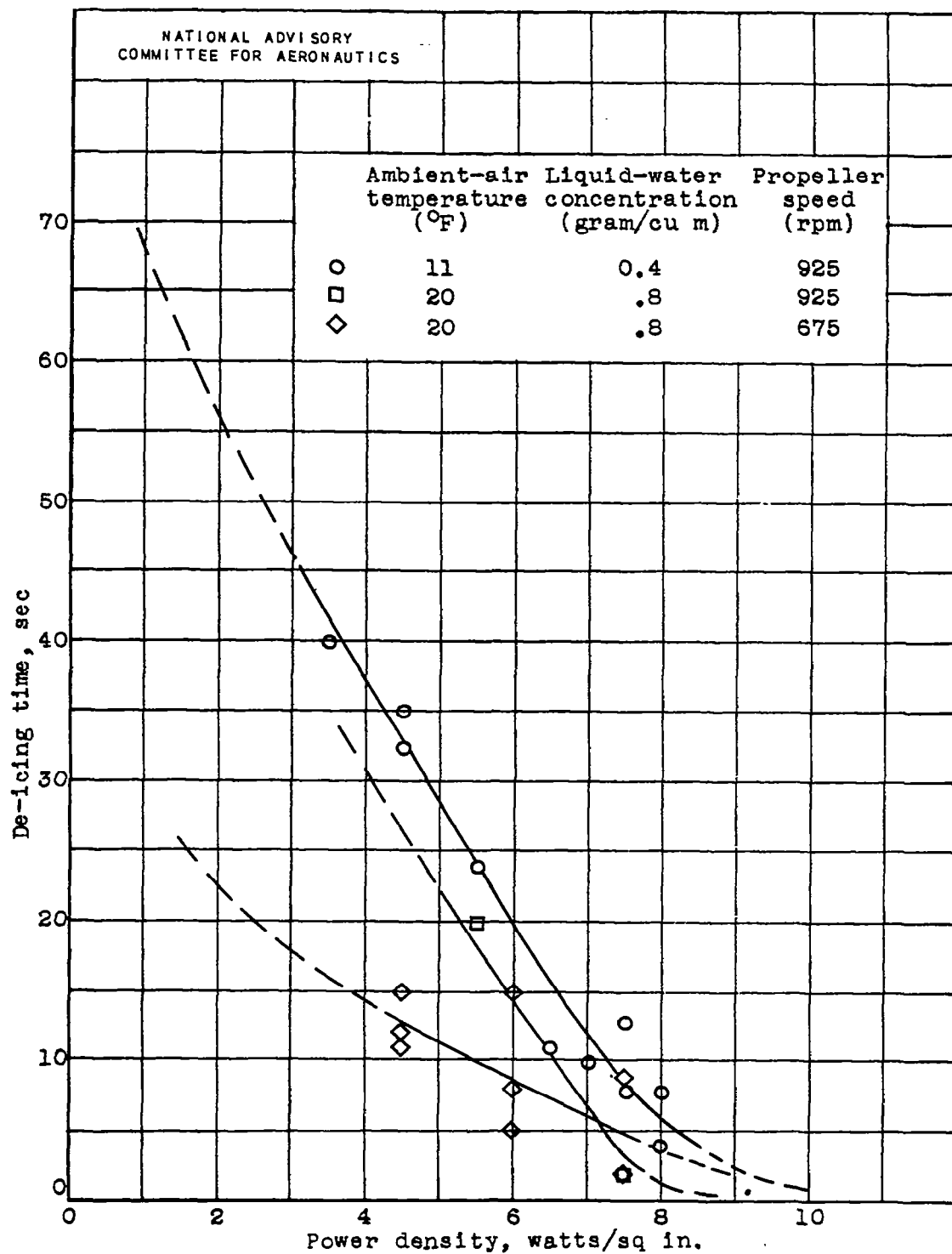
Figure 14. - Variation of de-icing time with power density at several icing and propeller-speed conditions.
