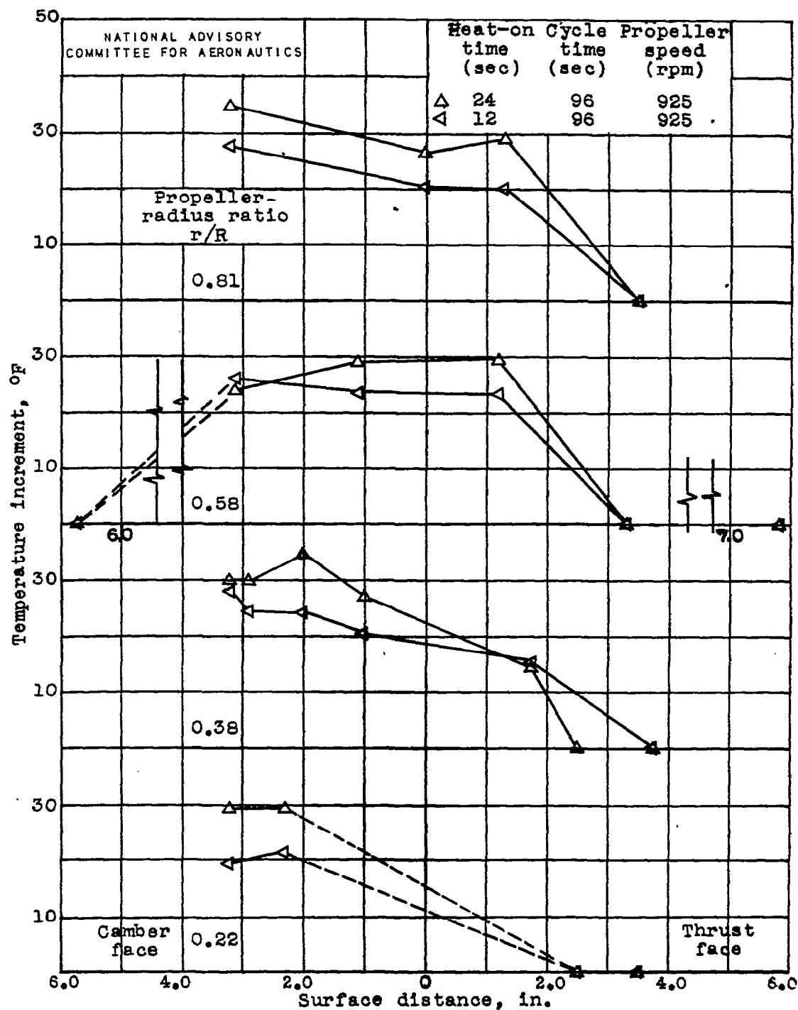
(a) Heating pattern 5; ambient-air temperature, 20° F.
