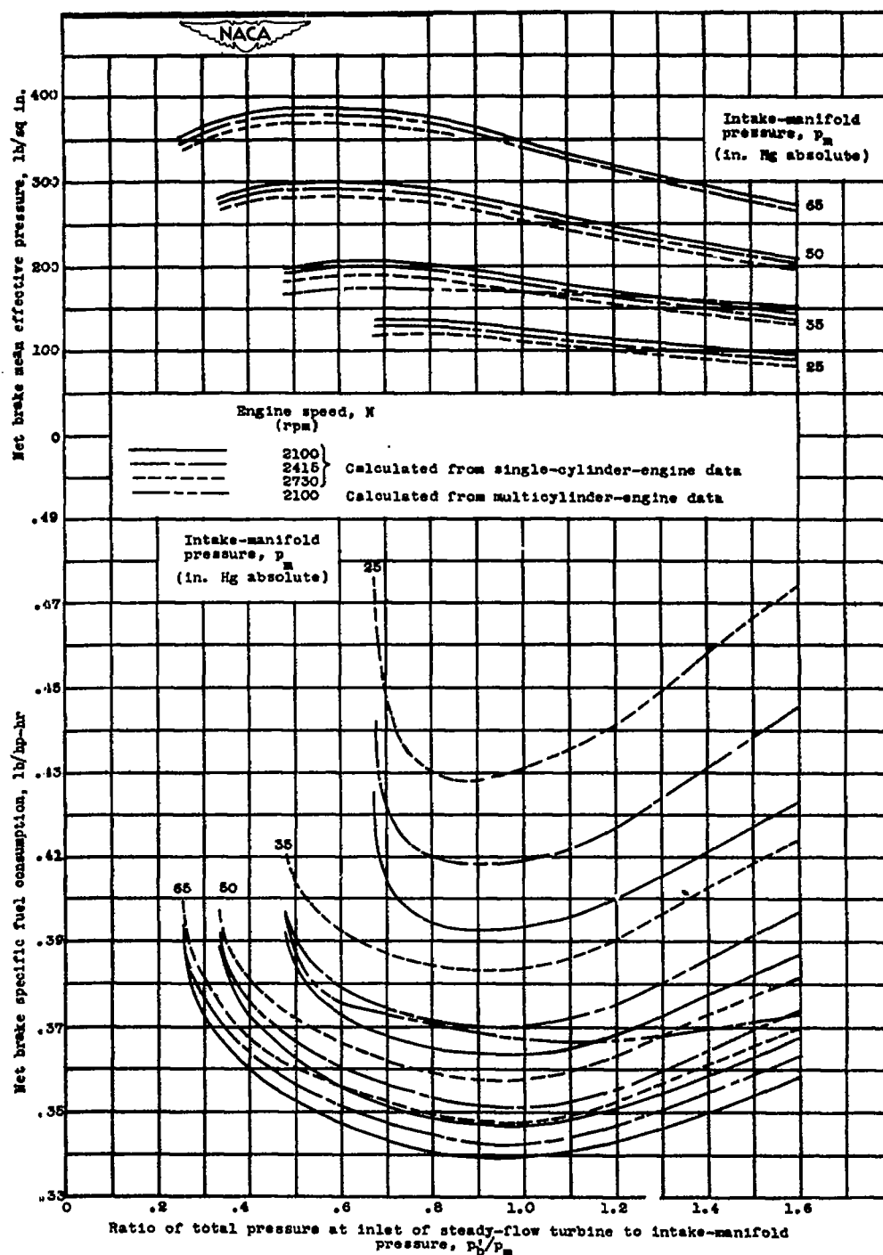
(b) Altitude, 15,000 feet. Figure 4. - Continued. Net brake mean effective pressure and brake specific fuel consumption of variable-component system for various intake-manifold pressures and engine speeds. Fuel-air ratio, 0.067; turbine and supercharger efficiencies, 70 percent; gear efficiencies, 85 percent.
