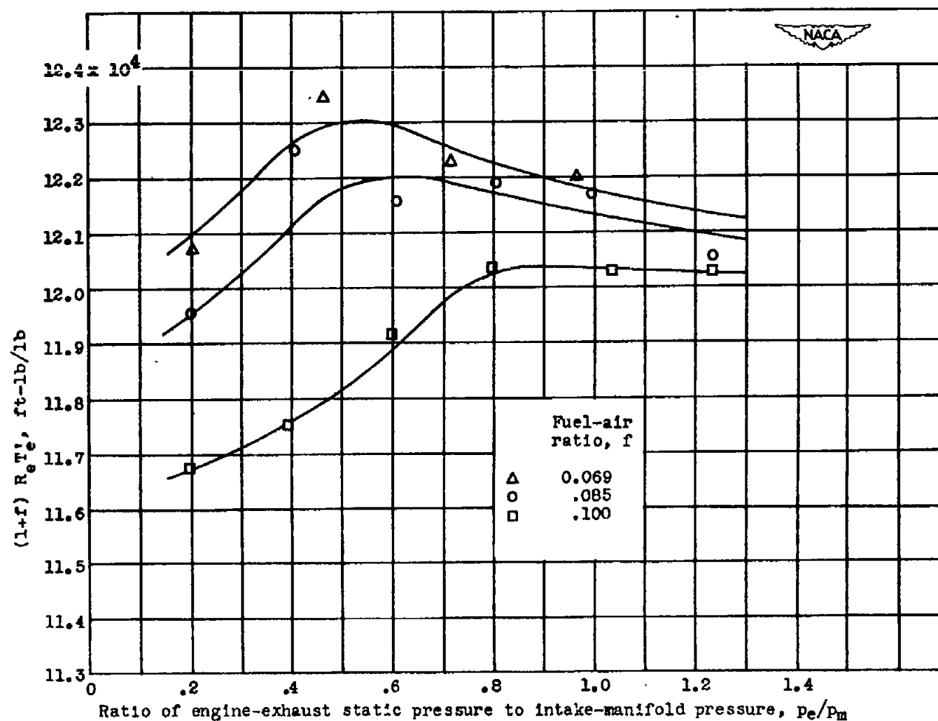
Figure 14. - Variation of (1+f)R_eT_e^i with exhaust pressure and fuel-air ratio. 18-cylinder multi-cylinder-engine data; intake-manifold pressure, 40 inches mercury absolute; engine speed, 2000 rpm.
