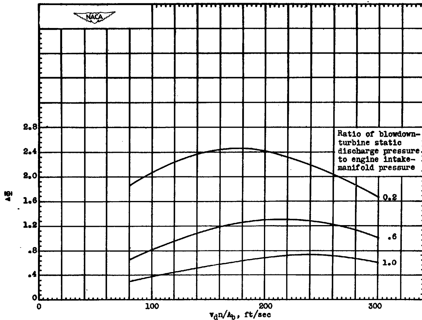
Figure 2. - Variation of net change in engine and blowdown-turbine power with ratio v_d n / A_b . Single-cylinder-engine data.
