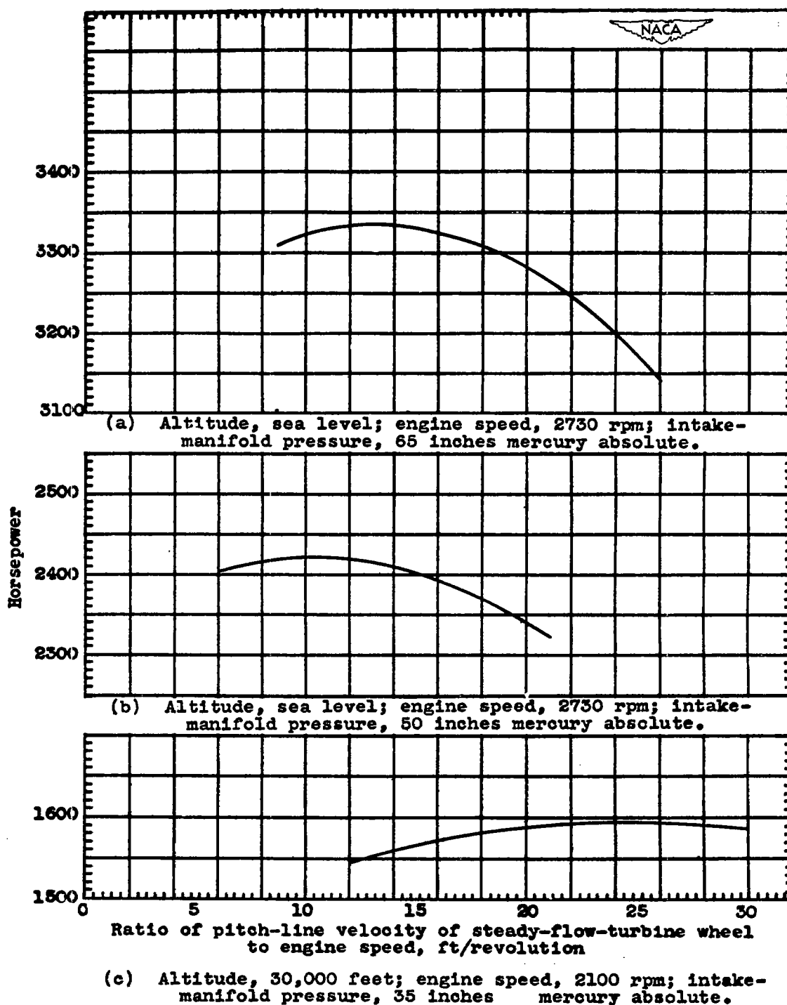
Figure 12. - Variation of power of composite engine with steady-flow turbine speed. Single-cylinder-engine data; turbine and supercharger efficiencies, 70 percent.
