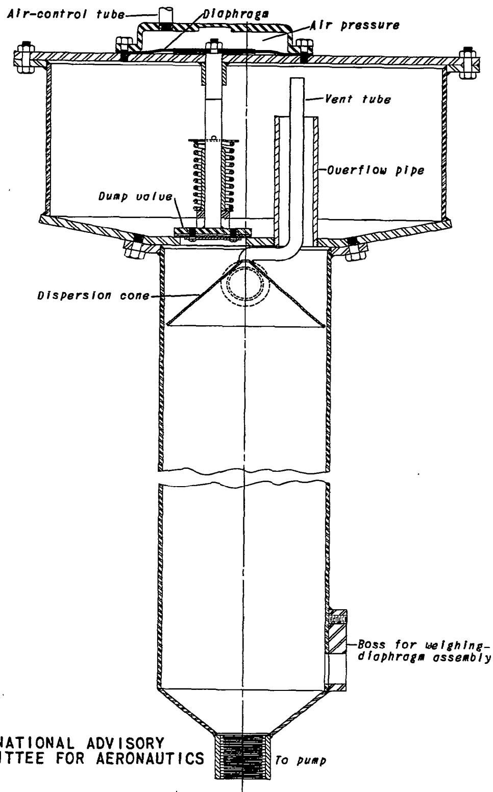
Figure 4. - Cross section of single-cylinder-engine oil-weighing tank.
