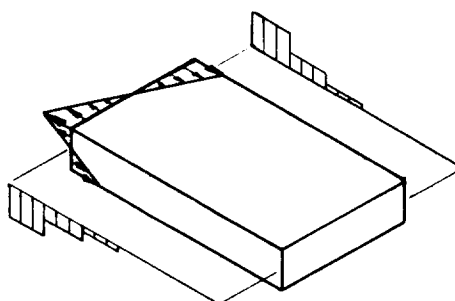
(b) Stress distribution to produce warping of root cross section.
