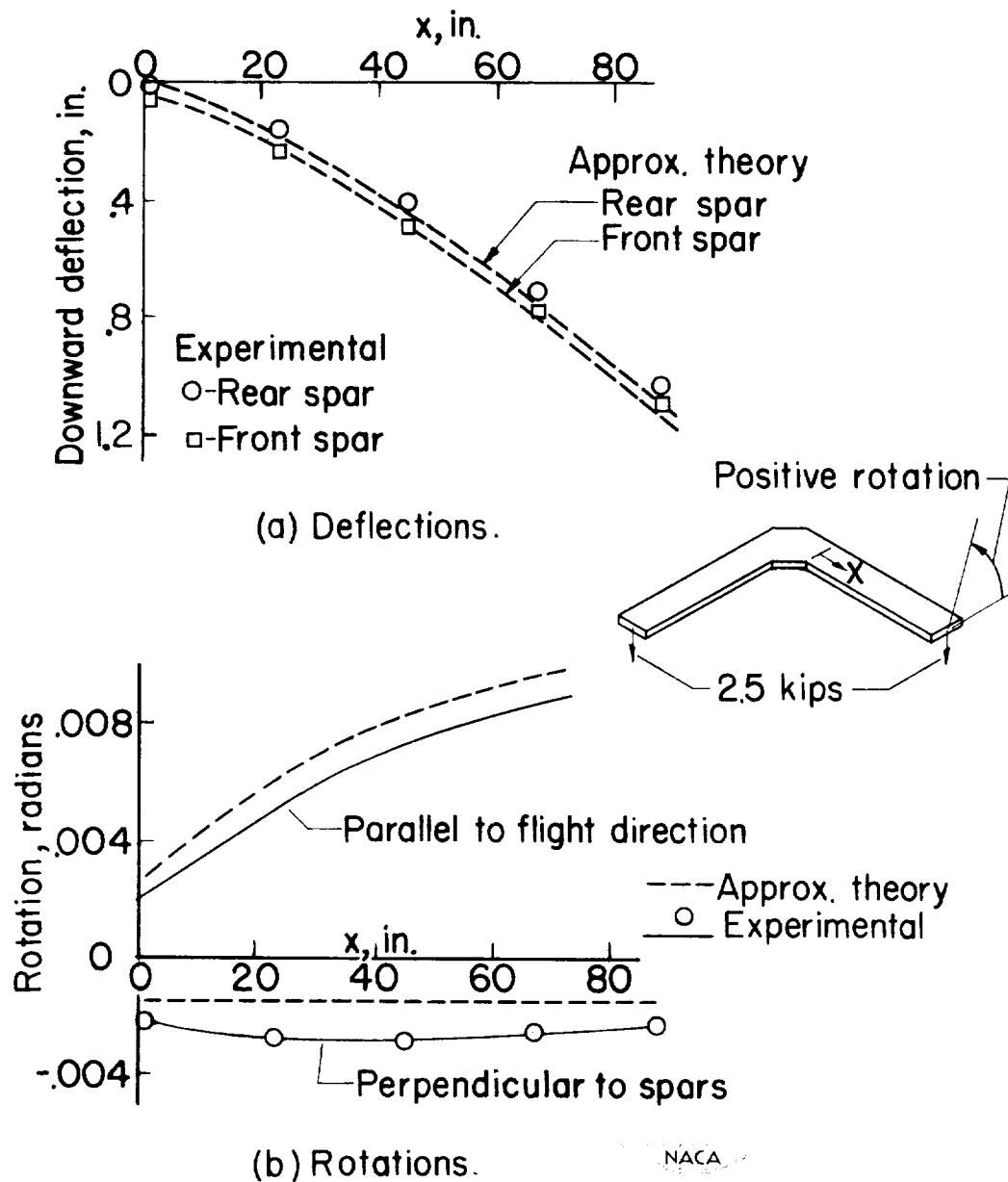
Figure 8:- Distortions of sweptback box beam for tip bending load.
