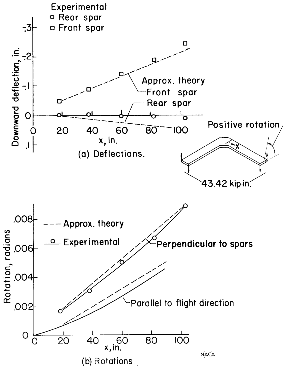
Figure 9.-Distortions of sweptback box beam for tip torque.
