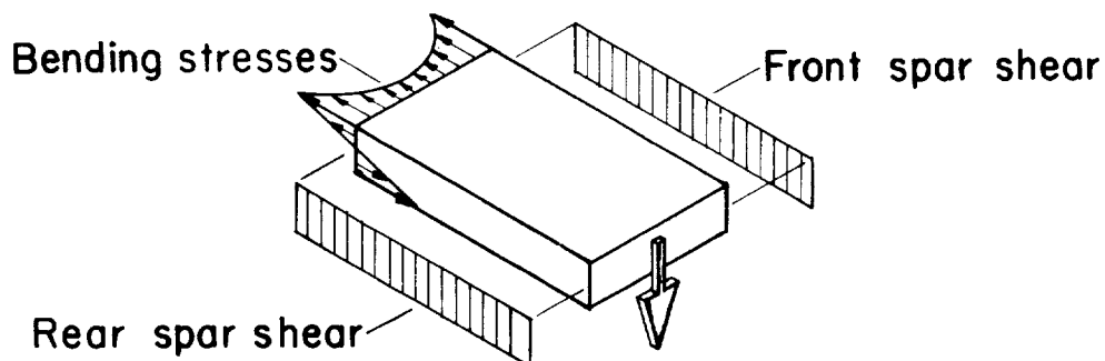
(a) Stress distributions for symmetrical restraint at cantilever root.
