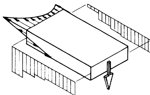
(c) Stress distribution in cantilever portion of sweptback box beam, obtained by superposition of (a) and (b).
