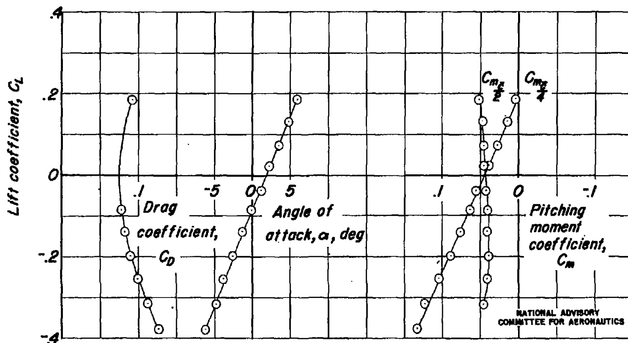
Figure 20. - Variation of drag coefficient, angle of attack, and pitching-moment coefficient with lift coefficient for configuration B_s W_{60} V_1 - \delta_0 = -9.9^\circ at 1.13 \times 10^6 Reynolds number.
