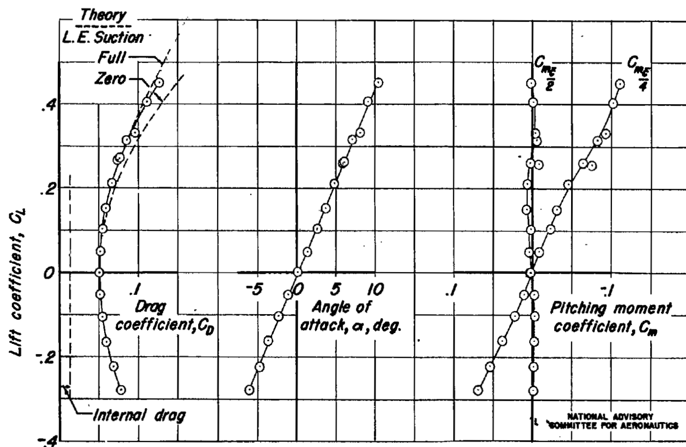
Figure 8.- Variation of drag coefficient, angle of attack, and pitching-moment coefficient with lift coefficient for the wing and fuselage (B 5 W 60 ) at 1.13 \times 10^6 Reynolds number.
