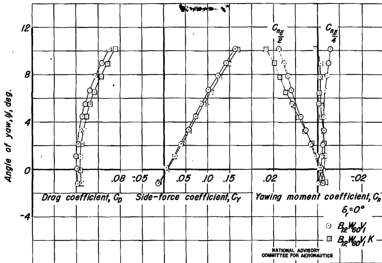
Figure 19.-Variation of drag, side-force, and yawing-moment coefficients with angle of yaw for configurations B_{12}W_{60}V_1 and B_{12}KW_{60}V_1 , \delta_r = 0^\circ at 1.13 \times 10^6 Reynolds number.
