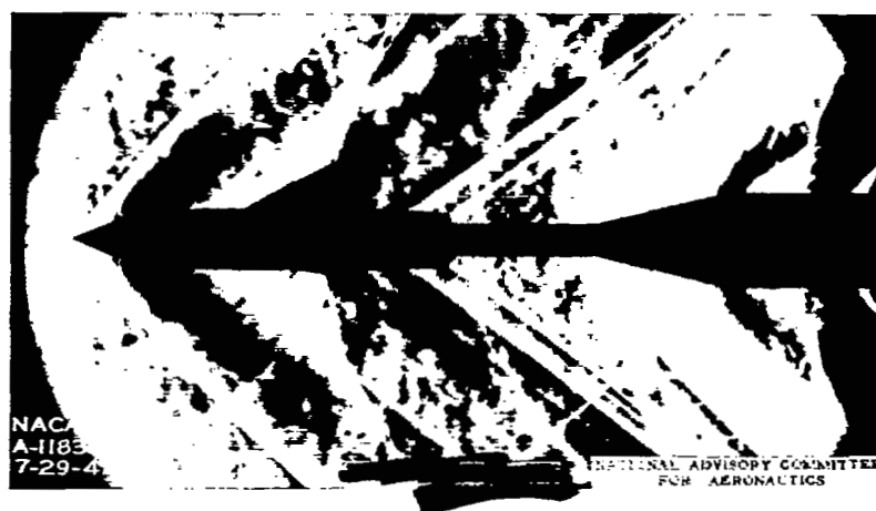
Figure 12.- Profile schlieren photograph of configuration B_8W_{60}V_1 at 1.13 \times 10^6 Reynolds number.
