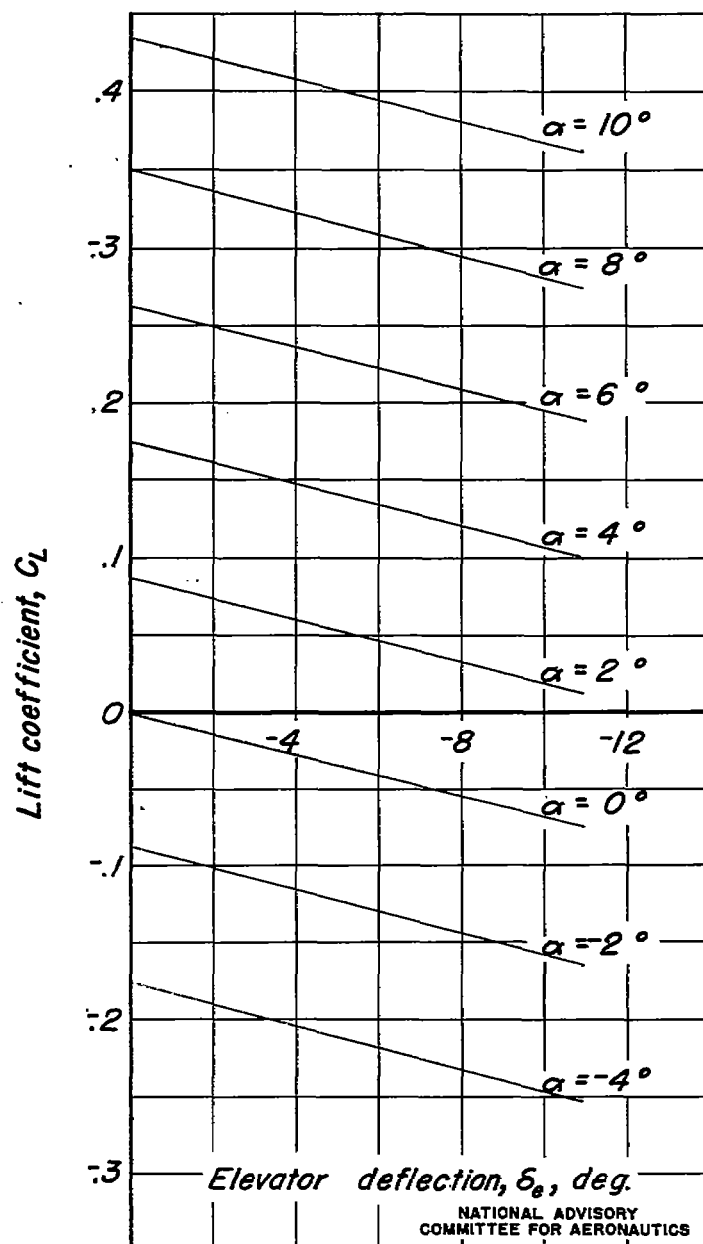
Figure 24.—Variation of lift coefficient with elevator deflection at several angles of attack for configuration B_5W_{60}V_2 at 1.13 \times 10^6 Reynolds number.
