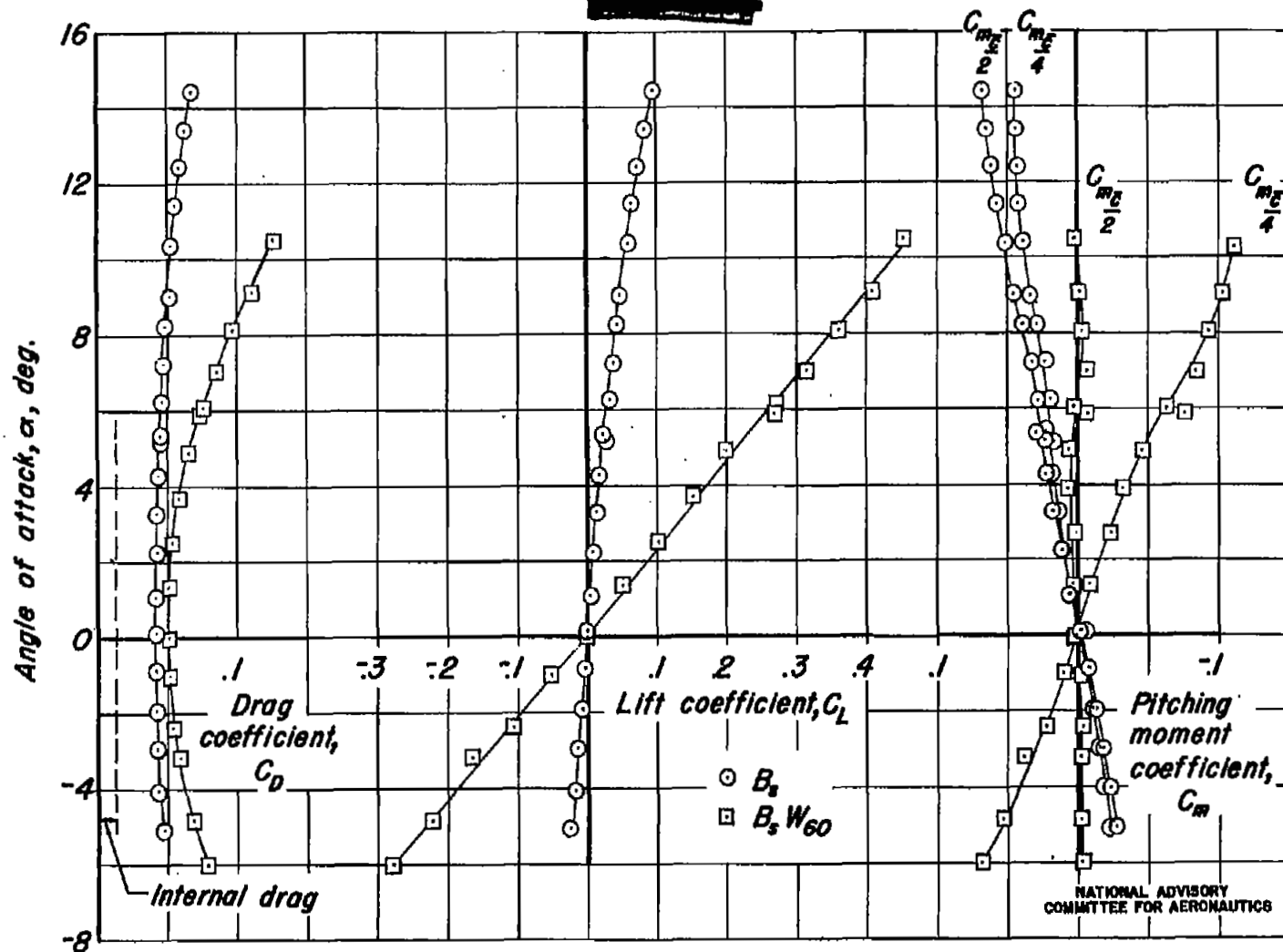
Figure 7.- Variation of drag, lift, and pitching-moment coefficients with angle of attack for the fuselage alone ( B_s ) and the wing and fuselage ( B_s W_{60} ) at 1.13 \times 10^6 Reynolds number.
