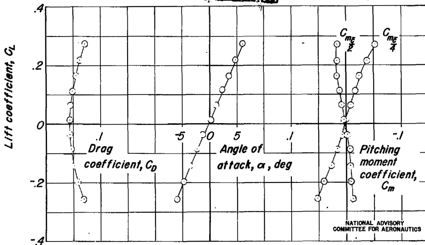
Figure 15. - Variation of drag coefficient, angle of attack, and pitching-moment coefficient with lift coefficient for configuration, B_{12} KW_{60} V_e - \delta_a = 0^\circ at 1.13 \times 10^6 Reynolds number.
