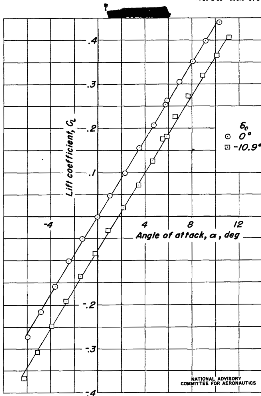
Figure 22. - Effect of elevator deflection on the variation of lift coefficient with angle of attack for configuration B_S W_{60} V_2 at 1.13 \times 10^6 Reynolds number.
