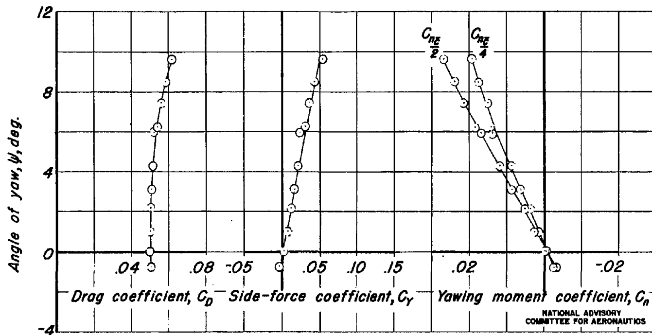
Figure 16. - Variation of drag, side-force, and yawing-moment coefficients with angle of yaw for the wing and fuselage ( B_5 W_{60} ) without vertical fin at 1.13 \times 10^6 Reynolds number.
