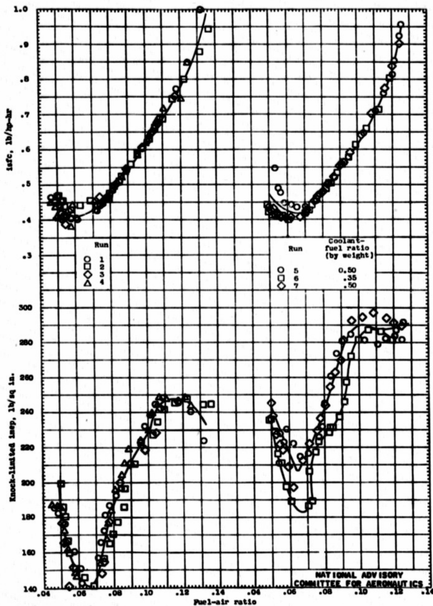
(a) No internal coolant. (b) Internal coolant, water. Figure 1. - Effect of water as internal coolant on knock-limited performance of AN-V-28, Amendment-2, fuel, CFR engine; engine speed, 2500 rpm; compression ratio, 7.0; spark advance, 30° B.T.C.; inlet-air temperature, 250° F; jacket temperature, 250° F.
