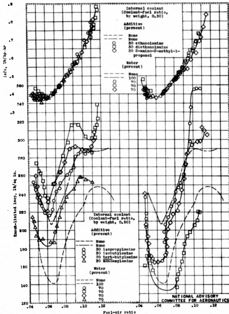
(a) Internal-coolant additives, alkyl amines. (b) Internal-coolant additives, alkanolamines. Figure 2. - Effect of various alkyl amines and alkanolamines as internal-coolant additives on knock-limited performance of AN-F-28, Amendment-2, fuel. CFR engine; engine speed, 2800 rpm; compression ratio, 7.0; spark advance, 30° B.T.C.; inlet-air temperature, 250° F; jacket temperature, 280° F.
