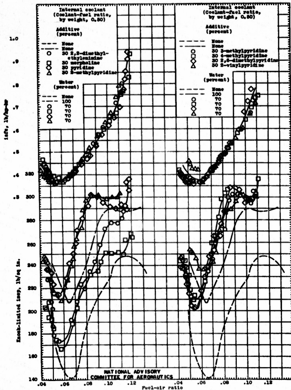
Figure 4. - Effect of various heterocyclic compounds as internal-coolant additives on knock-limited performance of AN-P-28, Amendment-2, fuel. CFR engine; engine speed, 2500 rpm; compression ratio, 7.0; spark advance, 30° B.T.C.; inlet-air temperature, 250° F; jacket temperature, 250° F.
