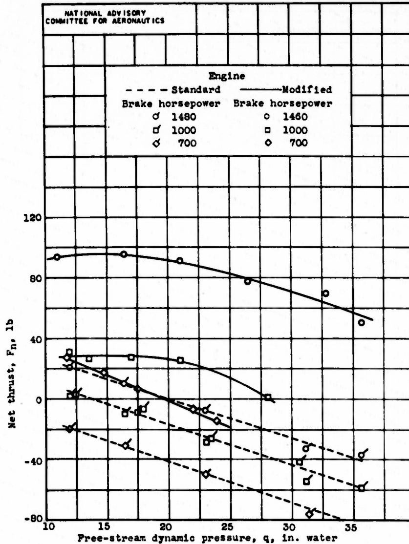
Figure 17. - Comparison of net thrust of cooling air and exhaust gas for modified and standard engines.
