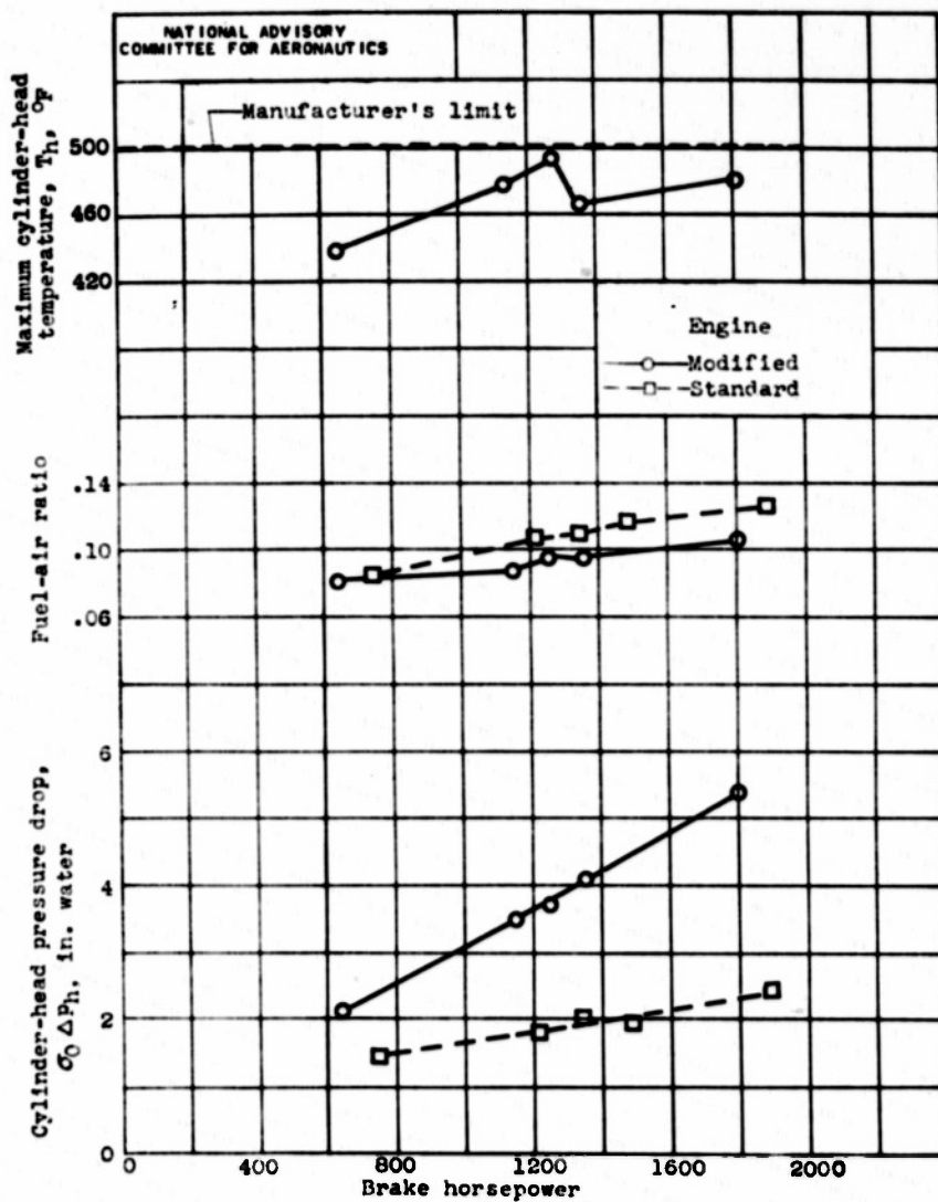
Figure 12. - Cooling characteristics of modified and standard engines on ground with cowl flaps open at free-air temperature of 35° F.
