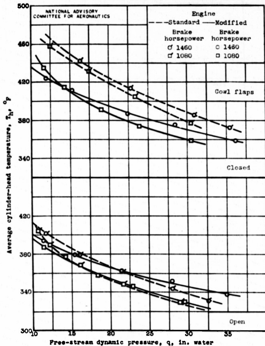
Figure 14. - Variation of average cylinder-head temperature with free-stream dynamic pressure at altitude of 5000 feet and free-air temperature of 46° F.
