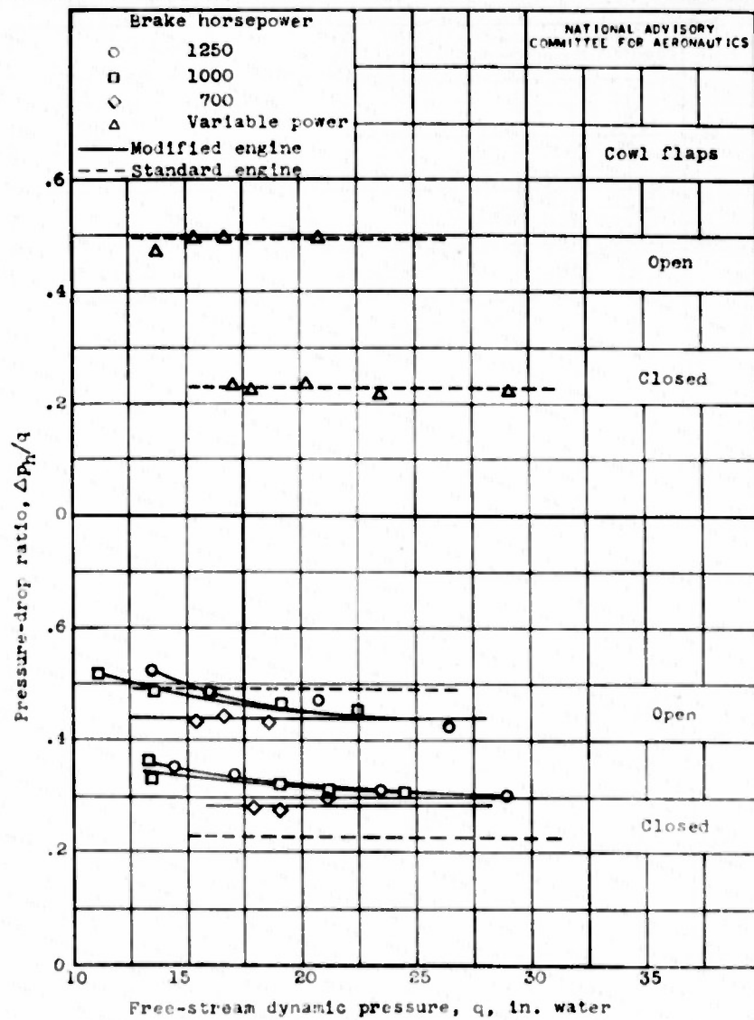
Figure 13. - Concluded. Available engine cylinder-head cooling-air pressure drop.
