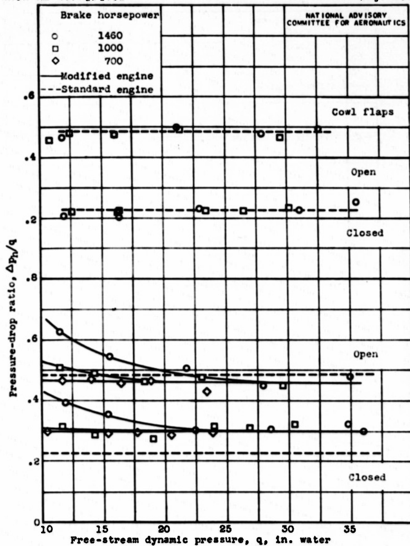
Figure 13. - Available engine cylinder-head cooling-air pressure drop.
