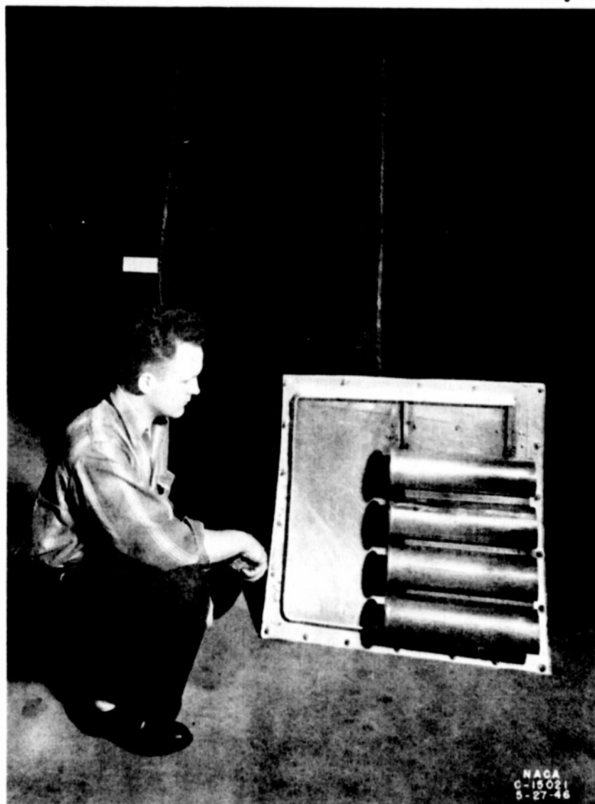
Figure 6. - First-stage ejectors mounted on removable accessory skin panel.
