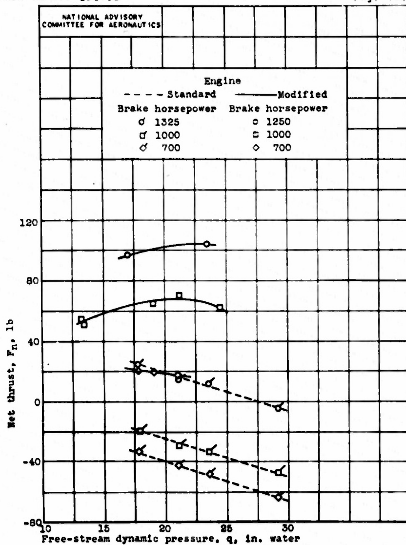
Figure 17. - Concluded. Comparison of net thrust of cooling air and exhaust gas for modified and standard engines.
