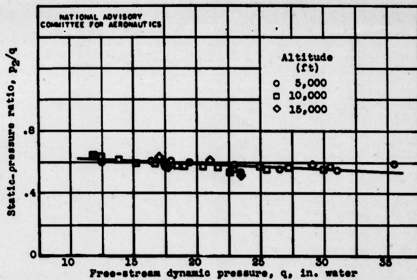
Figure 9. - Average static pressure behind standard engine with cowl flaps closed.
