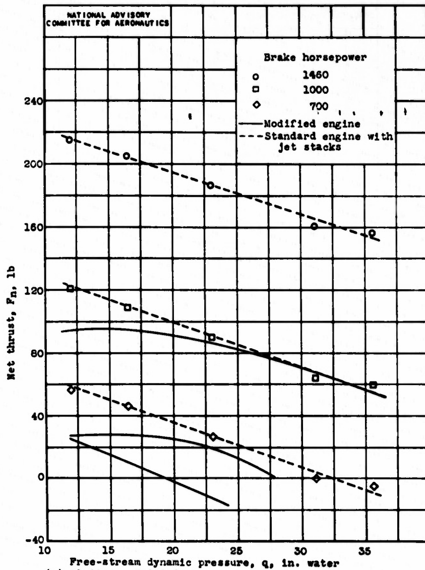
Figure 18. - Comparison of net thrust of cooling air and exhaust gas for modified engine and standard engine with jet stacks.
