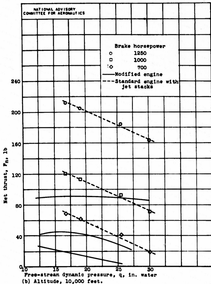
Figure 18. - Continued. Comparison of net thrust of cooling air and exhaust gas for modified engine and standard engine with jet stacks.
