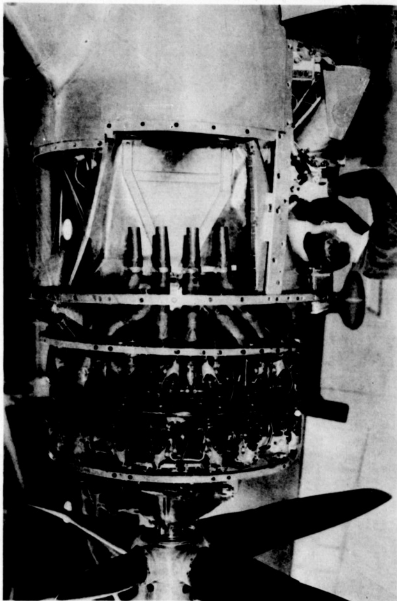
Figure 2. - Exhaust-ejector installation in left nacelle of test airplane.
