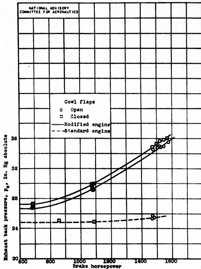
Figure 15. - Variation of exhaust back pressure with engine power at altitude of 5000 feet.
