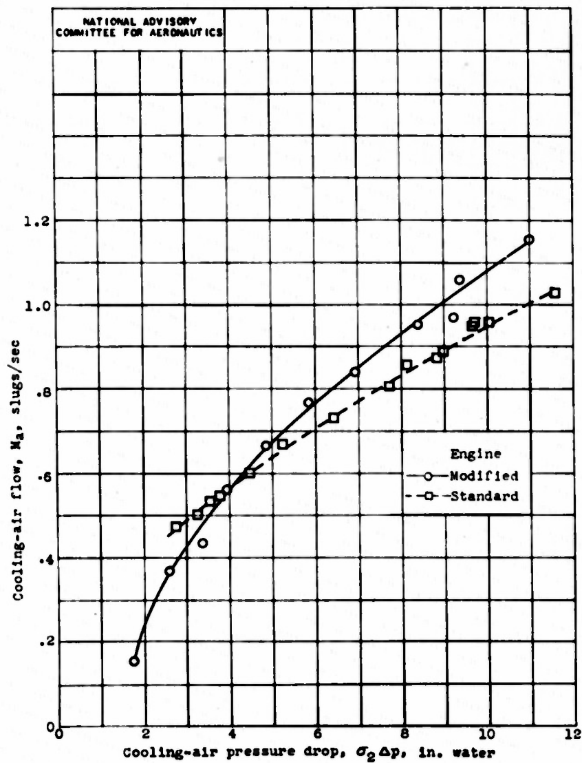
Figure 11. - Engine cooling-air-flow calibration from cooling blower.
