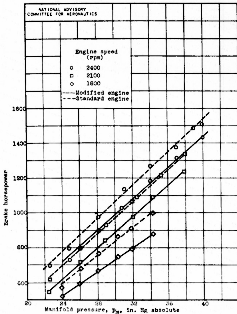
Figure 16. - Engine calibrations at altitude of 5000 feet.
