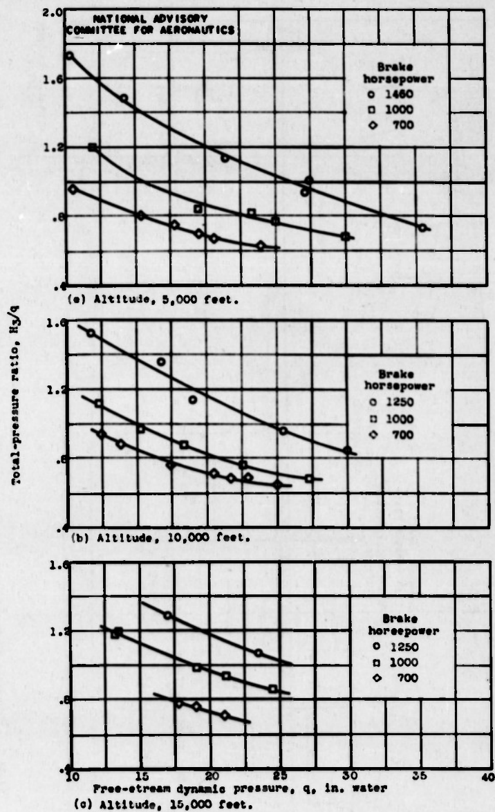
Figure 8. - Average total pressure in exhaust ejectors with cowl flaps closed.
