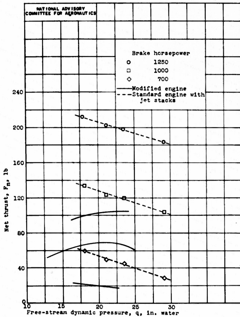
Figure 18. - Concluded. Comparison of net thrust of cooling air and exhaust gas for modified engine and standard engine with jet stacks.
