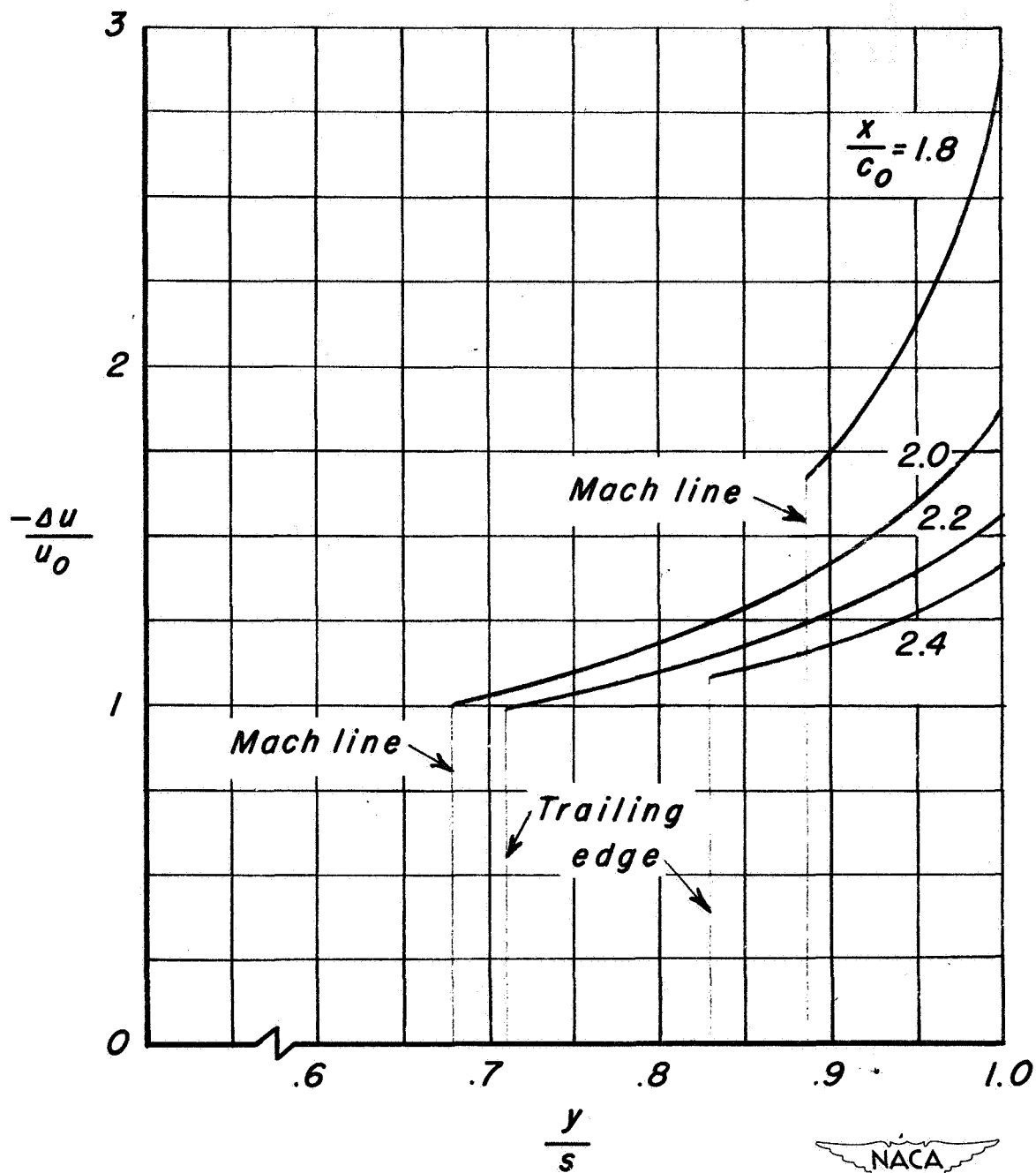
Figure 16.— Spanwise distribution of incremental velocity at various chordwise stations within the Mach cone from the tip of the untapered wing.
