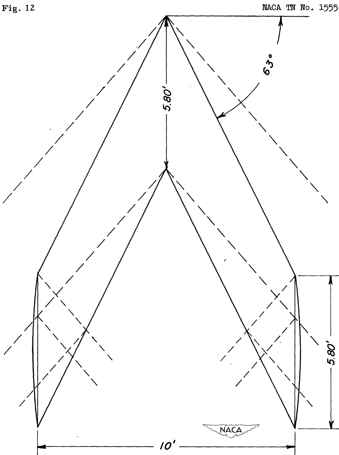
Figure 12.— Untapered wing for which pressure distribution was calculated, showing primary and secondary Mach lines at M=1.5 .
