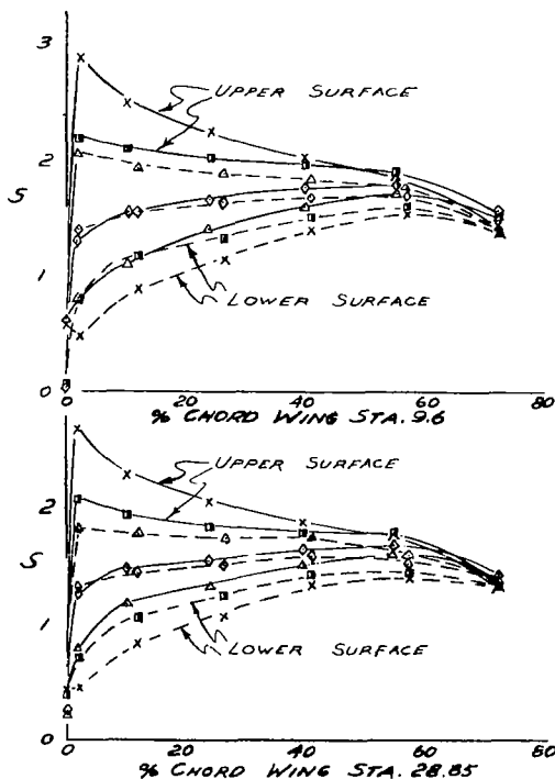
(d) Wing and fuselage pressure distribution at Mach numbers 0.3 and 0.5.
