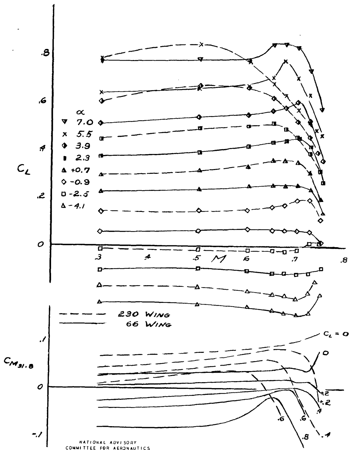
Figure 37.- Comparison of 230 wing and 66 wing with large booms, fuselage, all accessories, tail.
