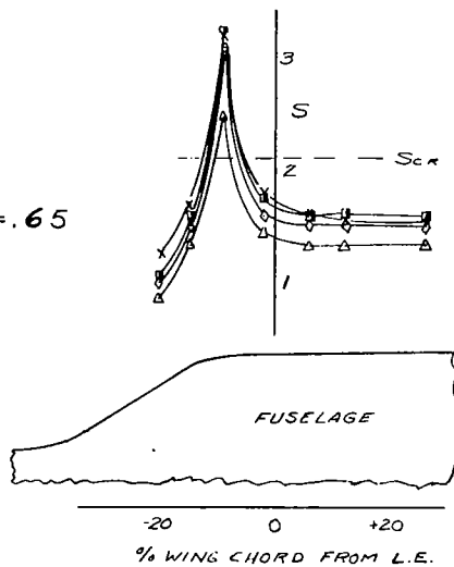
(e) Wing and fuselage pressure distribution at Mach numbers of 0.6 and 0.65.
