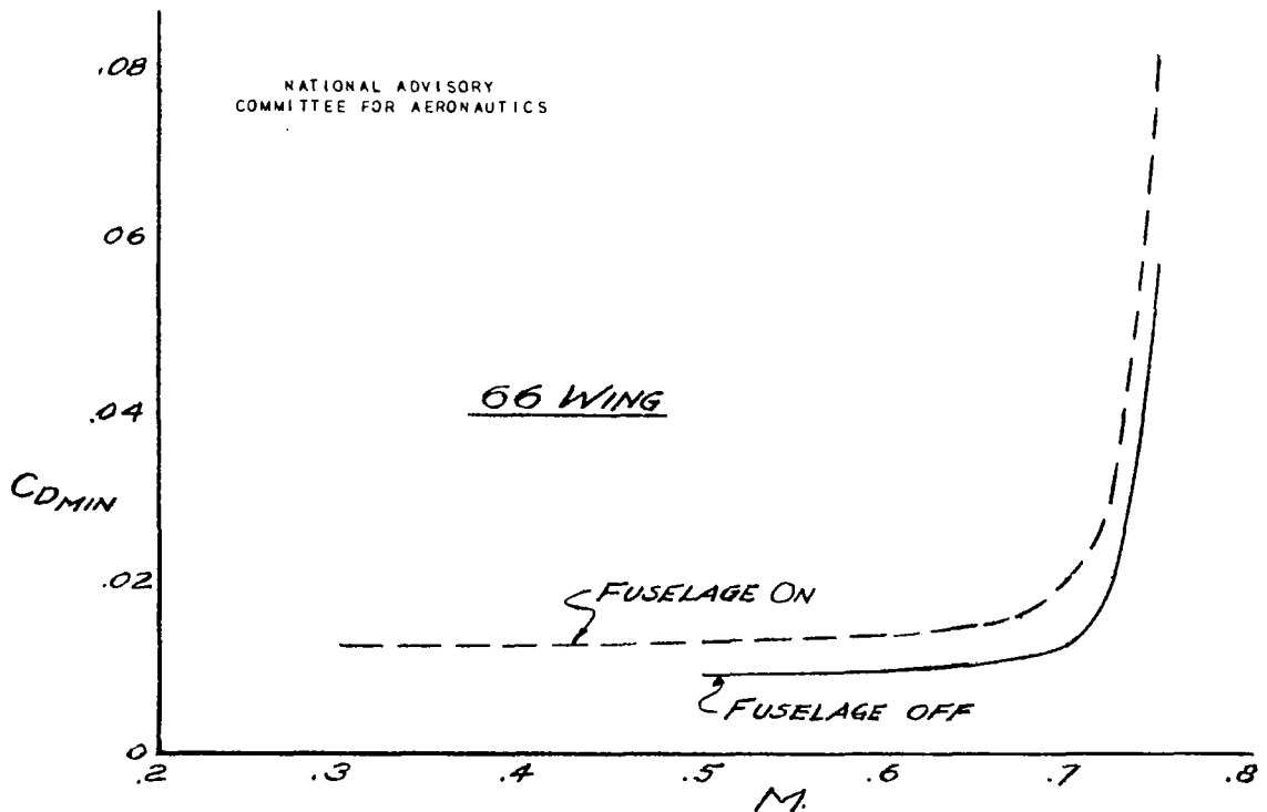
Figure 30.- Effect of fuselage on C_{D_{min}} with large booms, tail.
