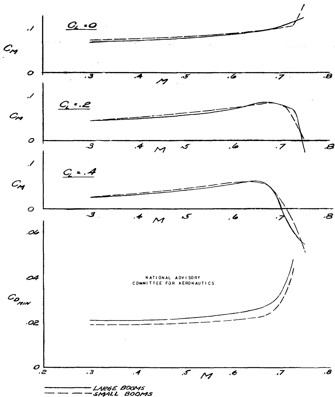
Figure 32.- Effect of boom size on C_M and C_{D_{min}} ; 230 wing, fuselage, all accessories, tail.
