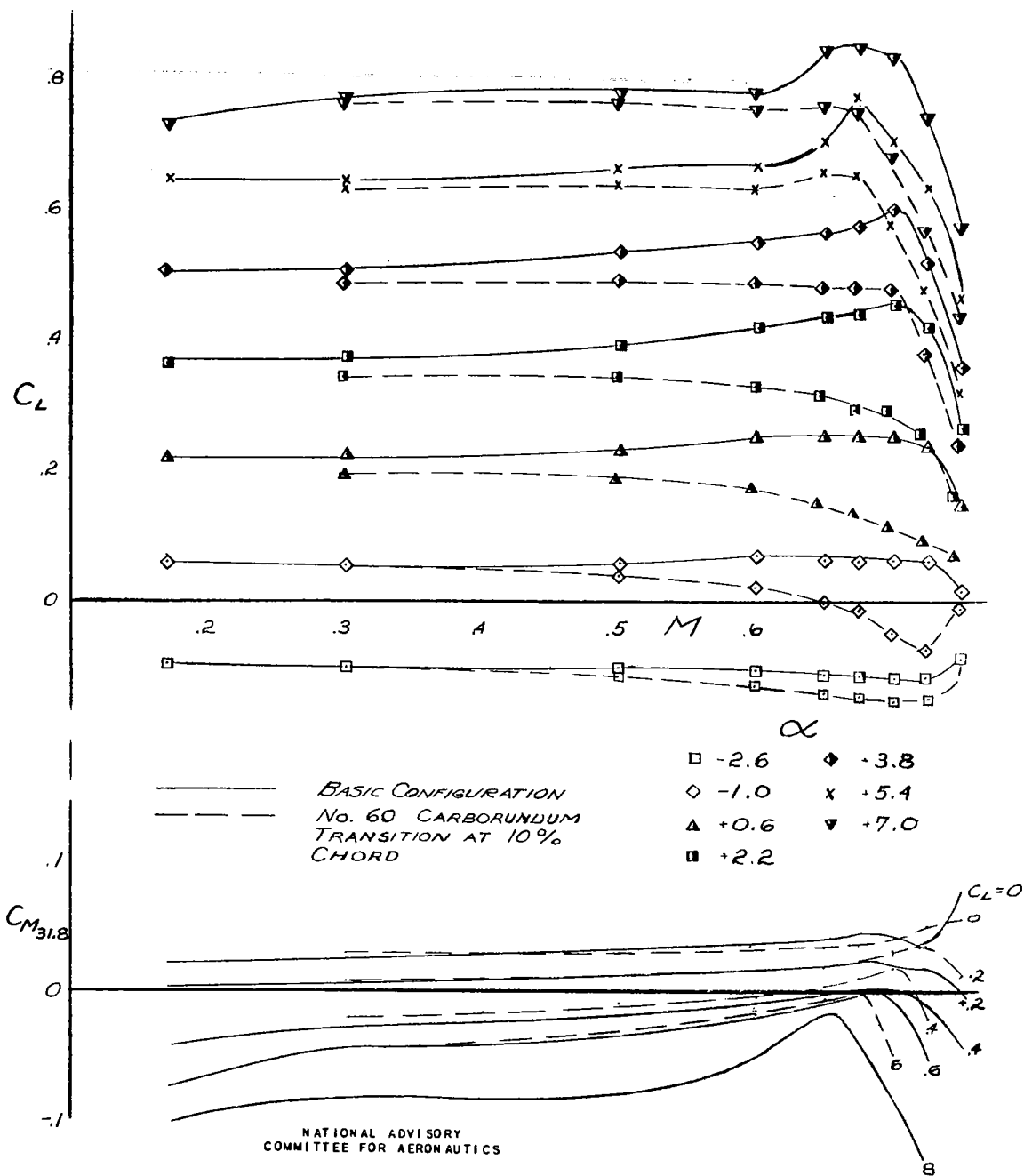
Figure 41.- Effect of fixing transition on C_L and C_M ; 66 wing, large booms, fuselage, all accessories, tail.
