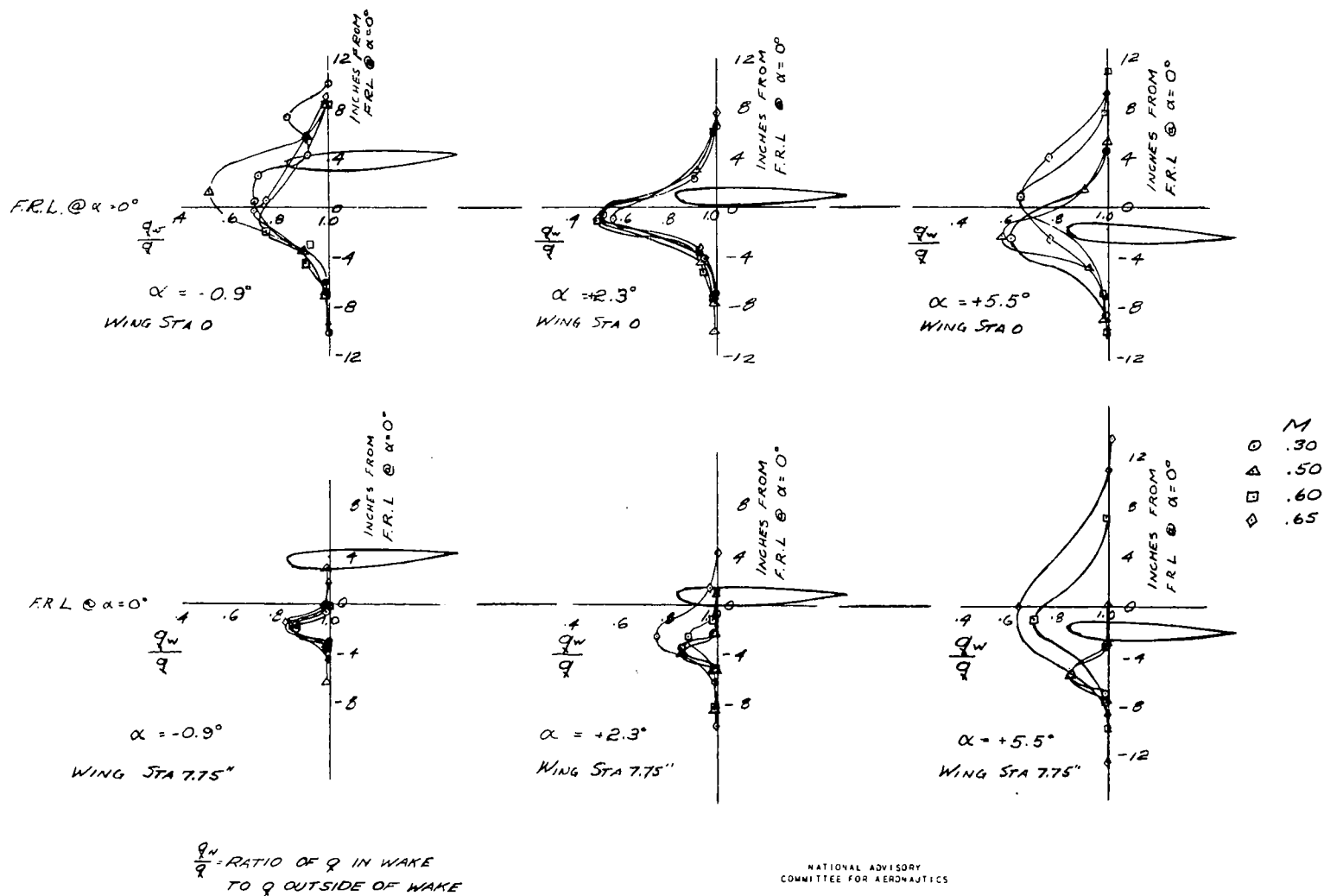
Figure 23.- Wake position at tail; 230 wing, large booms, fuselage, all accessories.
