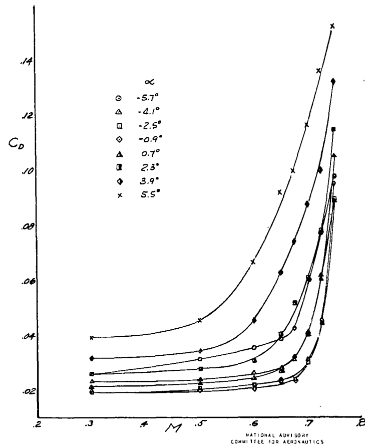
(c) Variation of C_L , C_D , and C_M with Mach number.
