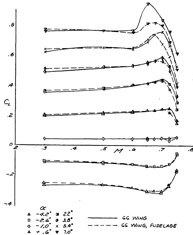
Figure 29.- Effect of fuselage on C_L with large booms, tail.
