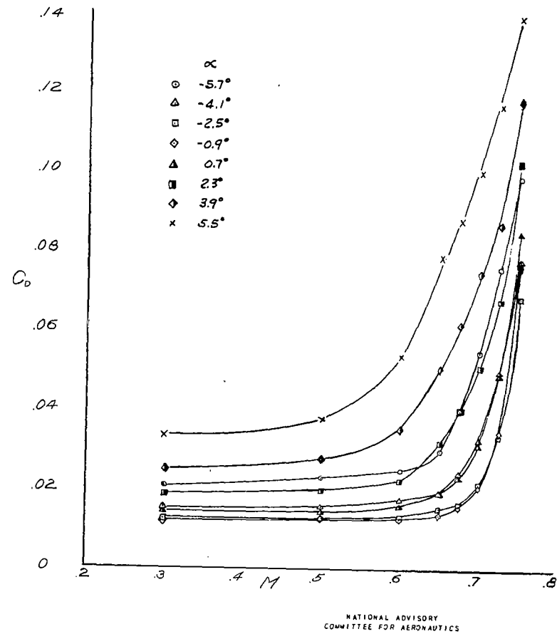
(c) Variation of C_L , C_D , and C_M with Mach number.
