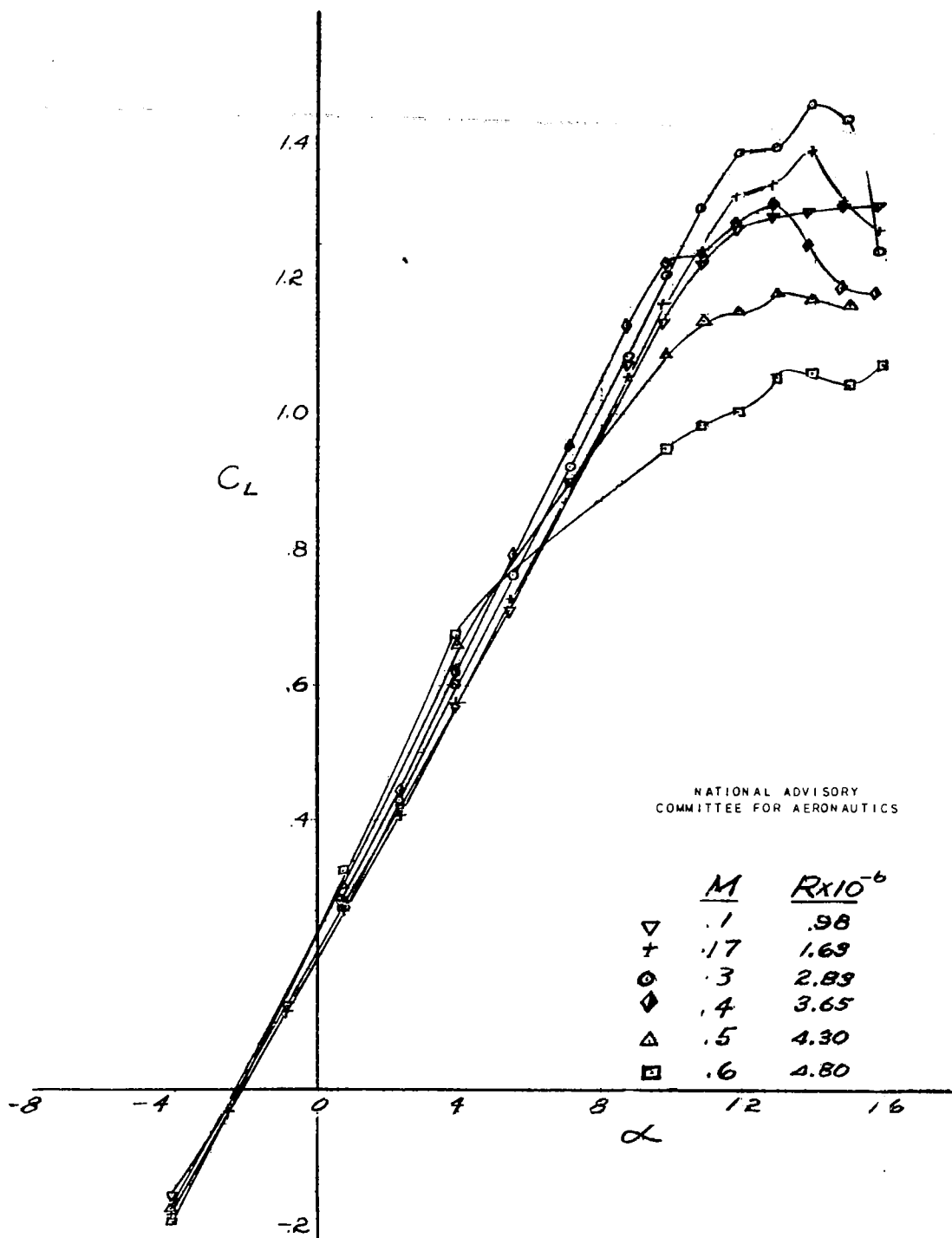
(e) Variations of C_L with angle of attack at Mach numbers of 0.1 through 0.6.
