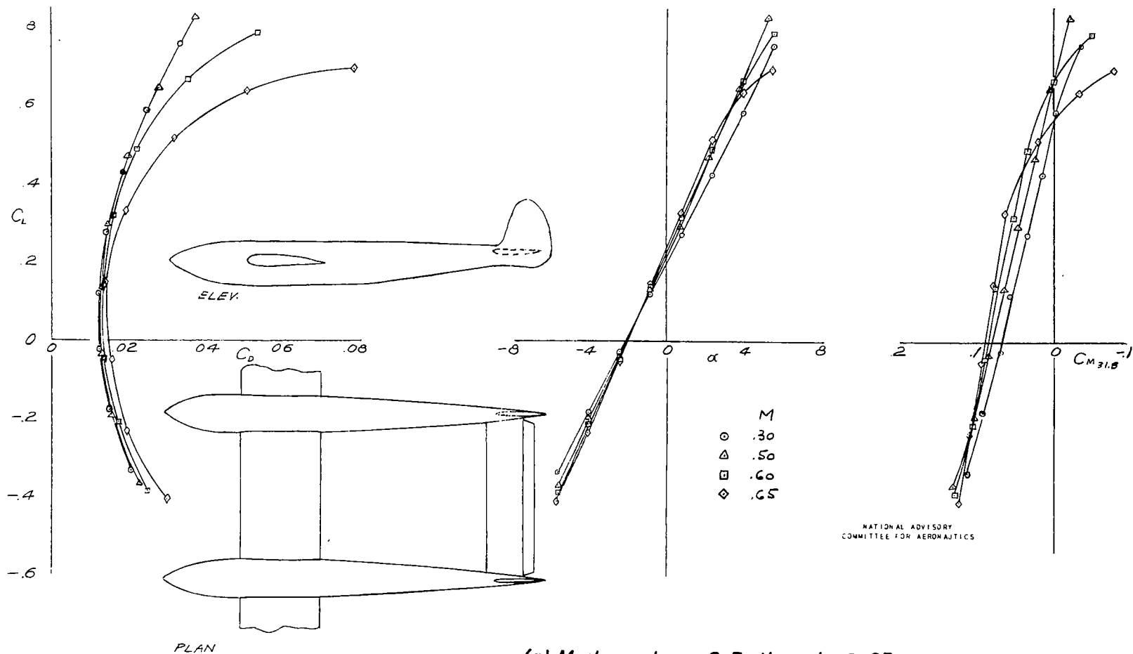
Figure 7.- Characteristics with 230 wing, large booms, tail.
