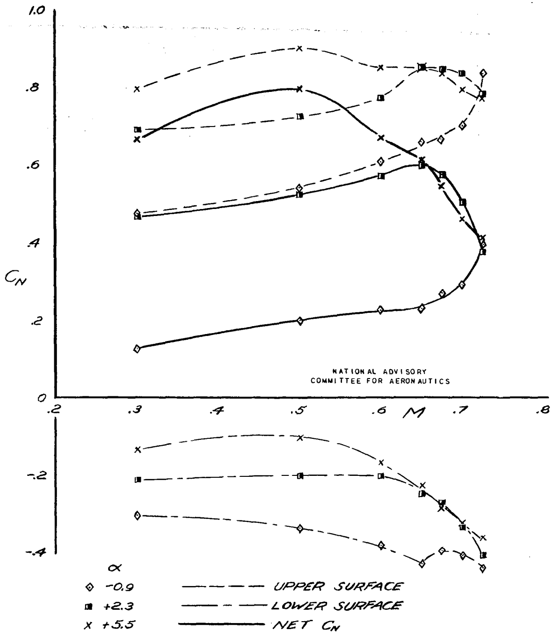
Figure 36.— Normal force coefficients, station 9.6; modified 230 wing, large booms, fuselage, all accessories, tail.
