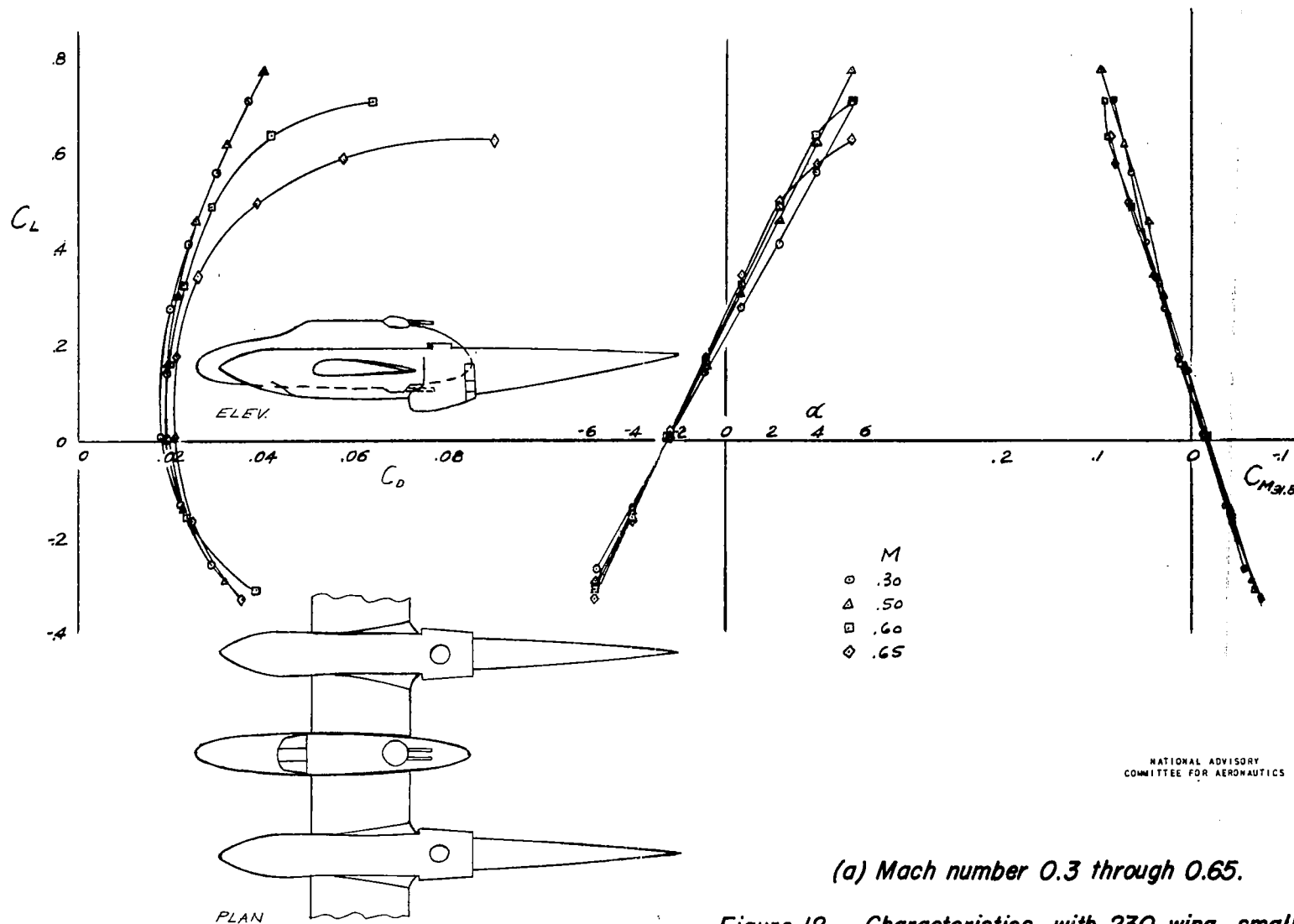
Figure 12.- Characteristics with 230 wing, small booms, fuselage, all accessories.
