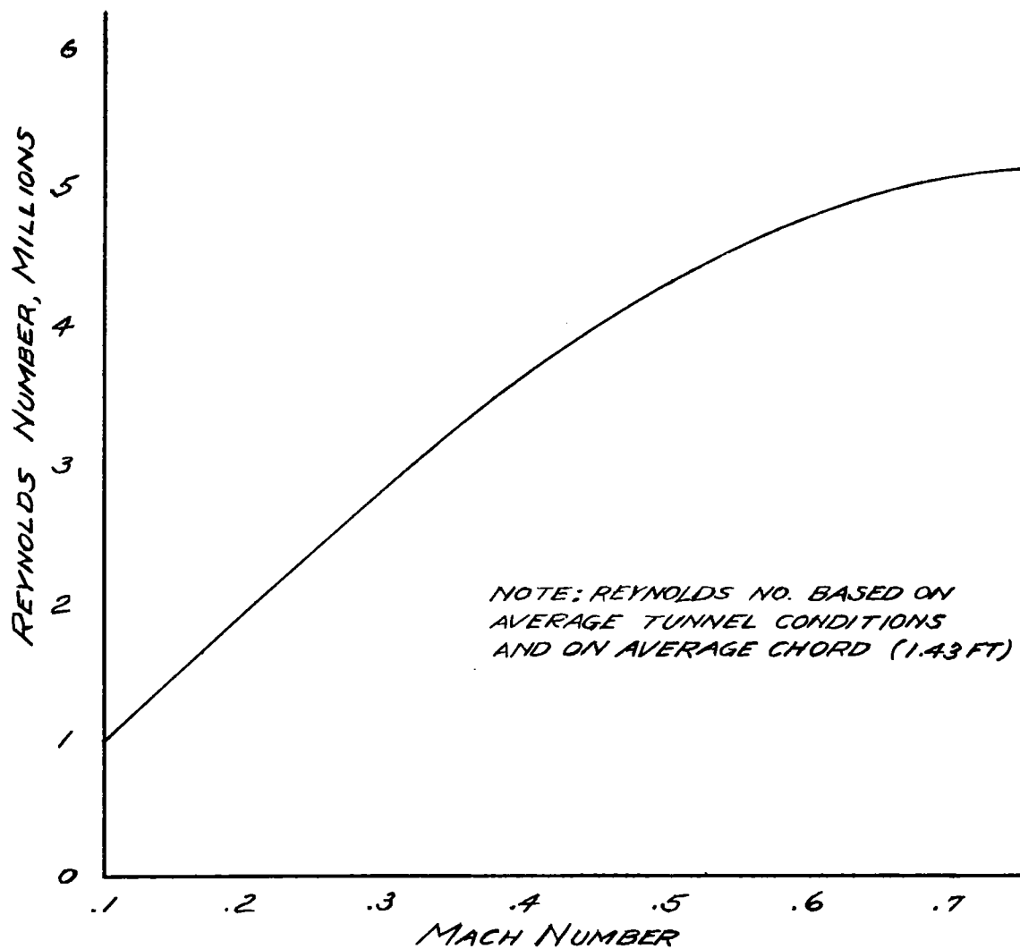
Figure 39.- Reynolds number variation with Mach number for average tunnel conditions.
