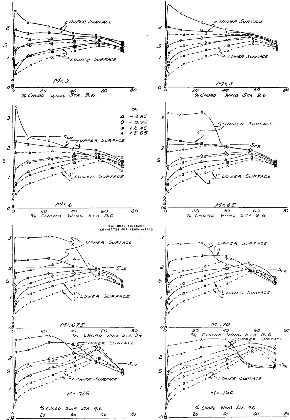
(d) Wing pressure distribution at various Mach numbers.
