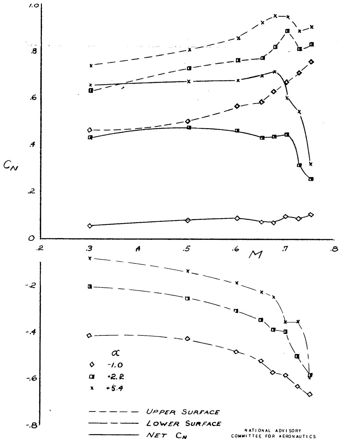
Figure 34.— Normal force coefficients, wing station 9.6; 66 wing, large booms, fuselage, tail.
