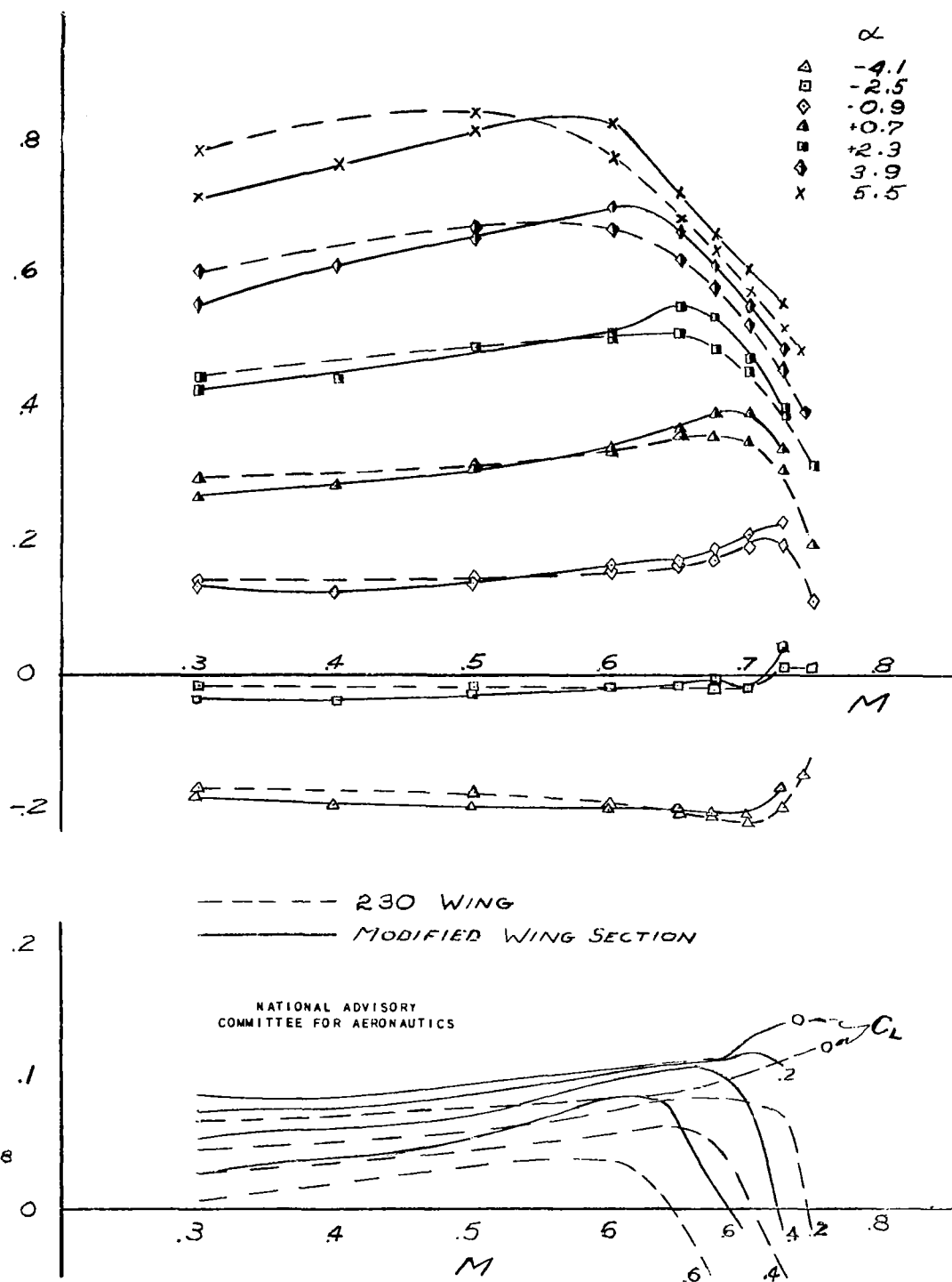
Figure 35.— Effect of 230 wing modification on C_L and C_M with large booms, fuselage, all accessories, tail.
