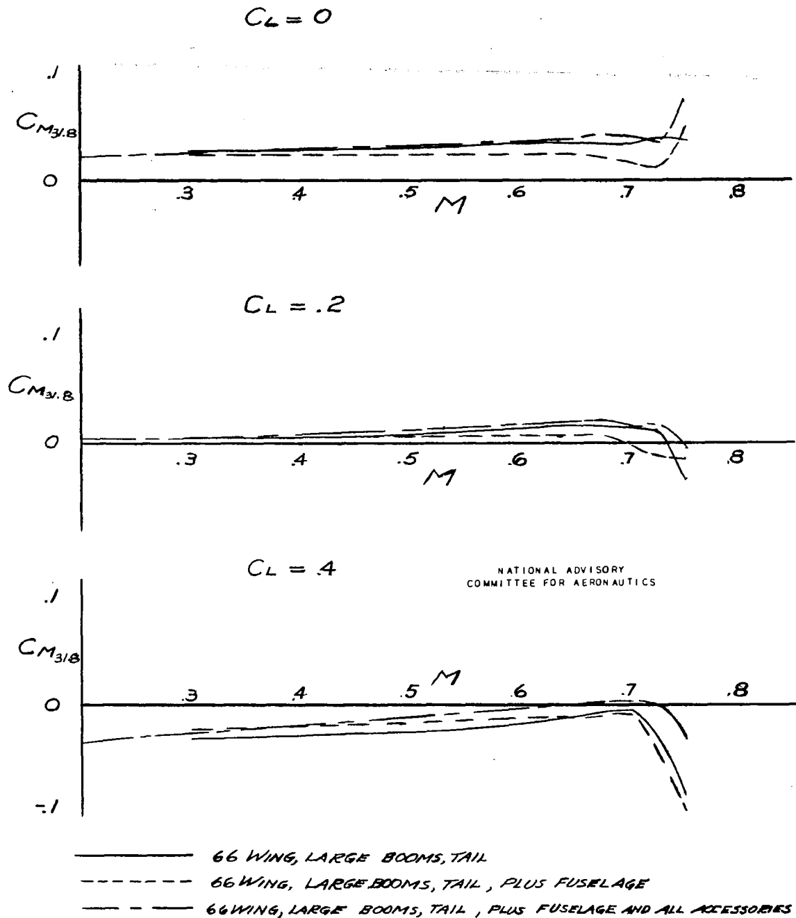
Figure 28.- Effect of build-up on C_M with 66 wing, large booms, tail.
