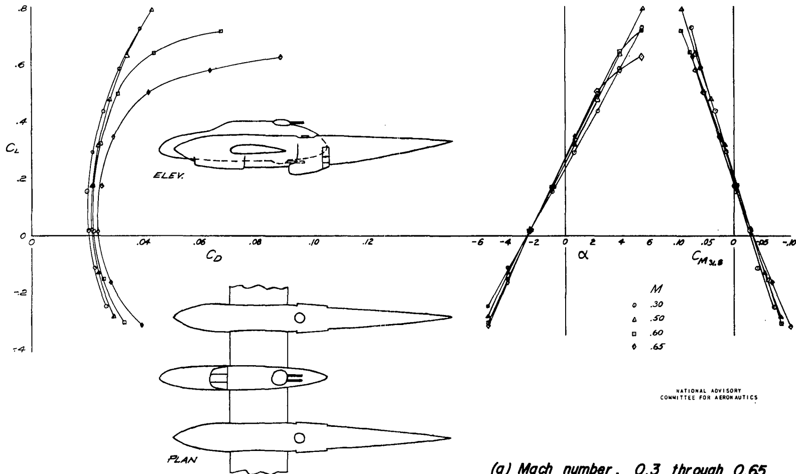
Figure 9.- Characteristics with 230 wing, large booms, fuselage, all accessories.
