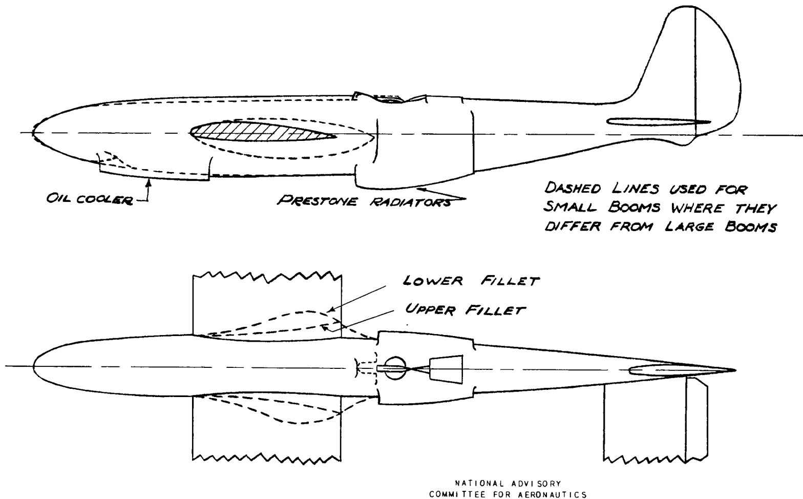
Figure 4.- Outlines of the large and small booms.
