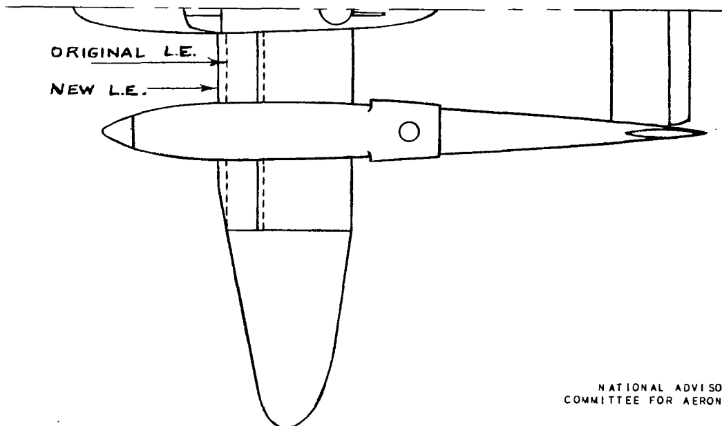
Figure 3.- Modification of the 23016 wing section.
