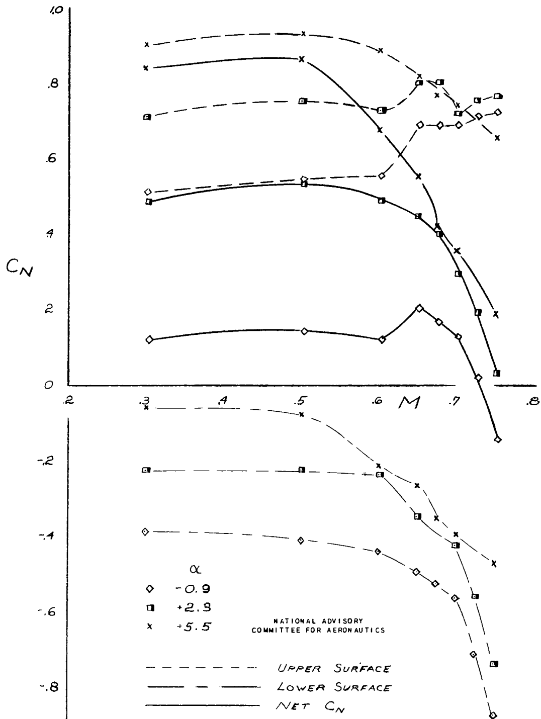
Figure 33.- Normal force coefficients; wing station 9.6; 230 wing, large booms, fuselage, tail.
