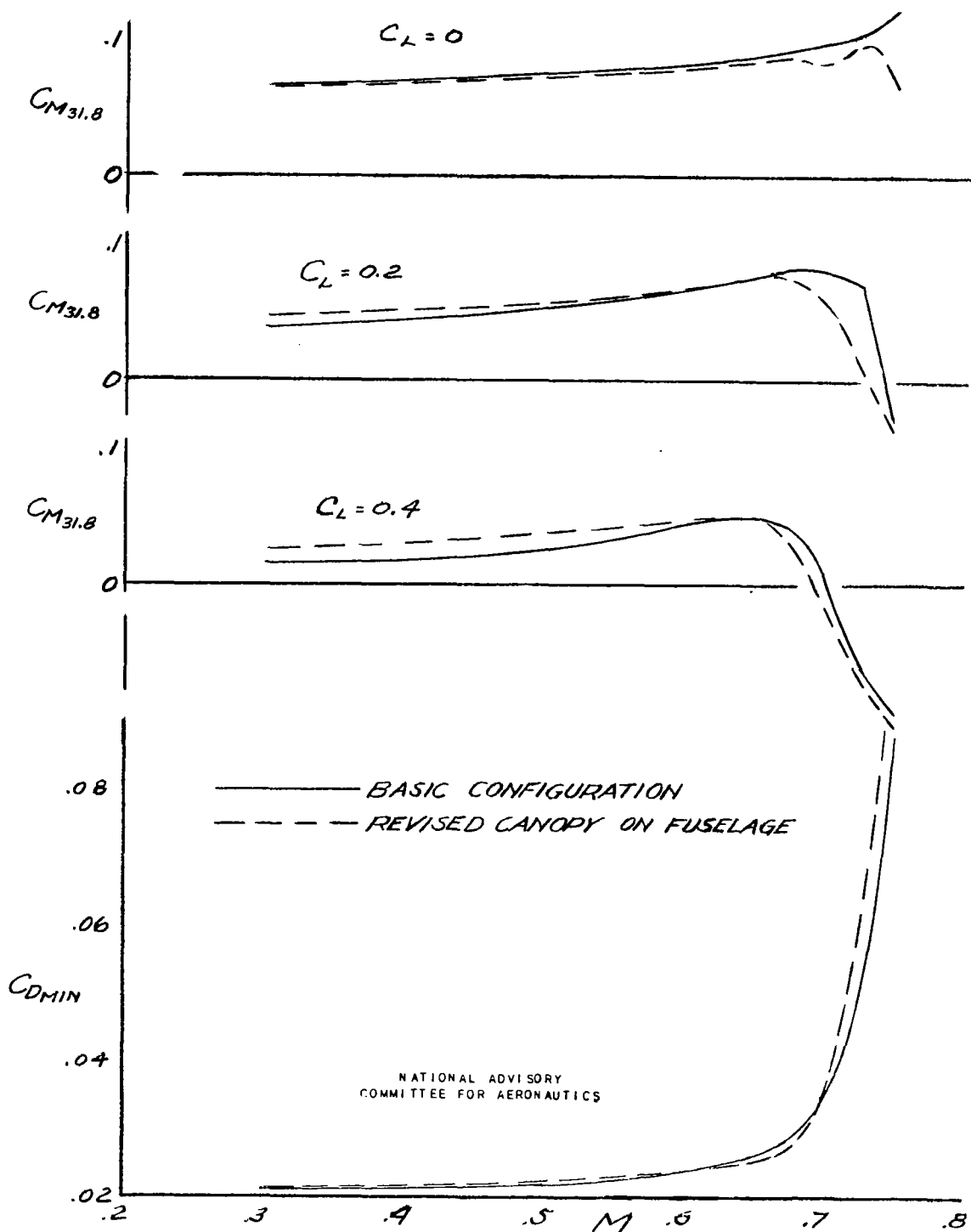
Figure 31.- Effect of canopy revision on C_M and C_{D_{min}} ; 230 wing, large booms, fuselage, all accessories, tail.
