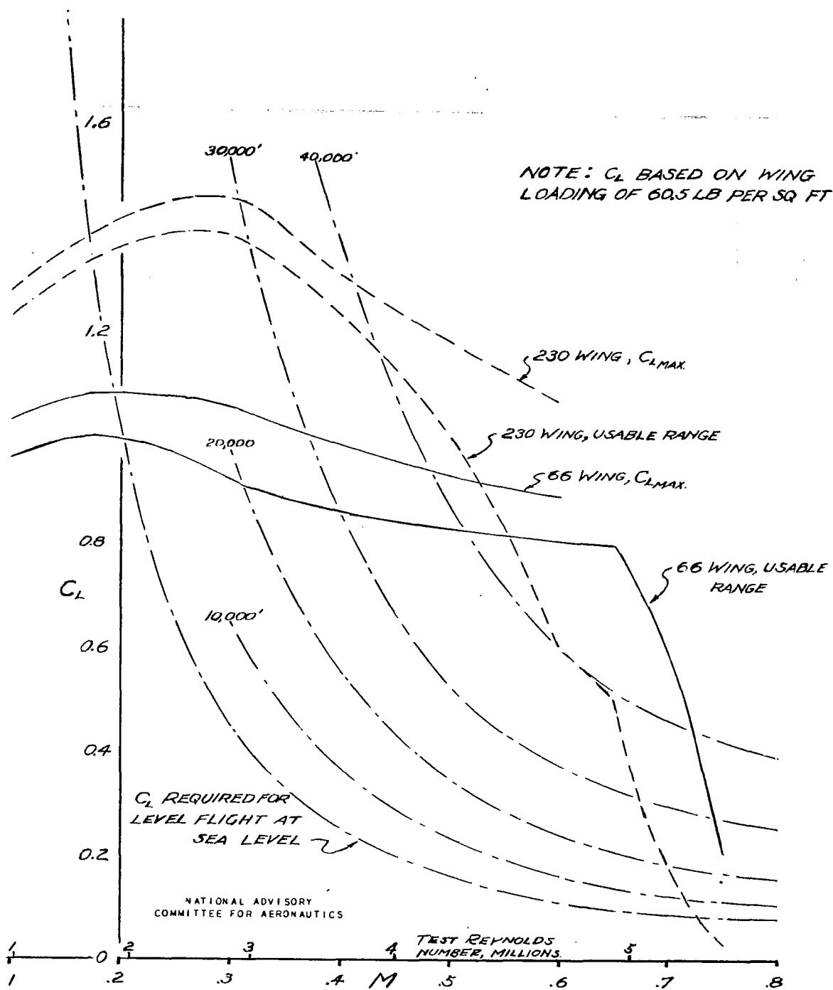
Figure 38.— Maximum C_L , usable C_L range, and C_L for level flight for 230 wing and 66 wing with large booms, fuselage, all accessories, tail.
