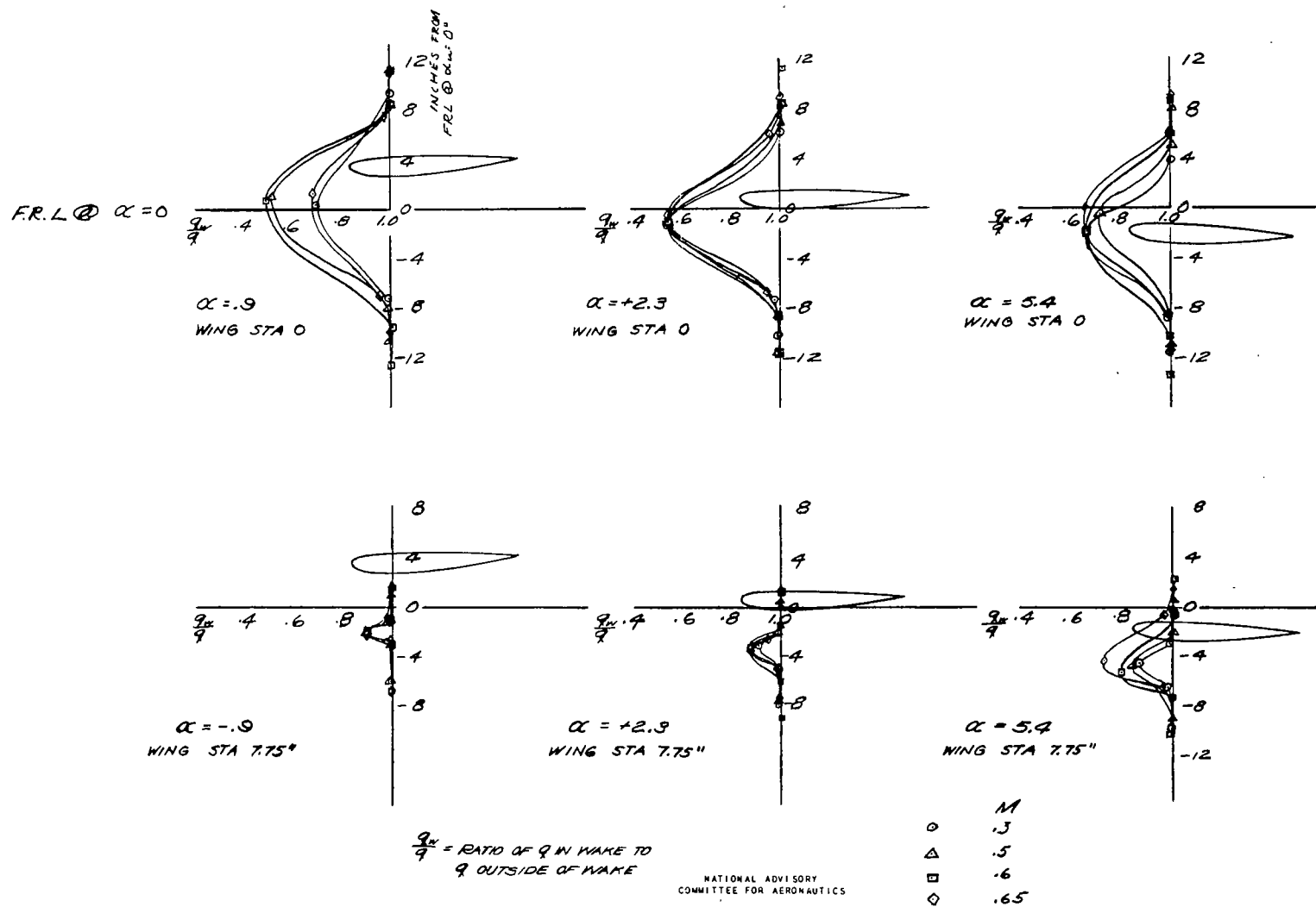
Figure 25.- Wake position at tail; 66 wing, large booms, fuselage, all accessories.
