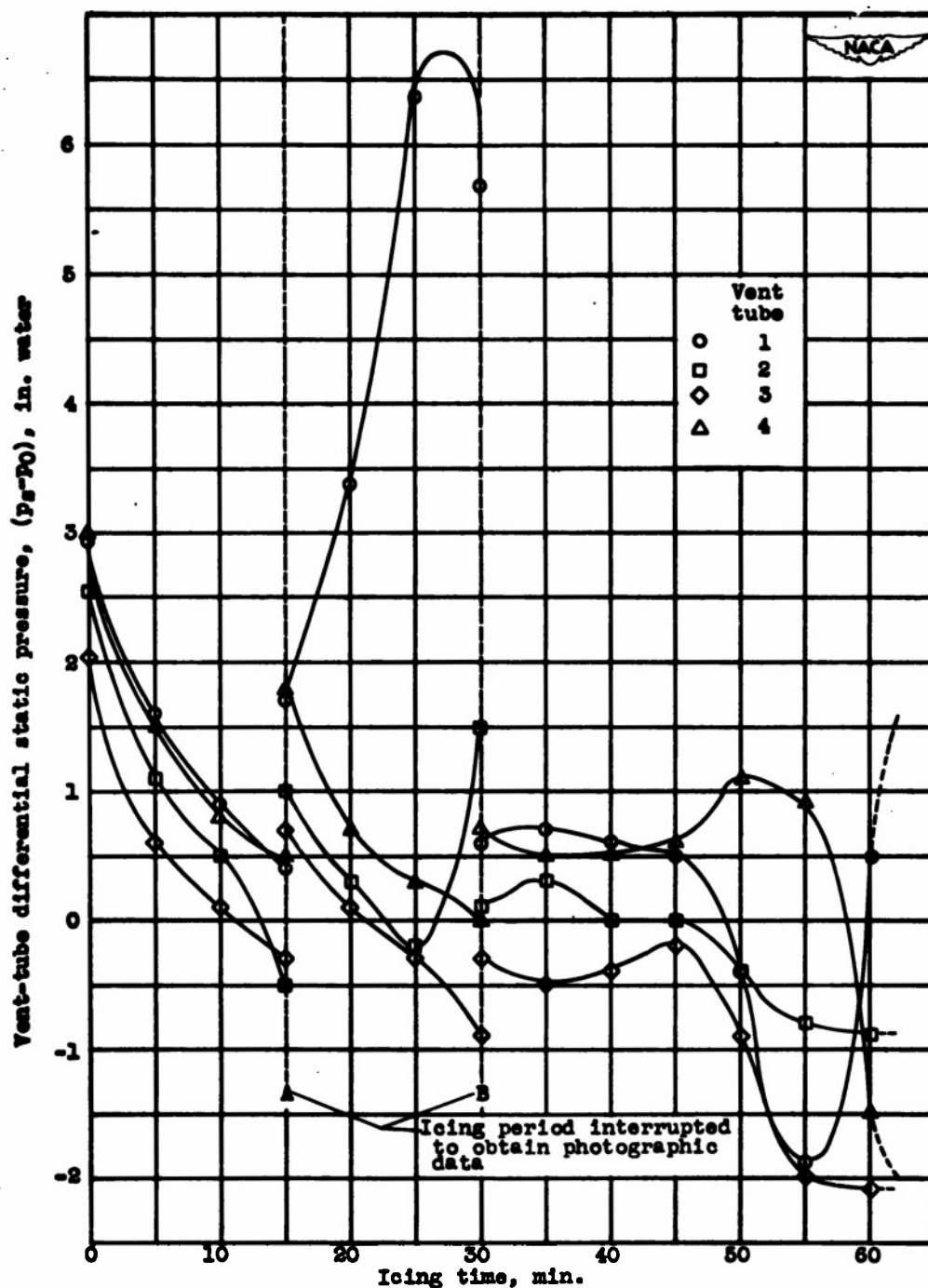
Figure 6. - Variation of vent-tube differential static pressure with icing time for 62-minute icing period. Tunnel-air velocity, 220 feet per second; angle of attack, 14^\circ ; ambient-air temperature, 23^\circ F; liquid-water content, 1.5 grams per cubic meter.
