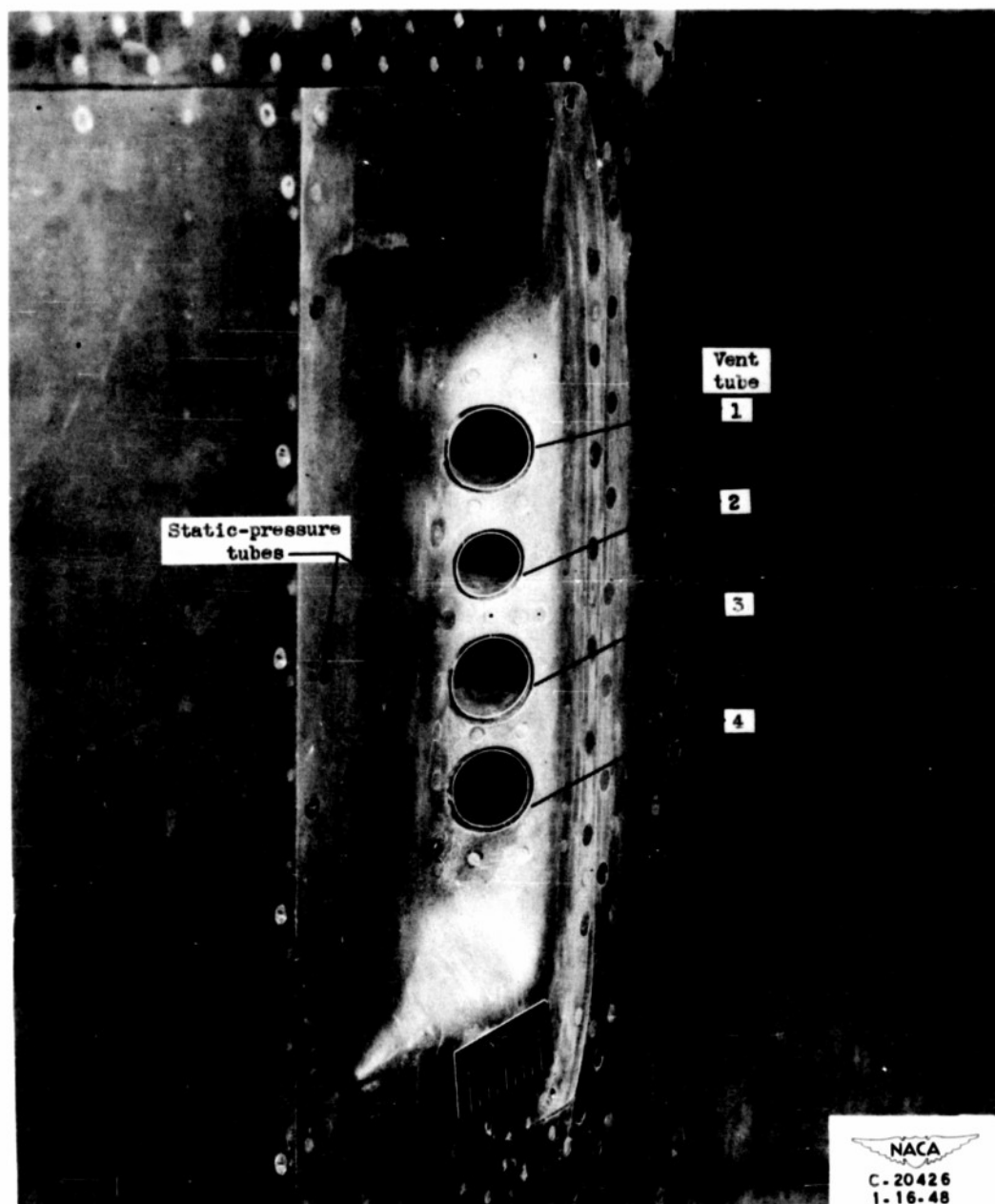
(b) Close-up view of vent installation.
