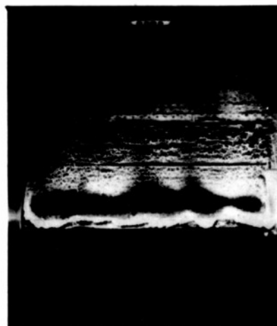
Figure 5. - Photographs of ice on airfoil and at vent recess. Tunnel-air velocity, 220 feet per second; angle of attack, 14°; ambient-air temperature, 230 F; liquid water content, 1.5 grams per cubic meter.
