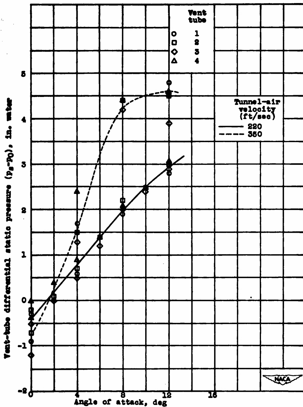
Figure 4. - Variation of vent-tube differential static pressure with angle of attack. No vent air flow.
