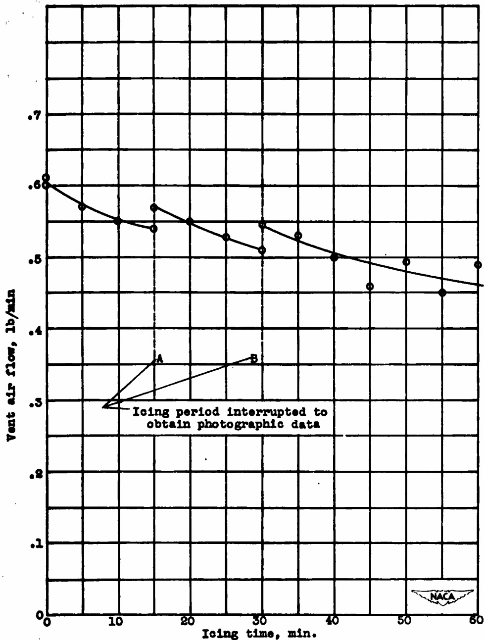
Figure 7. - Variation of typical vent air flow (vent tube 3) with icing time for 62-minute icing period. Tunnel-air velocity, 220 feet per second; angle of attack, 14°; ambient-air temperature, 23° F; liquid-water content, 1.5 grams per cubic meter.
