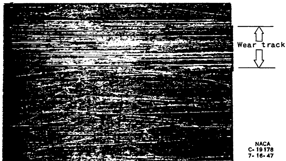
(c) Surface of steel disk specimen showing wear track formed by spherical rider and an adjacent unrun surface with random finish. Load, 269 grams. X18.
