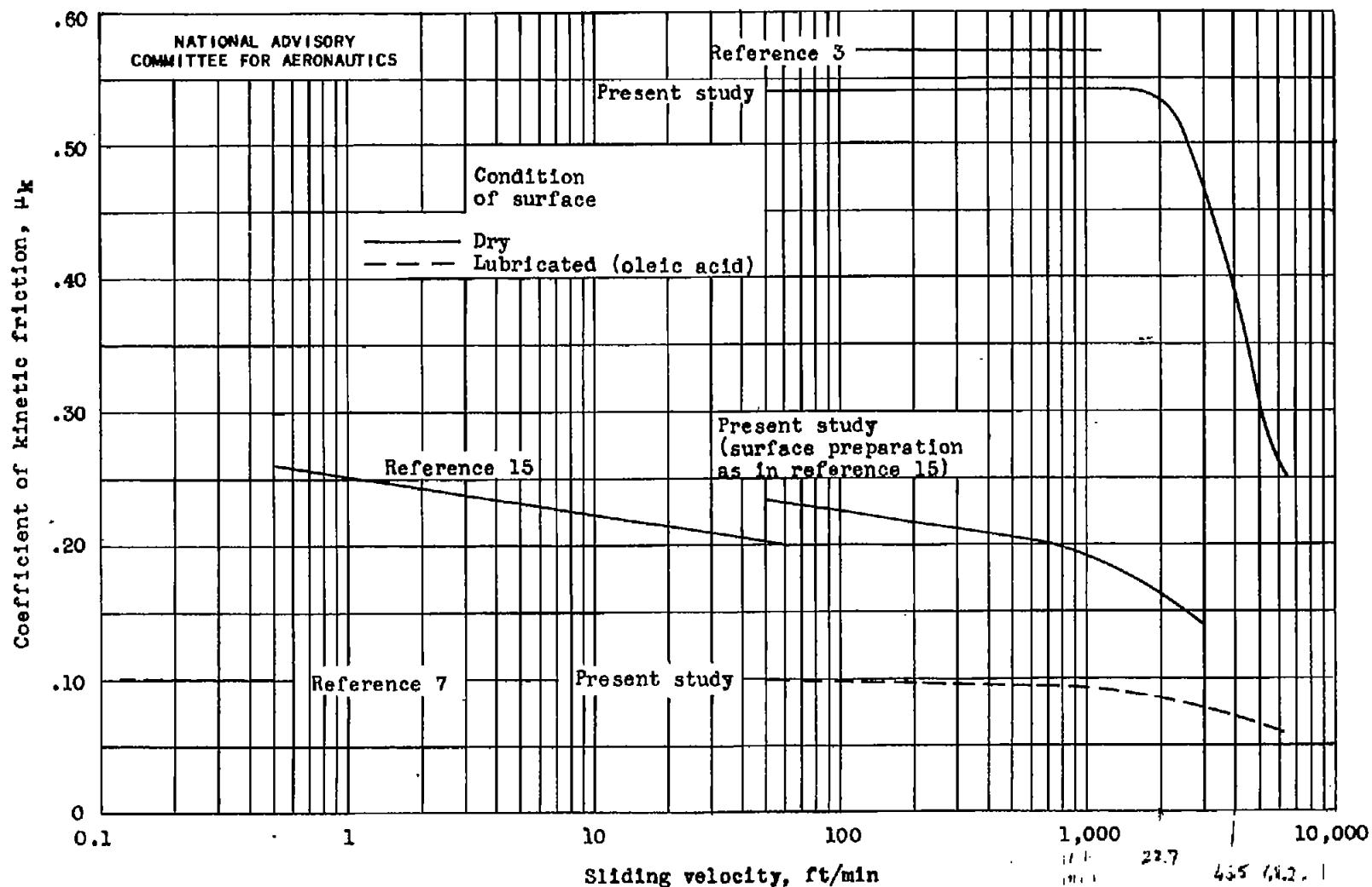
Figure 7. - Comparison of data from present study with that of other investigations.
