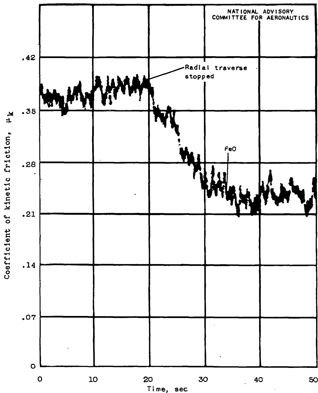
Figure 12. - Recording-potentiometer data showing effect of high-velocity sliding over a continuous path (without radial traverse) on coefficient of kinetic friction. Ferrous oxide (FeO) was visibly present as the decreasing friction trend began to stabilize. Dry steel; load, 269 grams; sliding velocity, 4000 feet per minute.
