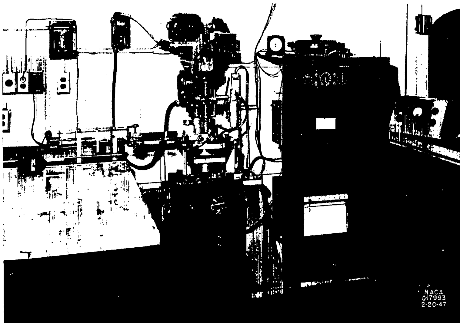
Figure 2. - Sliding-friction apparatus used for friction and wear studies.
