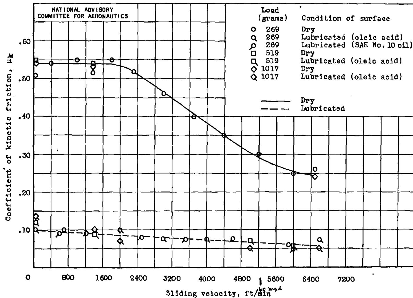
Figure 5. - Effect of sliding velocity on coefficient of kinetic friction for dry and boundary-lubricated steel surfaces.
