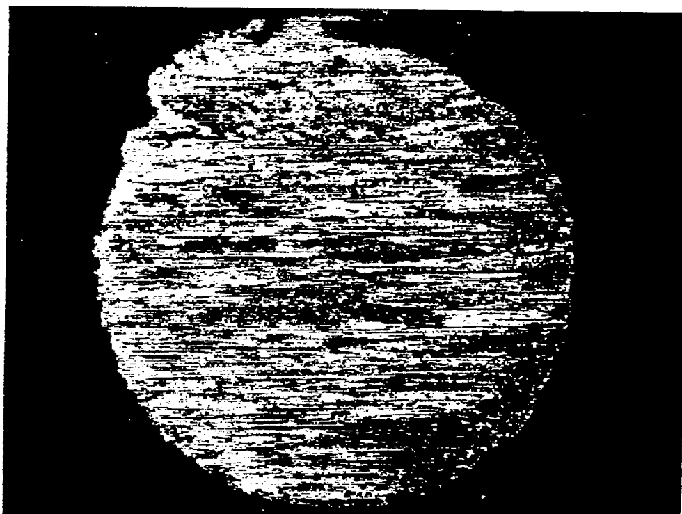
(a) Dry steel disk; coefficient of kinetic friction \mu_k , 0.48; wear-spot diameter, 0.96 millimeter (0.038 in.).
