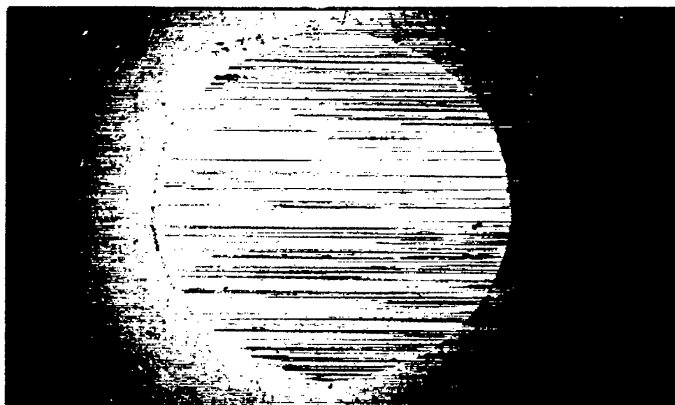
(b) Steel disk boundary-lubricated with oleic acid; coefficient of kinetic friction \mu_k , 0.10; wear-spot diameter, 0.71 millimeter (0.028 in.).
