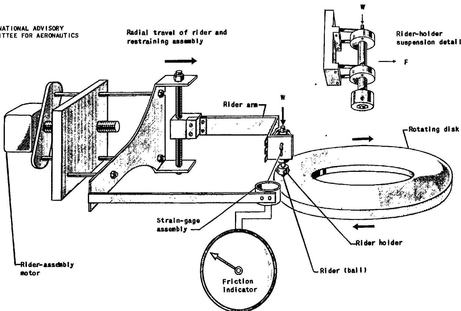
Figure 1. - Schematic diagram of sliding-friction apparatus.
