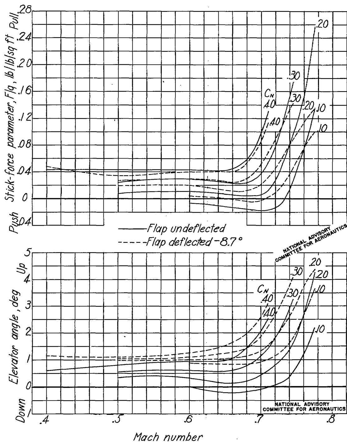
Figure 11.- Effect of negative flap deflection on the variation with Mach number of the elevator angle and the stick-force parameter, F_{lq} , required for balance. Airplane 2.
