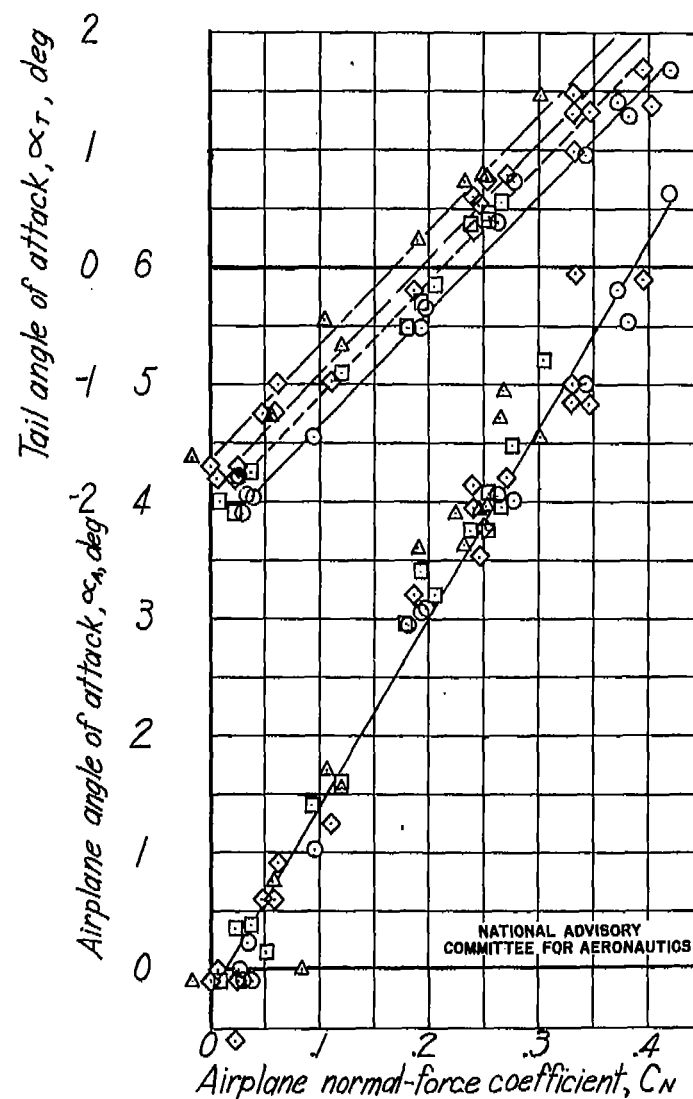
Figure 8.- Typical data from which resultant curves were obtained. Airplane 1. \delta_f = 0 M = .74-.76 .
