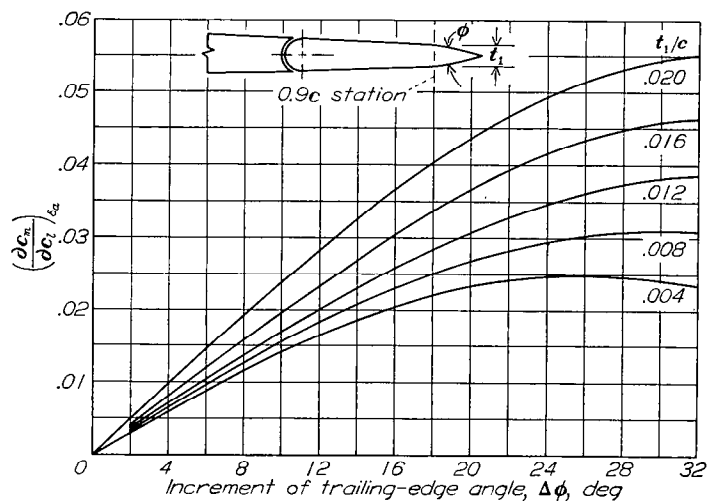
FIGURE 21.—Effect of trailing-edge modifications on the parameter \left(\frac{\partial c_m}{\partial \alpha}\right)_{s_a} . Reference 56.
