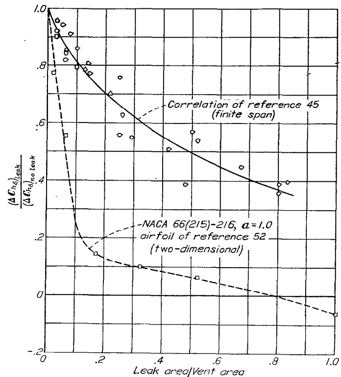
FIGURE 38.—Effect of leakage on the incremental hinge-moment slope \Delta C_{h\delta} caused by internal balances. Symbols identified in table IV.
