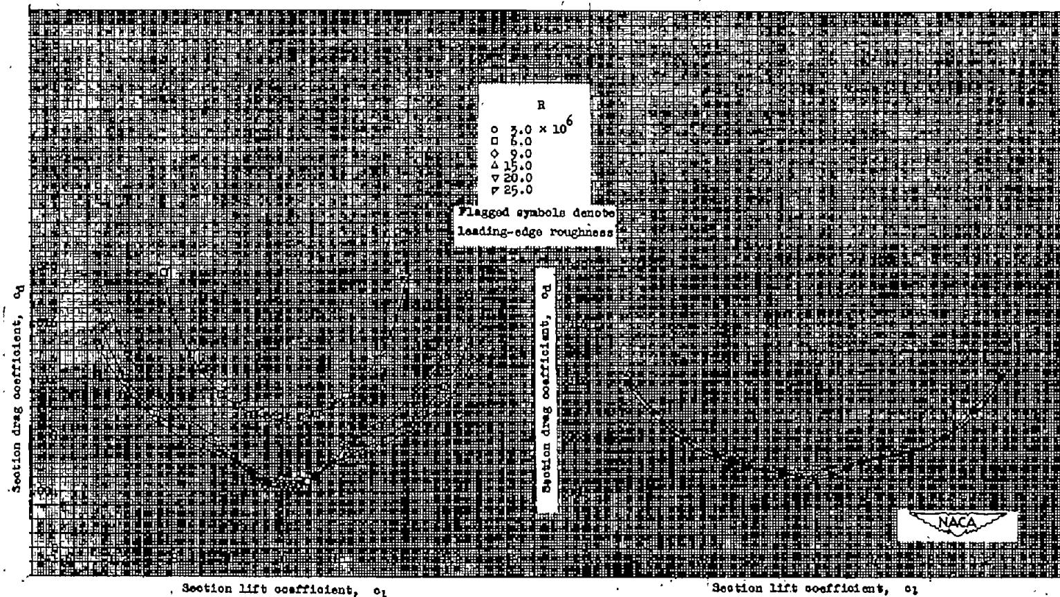
(b) Drag characteristics.
