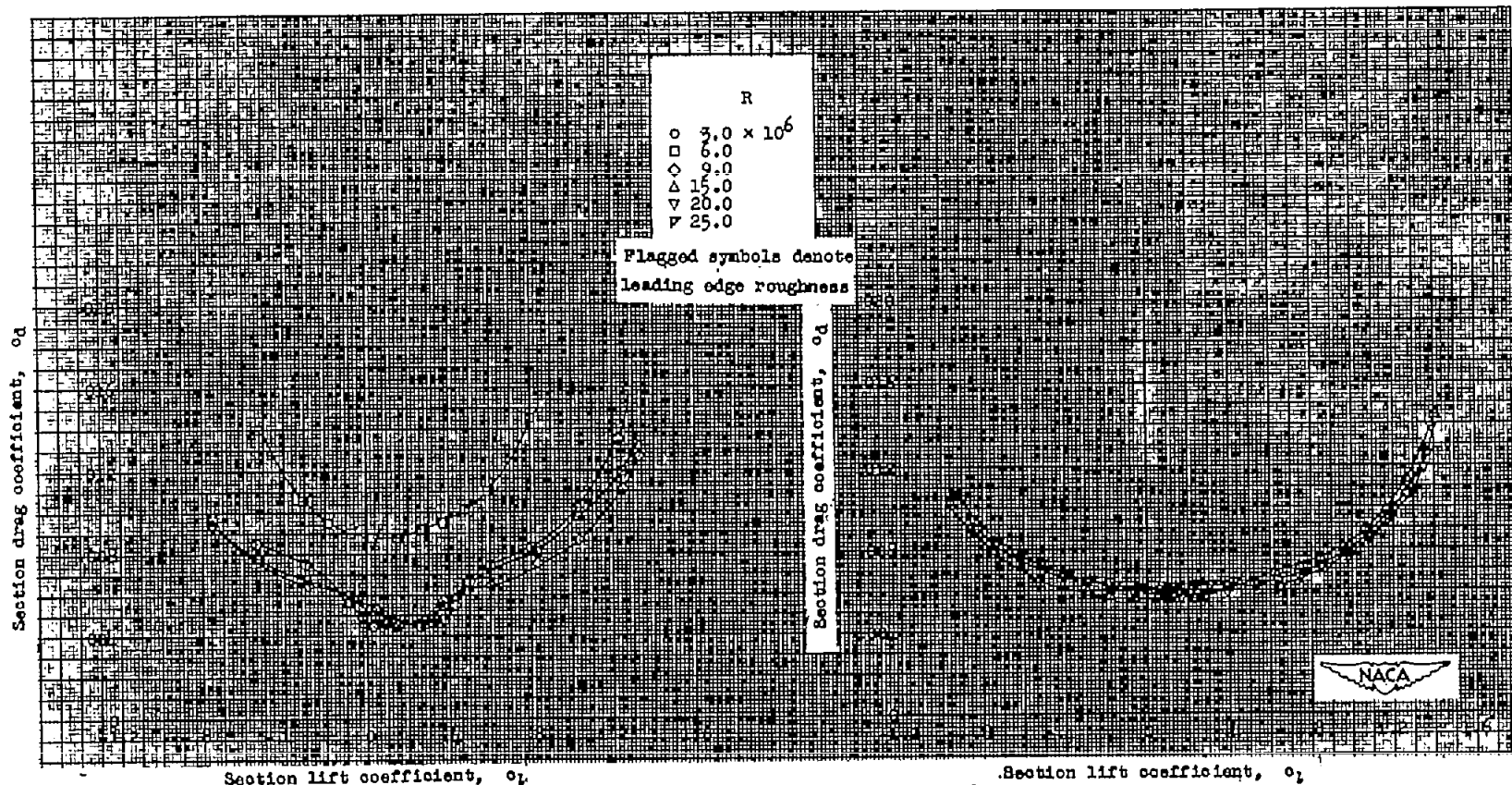
(b) Drag characteristics.
