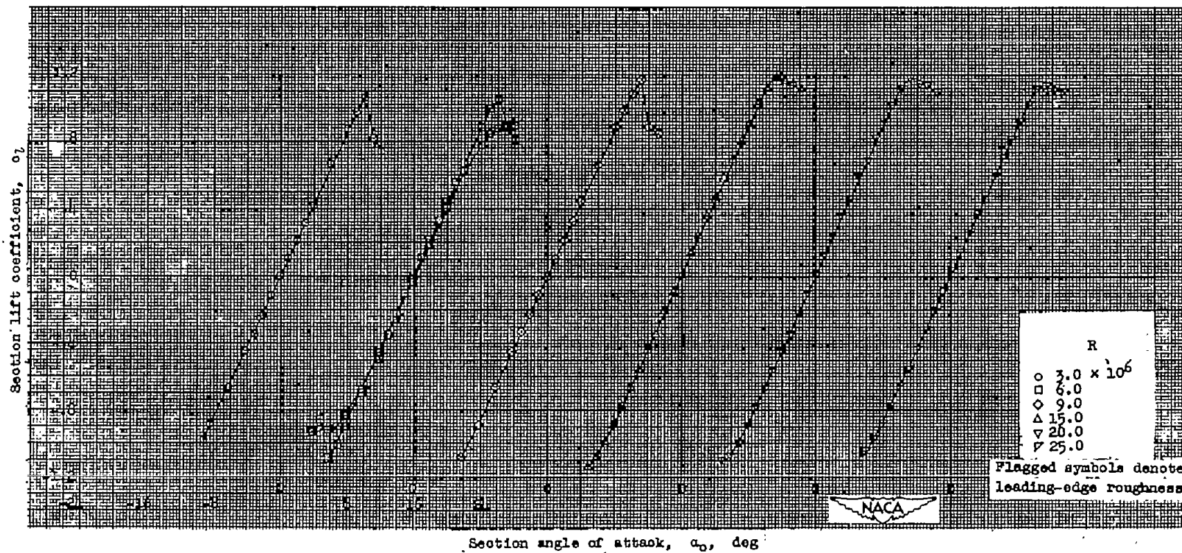
(a) Lift characteristics.
