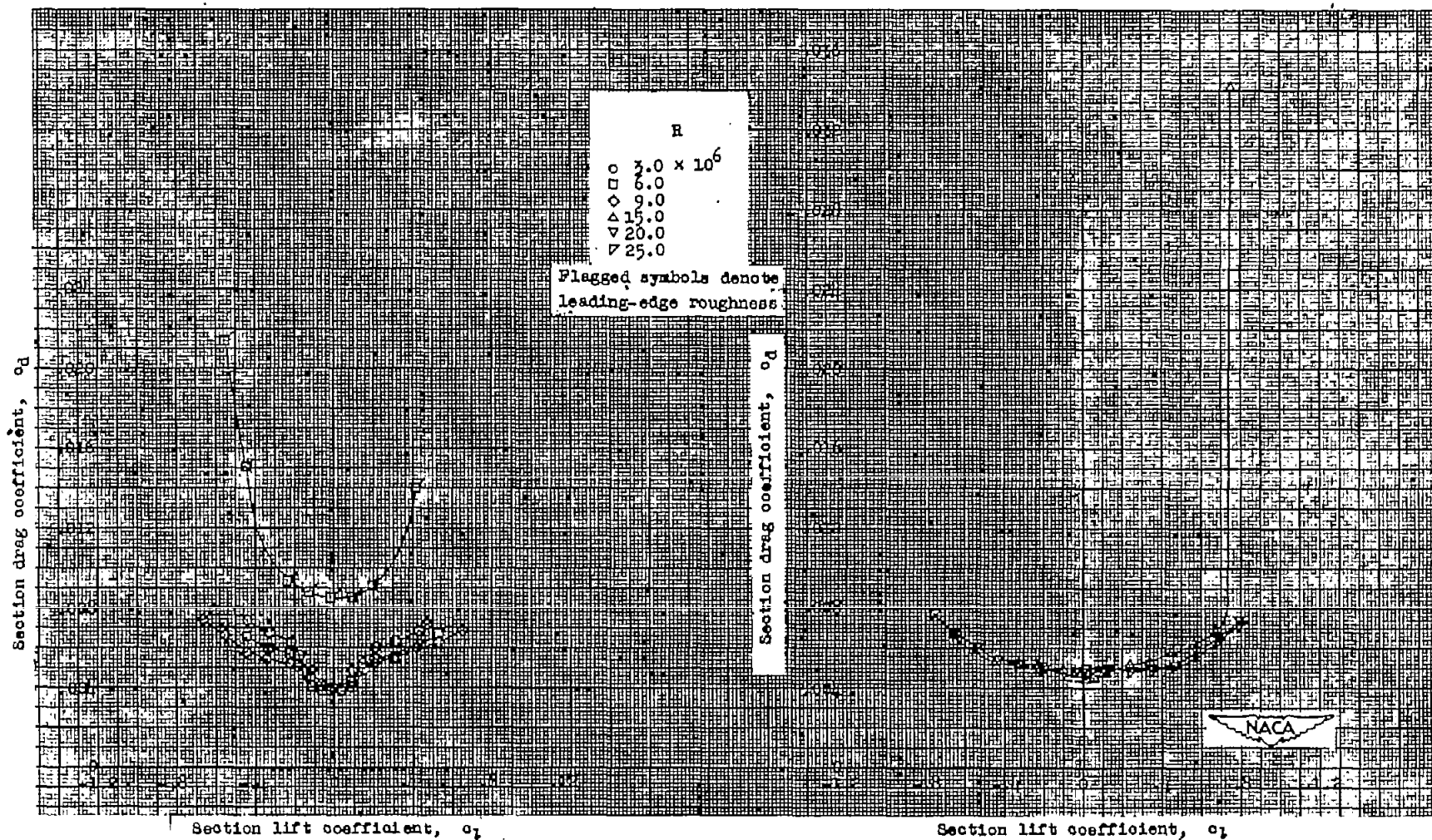
(b) Drag characteristics.
