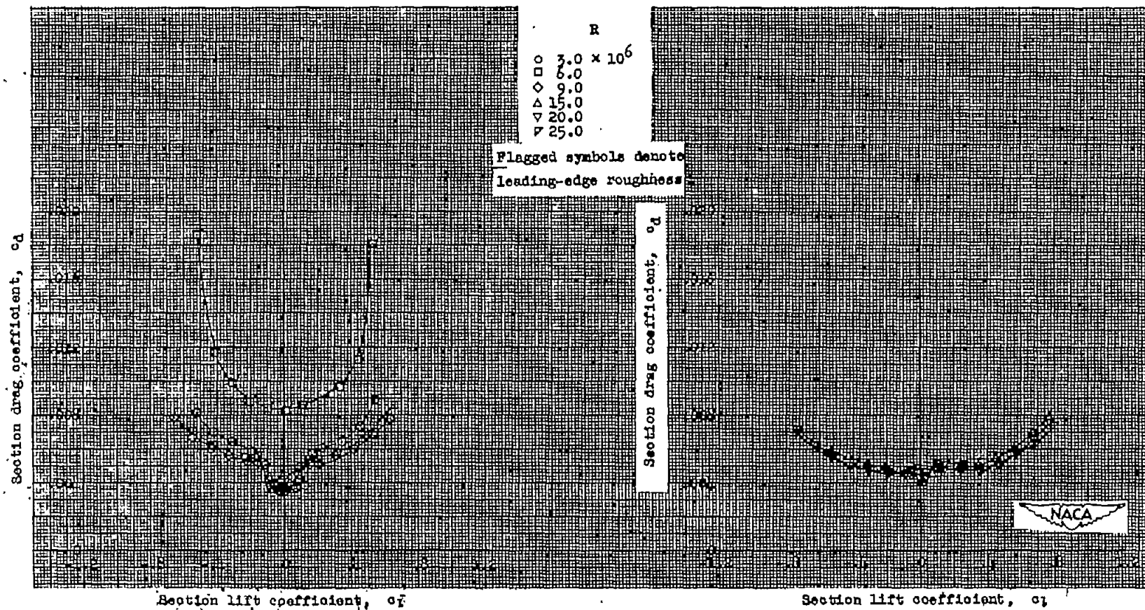
(b) Drag characteristics.
