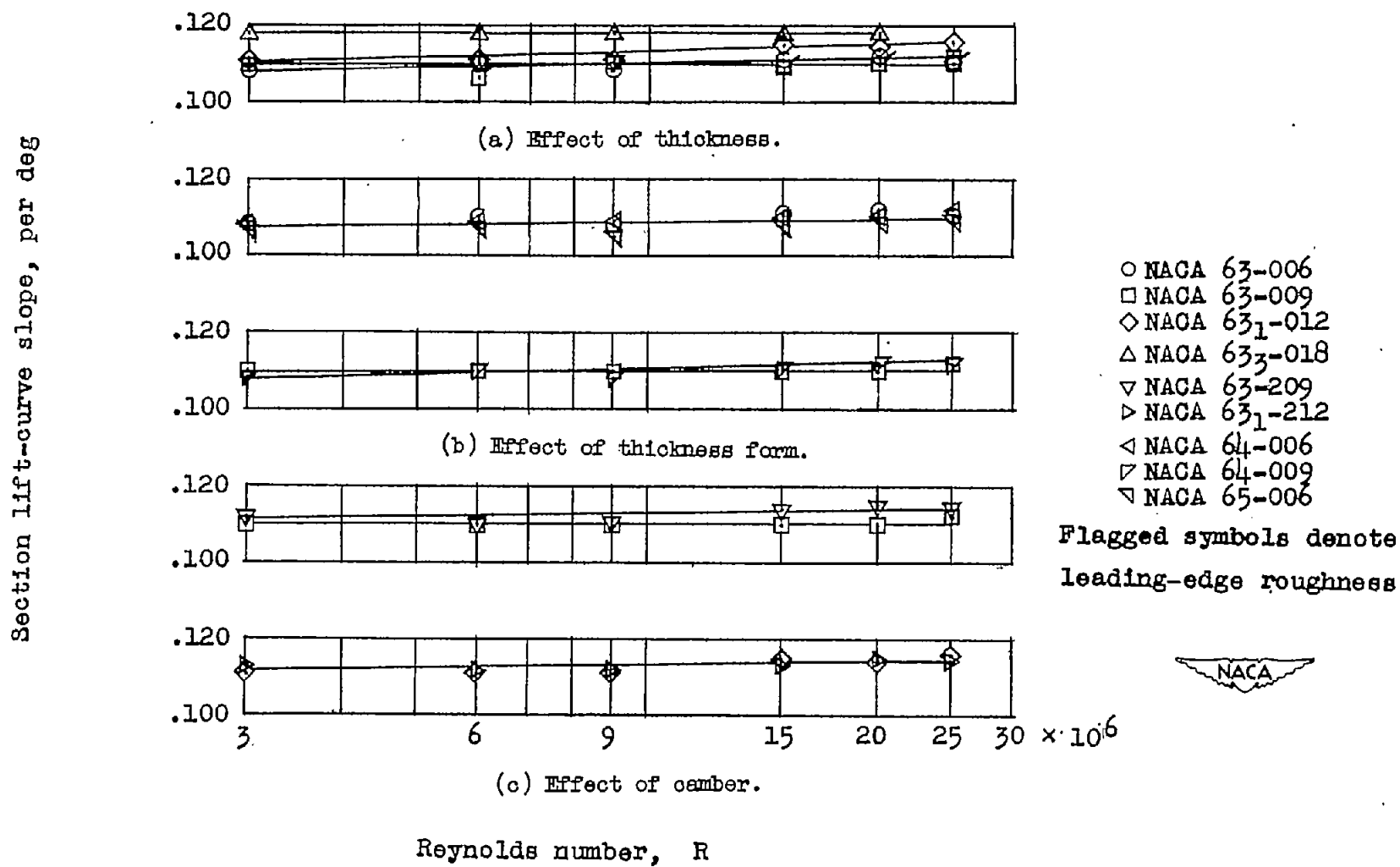
Figure 11.— Variation of section lift-curve slope with Reynolds number for nine NACA 6-series airfoils of varying thickness, thickness form, and camber.
