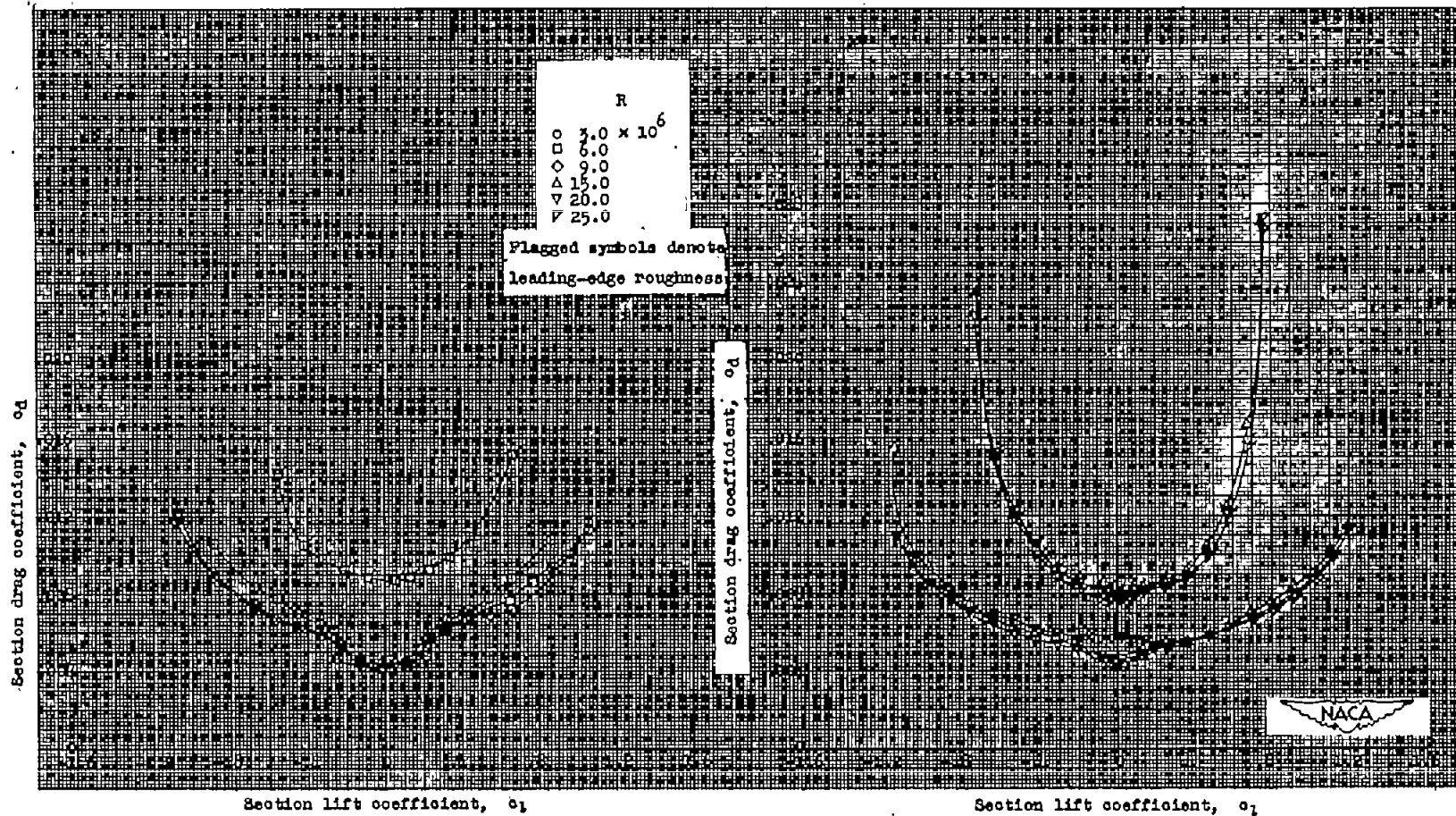
(c) Drag characteristics.
