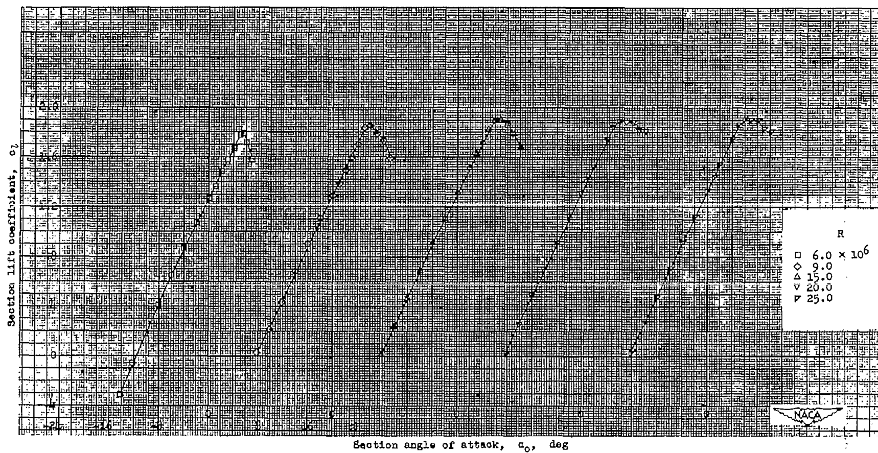
(b) Lift characteristics with 0.20c simulated split flap deflected 60^\circ .
