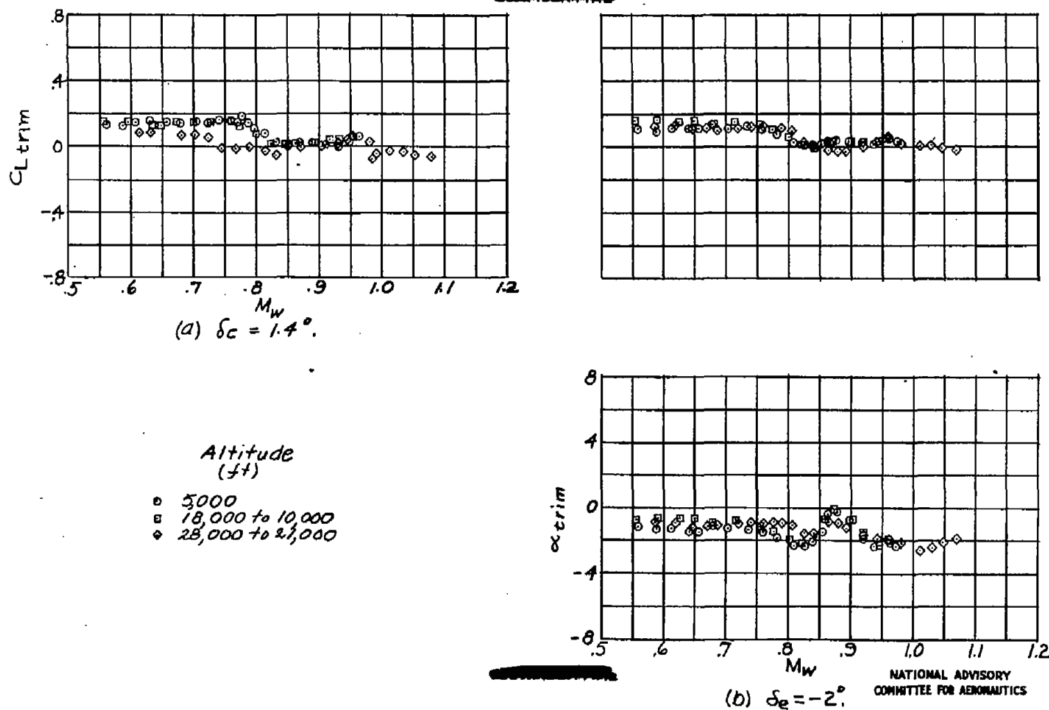
Figure 7.- Variation with Mach number of lift coefficient and angle of attack for trim with various elevator deflections and stabilizer set at 3.7^\circ . Angle of attack not determined for \delta_e = 1.4^\circ .
