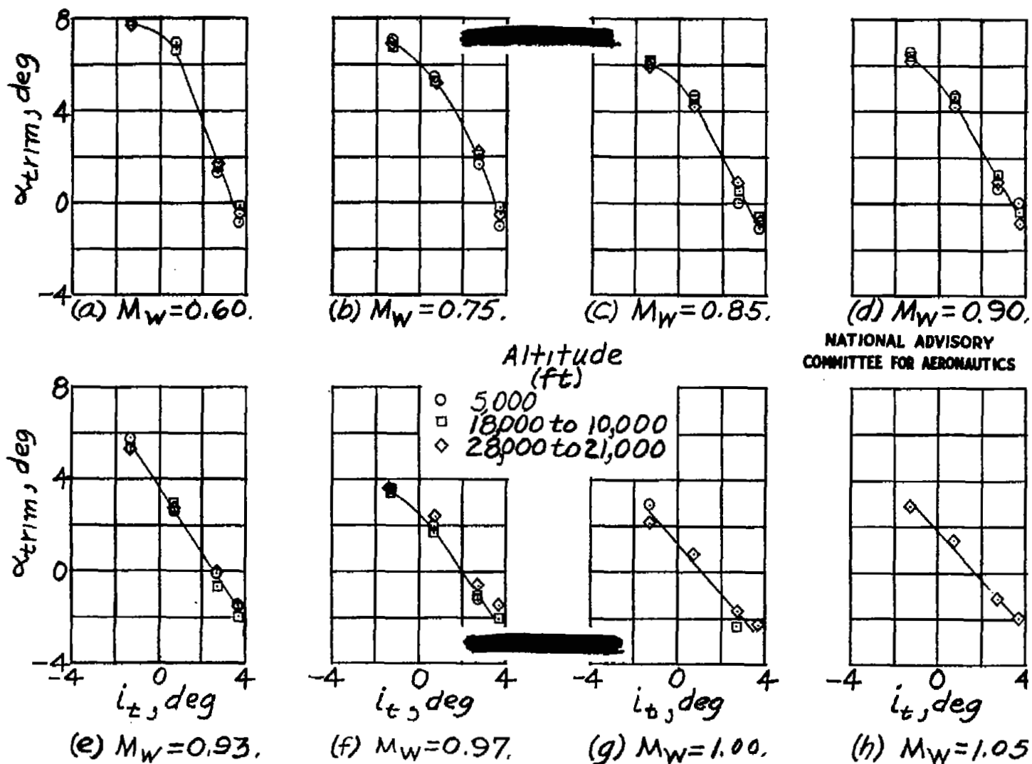
Figure 10.- Variation of angle of attack for trim with stabilizer setting for various Mach numbers. \delta_0 = 0 .
