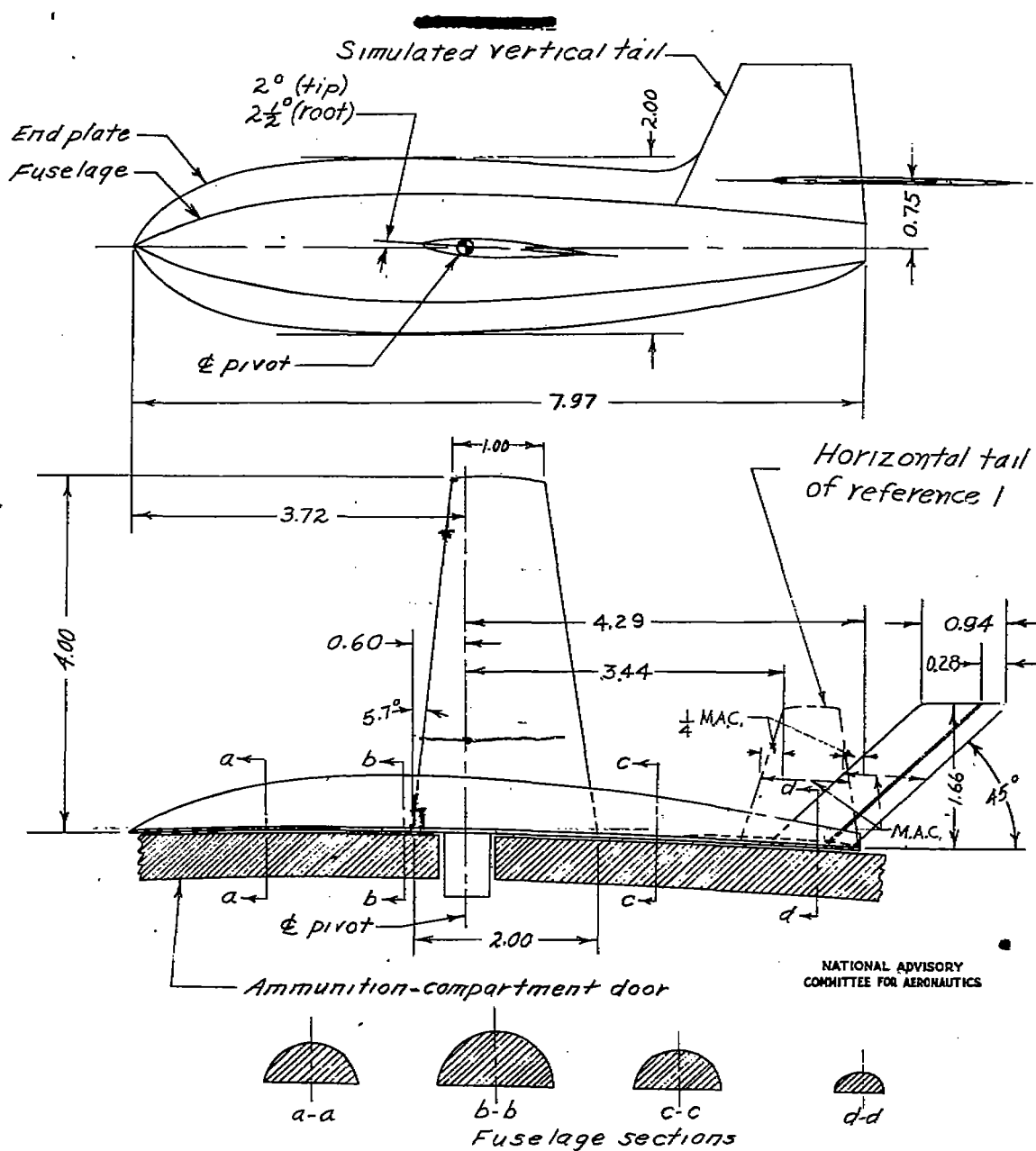
Figure 3.- Details of semispan airplane model. All dimensions are in inches.
