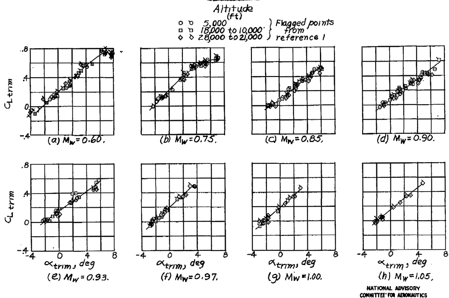
Figure 8.- Variation of lift coefficient with angle of attack for various Mach numbers.
