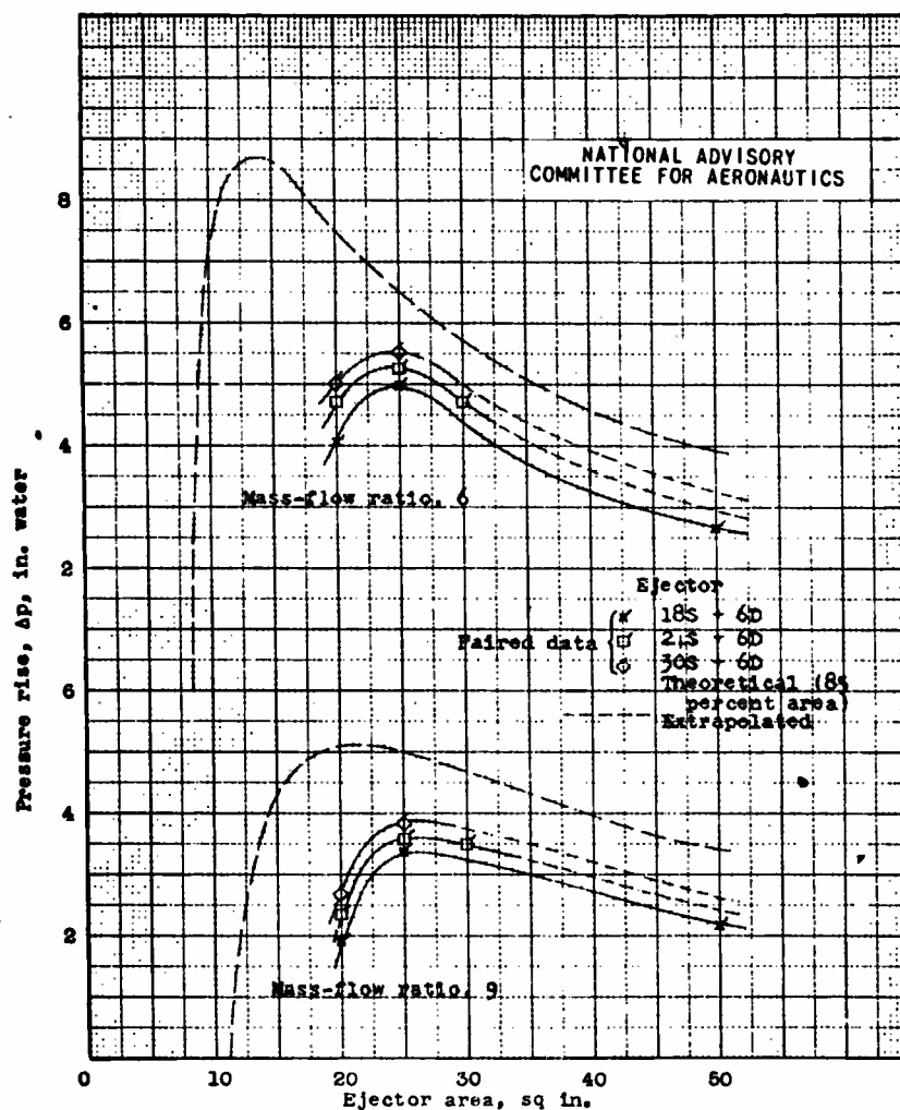
Figure 11.- Variation of pressure rise with ejector area for 6-inch diffuser ejectors actuated by exhaust of single-cylinder 1820-G engine. Aspect ratio, 3; exhaust-gas mass-flow rate, 8 pounds per minute; exhaust-nozzle area, 2.6 square inches; fuel-air ratio, 0.08; indicated horsepower, 85.
