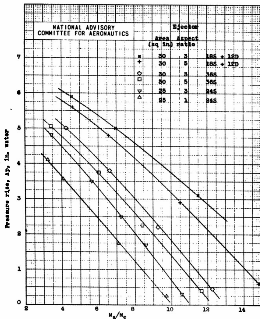
Figure 15.- Effect of mixing-section aspect ratio on performance of ejectors actuated by exhaust of single-cylinder 1820-G engine. Exhaust-gas mass-flow rate, 8 pounds per minute; exhaust-nozzle area, 2.6 square inches; fuel-air ratio, 0.08; indicated horsepower, 85. For further details see table I.
