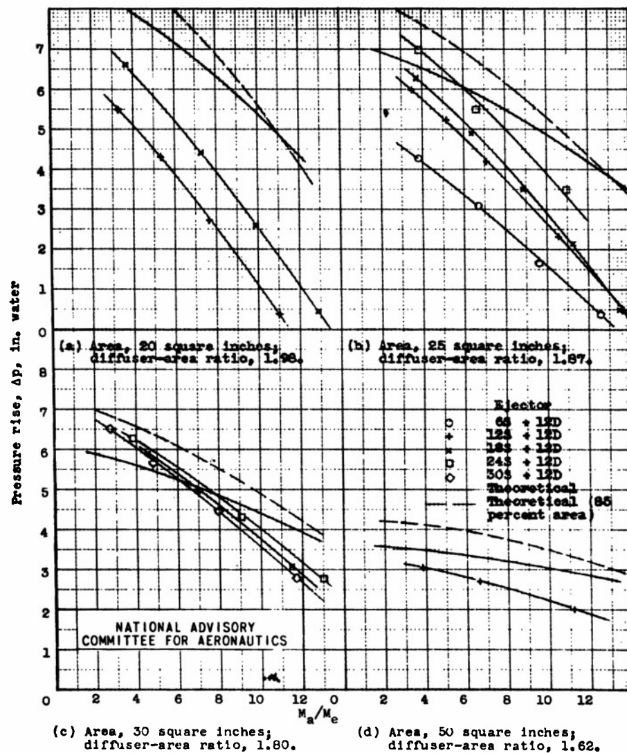
Figure 8.- Performance curves for 12-inch diffuser ejectors actuated by exhaust of single-cylinder 1820-G engine. Aspect ratio, 3; exhaust-gas mass-flow rate, 8 pounds per minute; exhaust-nozzle area 2.6 square inches; fuel-air ratio, 0.08; indicated horsepower, 85. For further details see table I.
