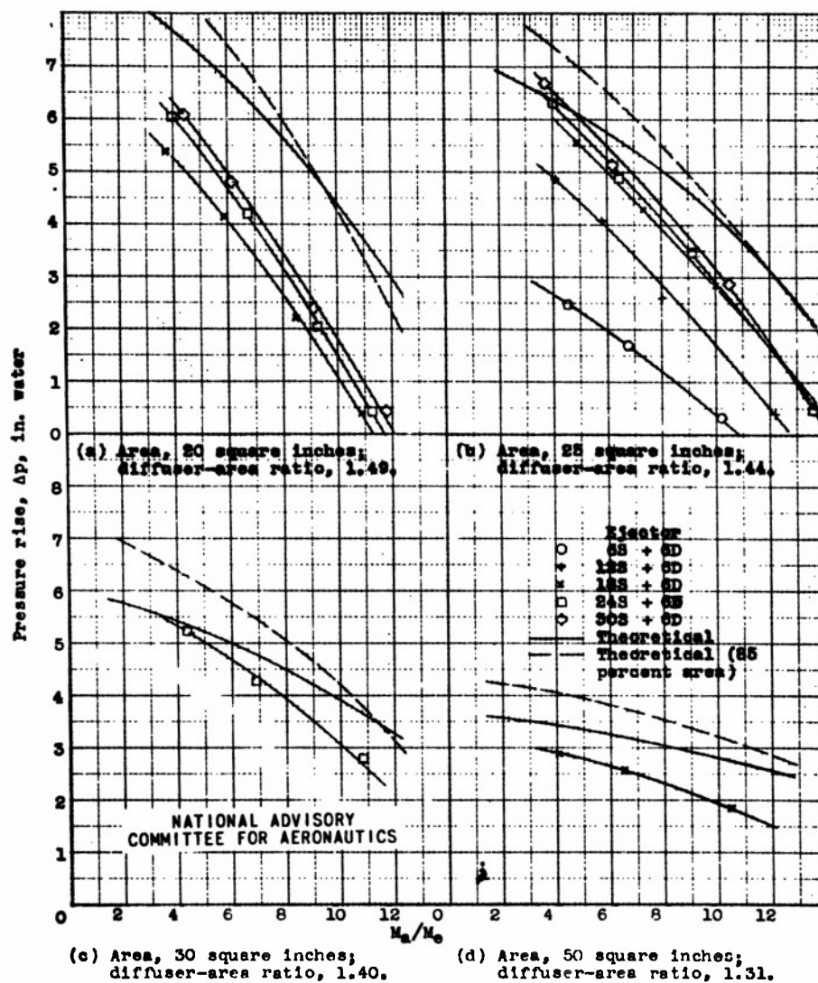
Figure 7.- Performance curves for 6-inch diffuser ejectors actuated by exhaust of single-cylinder 1820-G engine. Aspect ratio, 3; exhaust-gas mass-flow rate, 8 pound per minute; exhaust-nozzle area, 2.6 square inches; fuel-air ratio, 0.08; indicated horsepower, 85. For further details see table I.
