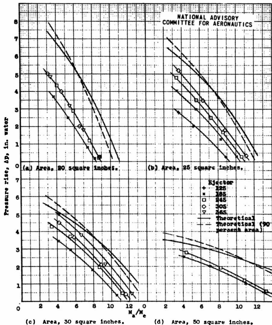
Figure 4.- Performance curves for straight ejectors actuated by exhaust of single-cylinder 1820-G engine. Aspect ratio, 3; exhaust-gas mass-flow rate, 8 pounds per minute; exhaust-nozzle area, 2.6 square inches; fuel-air ratio, 0.08; indicated horsepower, 85. For further details see table I.
