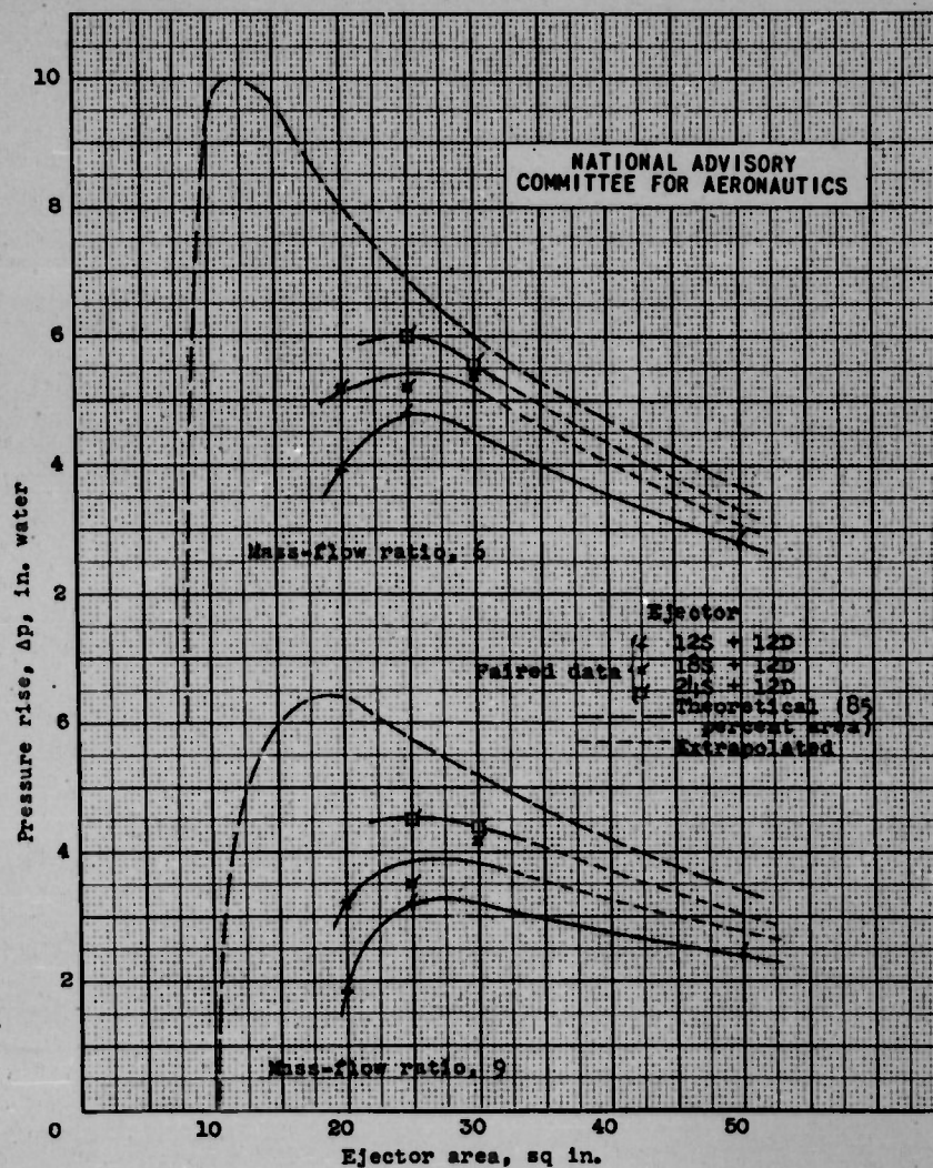
Figure 12.- Variation of pressure rise with ejector area for 12-inch diffuser ejectors actuated by exhaust of single-cylinder 1820-C engine. Aspect ratio, 3; exhaust-gas mass-flow rate, 8 pounds per minute; exhaust-nozzle area, 2.6 square inches; fuel-air ratio, 0.08; indicated horsepower, 85.
