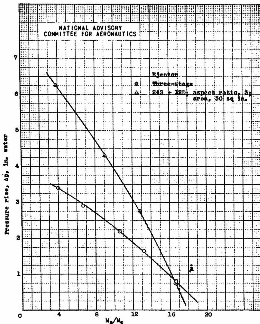
Figure 17.- Performance curves for a multistage ejector actuated by exhaust of single-cylinder 1820-C engine. Exhaust-gas mass-flow rate, 8 pounds per minute; exhaust-nozzle area, 2.6 square inches; fuel-air ratio, 0.08; indicated horsepower, 85. For further details see table II.
