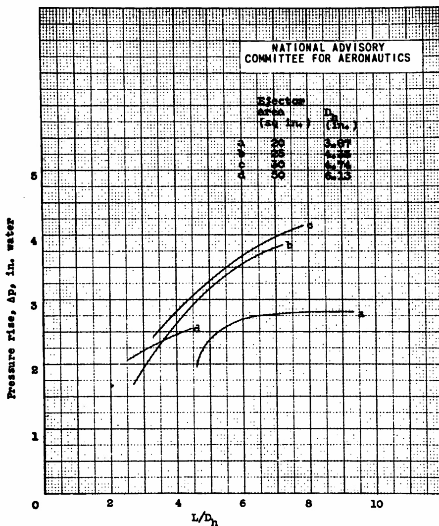
Figure 5 - Variation of pressure rise with length-hydraulic diameter ratio for straight ejectors actuated by exhaust of single-cylinder 1820-G engine. Aspect ratio, 3; exhaust-gas mass-flow rate, 8 pounds per minute; exhaust-nozzle area, 2.6 square inches; fuel-air ratio, 0.08; indicated horsepower, 85; mass-flow ratio, 6.
