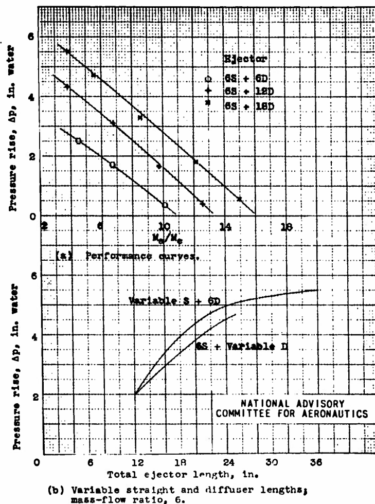
Figure 9.- Effect of incremental straight and diffuser length on performance of ejectors actuated by exhaust of single-cylinder 1820-G engine. Area, 25 square inches; ejector aspect ratio, 3; exhaust-gas mass-flow rate, 8 pounds per minute; exhaust-nozzle area, 2.6 square inches; exhaust-nozzle-exit aspect ratio, 12; fuel-air ratio, 0.08; indicated horsepower, 85. For further details see table I.
