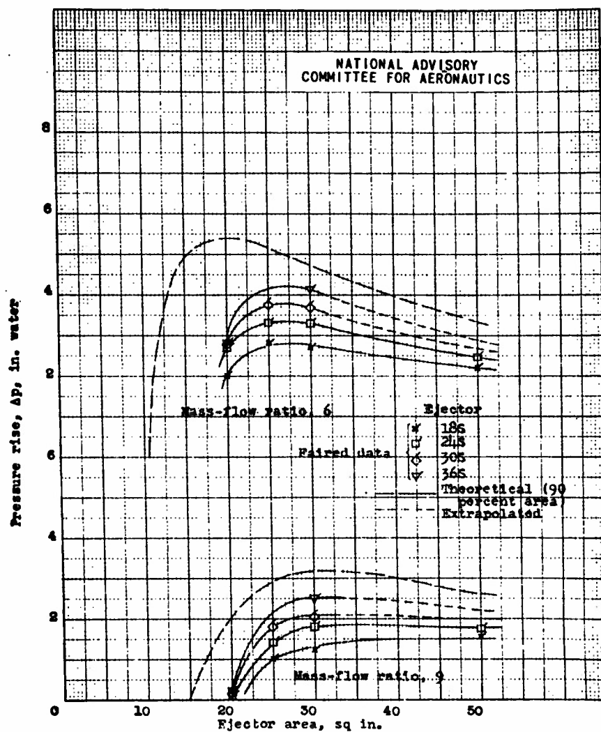
Figure 6.- Variation of pressure rise with ejector area for straight ejectors actuated by exhaust of single-cylinder 1820-G engine. Aspect ratio, 3; exhaust-gas mass-flow rate, 8 pounds per minute; exhaust-nozzle area, 2.6 square inches; fuel-air ratio, 0.08; indicated horsepower, 85.
