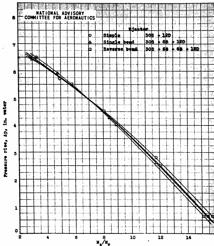
Figure 14.- Performance curves for curved ejectors actuated by exhaust of single-cylinder 1820-G engine. Area, 30 square inches; aspect ratio, 3; exhaust-gas mass-flow rate, 8 pounds per minute; exhaust-nozzle area, 2.6 square inches; fuel-air ratio, 0.08; indicated horsepower, 85. For further details see table II.
