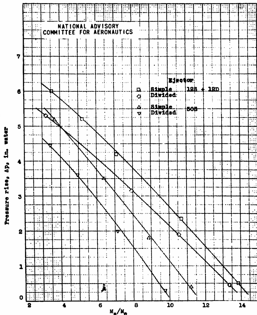
Figure 16.- Performance curves for divided ejectors actuated by exhaust of single-cylinder 1820-G engine. Area, 25 square inches; aspect ratio, 3; exhaust-gas mass-flow rate, 8 pounds per minute; exhaust-nozzle area, 2.6 square inches; fuel-air ratio, 0.08; indicated horsepower, 85. For further details see table II.
