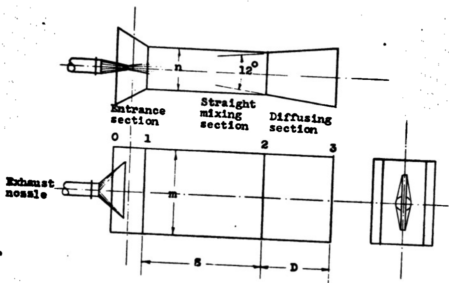
Figure 3.- Ejector details and terminology.
