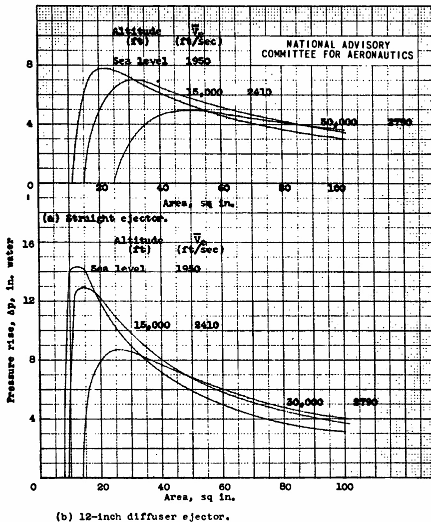
Figure 20.- Theoretical variation of pressure rise with ejector area at various altitudes. Mass-flow ratio, 6; exhaust-gas mass-flow rate, 12 pounds per minute; exhaust-gas temperature, 1500° F; air temperature, 75° F; exhaust-nozzle area, 2.6 square inches.
