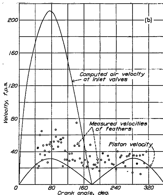
(b) Engine speed, 1,000 r. p. m.
