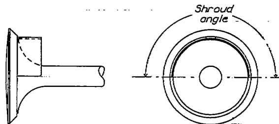
FIGURE 3.—Sketch of shrouded intake valve.
