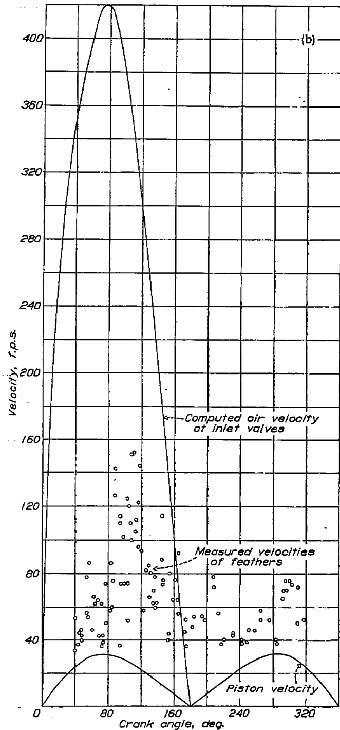
(b) Engine speed, 1,000 r. p. m.
