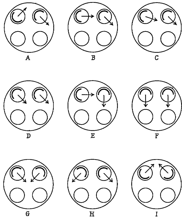
FIGURE 7.—Arrangements of the shrouded intake valves.
