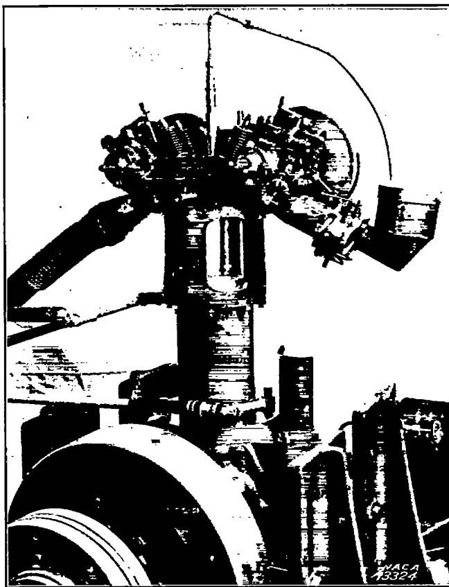
FIGURE 1.—Test engine with glass cylinder.
