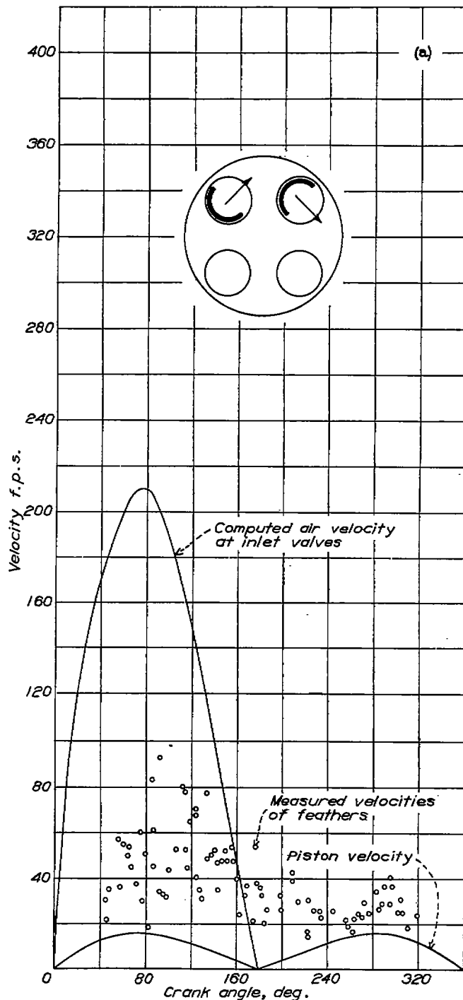
(a) Engine speed, 500 r. p. m.
