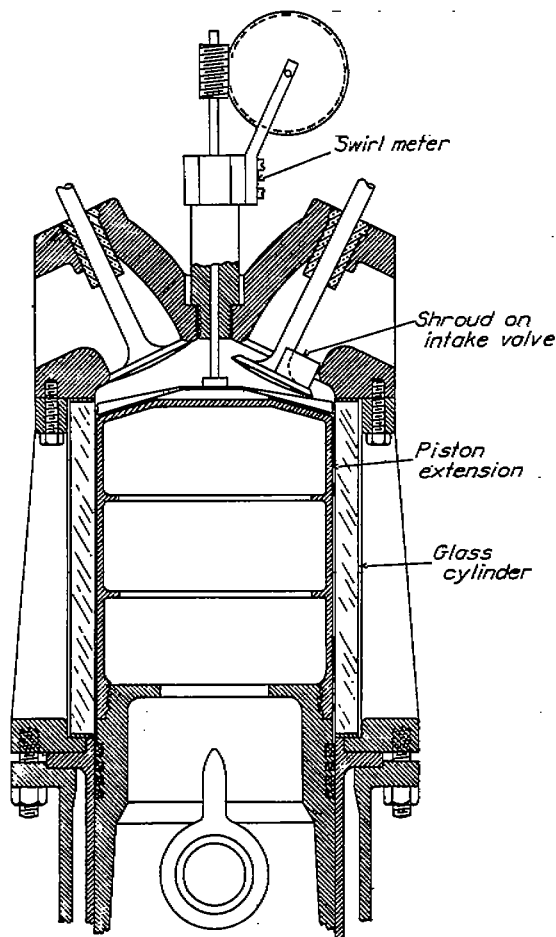
FIGURE 2.—Sketch showing glass cylinder and cylinder head.
