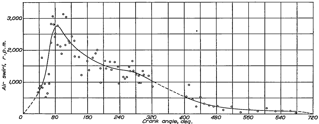
FIGURE 14.—Air swirl created by altering shape of intake-air passage. Engine speed, 500 r. p. m.
