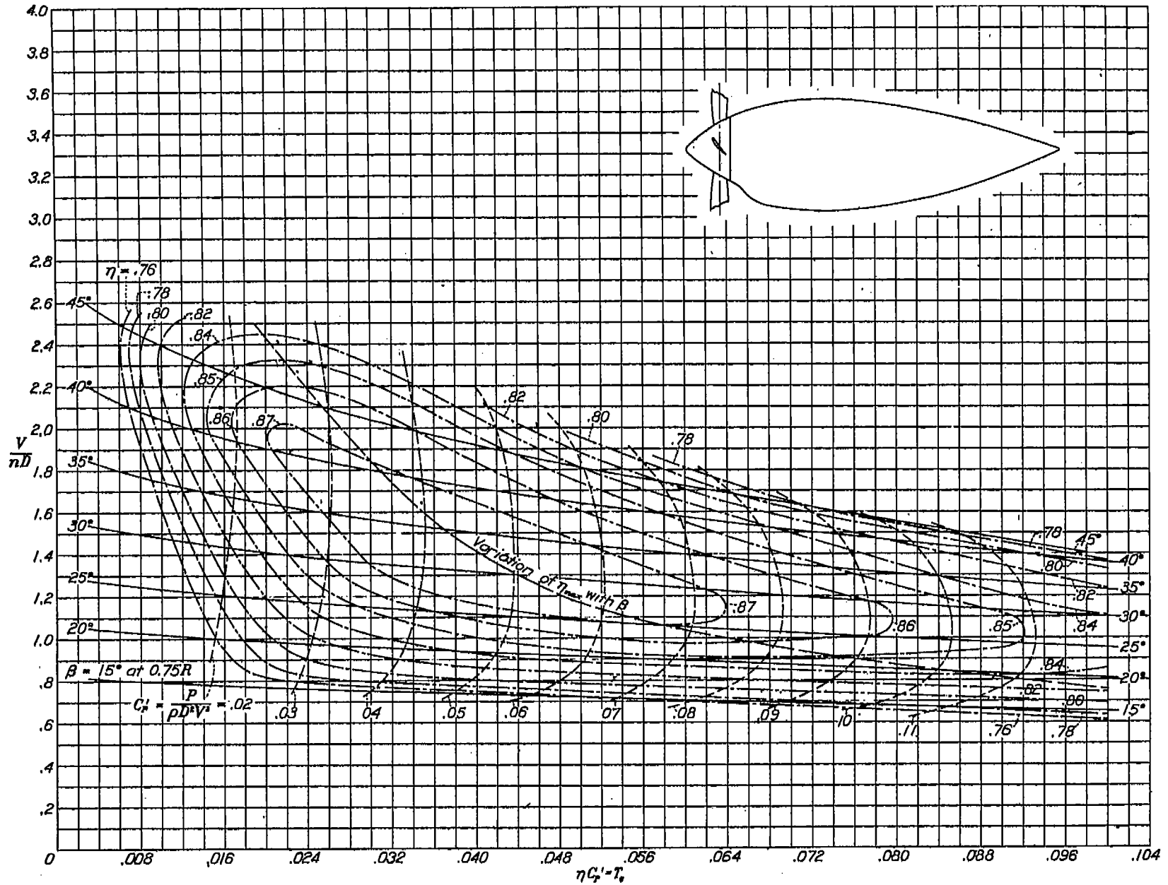
FIGURE 16.—Chart of V/nD against T_1 for four-blade propeller 5862-9. Liquid-cooled engine nacelle, with spinner; single rotation. Data taken from reference 5.
