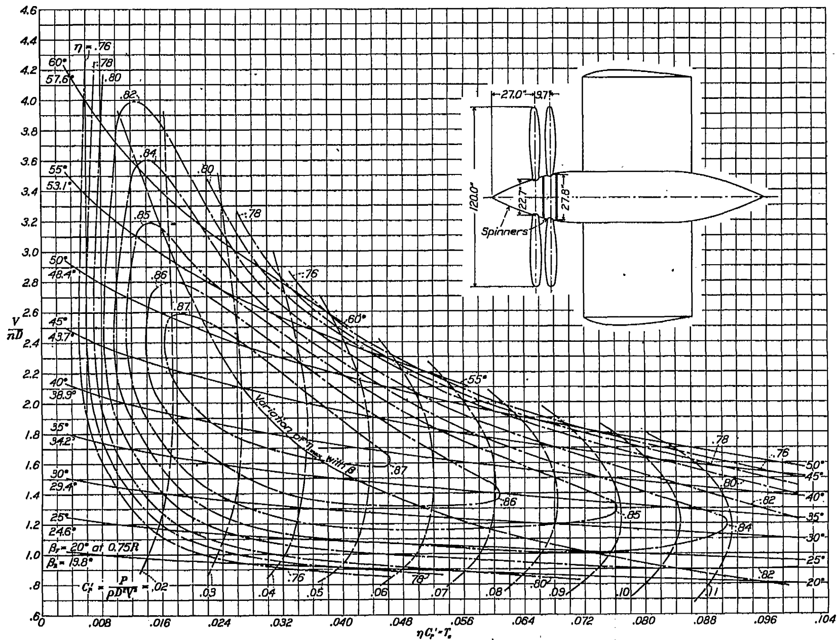
FIGURE 9.—Chart of V/nD against T , for two two-blade propellers 8155-6 and 8156-6. Streamline body, with spinner, on symmetrical wing; dual rotation. Propeller data taken from reference 2.
