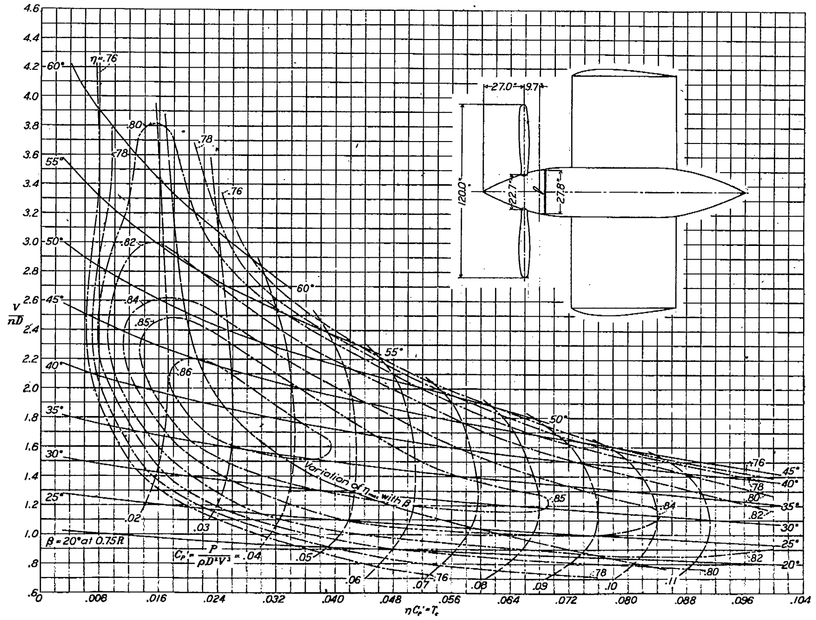
FIGURE 1.—Chart of V/nD against T_e for four-blade propeller 8185-6. Streamline body, with spinner, on symmetrical wing; single rotation. Propeller data taken from reference 2.
