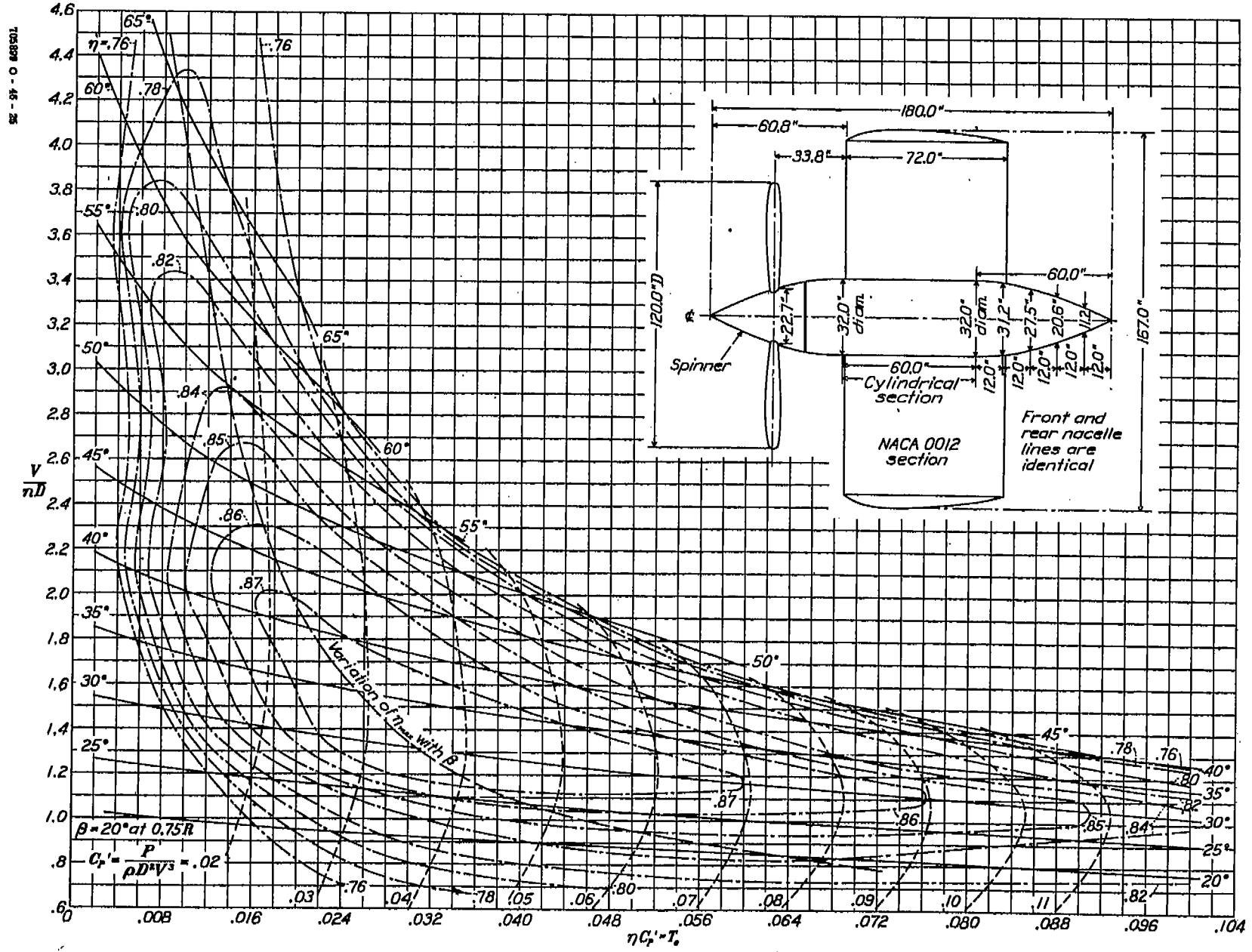
FIGURE 1.—Chart of V/nD against T_s for three-blade propeller 8165-6. Streamline body, with spinner, on symmetrical wing; single rotation. Propeller data taken from reference 1.
