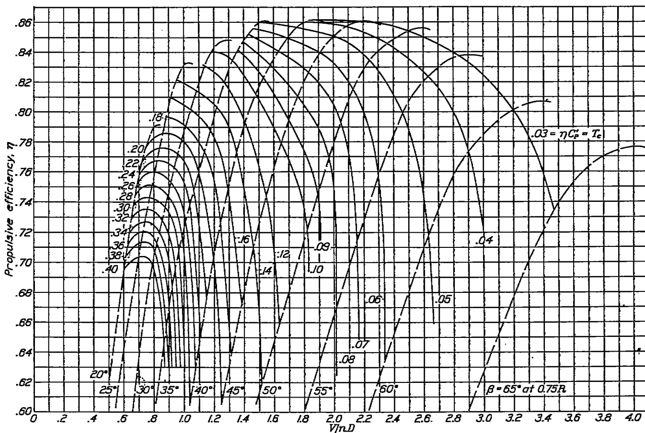
FIGURE 8.—Chart of \eta against V/nD for six-blade propeller 3155-6. Streamline body, with spinner, on symmetrical wing; single rotation. (The 60° efficiency curve was interpolated.) Propeller data taken from reference 2.
