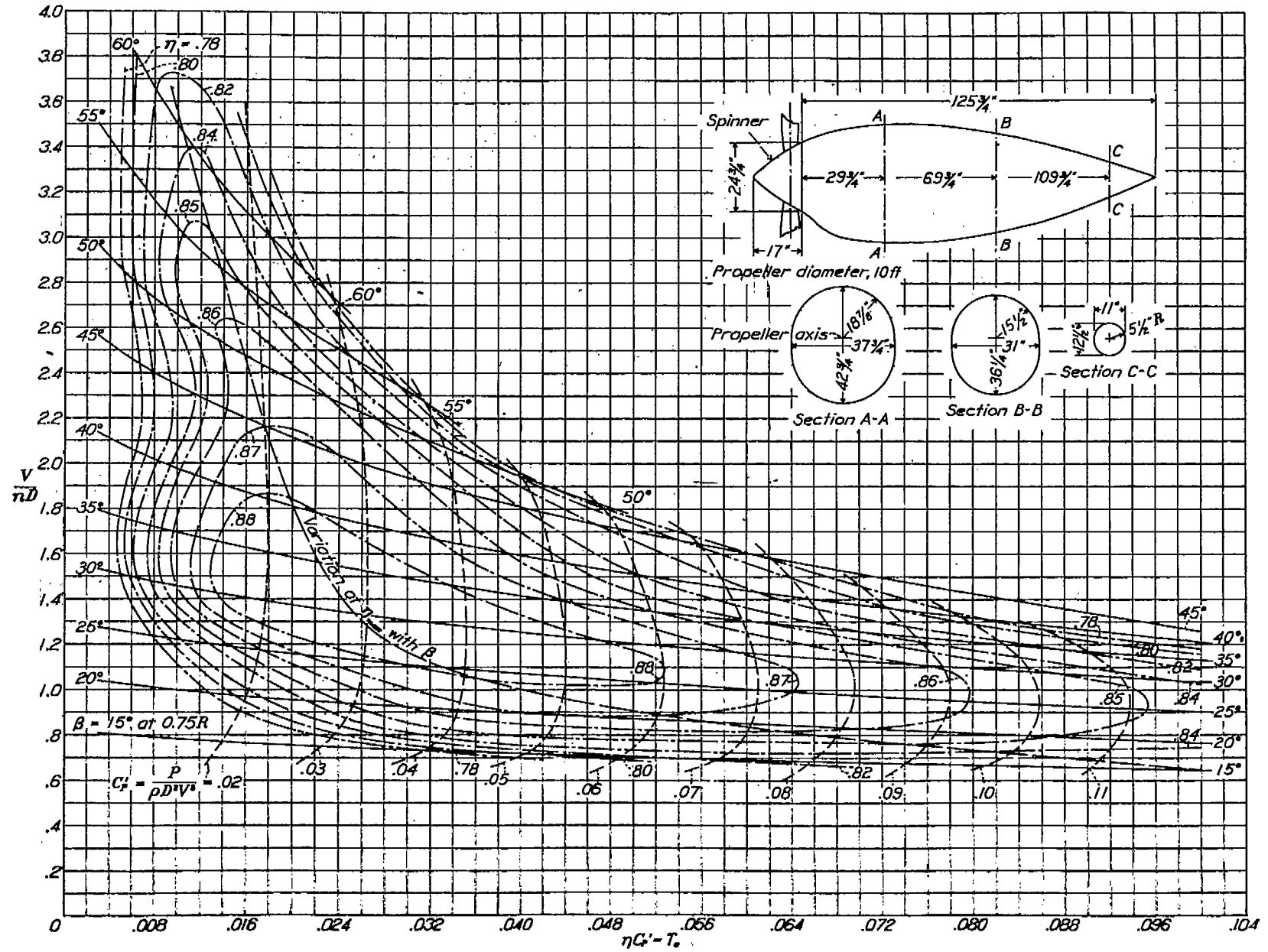
FIGURE 13.—Chart of V/nD against T_e for three-blade propeller 5992-2. Liquid-cooled engine nacelle, with spinner; single rotation. Propeller data taken from reference 3.
