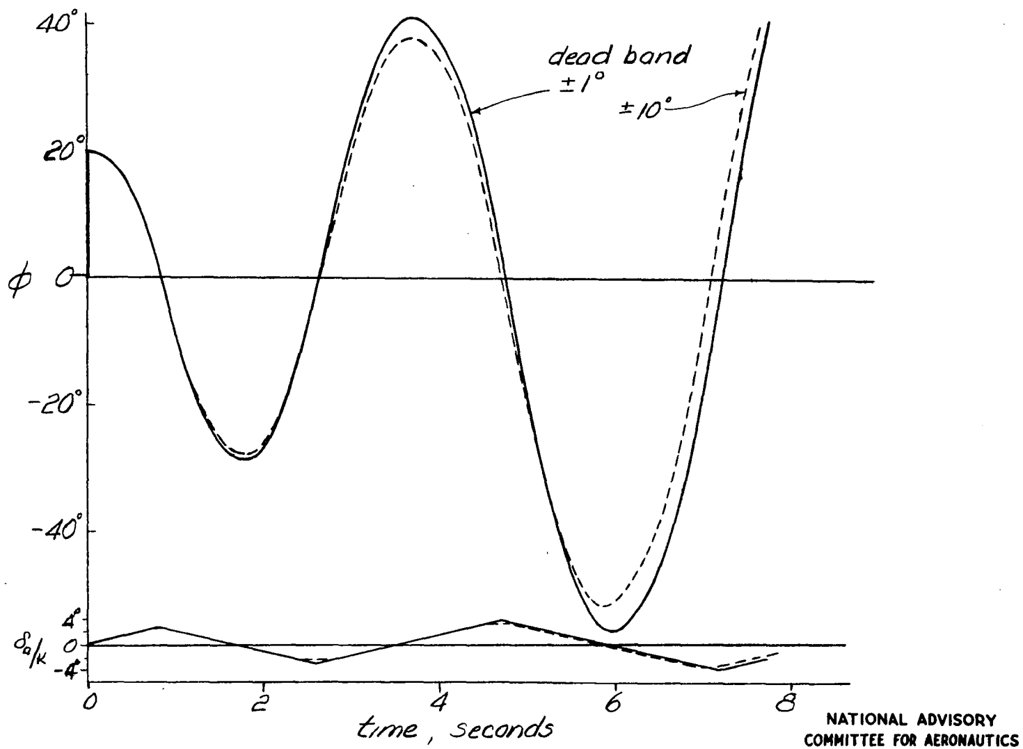
Figure 8.- Effect of width of dead band on stability. Lateral response, K = 1/2 ; \delta_a = 1.5^\circ per second; dead band = \pm 1^\circ and \pm 10^\circ .
