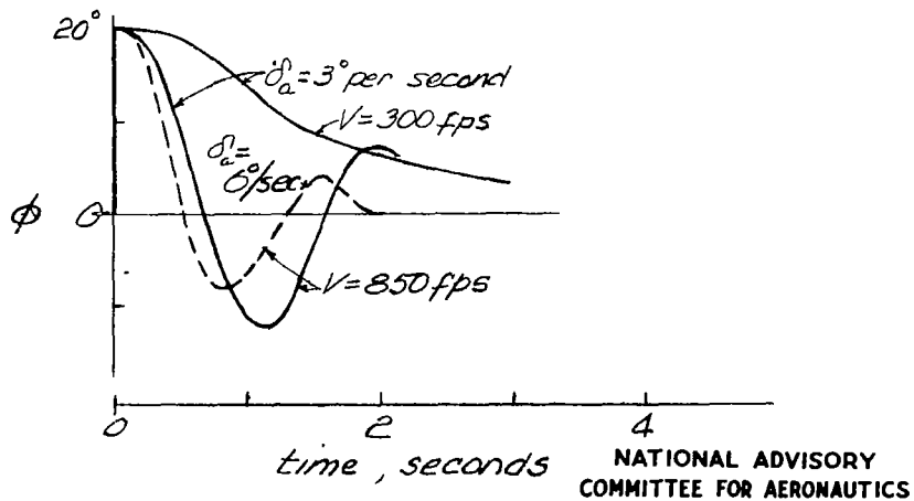
Figure 10.- Lateral motions, K = 1/12 . Lag = 0.15 seconds.
