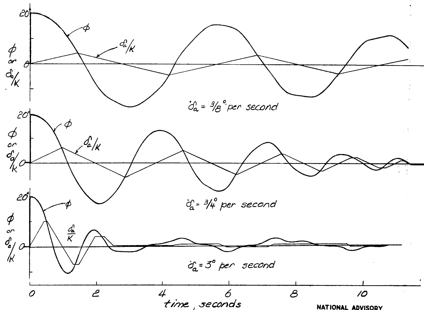
Figure 7.- Lateral responses, K = 1/8 . Other conditions as in figure 5.
