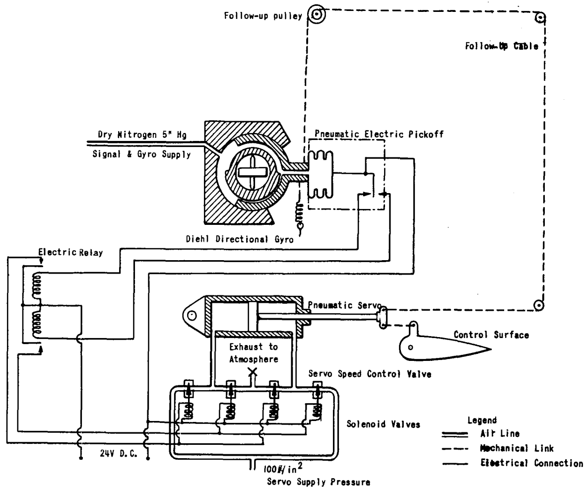
Figure 1.- Schematic Diagram - Pneumatic Servo
