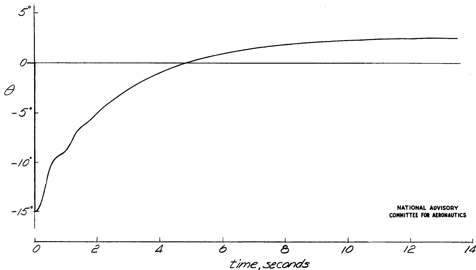
Figure 13. -Longitudinal motion, K=1/8 ; \dot{\delta}_e = 6.75 degrees per second, dead band \pm 3^\circ . V=850 feet per second.
