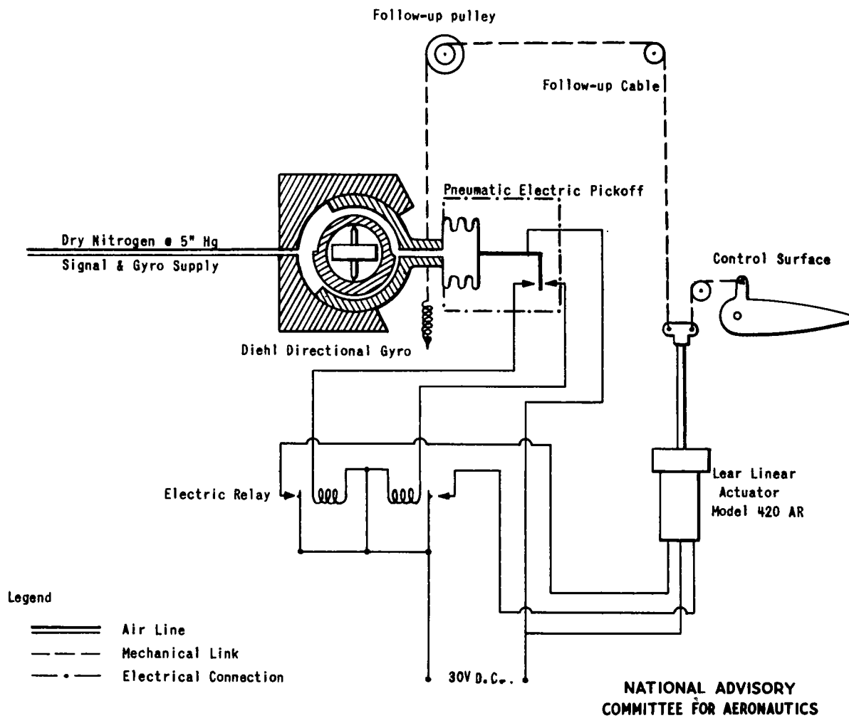
Figure 2.- Schematic Diagram - Electric Motor Servo
