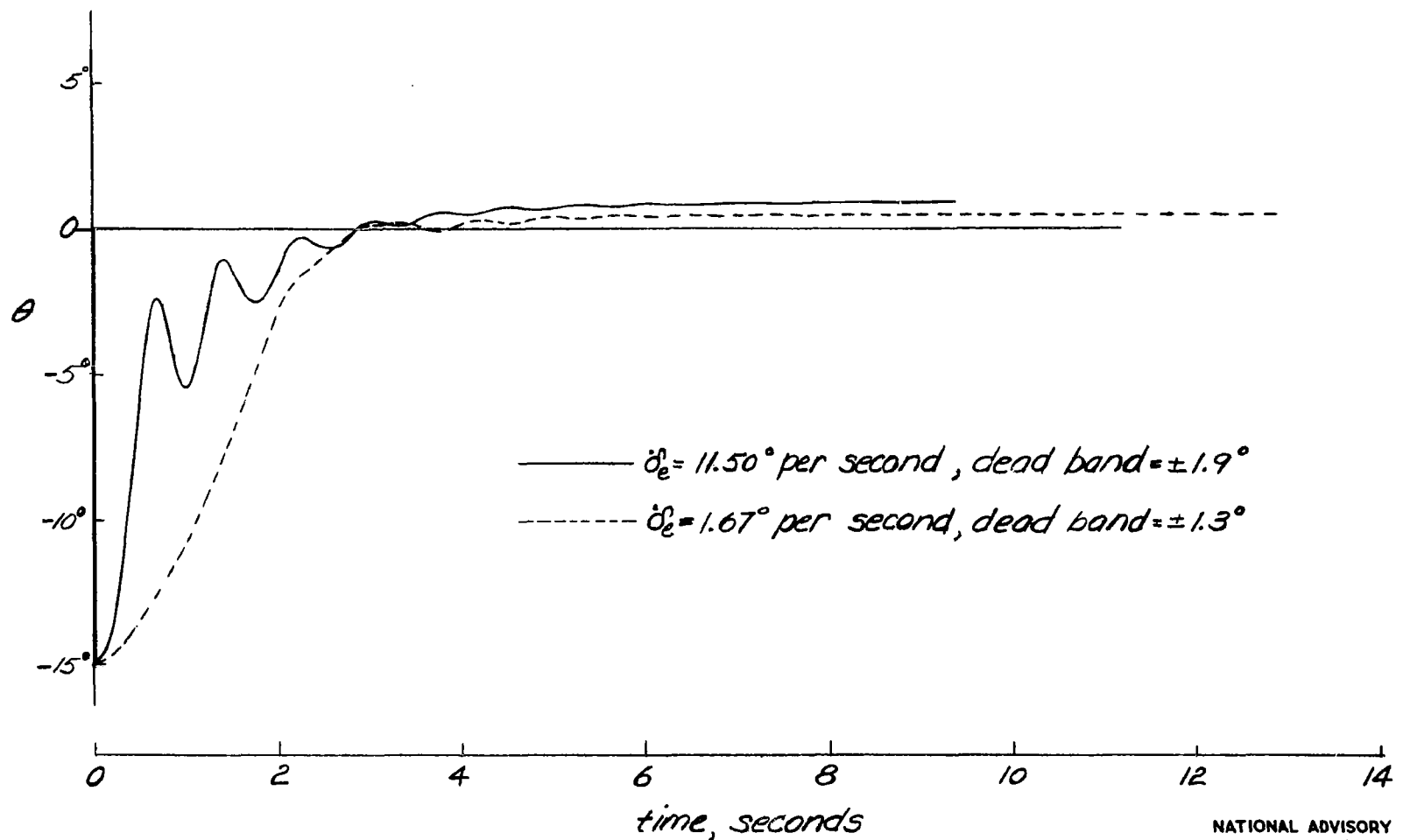
Figure 11.-Longitudinal motions, K=1/2 . No lag or coast included V=850 feet per second
