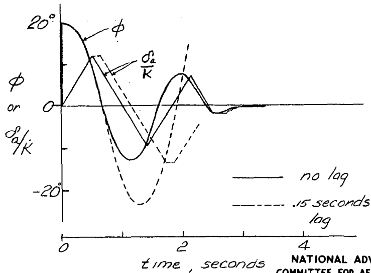
Figure 9.-Lateral motions, K = 1/8 and \delta_a = 3^\circ per second. Effect of servo coast causing 0.11^\circ of aileron motion after entering dead band, and of lag. V = 850 feet per second.
