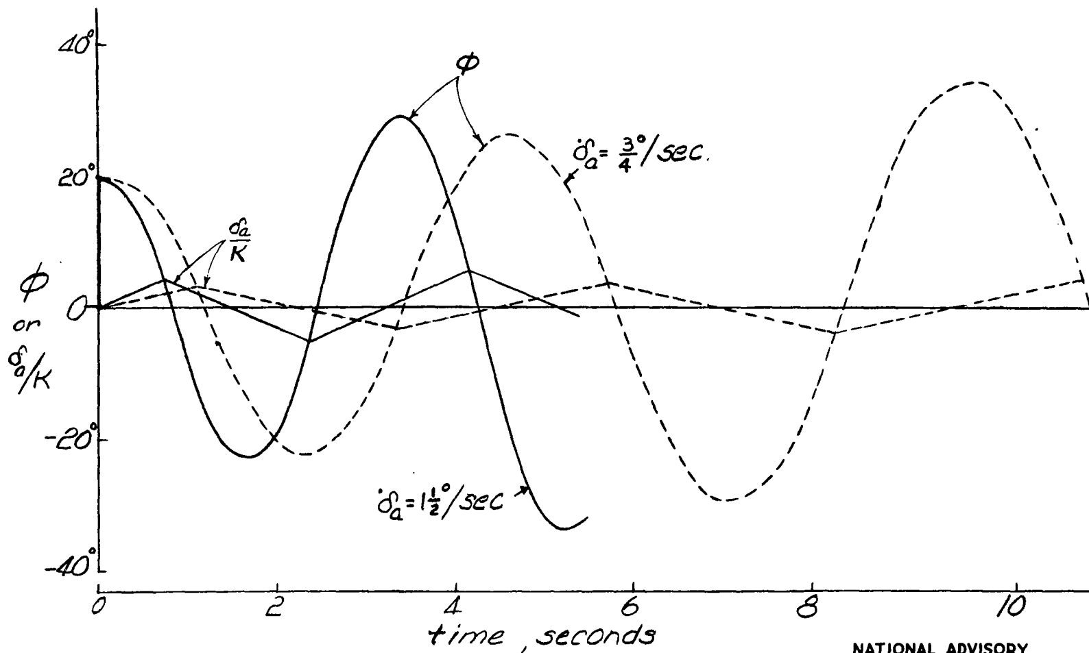
Figure 6.- Lateral responses, K = 1/4 . Dead band = \pm 1 degree. Other conditions are as given for figure 5. Motion of the gyro reference is also shown.
