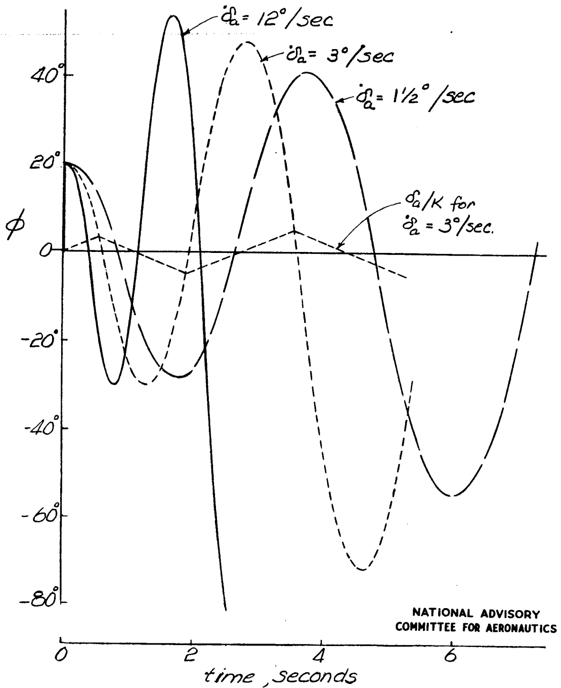
Figure 5.- Lateral responses, K = 1/2 . No lag or coast included. Dead bands vary from \pm 1 degree to \pm 4.5 degrees, increasing with \dot{\delta}_a . V = 850 feet per second.
