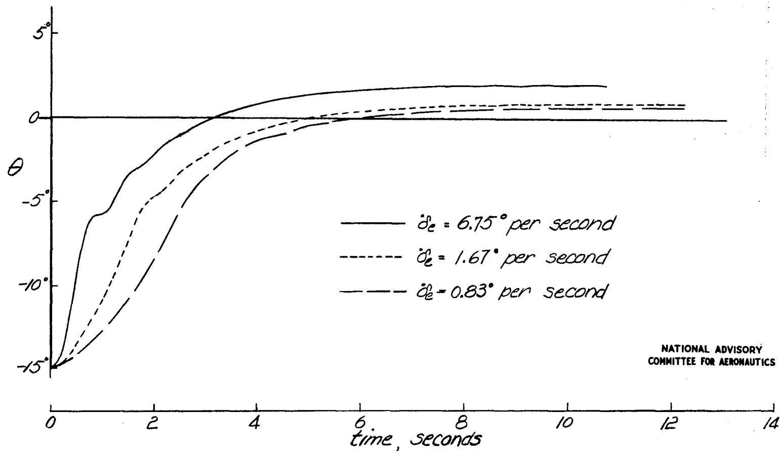
Figure 12.-Longitudinal motions, K=1/4 . Dead bands vary from \pm 2.5^\circ to \pm 1.3^\circ . V=850 feet per second.
