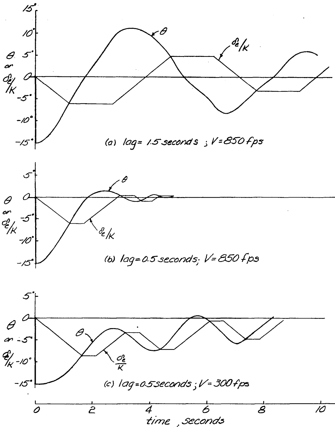
Figure 14.- Longitudinal motions, K = 1/2 , showing the effect of lag.
