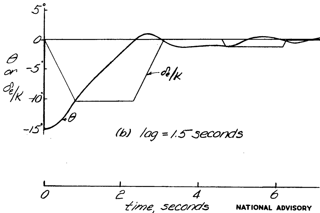
Figure 16.- Longitudinal motion, K = 1/5 ; lag = 0.5 and 1.5 seconds; V = 850 feet per second.
