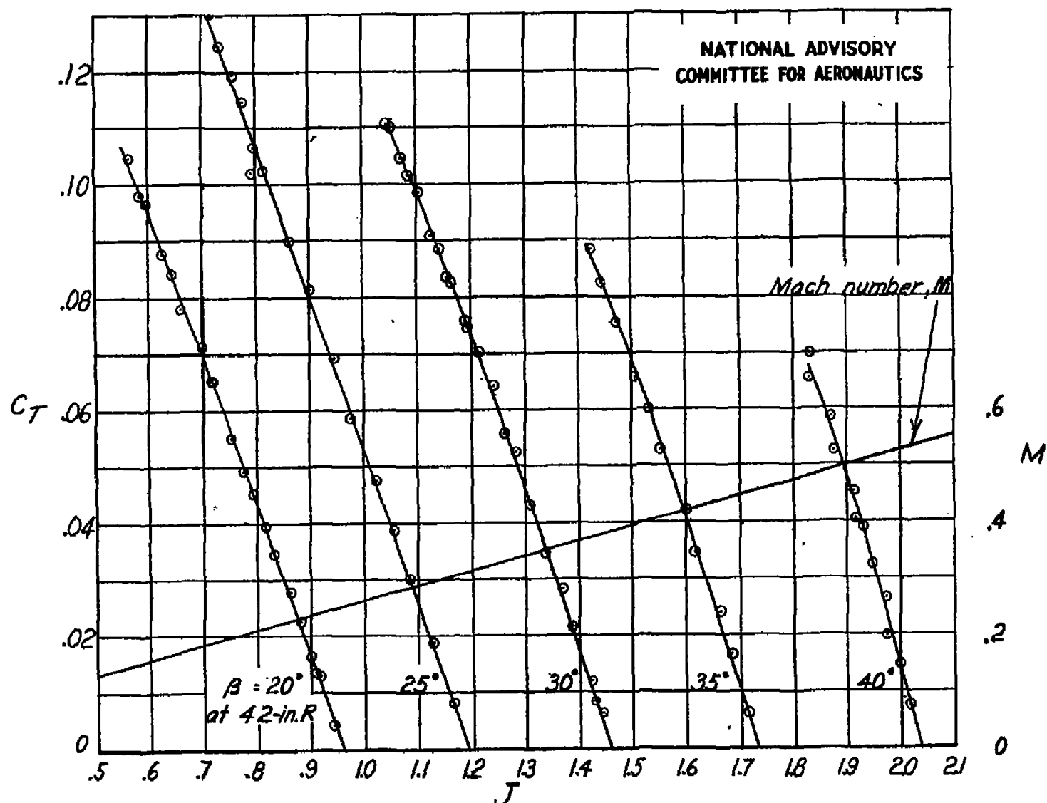
Figure 8.- Variation of thrust coefficient with advance ratio. Clean blades; D=10 feet.
