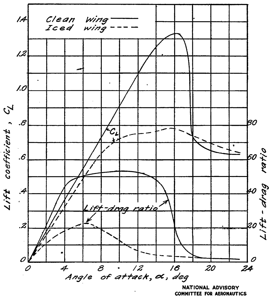
Figure 17.- Characteristics of an NACA 0012 airfoil for infinite aspect ratio.
