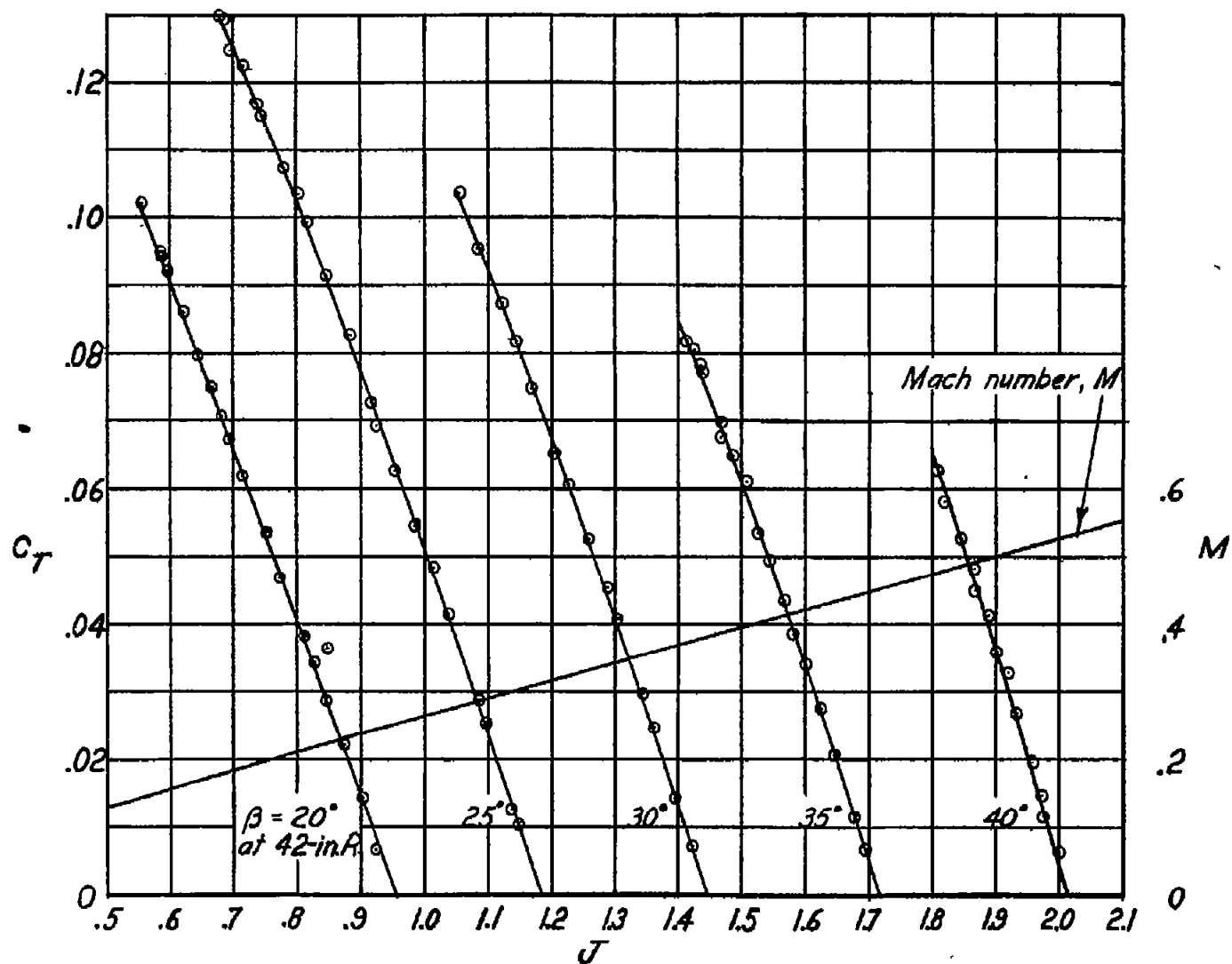
Figure 10.- Variation of thrust coefficient with advance ratio. Simulated ice on blades; D=10 feet.
