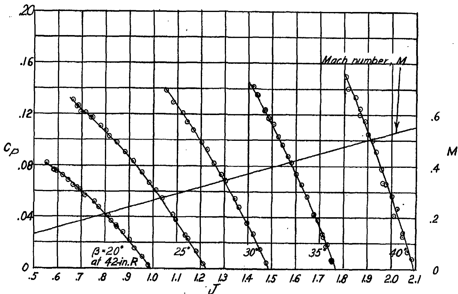
Figure 11.- Variation of power coefficient with advance ratio. Simulated ice on blades; D=10 feet.
