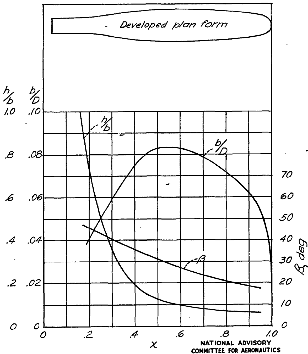
Figure 6.- Blade-form curves for Curtiss 89301-15 propeller. Activity factor, 98.0.
