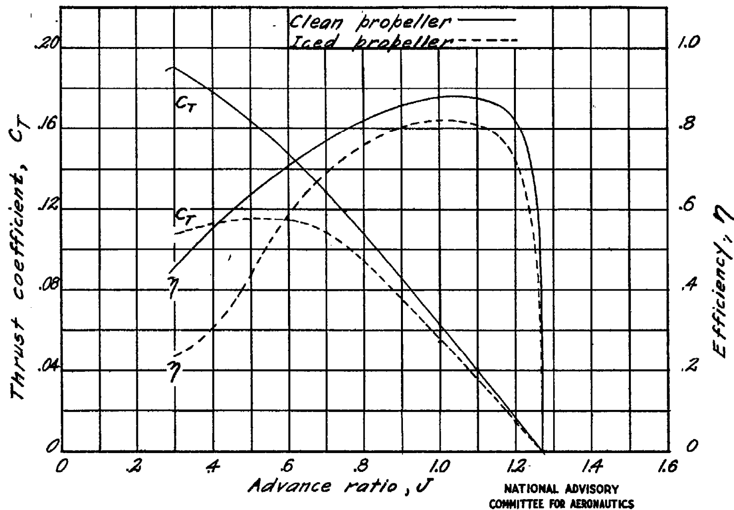
Figure 18.-Calculated propeller characteristics. NACA 0012 blade sections ; \beta, 30^\circ at 42-inch R.
