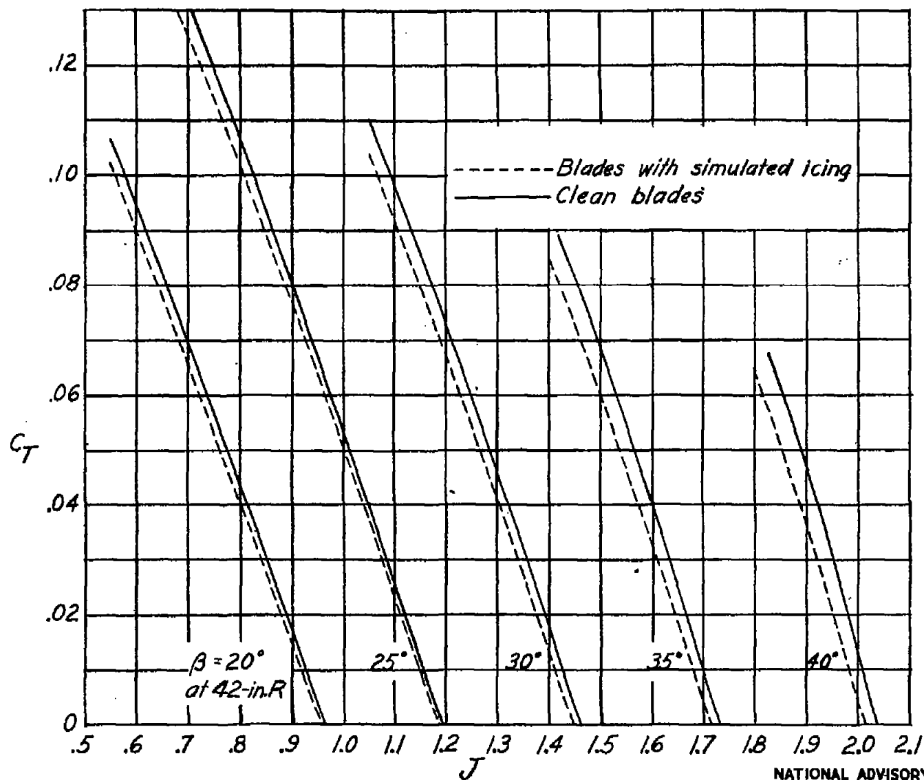
Figure 12.- The effect of icing on thrust coefficient. D=10 feet.
