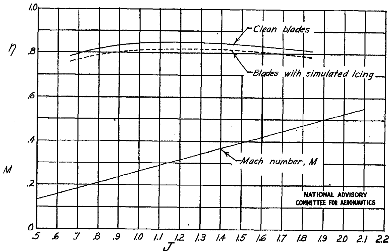
Figure 15.- A comparison of envelope propeller efficiencies to show effect of icing.
