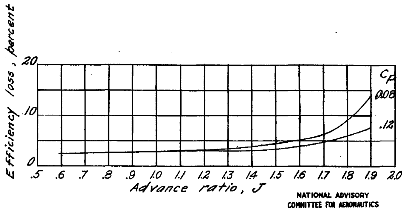
Figure 16.- Propeller efficiency loss due to ice formation for operation at constant-power coefficient.
