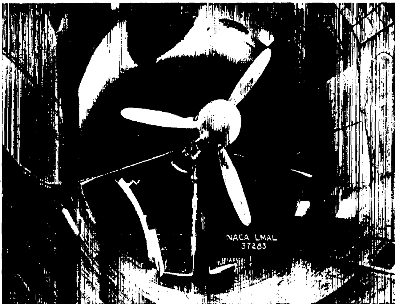
Figure 1.- Propeller dynamometer in test section. Clean blades.
