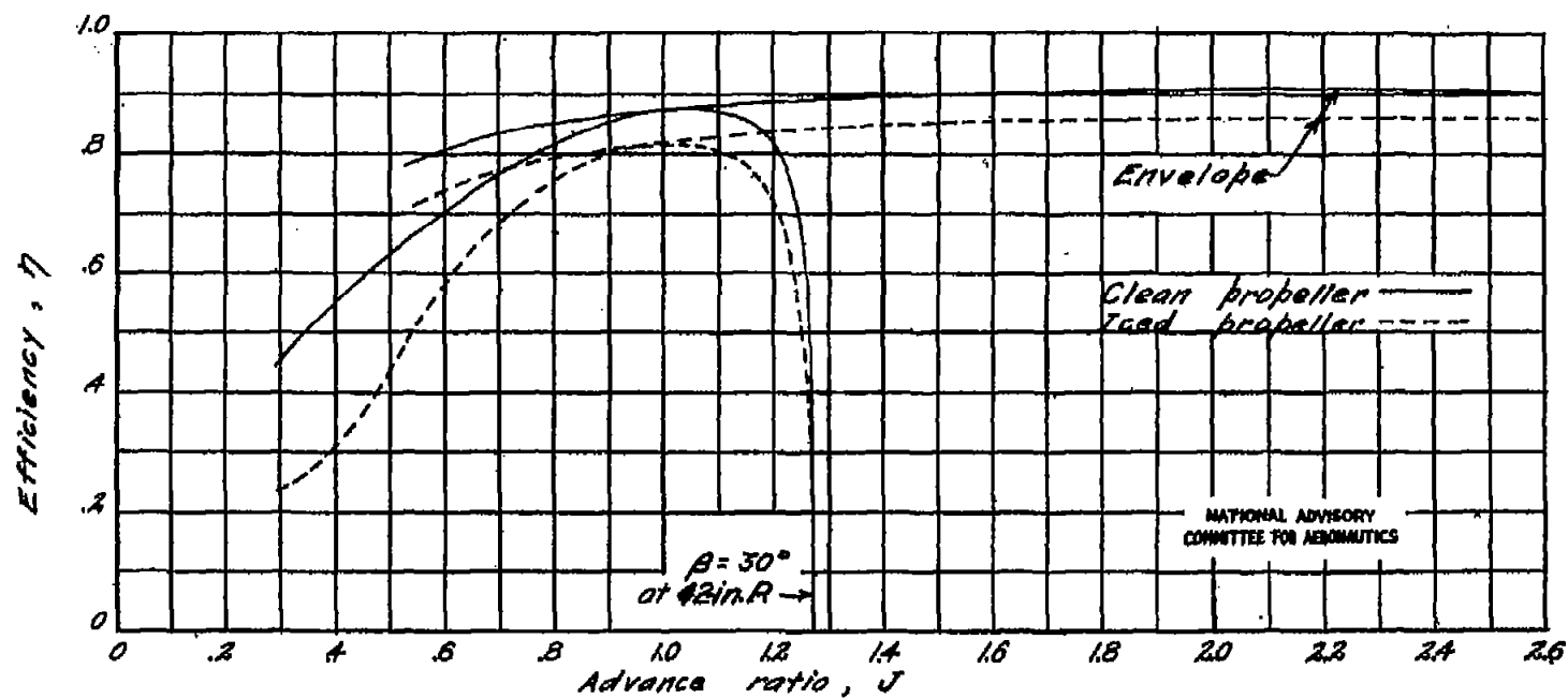
Figure 19.- Envelope curves of calculated propeller efficiency, NACA 0012 blade sections. D=10 feet.
