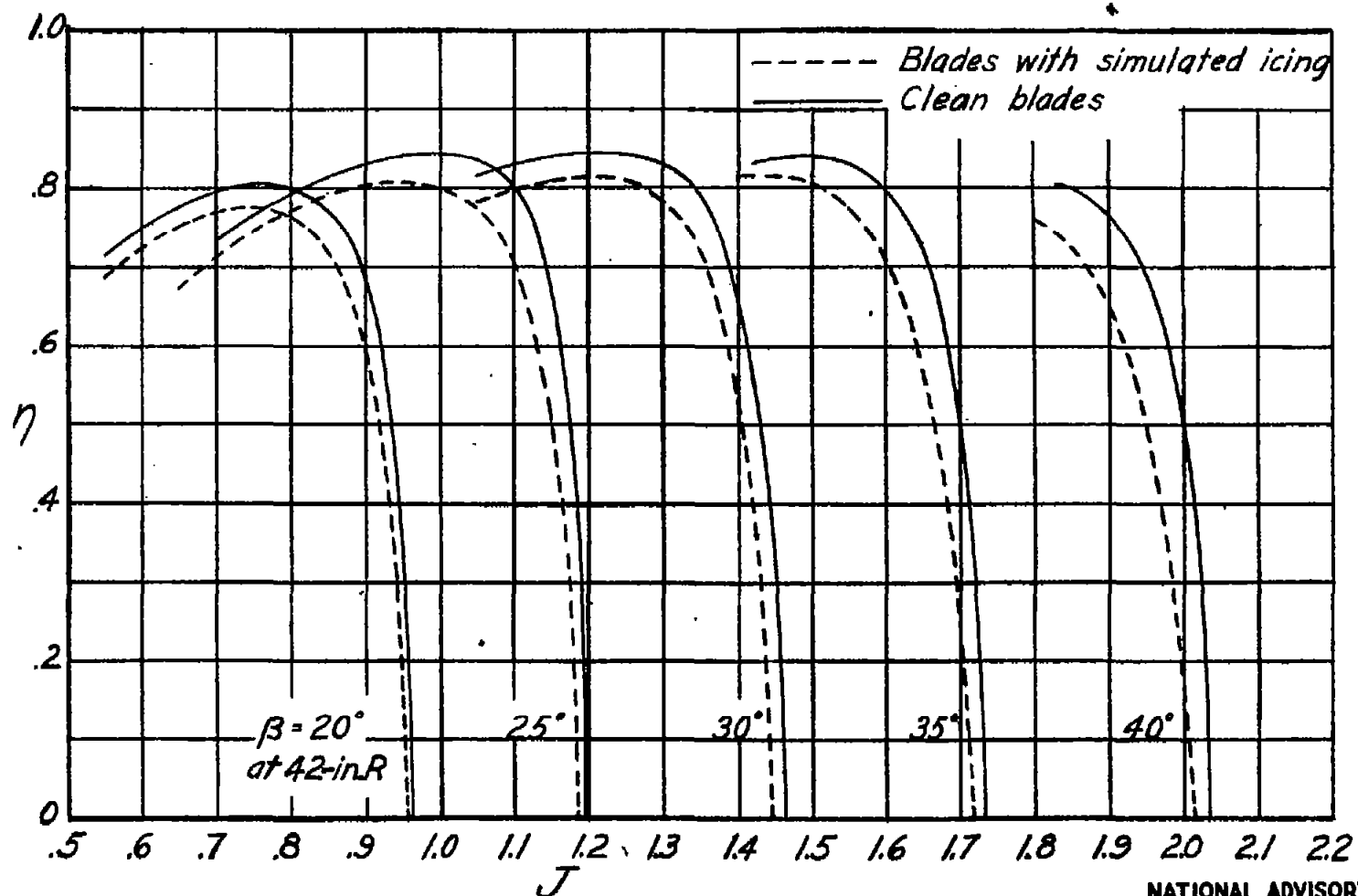
Figure 14.- The effect of icing on propeller efficiency. D = 10 feet.
