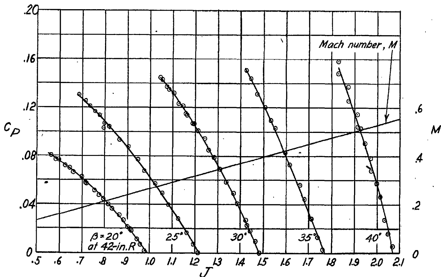
Figure 9.—Variation of power coefficient with advance ratio. Clean blades; D=10 feet.
