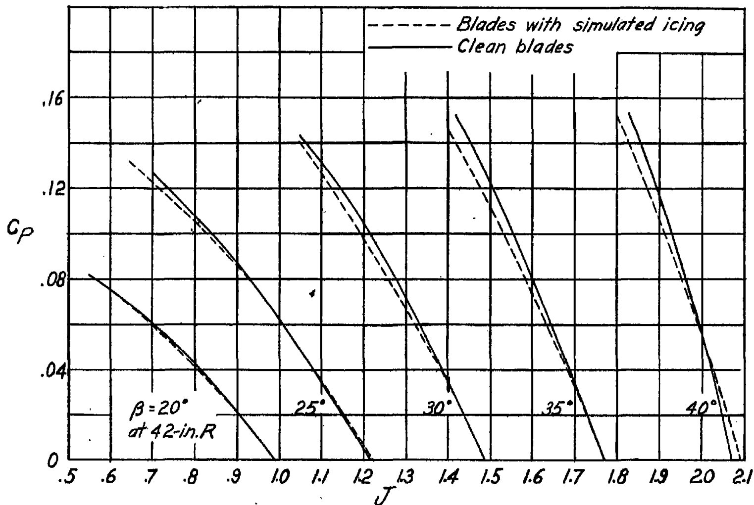
Figure 13.- The effect of icing on power coefficients. D = 10 feet.
