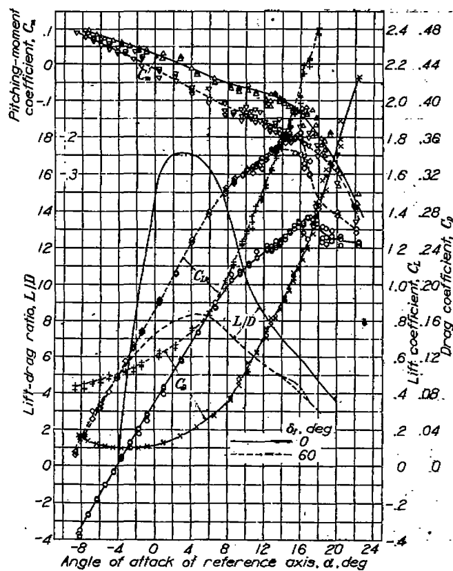
FIGURE 14.—Aerodynamic characteristics of model with 7-inch nacelles and 0.25c propeller location.
