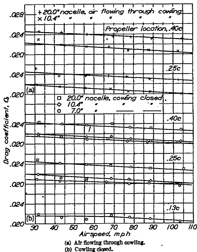
FIGURE 16.—Scale effect on drag coefficient at C_L=0.25 .
