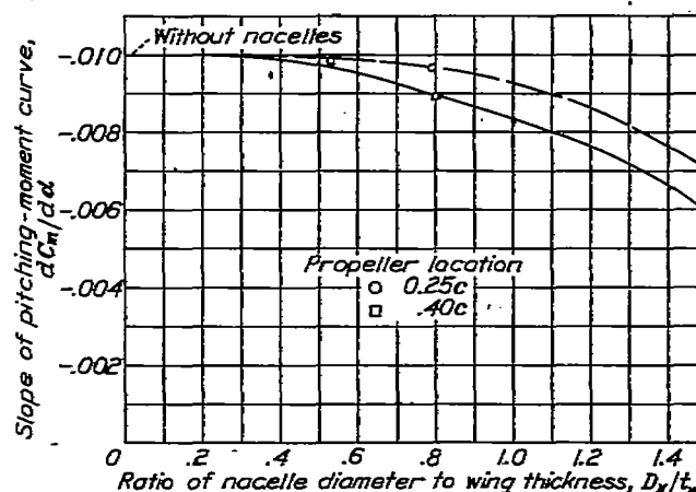
FIGURE 22.—Variation of the slope of the pitching-moment curve of the model for nacelles of various size.
