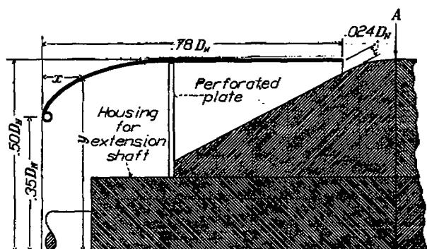
FIGURE 7.—Dimensions of cowling and cowling arrangement.
