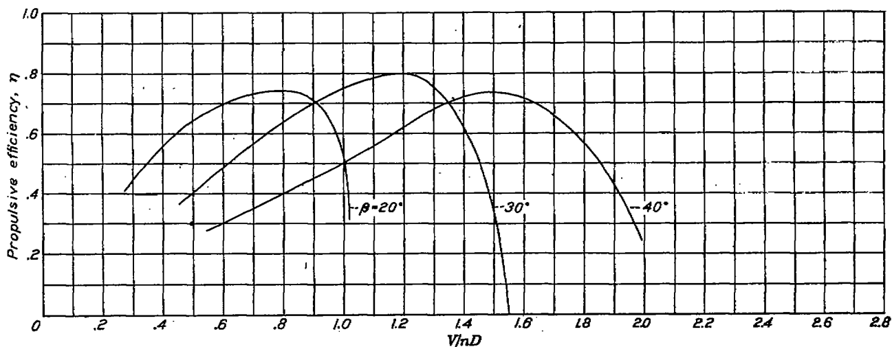
FIGURE 28.—Variation of propulsive efficiency with blade angle. The 7-inch nacelles; 0.25c propeller location; C_L , 0.25; cowling closed.
