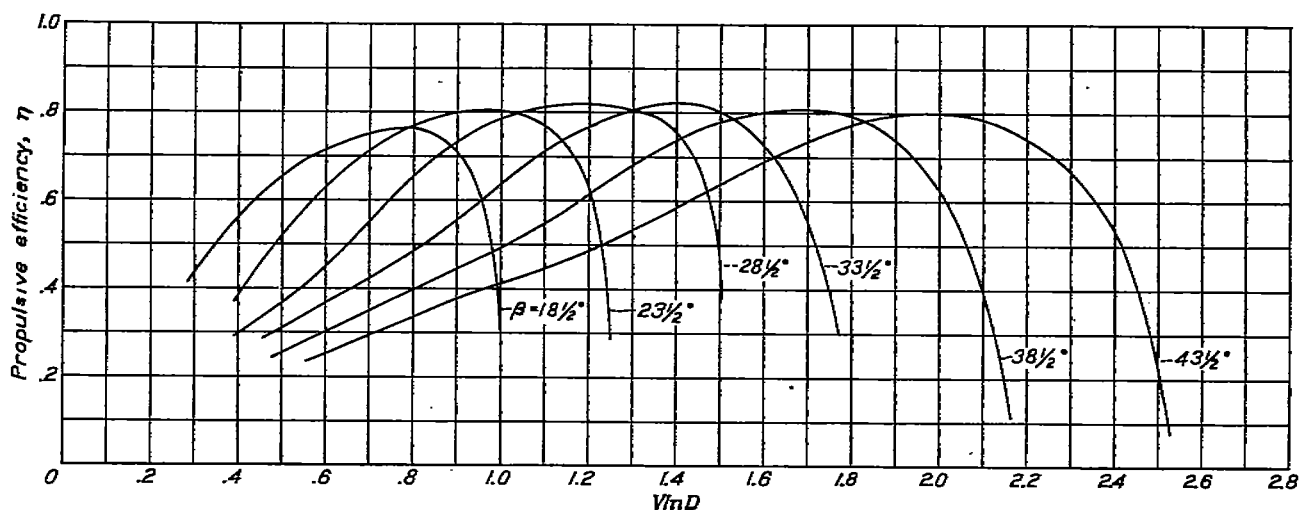
FIGURE 23.—Variation of propulsive efficiency with blade angle. The 20-inch nacelles; 0.40c propeller location; C_L , 0.25; air flowing through cowl.
