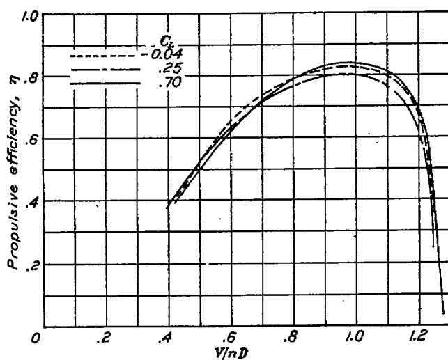
FIGURE 34.—Variation of propulsive efficiency with lift coefficient. The 20-inch nacelles; 0.40c propeller location; \beta , 23\frac{1}{2}^\circ ; air flowing through cowling.
