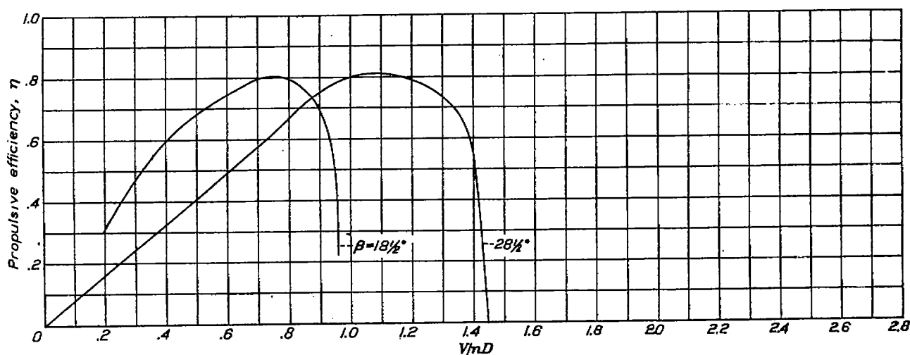
FIGURE 33.—Variation of propulsive efficiency with blade angle. The 10.4-inch nacelles; 0.25c propeller location; C_L , 0.25; cowling closed.
