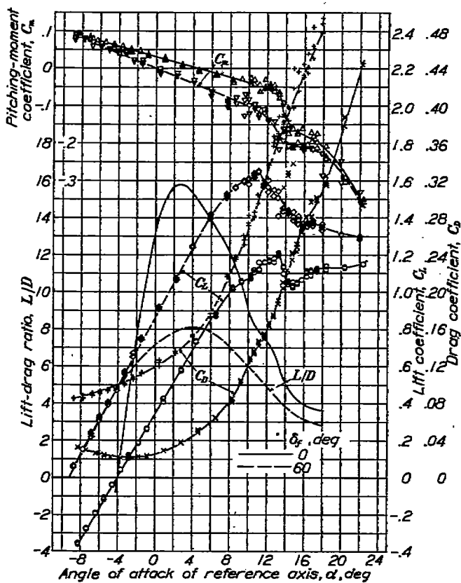
FIGURE 10.—Aerodynamic characteristics of model with 20-inch nacelles and 0.25c propeller location.
