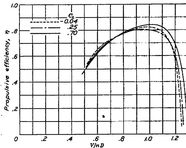
FIGURE 35.—Variation of propulsive efficiency with lift coefficient. The 20-inch nacelles; 0.25c propeller location; \beta , 23\frac{1}{2}^\circ ; air flowing through cowling.
