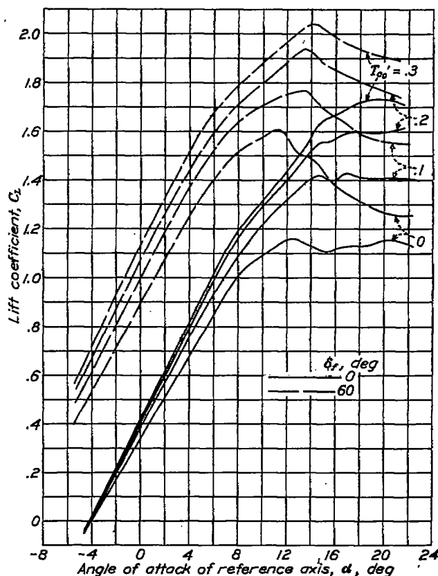
FIGURE 40.—Effect of propeller operation on lift coefficient of the model for various index thrust coefficients. The 20-inch nacelles; 0.40c propeller location.
