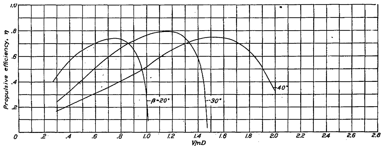
FIGURE 27.—Variation of propulsive efficiency with blade angle. The 7-inch nacelles; 0.40c propeller location; C_L , 0.25; cowling closed.
