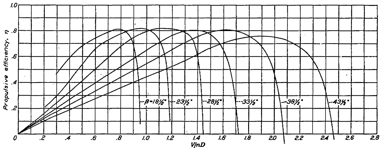
FIGURE 26.—Variation of propulsive efficiency with blade angle. The 10.4-inch nacelles; 0.25c propeller location; C_L , 0.25; air flowing through cowling.
