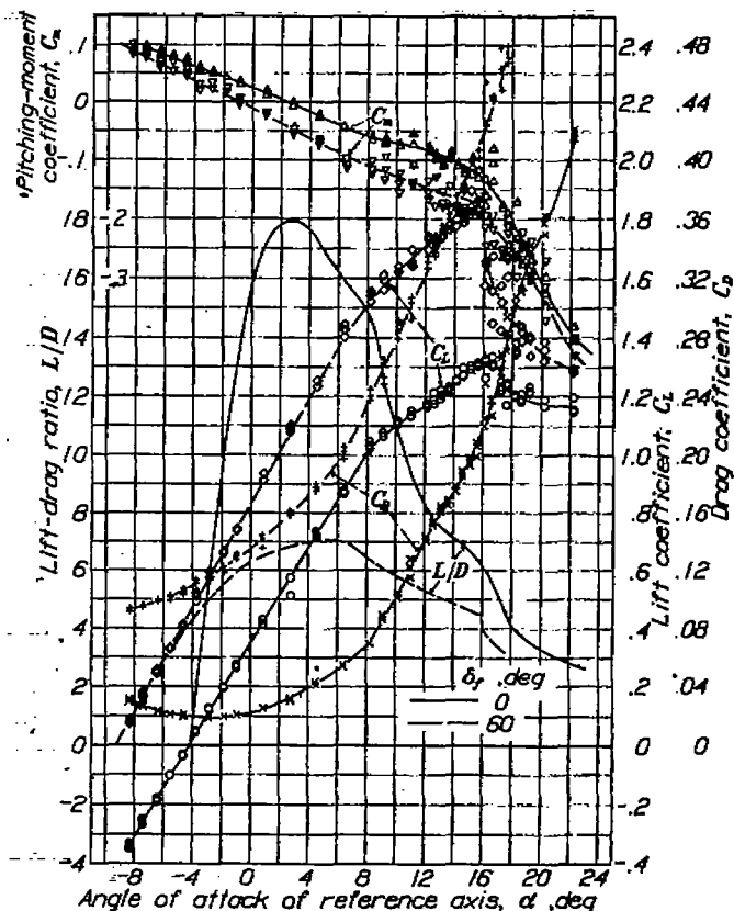
FIGURE 15.—Aerodynamic characteristics of model with 7-inch nacelles and 0.13c propeller location.
