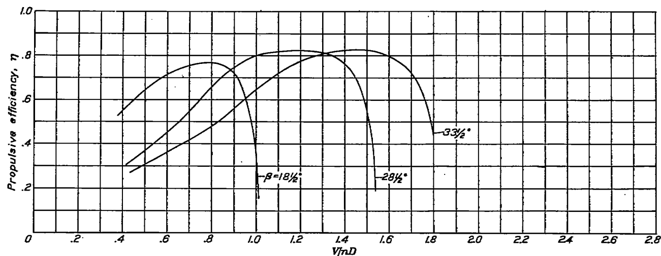
FIGURE 30.—Variation of propulsive efficiency with blade angle. The 20-inch nacelles; 0.40c propeller location; C_L , 0.25; cowling closed.
