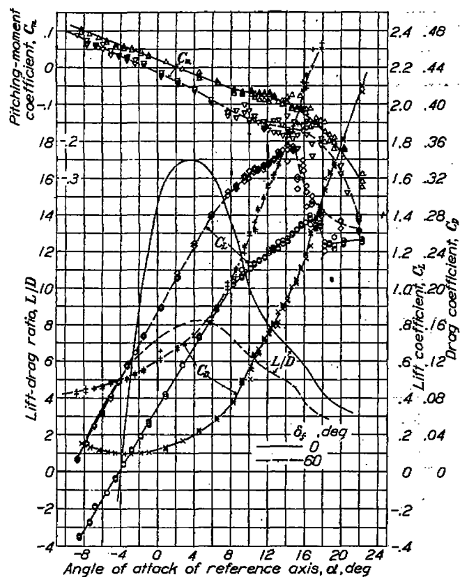
FIGURE 12.—Aerodynamic characteristics of model with 10.4-inch nacelles and 0.25c propeller location.
