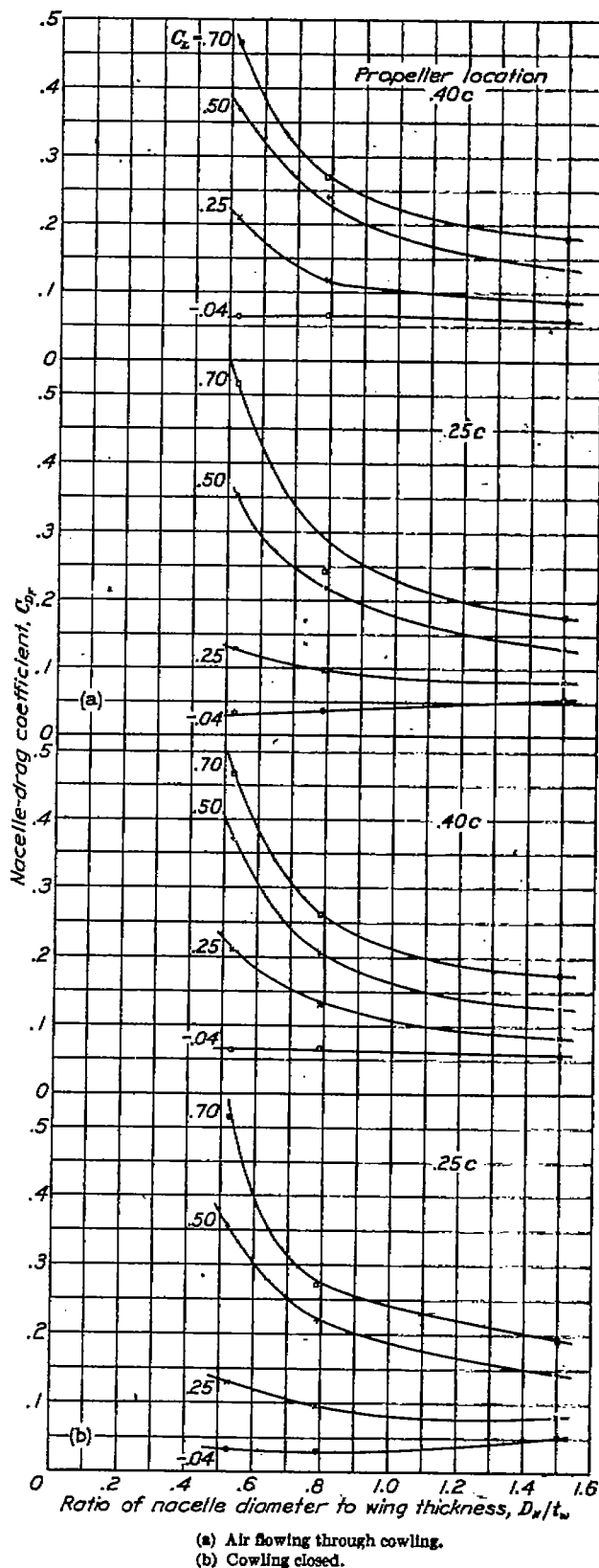
FIGURE 19.—Nacelle drag coefficient for nacelles of various size and for several lift coefficients.
