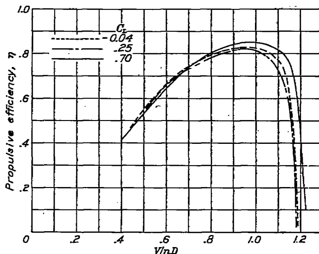
FIGURE 37.—Variation of propulsive efficiency with lift coefficient. The 10.4-inch nacelles; 0.25c propeller location; \beta , 23\frac{1}{4}^\circ ; air flowing through cowling.
