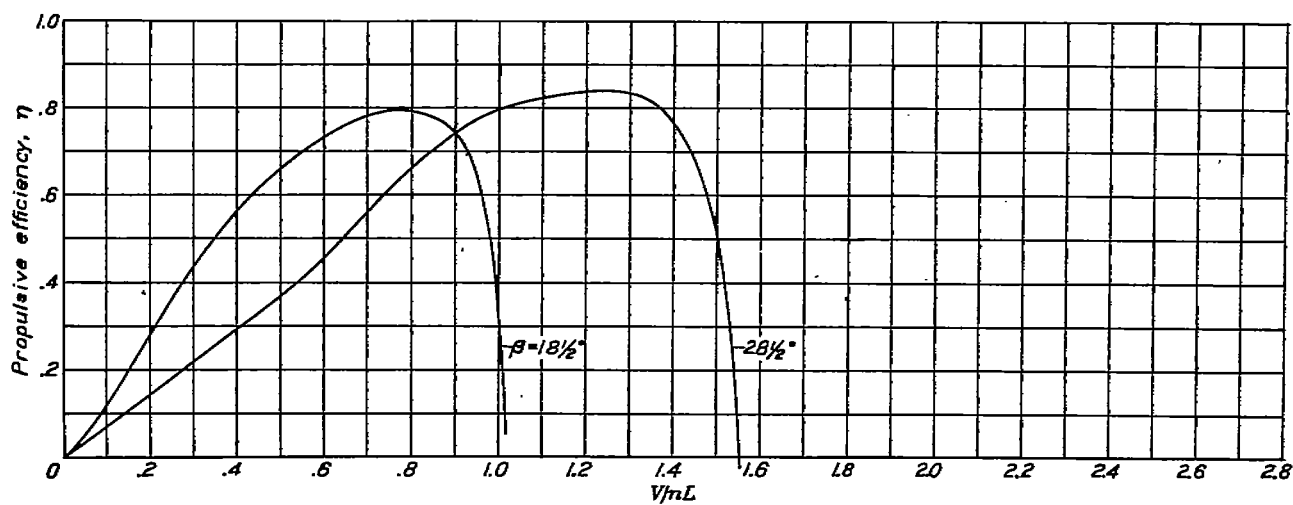
FIGURE 31.—Variation of propulsive efficiency with blade angle. The 20-inch nacelles; 0.25c propeller location; C_L , 0.25; cowling closed.
