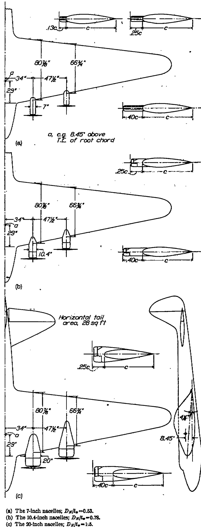
FIGURE 1.—Diagram of model showing arrangements of the nacelles.
