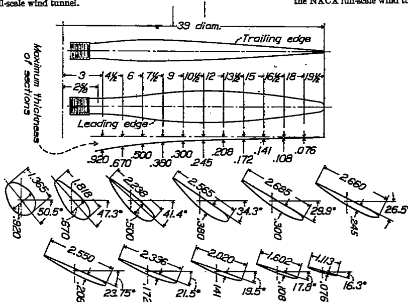
FIGURE 6.—Blade dimensions for three-blade model propellers. All linear dimensions given in inches.
