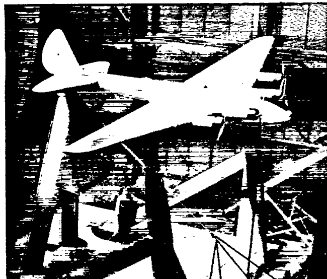
FIGURE 4.—Installation of model with 10.4-inch nacelles and 0.40c propeller location in the NACA full-scale wind tunnel.
