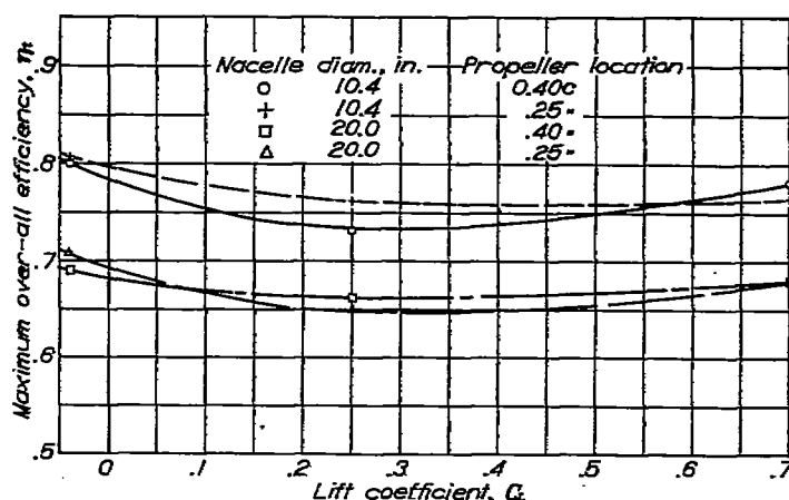
FIGURE 39.—Variation of maximum over-all efficiency with lift coefficient. Various nacelle arrangements; \beta , 23\frac{1}{2}^\circ ; cowling closed.
