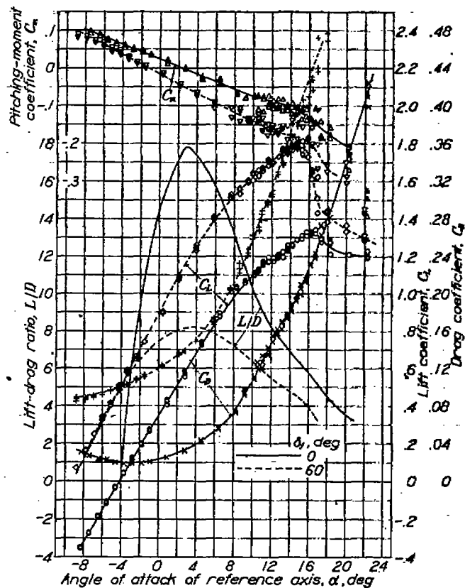
FIGURE 13.—Aerodynamic characteristics of model with 7-inch nacelles and 0.40c propeller location.
