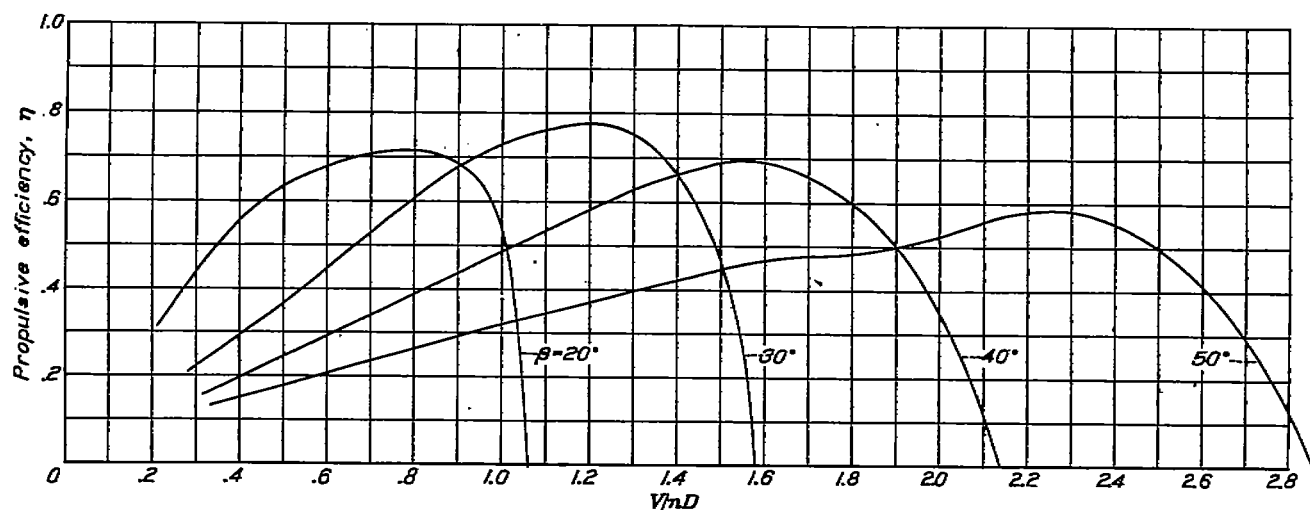
FIGURE 29.—Variation of propulsive efficiency with blade angle. The 7-inch nacelles; 0.13c propeller location; C_L , 0.25; cowling closed.
