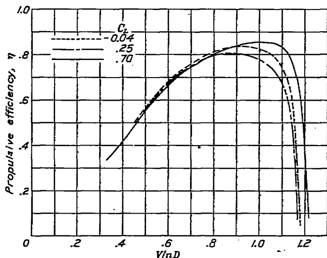
FIGURE 36.—Variation of propulsive efficiency with lift coefficient. The 10.4-inch nacelles; 0.40c propeller location; \beta , 23\frac{1}{4}^\circ ; air flowing through cowling.
