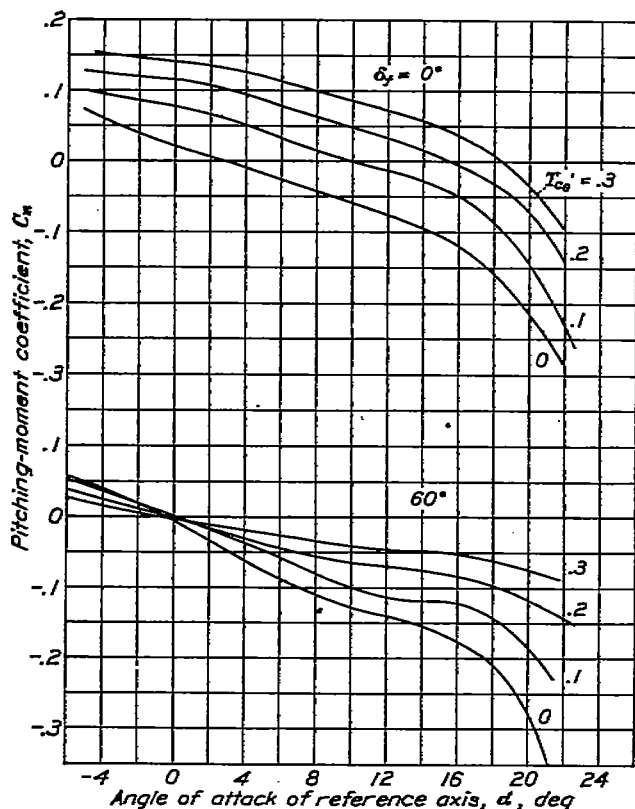
FIGURE 44.—Variation of pitching-moment coefficient of the model with index thrust coefficient. The 10.4-inch nacelles; 0.25c propeller location.
