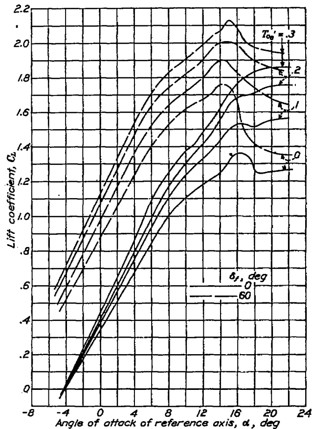
FIGURE 41.—Effect of propeller operation on lift coefficient of the model for various index thrust coefficients. The 10.4-inch nacelles; 0.25c propeller location.
