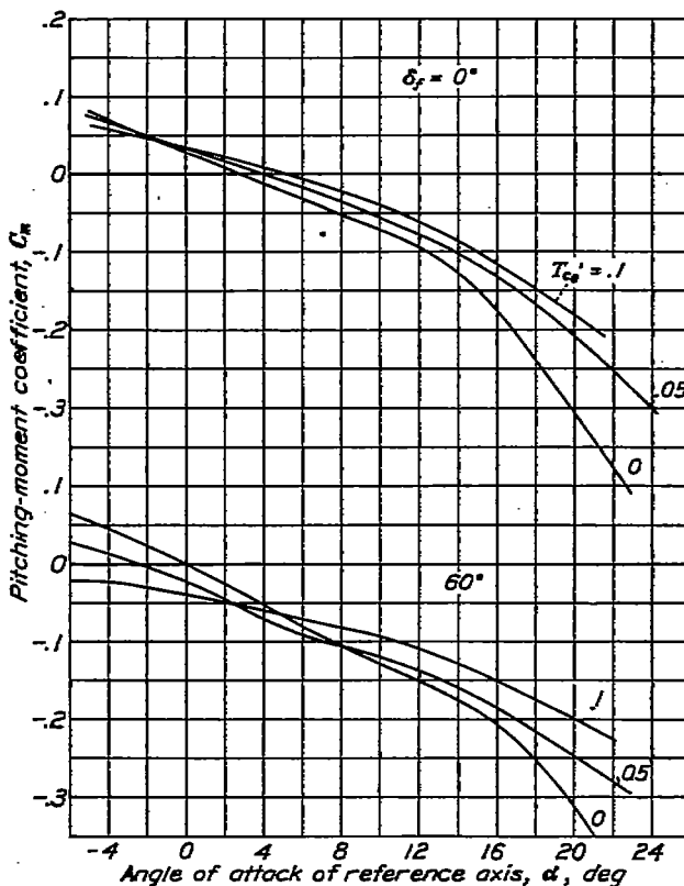
FIGURE 45.—Variation of pitching-moment coefficient of the model with index thrust coefficient. The 7-inch nacelles; 0.13c propeller location.
