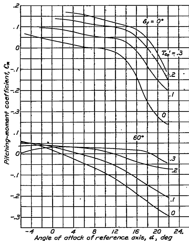
FIGURE 43.—Variation of pitching-moment coefficient of the model with index thrust coefficient. The 20-inch nacelles; 0.40c propeller location.
