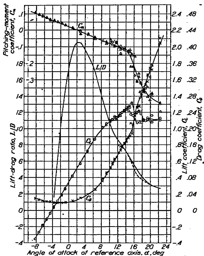
FIGURE 8.—Aerodynamic characteristics of model without nacelles.
