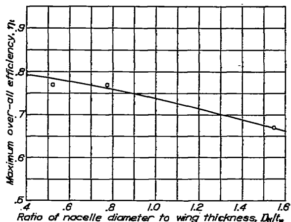
FIGURE 38.—Variation of maximum over-all efficiency with nacelle size. The 0.25c propeller location; C_L , 0.25; \beta , approximately 30^\circ ; air flowing through cowling.
