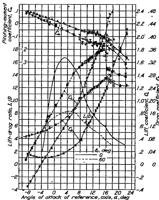
FIGURE 11.—Aerodynamic characteristics of model with 10.4-inch nacelles and 0.40c propeller location.
