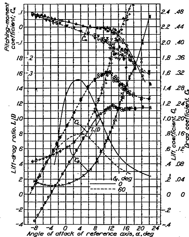
FIGURE 9.—Aerodynamic characteristics of model with 20-inch nacelles and 0.40c propeller location.
