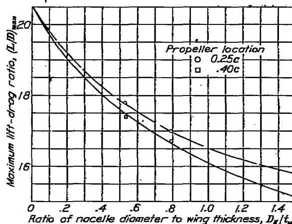
FIGURE 21.—Variation of the maximum lift-drag ratio of the model for nacelles of various size.
