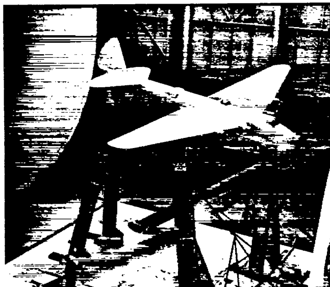
FIGURE 3.—Installation of model with 7-inch nacelles and 0.13c propeller location in the NACA full-scale wind tunnel.
