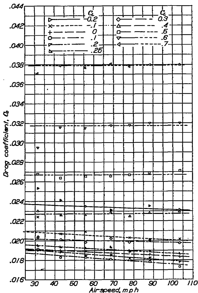
FIGURE 17.—Scale effect on the model without nacelles for the range of lift coefficients.
