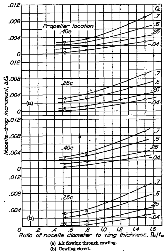
FIGURE 18.—Drag increments due to nacelles for nacelles of various size and for several lift coefficients.
