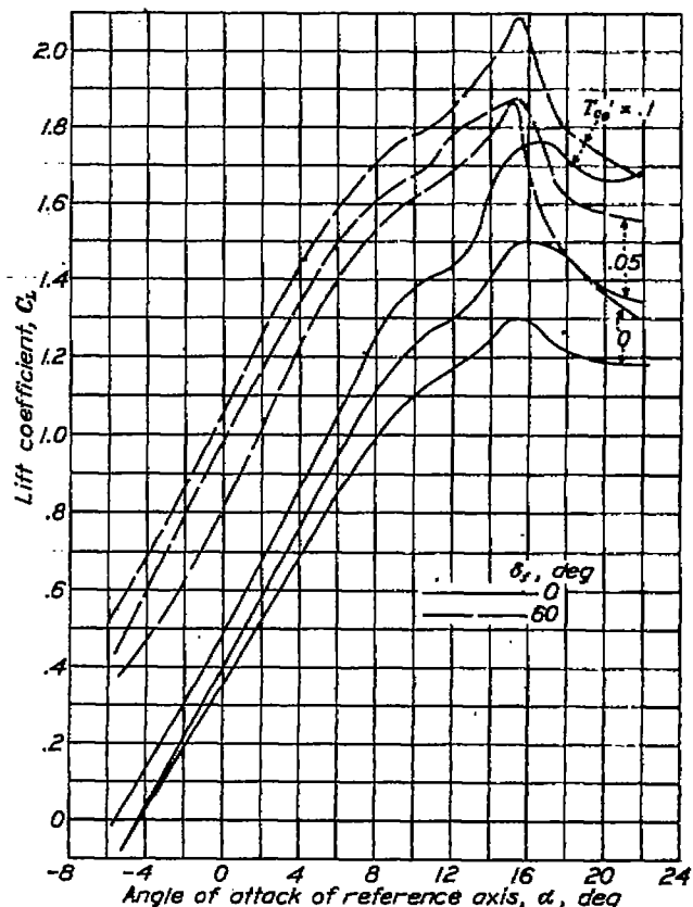
FIGURE 42.—Effect of propeller operation on lift coefficient of the model for various index thrust coefficients. The 7-inch nacelles; 0.13c propeller location.
