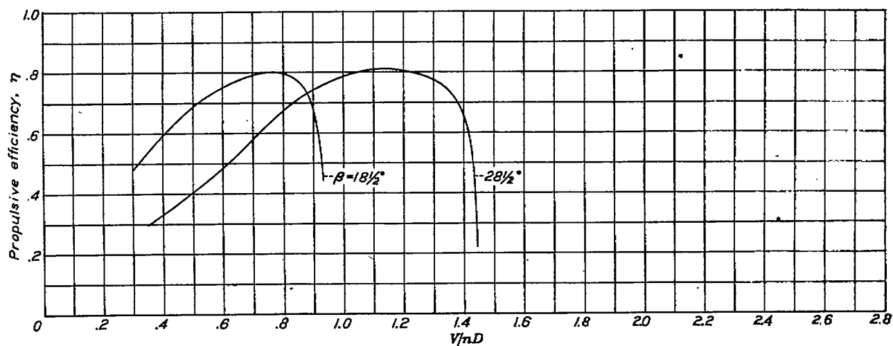
FIGURE 32.—Variation of propulsive efficiency with blade angle. The 10.4-inch nacelles; 0.40c propeller location; C_L , 0.25; cowling closed.
