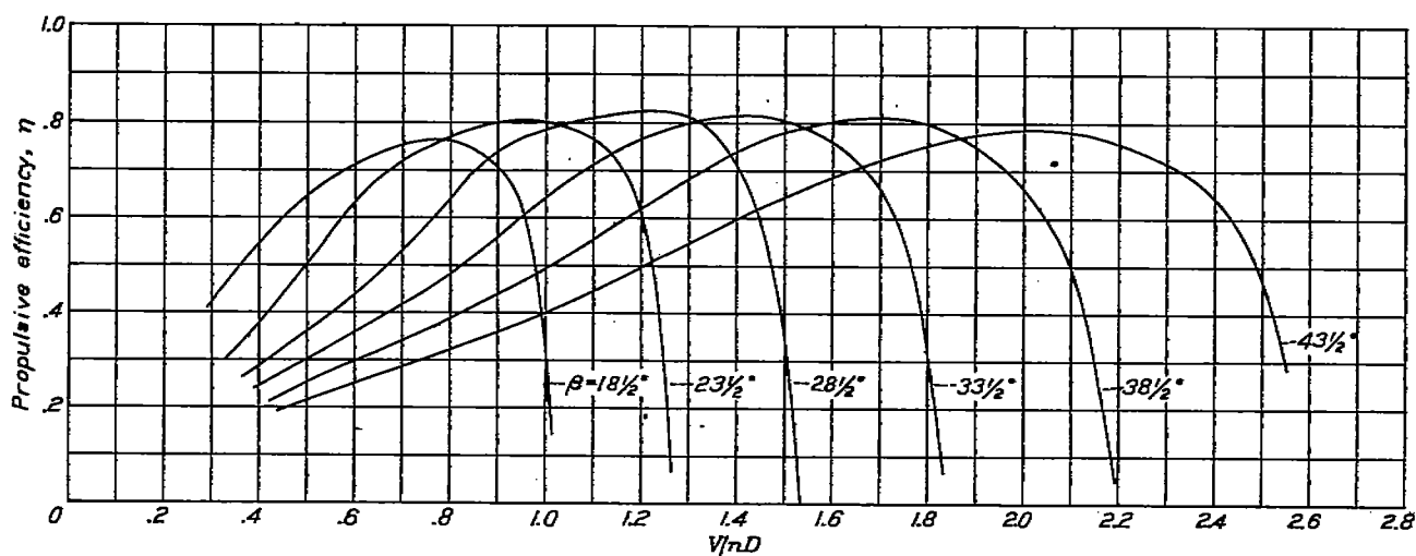
FIGURE 24.—Variation of propulsive efficiency with blade angle. The 20-inch nacelles; 0.25c propeller location; C_L , 0.25; air flowing through cowl.
