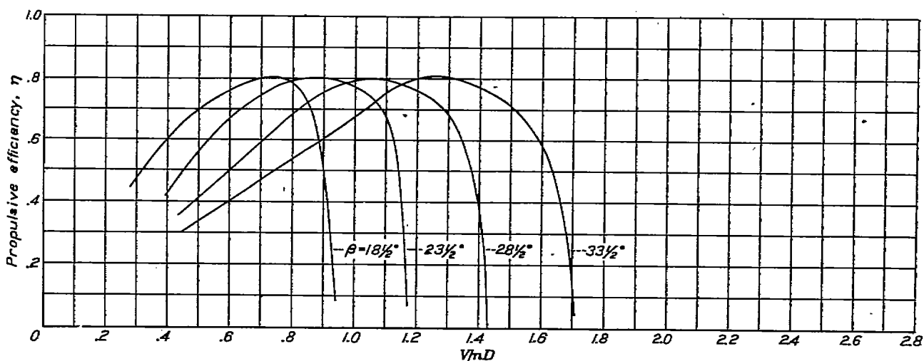
FIGURE 25.—Variation of propulsive efficiency with blade angle. The 10.4-inch nacelles; 0.40c propeller location; C_L , 0.25; air flowing through cowl.
