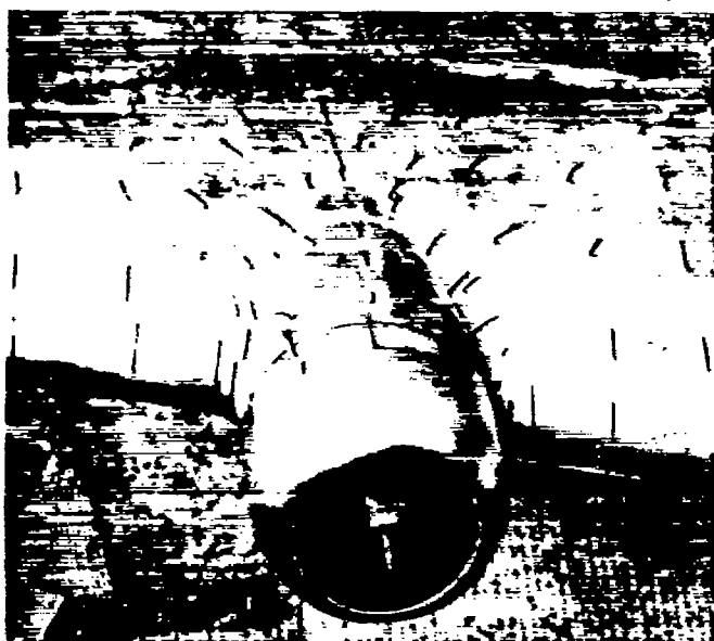
FIGURE 20.—Air flow over upper surface of wing and nacelle. The 20-inch nacelle; 0.25c propeller location; \alpha , 12°.
