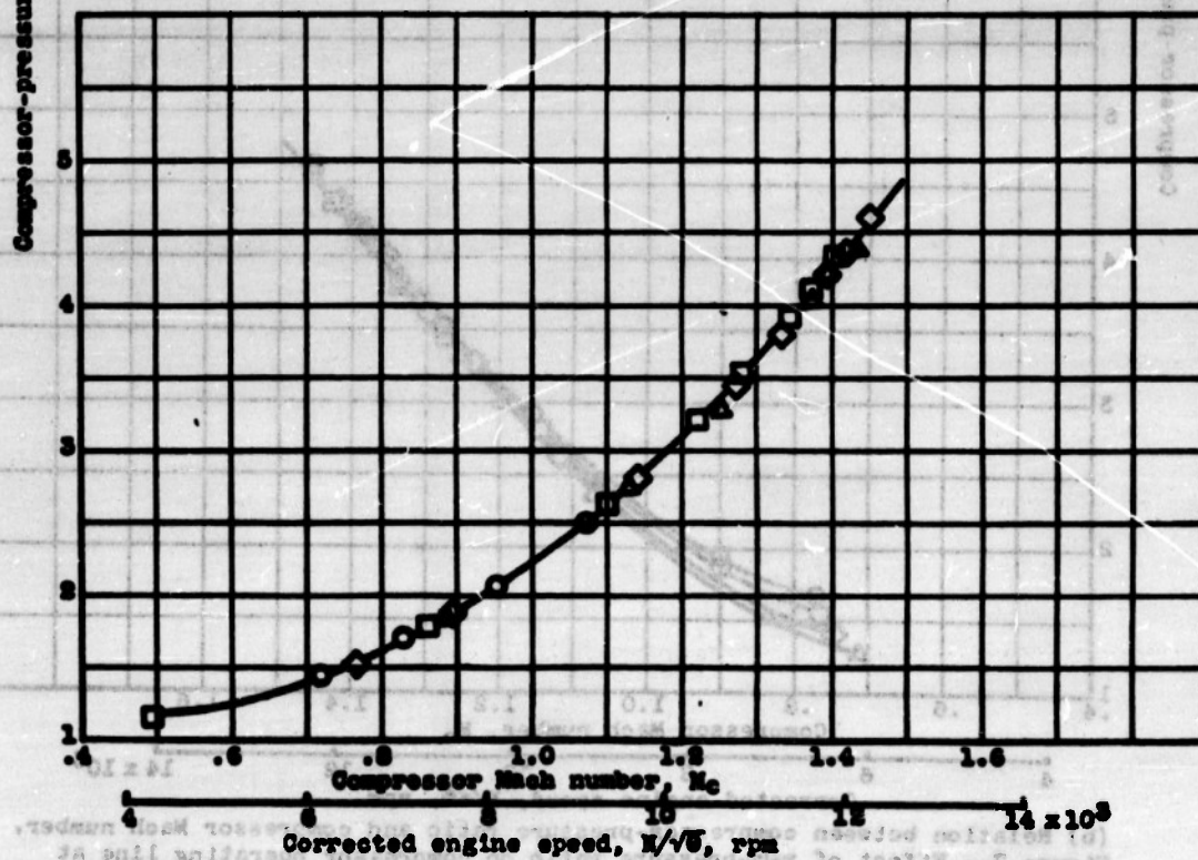
(b) Relation between compressor-pressure ratio and compressor Mach number. Figure 6.- Effect of altitude on compressor operating line at ram-pressure ratio of 1.20.
