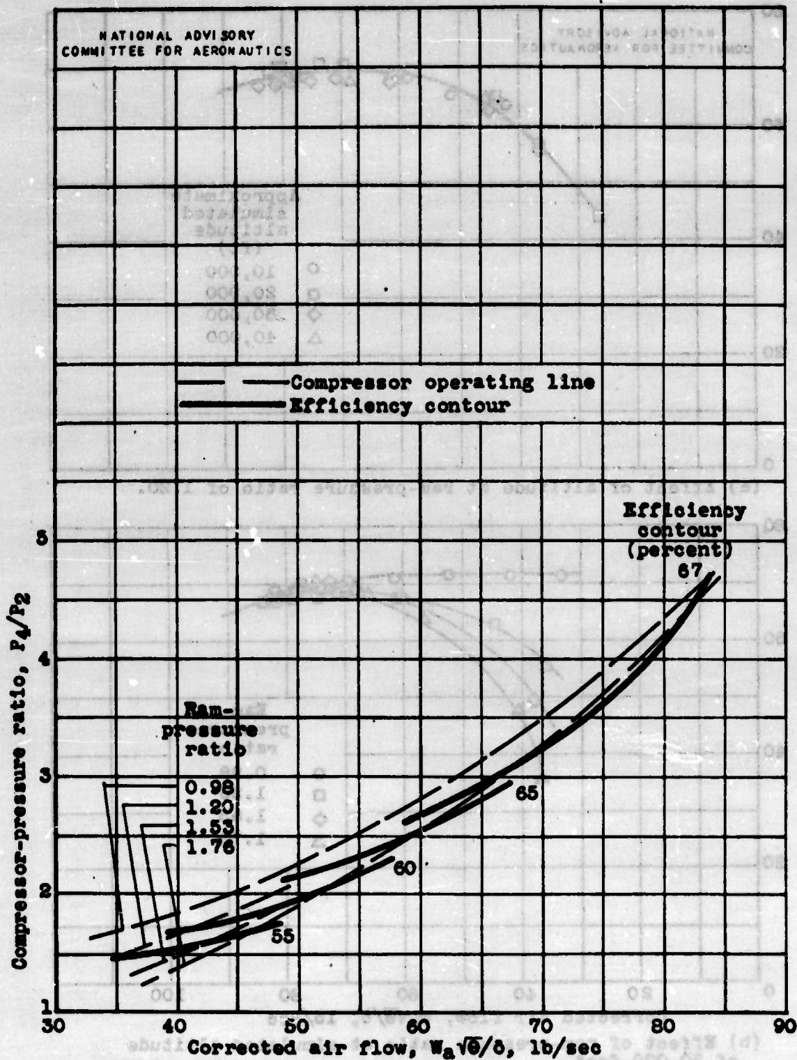
Figure 9.- Adiabatic temperature-rise efficiency characteristics at simulated altitude of 30,000 feet.
