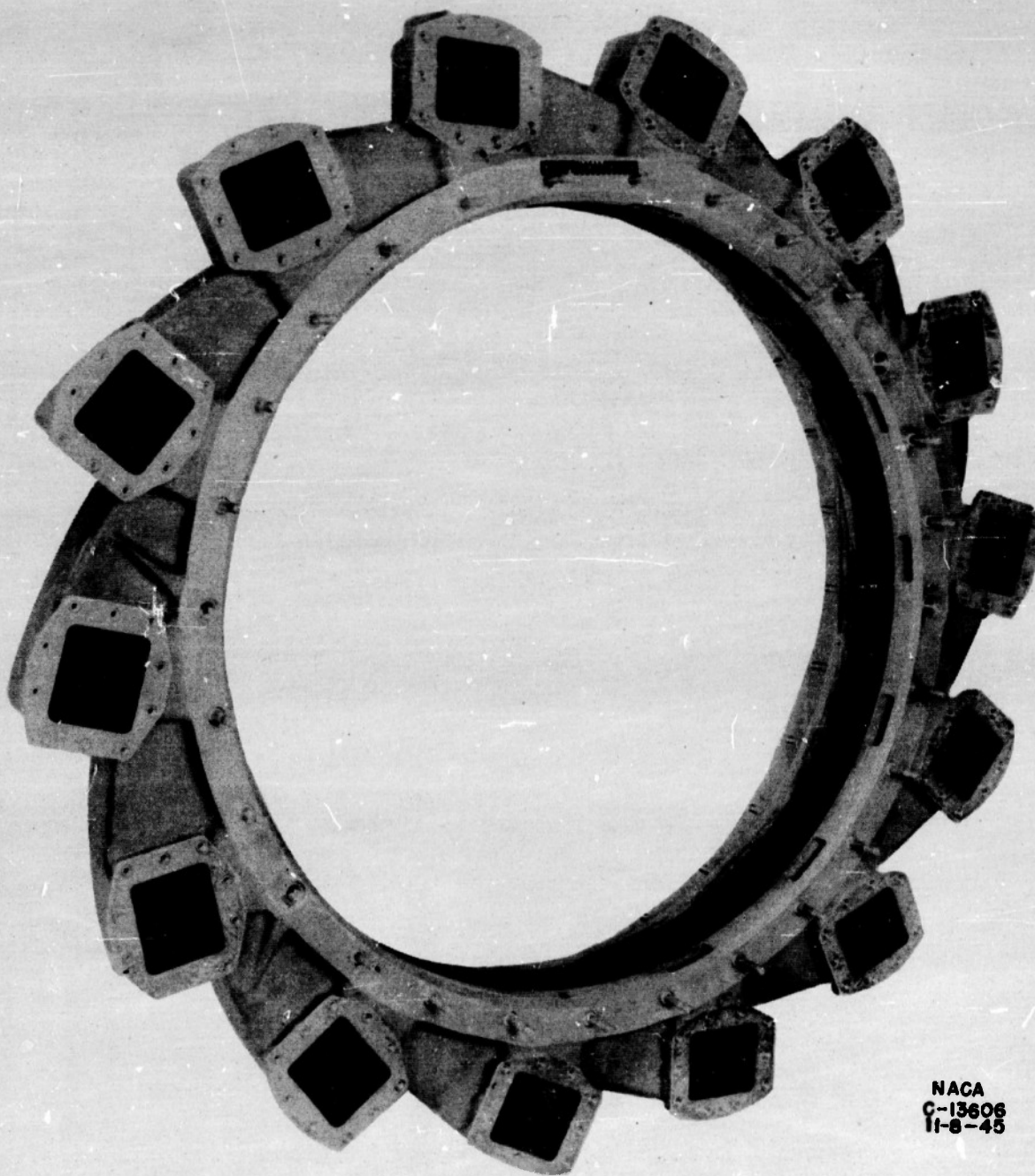
Figure 3. - General Electric I-40 diffuser showing vanes around periphery and turning vanes in diffuser elbows.
