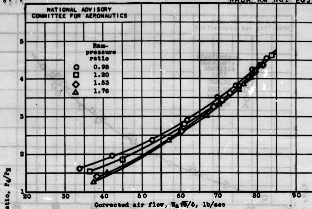
(a) Relation between compressor-pressure ratio and corrected air flow.
