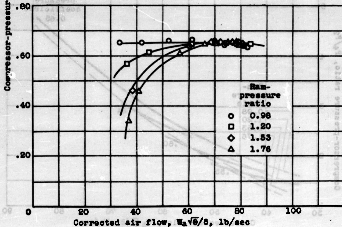
(b) Effect of ram-pressure ratio at simulated altitude of 30,000 feet.
