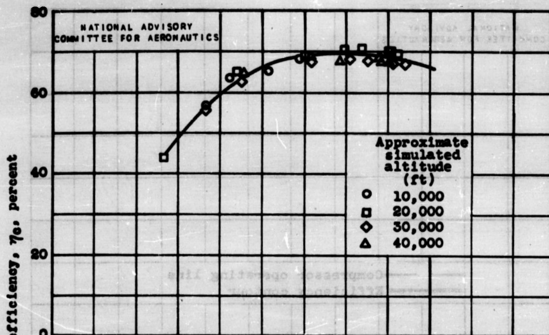
(a) Effect of altitude at ram-pressure ratio of 1.20.
