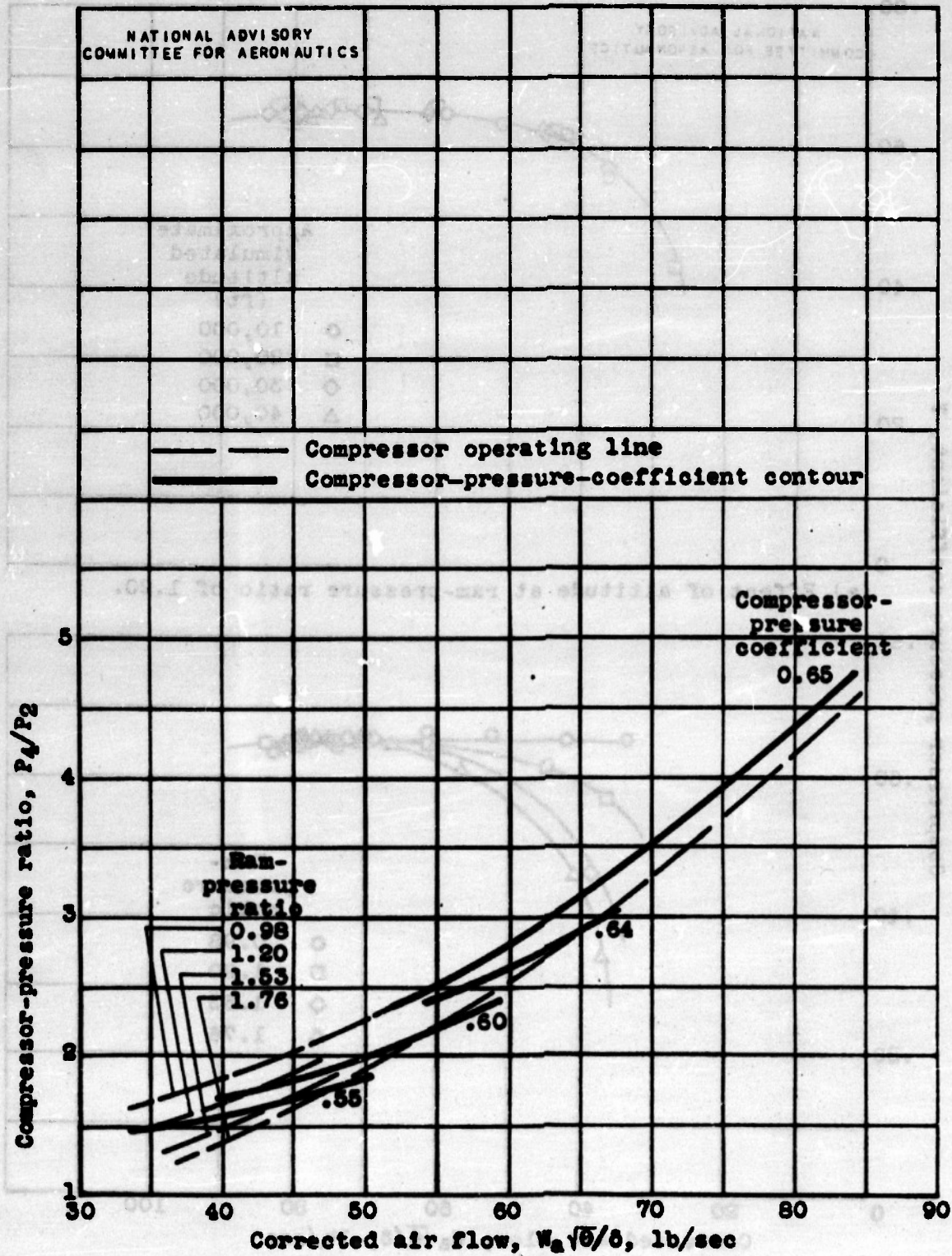
Figure 11.- Pressure-coefficient contours at simulated altitude of 30,000 feet.
